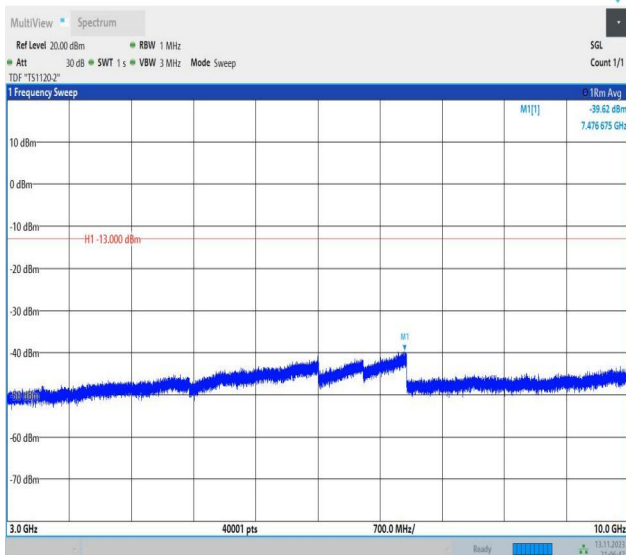
Band26_3MHz_QPSK_26805_1RB#0_3000~10000_3000~10000
