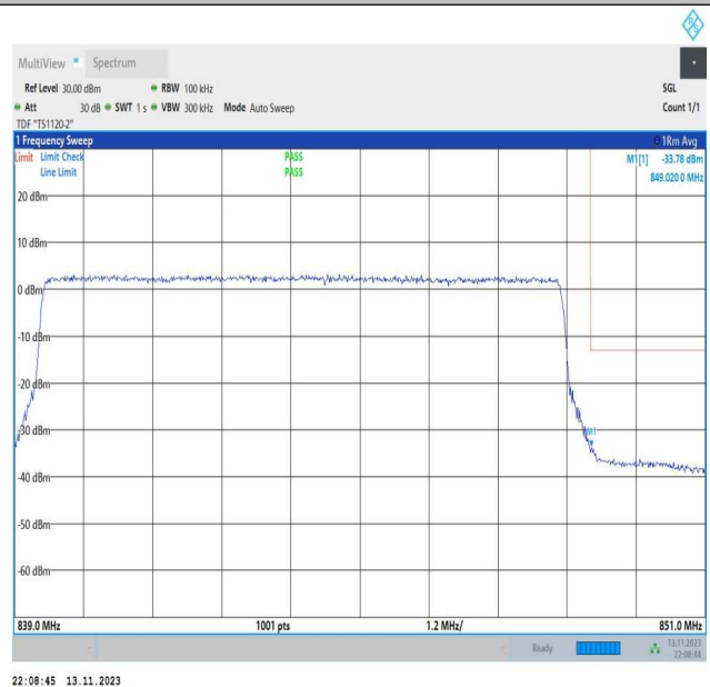
Band26_10MHz_16QAM_26990_50RB#0
