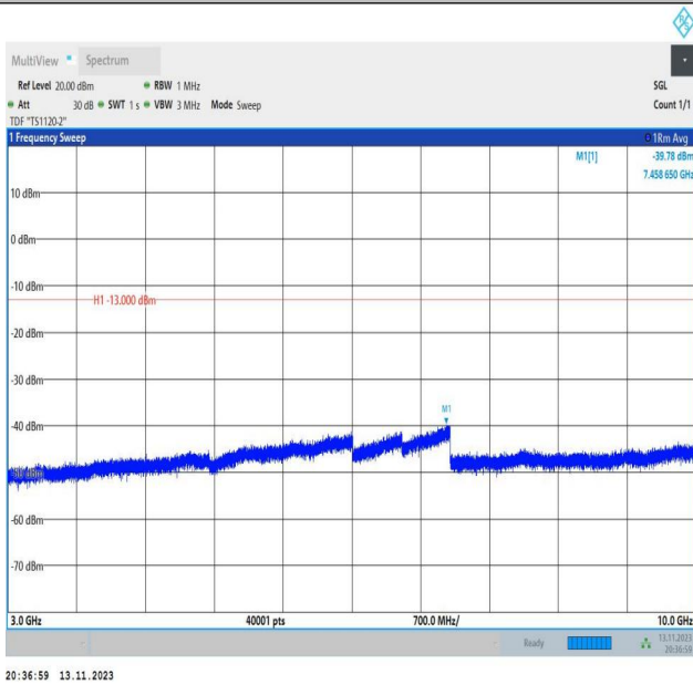
Band26_1.4MHz_QPSK_26915_1RB#0_3000~10000_3000~10000
