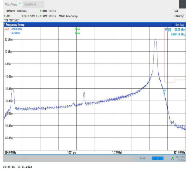
Band26_15MHz_16QAM_26965_1RB#74
