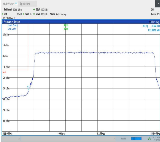
Band26_10MHz_QPSK_26840_50RB#0
