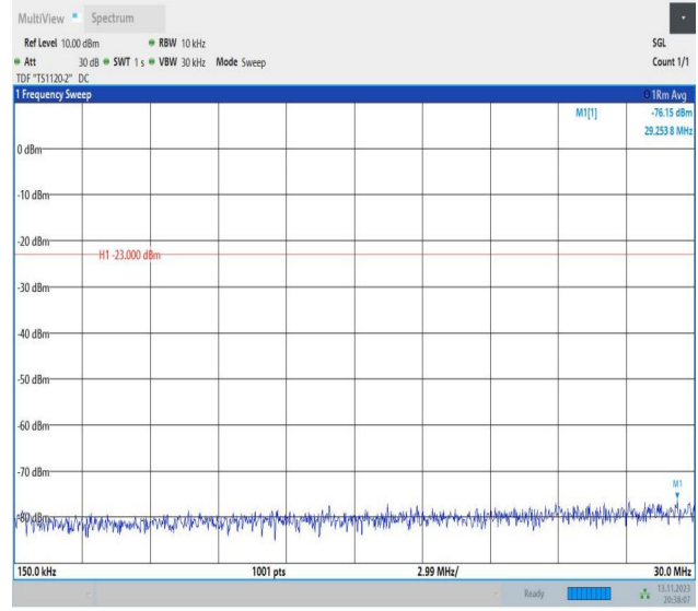
Band26_1.4MHz_QPSK_27033_1RB#0_0.15~30_0.15~30
