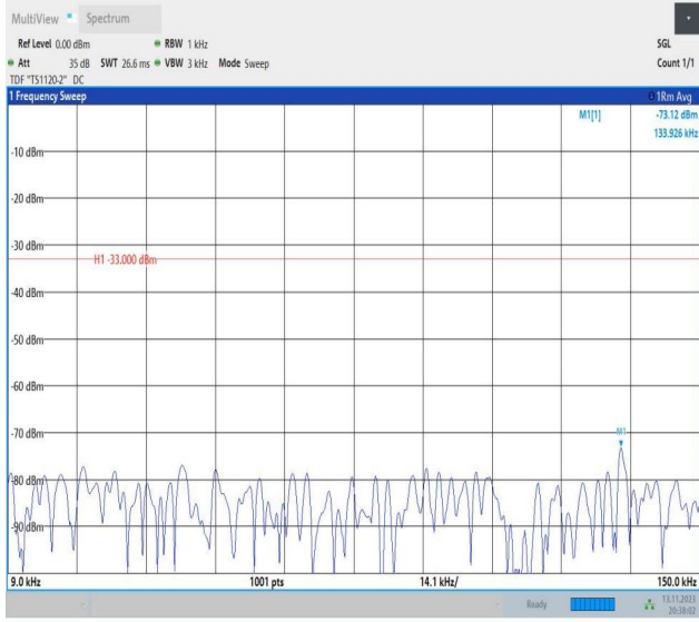
Band26_1.4MHz_QPSK_27033_1RB#0_0.009~0.15_0.009~0.15
