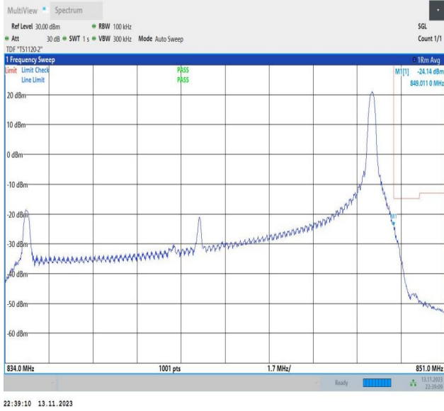
Band26_15MHz_QPSK_26965_1RB#74
