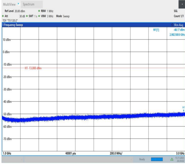
Band26_1.4MHz_16QAM_27033_1RB#0_1000~3000_1000~3000
