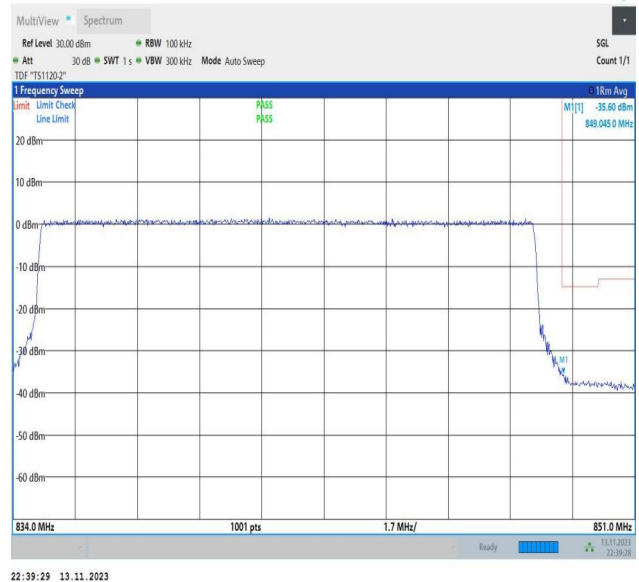
Band26_15MHz_16QAM_26965_75RB#0
