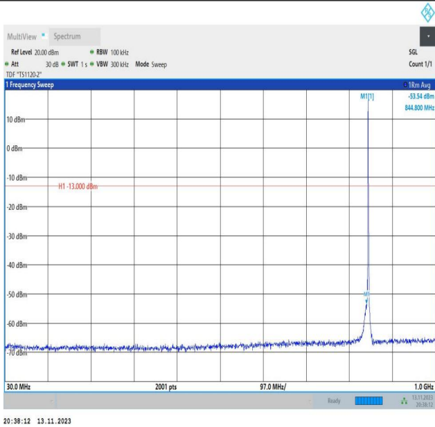
Band26_1.4MHz_QPSK_27033_1RB#0_30~1000_30~1000
