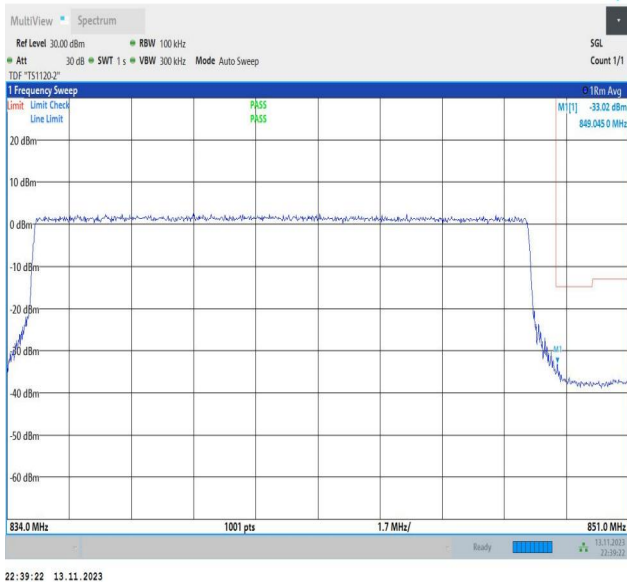
Band26_15MHz_QPSK_26965_75RB#0
