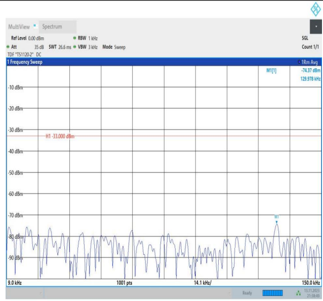
Band26_5MHz_16QAM_26815_1RB#0_0.009~0.15_0.009~0.15
