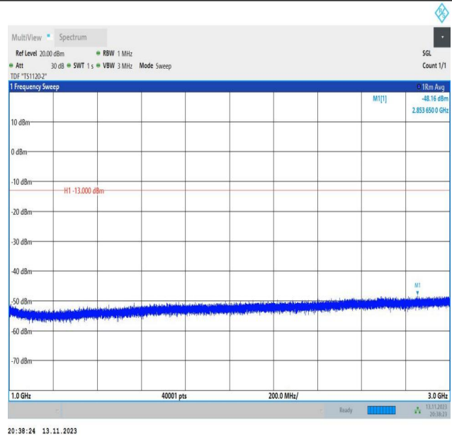
Band26_1.4MHz_QPSK_27033_1RB#0_1000~3000_1000~3000
