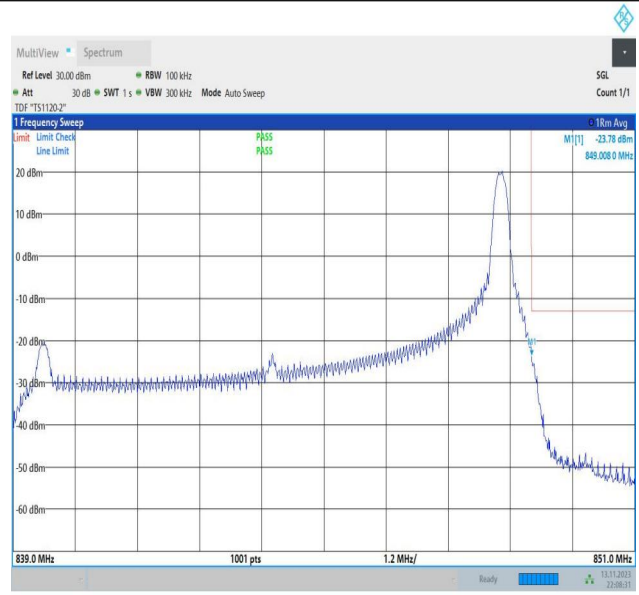
Band26_10MHz_16QAM_26990_1RB#49
