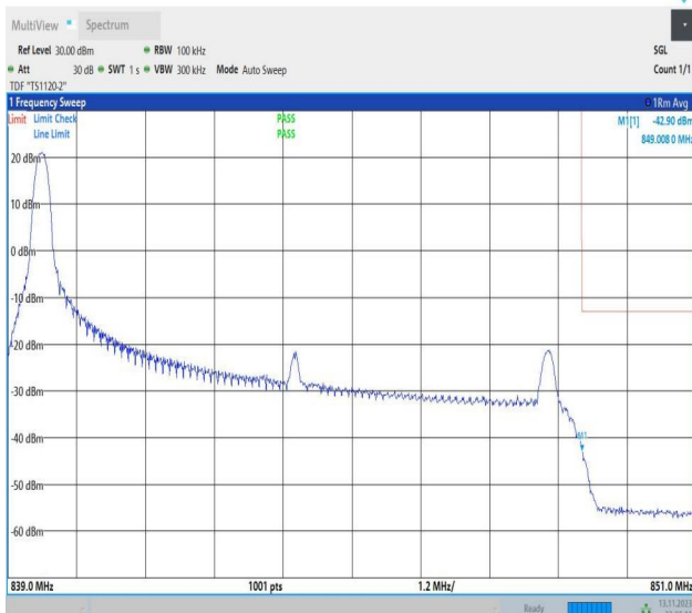
Band26_10MHz_QPSK_26990_1RB#0
