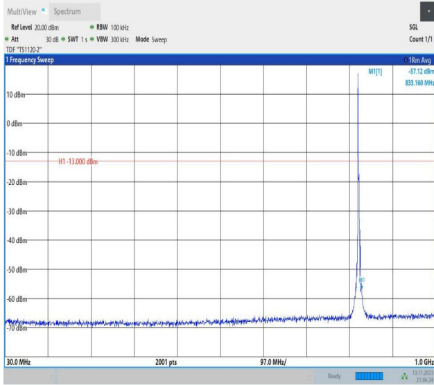
Band26_3MHz_QPSK_26805_1RB#0_30~1000_30~1000
