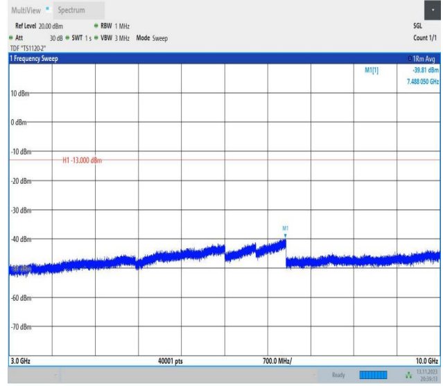
Band26_1.4MHz_16QAM_27033_1RB#0_3000~10000_3000~10000
