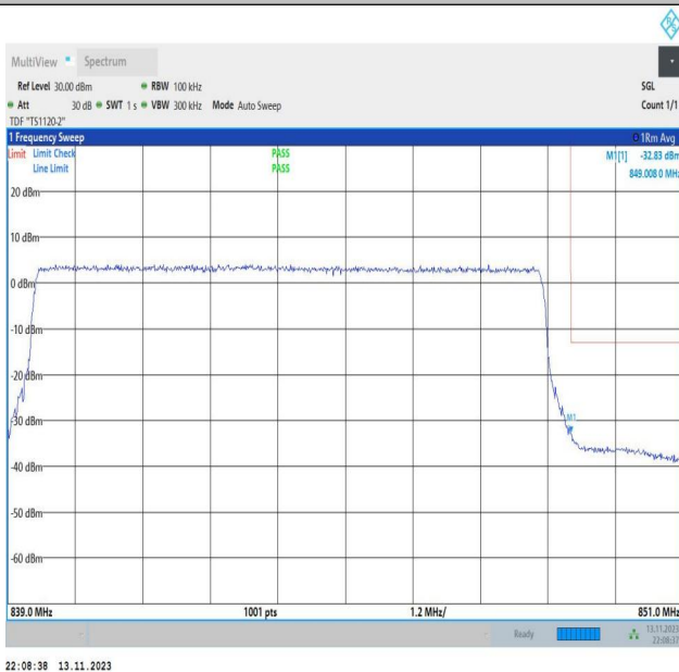
Band26_10MHz_QPSK_26990_50RB#0
