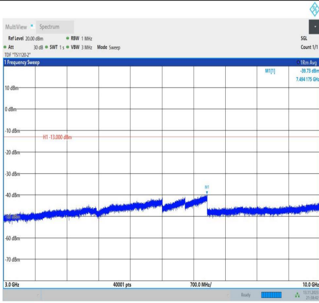
Band26_5MHz_QPSK_26815_1RB#0_3000~10000_3000~10000
