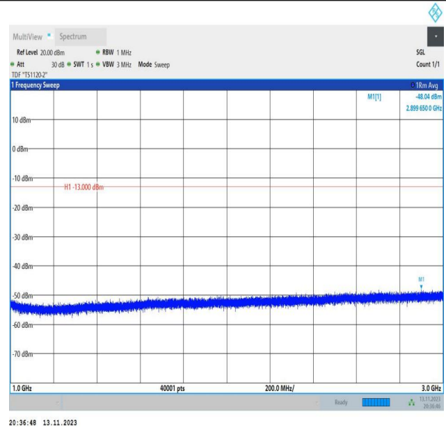
Band26_1.4MHz_QPSK_26915_1RB#0_1000~3000_1000~3000
