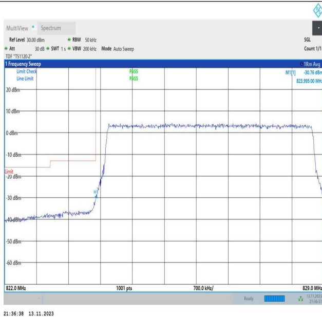
Band26_5MHz_QPSK_26815_25RB#0
