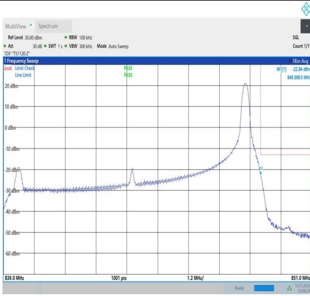
Band26_10MHz_QPSK_26990_1RB#49
