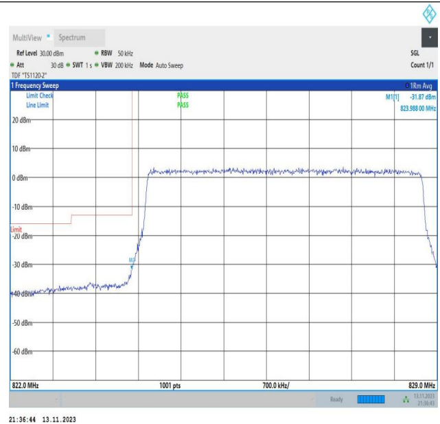
Band26_5MHz_16QAM_26815_25RB#0
