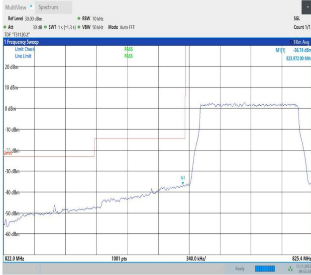
Band5_1.4MHz_QPSK_20407_6RB#0
