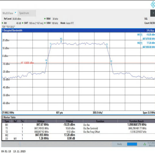
Band5-1.4MHz-QPSK-20643-6RB#0-PASS
