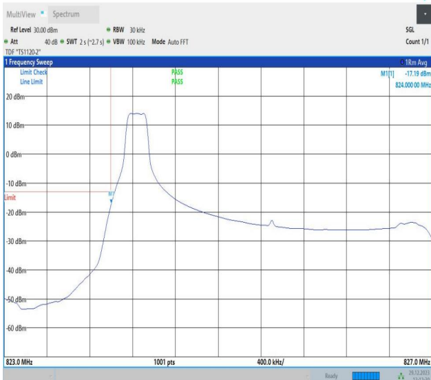
Band5_3MHz_64QAM_20415_1RB#0
