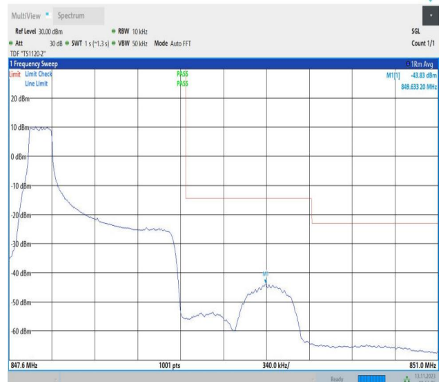
Band5_1.4MHz_16QAM_20643_1RB#0
