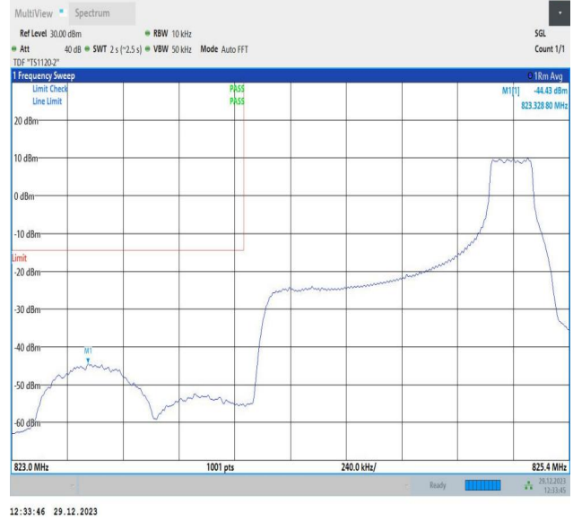
Band5_1.4MHz_64QAM_20407_1RB#5
