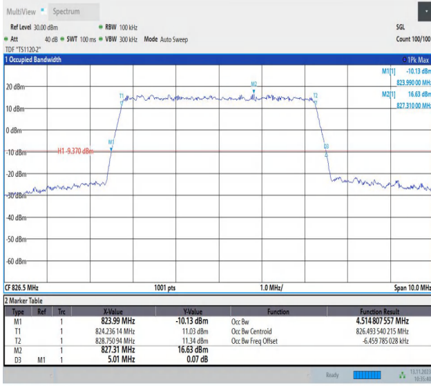
Band5-5MHz-QPSK-20425-25RB#0-PASS
