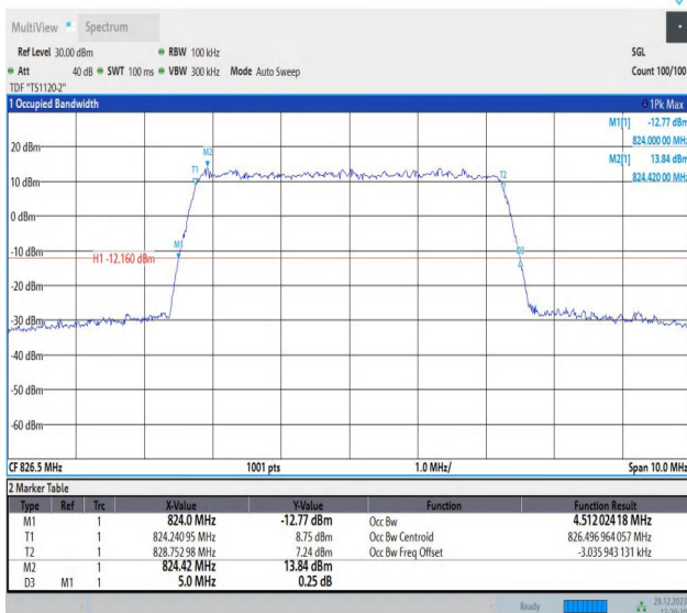
Band5-5MHz-64QAM-20425-25RB#0-PASS
