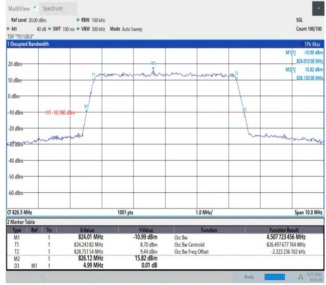
Band5-5MHz-16QAM-20425-25RB#0-PASS
