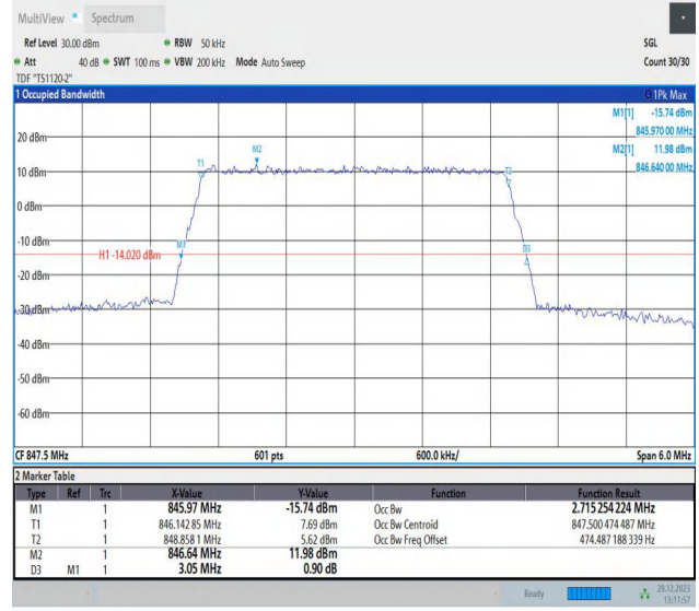
Band5-3MHz-64QAM-20635-15RB#0-PASS
