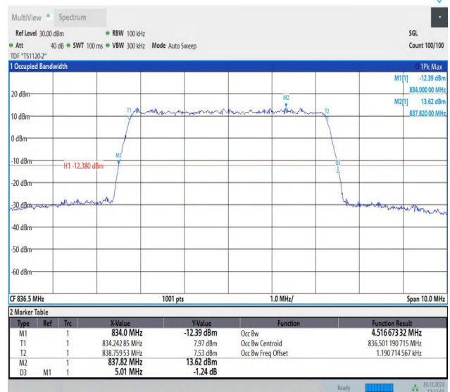
Band5-5MHz-64QAM-20525-25RB#0-PASS
