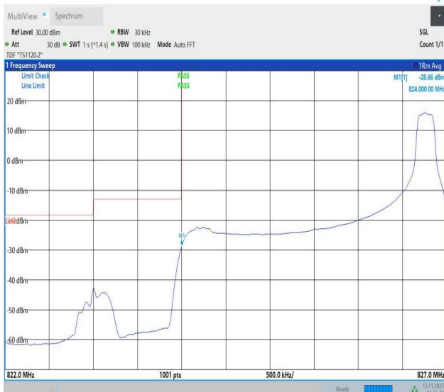
Band5_3MHz_QPSK_20415_1RB#14
