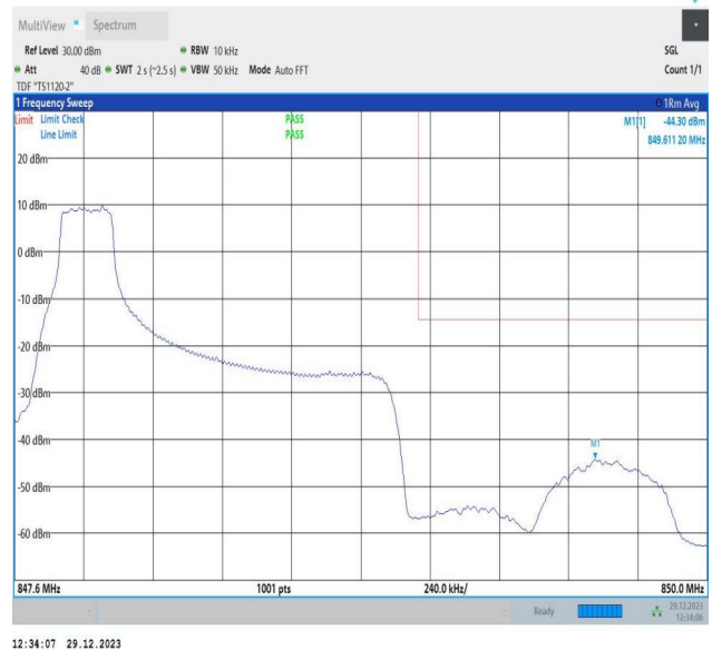
Band5_1.4MHz_64QAM_20643_1RB#0
