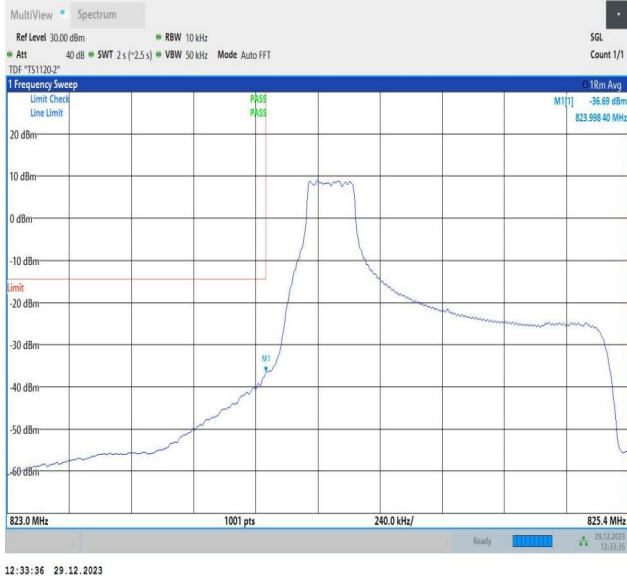
Band5_1.4MHz_64QAM_20407_1RB#0
