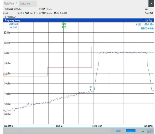
Band5_1.4MHz_16QAM_20407_6RB#0
