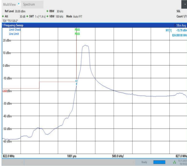
Band5_3MHz_QPSK_20415_1RB#0
