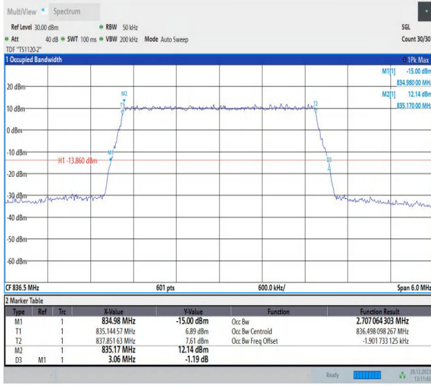
Band5-3MHz-64QAM-20525-15RB#0-PASS
