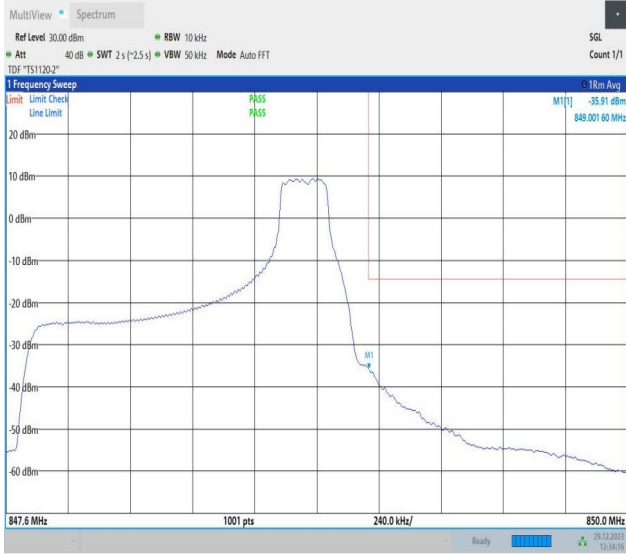
Band5_1.4MHz_64QAM_20643_1RB#5
