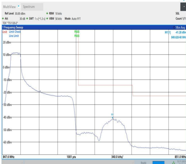
Band5_1.4MHz_QPSK_20643_1RB#0
