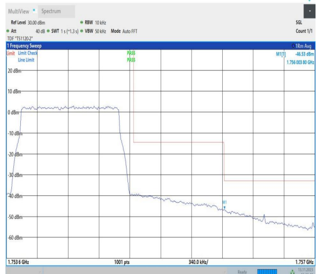
Band4_1.4MHz_16QAM_20393_6RB#0
