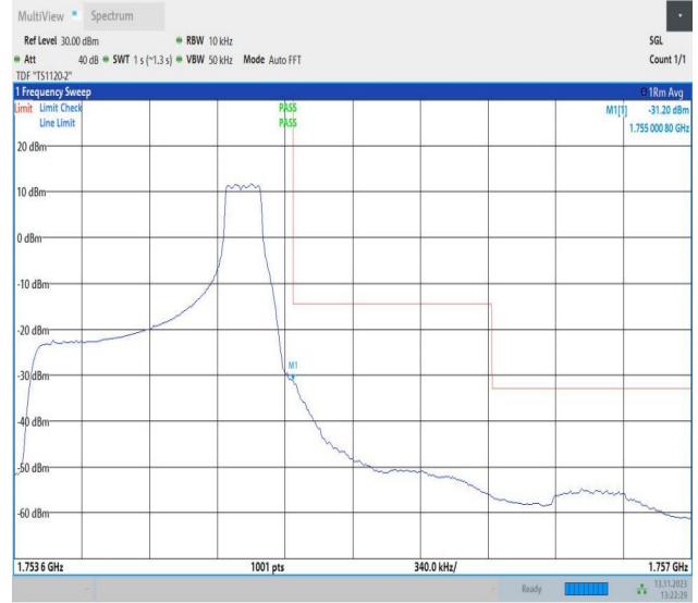
Band4_1.4MHz_16QAM_20393_1RB#5
