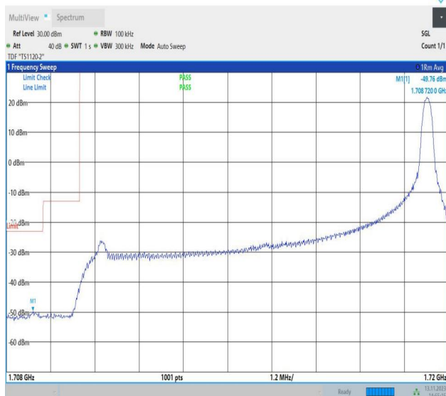
Band4_10MHz_QPSK_20000_1RB#49
