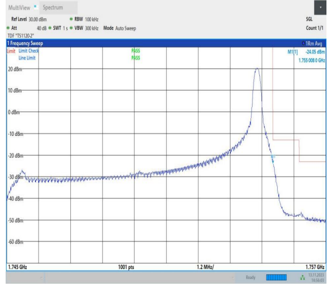
Band4_10MHz_16QAM_20350_1RB#49
