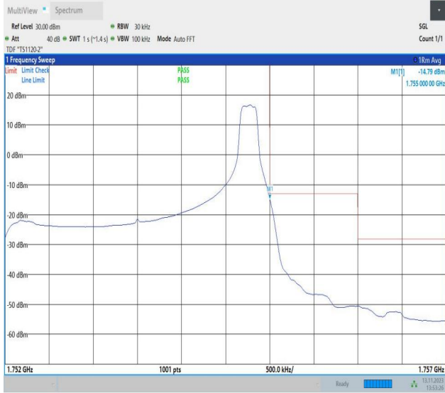
Band4_3MHz_QPSK_20385_1RB#14
