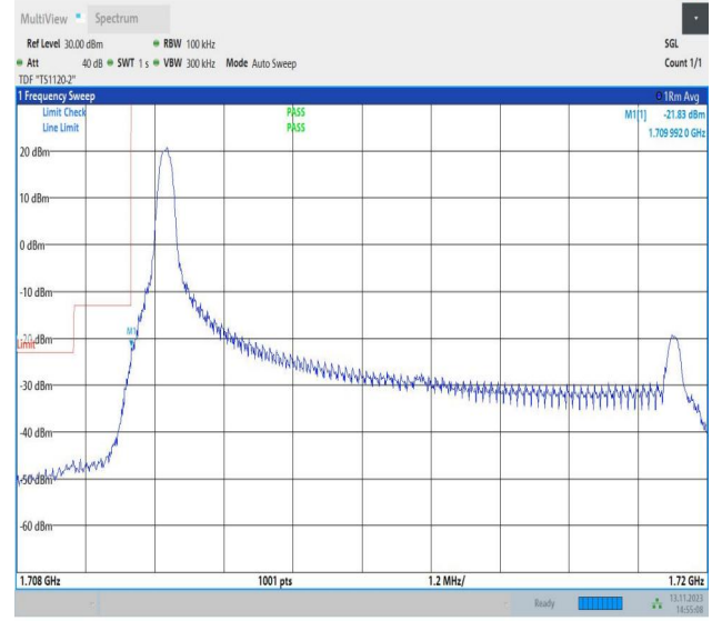
Band4_10MHz_16QAM_20000_1RB#0
