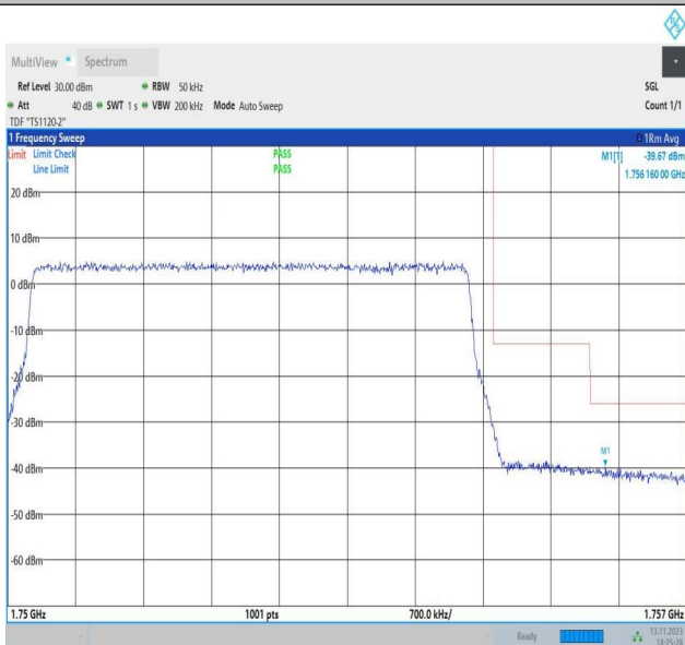
Band4_5MHz_QPSK_20375_1RB#24
