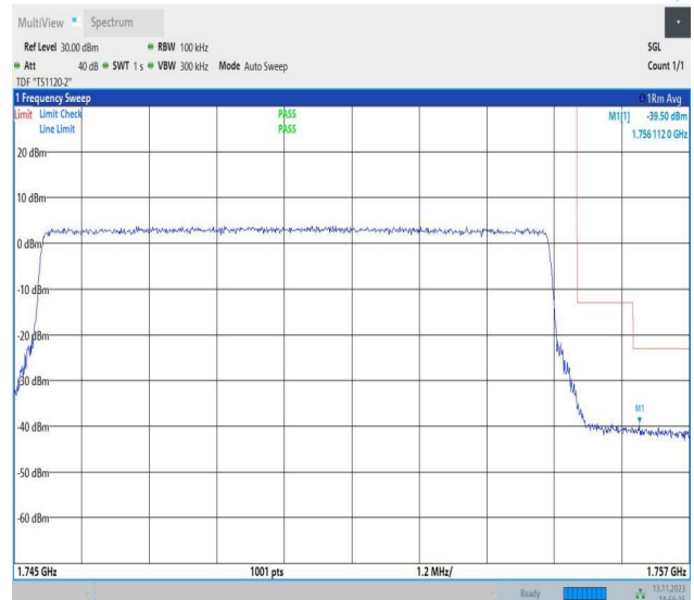
Band4_10MHz_16QAM_20350_50RB#0
