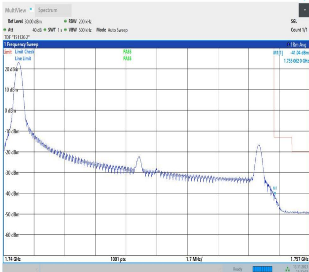
Band4_15MHz_QPSK_20325_1RB#0
