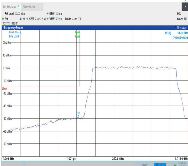
Band4_1.4MHz_64QAM_19957_6RB#0
