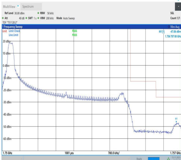
Band4_5MHz_QPSK_20375_1RB#0
