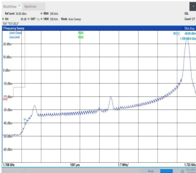
Band4_15MHz_QPSK_20025_1RB#74
