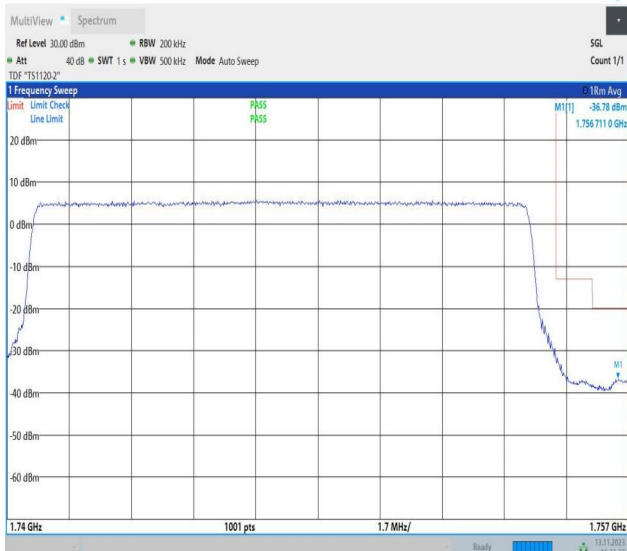
Band4_15MHz_QPSK_20325_75RB#0
