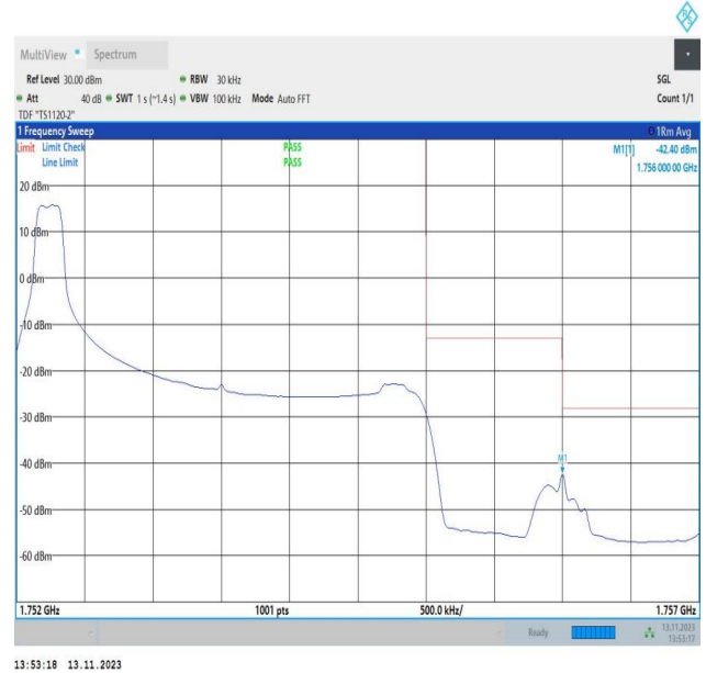
Band4_3MHz_16QAM_20385_1RB#0
