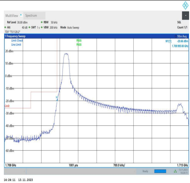
Band4_5MHz_16QAM_19975_1RB#0
