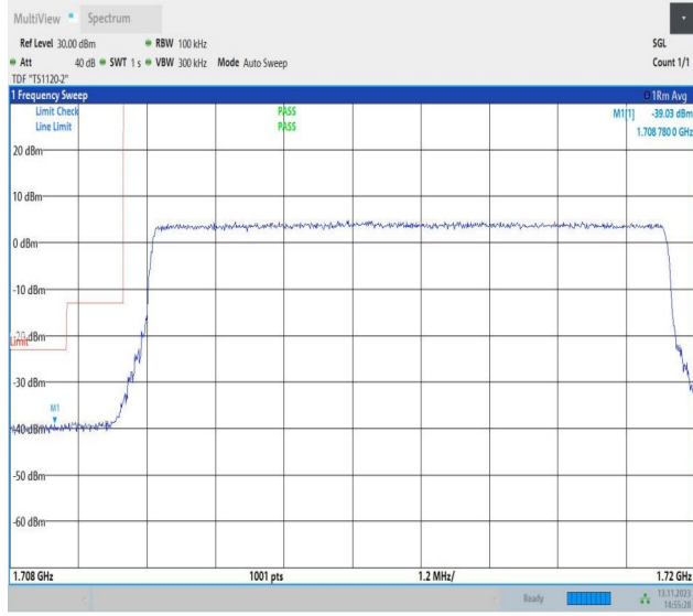
Band4_10MHz_QPSK_20000_50RB#0
