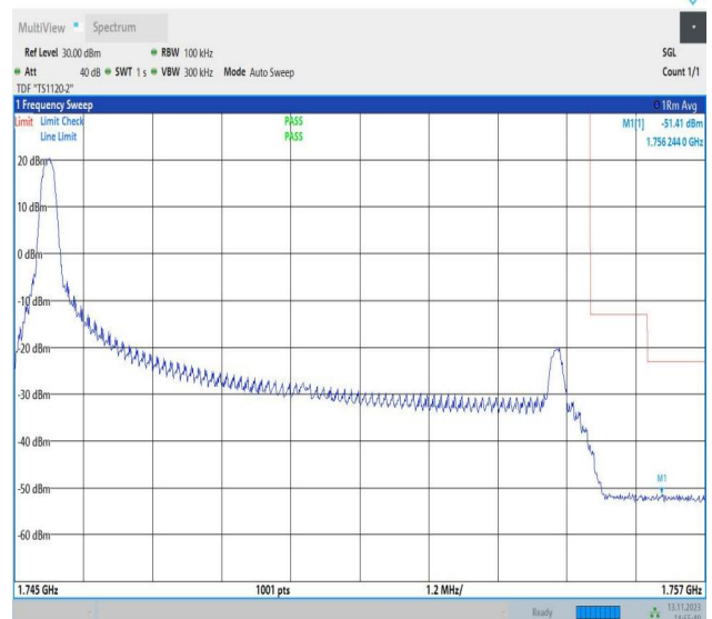
Band4_10MHz_16QAM_20350_1RB#0
