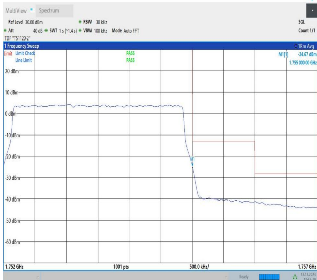
Band4_3MHz_QPSK_20385_15RB#0
