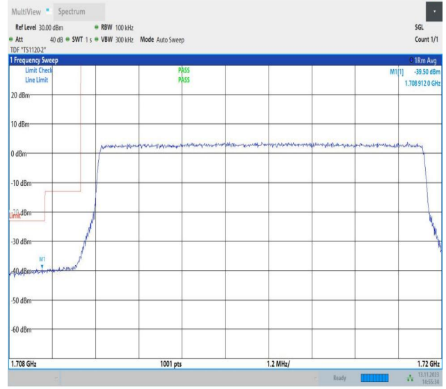
Band4_10MHz_16QAM_20000_50RB#0
