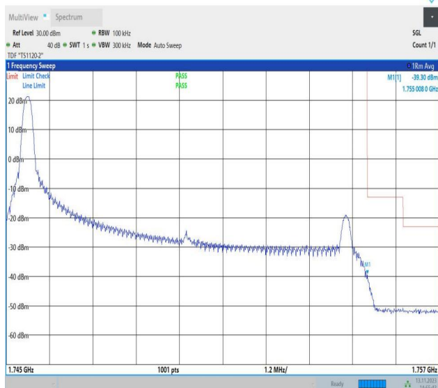
Band4_10MHz_QPSK_20350_1RB#0
