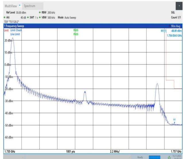
Band4_20MHz_16QAM_20300_1RB#0
