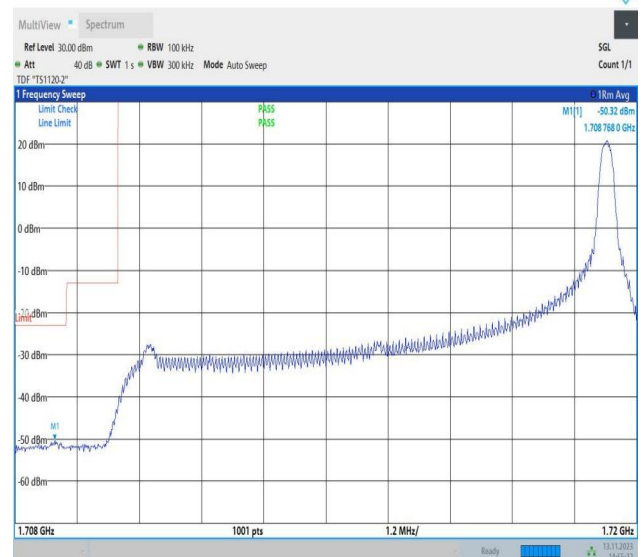
Band4_10MHz_16QAM_20000_1RB#49
