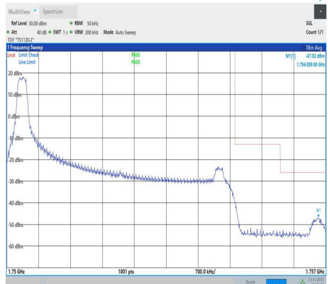
Band4_5MHz_16QAM_20375_1RB#0
