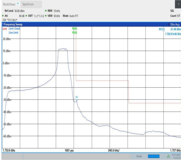
Band4_1.4MHz_QPSK_20393_1RB#5
