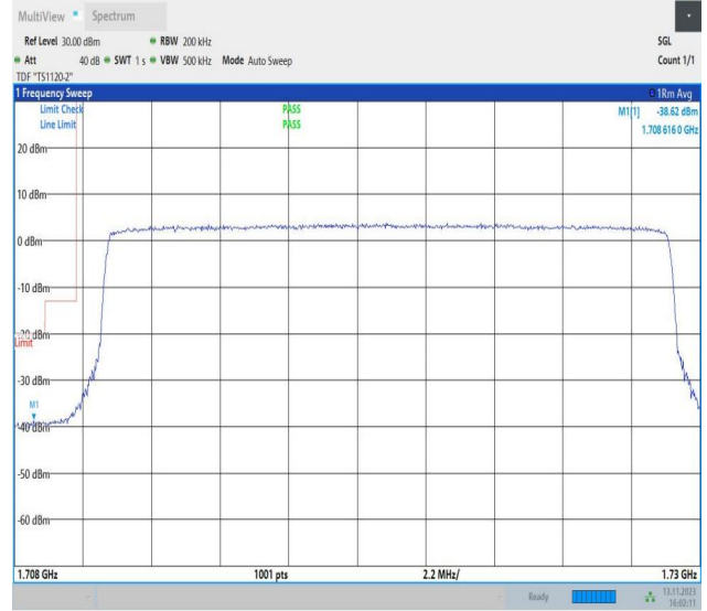
Band4_20MHz_16QAM_20050_100RB#0
