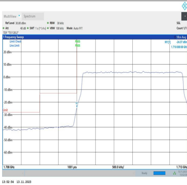
Band4_3MHz_QPSK_19965_15RB#0
