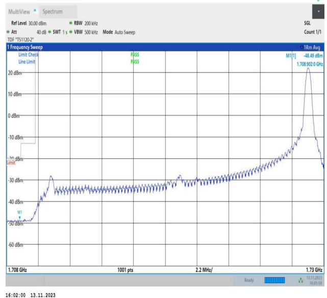
Band4_20MHz_16QAM_20050_1RB#99
