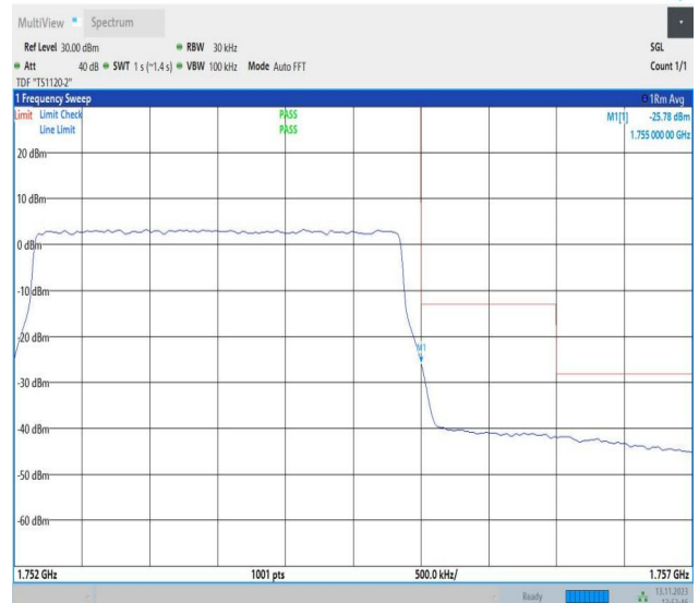
Band4_3MHz_16QAM_20385_15RB#0
