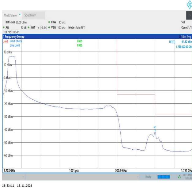
Band4_3MHz_QPSK_20385_1RB#0
