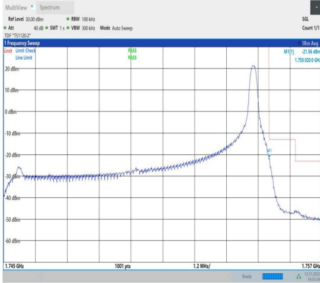
Band4_10MHz_QPSK_20350_1RB#49
