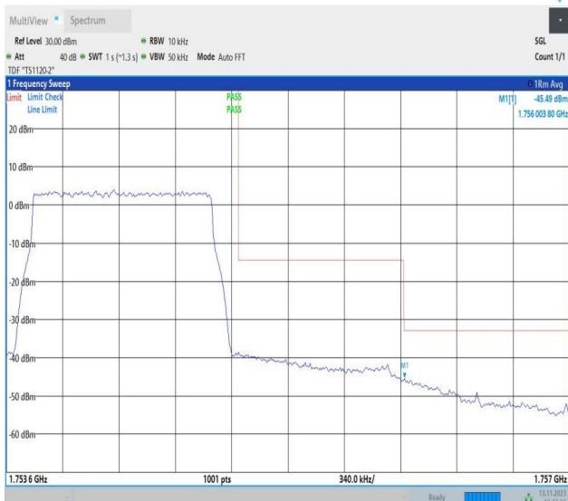
Band4_1.4MHz_QPSK_20393_6RB#0
