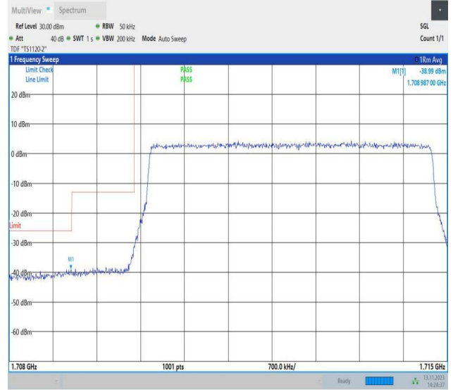
Band4_5MHz_16QAM_19975_25RB#0
