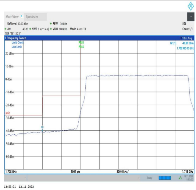
Band4_3MHz_16QAM_19965_15RB#0
