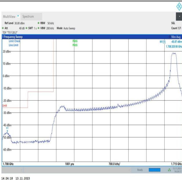
Band4_5MHz_QPSK_19975_1RB#24
