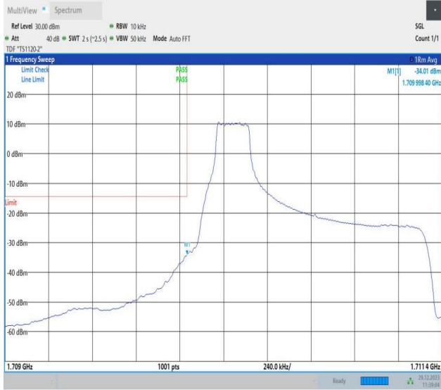
Band4_1.4MHz_64QAM_19957_1RB#0
