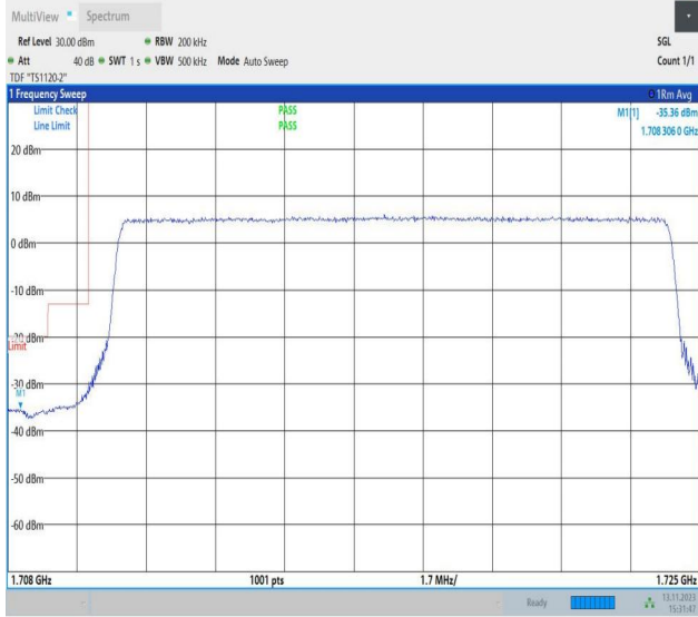
Band4_15MHz_QPSK_20025_75RB#0
