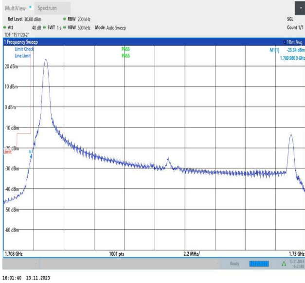
Band4_20MHz_QPSK_20050_1RB#0
