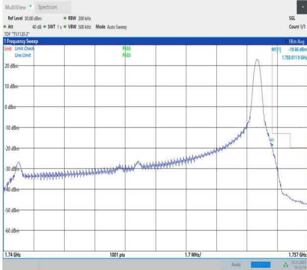
Band4_15MHz_QPSK_20325_1RB#74
