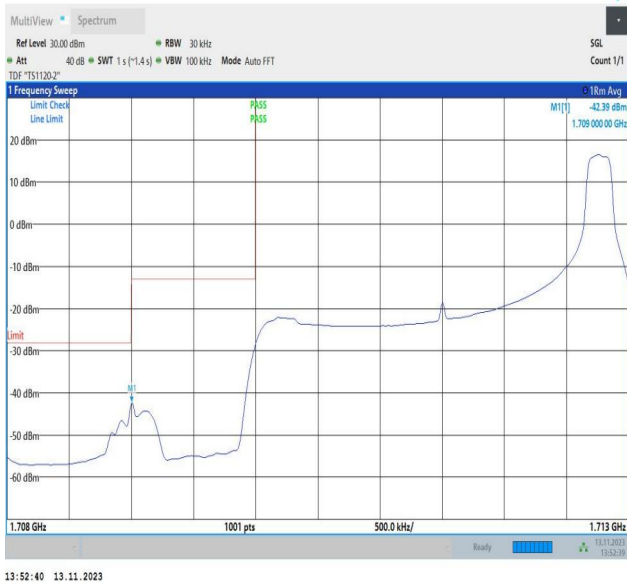
Band4_3MHz_QPSK_19965_1RB#14
