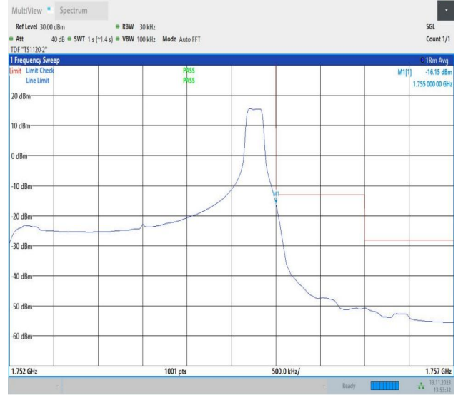
Band4_3MHz_16QAM_20385_1RB#14
