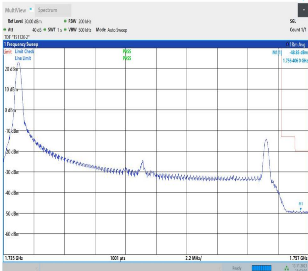
Band4_20MHz_QPSK_20300_1RB#0
