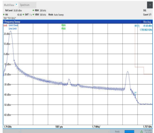
Band4_15MHz_16QAM_20325_1RB#0
