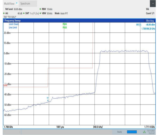
Band4_1.4MHz_16QAM_19957_6RB#0
