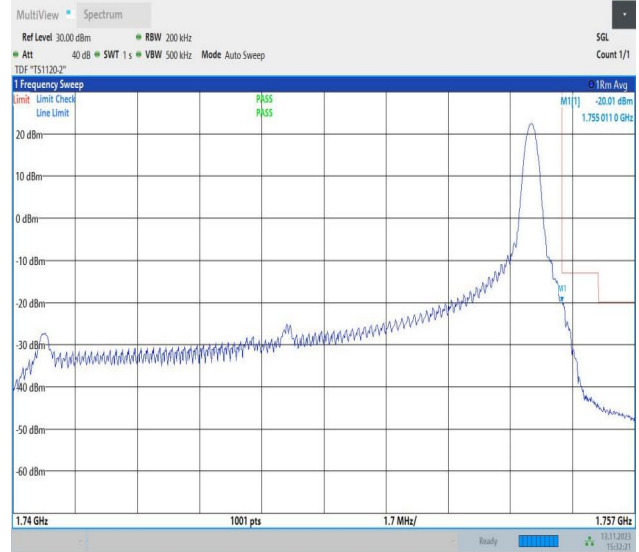
Band4_15MHz_16QAM_20325_1RB#74
