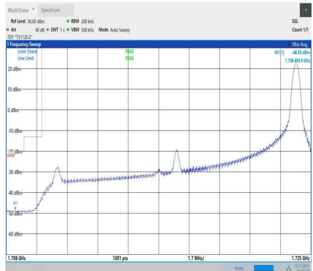
Band4_15MHz_16QAM_20025_1RB#74
