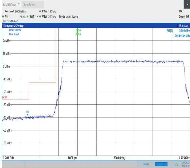
Band4_5MHz_QPSK_19975_25RB#0
