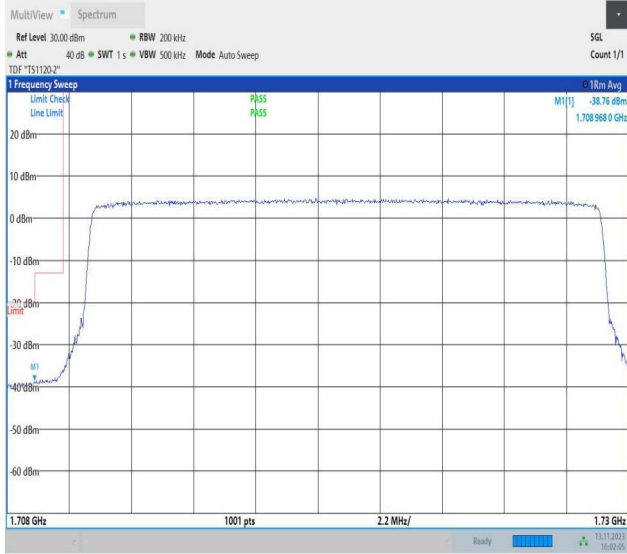
Band4_20MHz_QPSK_20050_100RB#0
