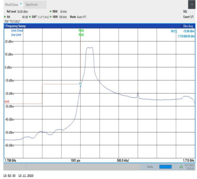
Band4_3MHz_16QAM_19965_1RB#0
