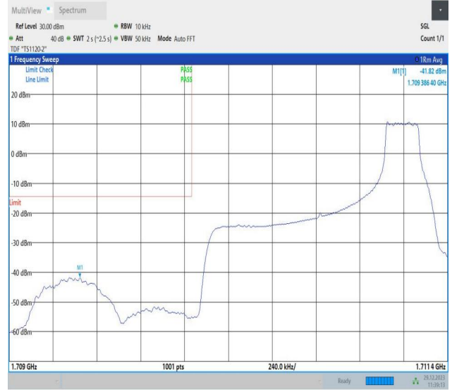
Band4_1.4MHz_64QAM_19957_1RB#5
