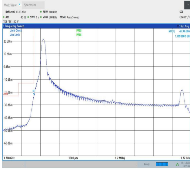
Band4_10MHz_QPSK_20000_1RB#0
