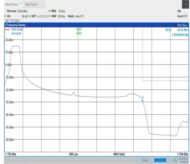
Band4_3MHz_64QAM_20385_1RB#0
