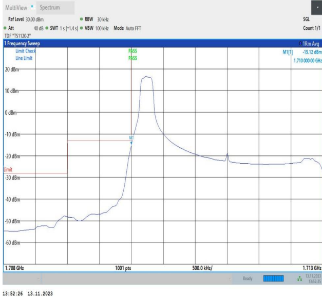
Band4_3MHz_QPSK_19965_1RB#0
