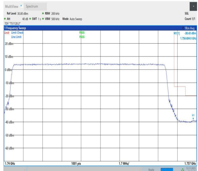
Band4_15MHz_16QAM_20325_75RB#0
