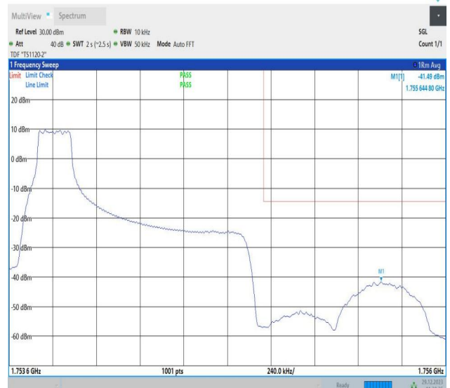
Band4_1.4MHz_64QAM_20393_1RB#0
