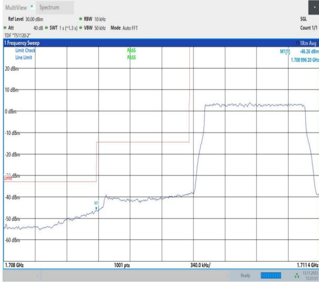
Band4_1.4MHz_QPSK_19957_6RB#0
