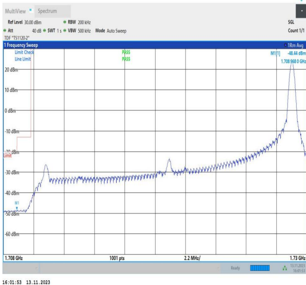
Band4_20MHz_QPSK_20050_1RB#99
