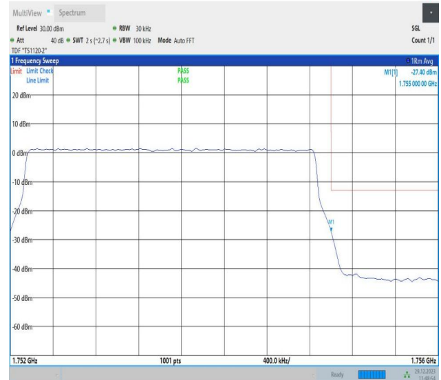
Band4_3MHz_64QAM_20385_15RB#0
