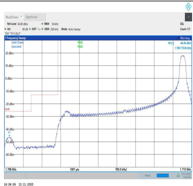
Band4_5MHz_16QAM_19975_1RB#24
