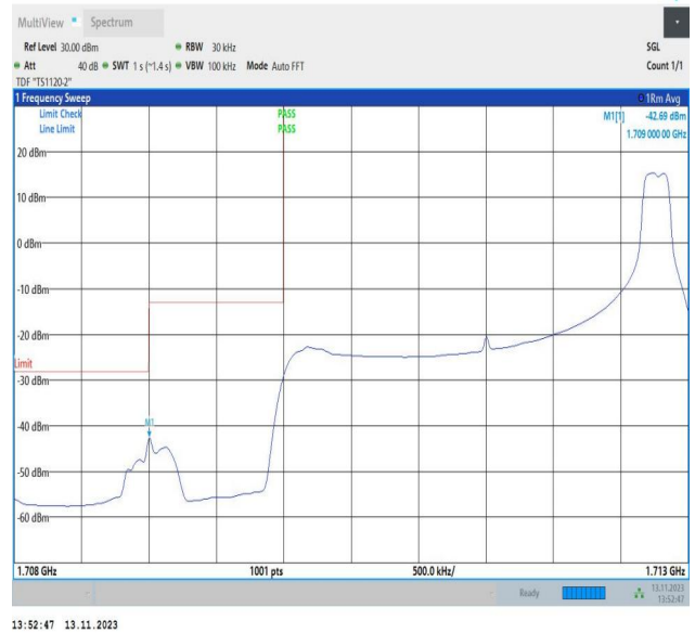
Band4_3MHz_16QAM_19965_1RB#14
