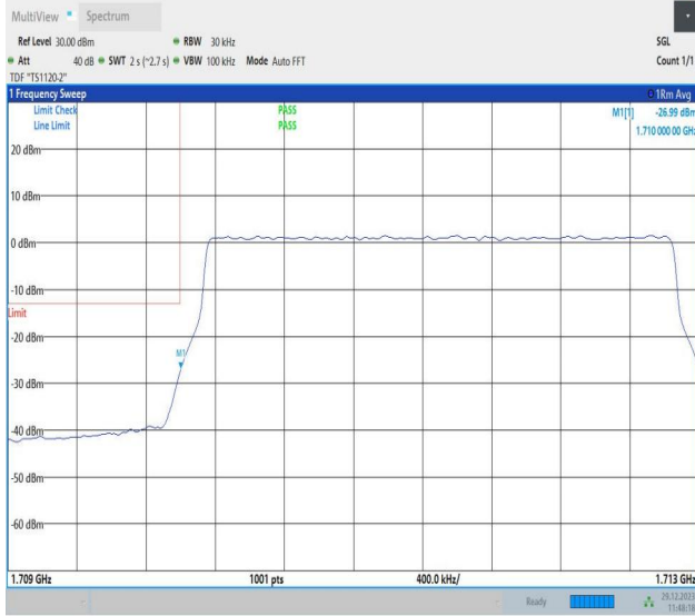
Band4_3MHz_64QAM_19965_15RB#0
