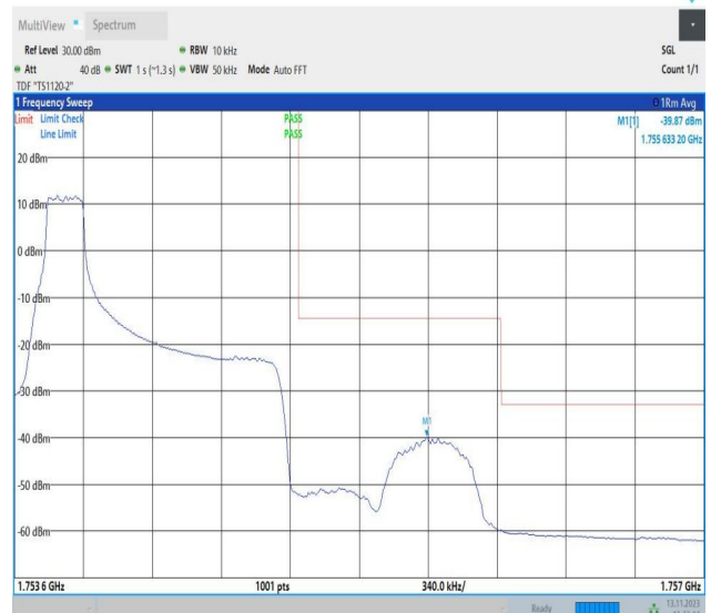
Band4_1.4MHz_16QAM_20393_1RB#0
