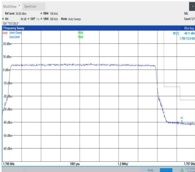
Band4_10MHz_QPSK_20350_50RB#0
