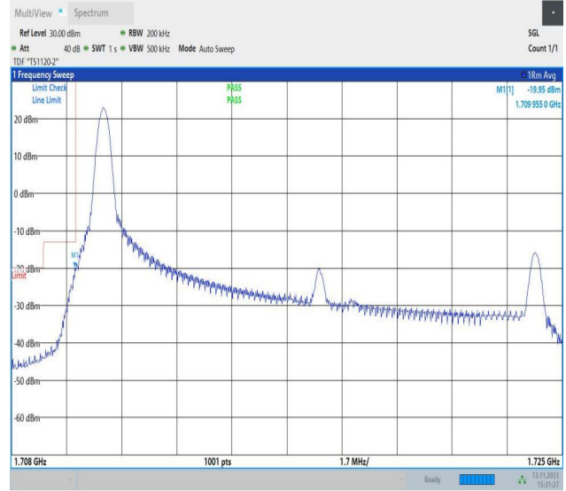
Band4_15MHz_16QAM_20025_1RB#0
