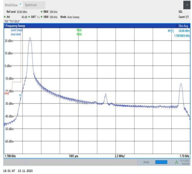
Band4_20MHz_16QAM_20050_1RB#0
