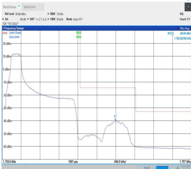
Band4_1.4MHz_QPSK_20393_1RB#0
