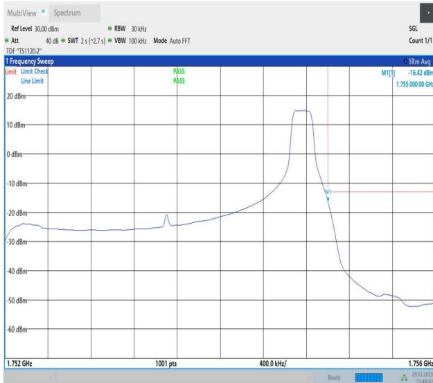
Band4_3MHz_64QAM_20385_1RB#14
