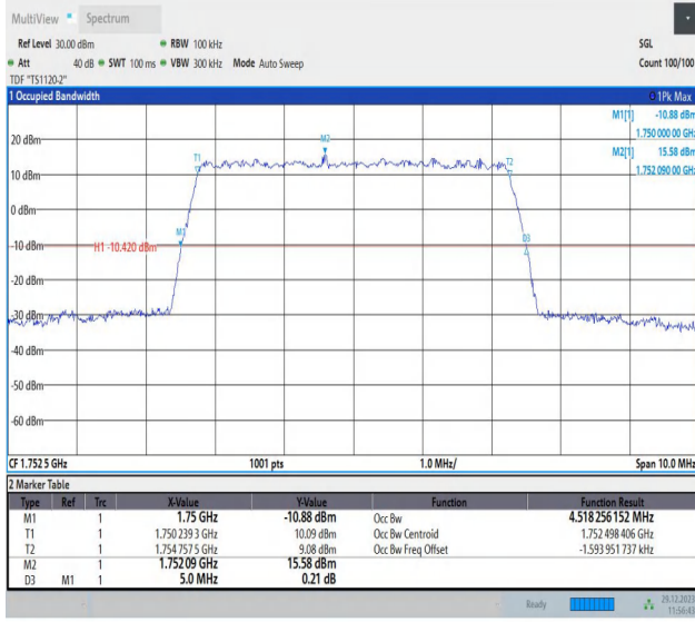
Band4-5MHz-64QAM-20375-25RB#0-PASS
