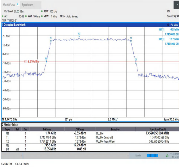
Band4-15MHz-QPSK-20325-75RB#0-PASS
