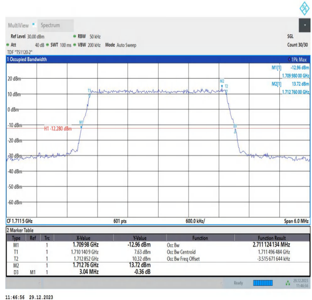
Band4-3MHz-64QAM-19965-15RB#0-PASS
