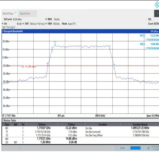
Band4-1.4MHz-64QAM-19957-6RB#0-PASS
