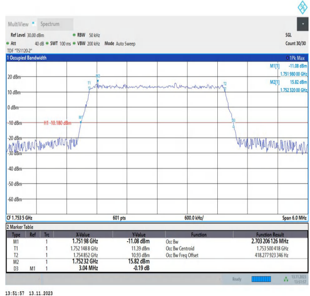
Band4-3MHz-16QAM-20385-15RB#0-PASS
