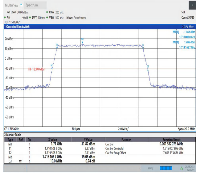
Band4-10MHz-64QAM-20000-50RB#0-PASS
