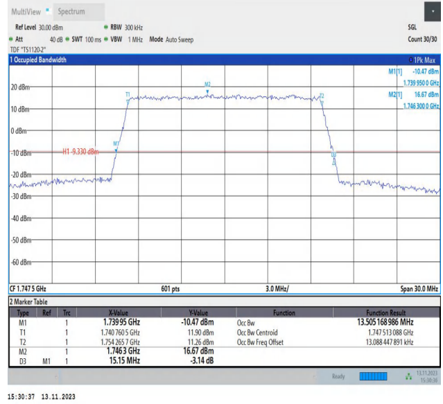
Band4-15MHz-16QAM-20325-75RB#0-PASS
