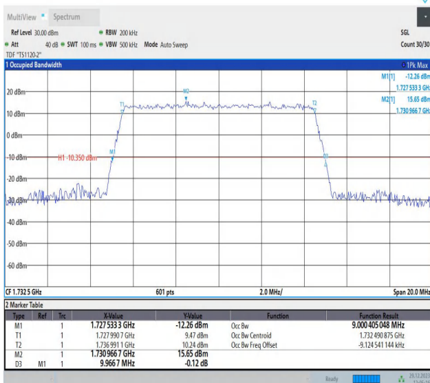
Band4-10MHz-64QAM-20175-50RB#0-PASS
