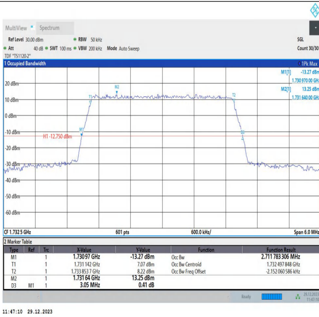
Band4-3MHz-64QAM-20175-15RB#0-PASS
