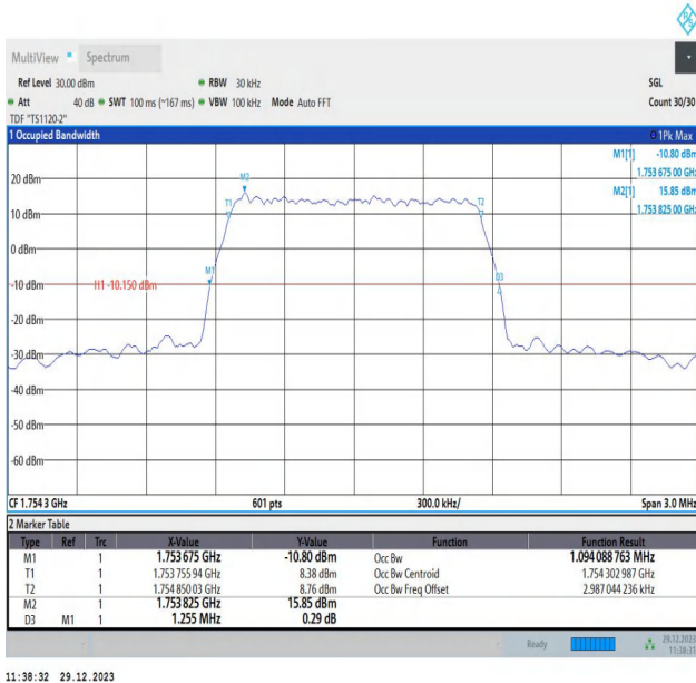
Band4-1.4MHz-64QAM-20393-6RB#0-PASS
