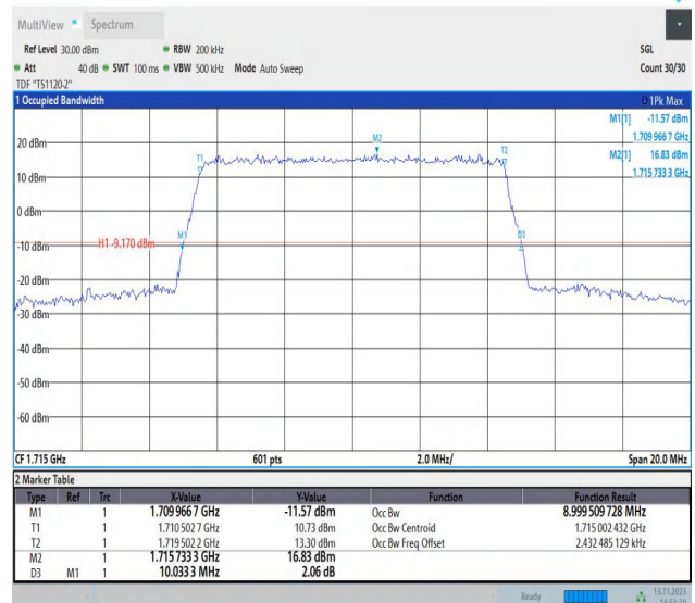
Band4-10MHz-16QAM-20000-50RB#0-PASS
