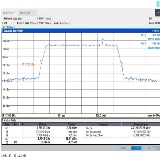
Band4-3MHz-QPSK-20385-15RB#0-PASS
