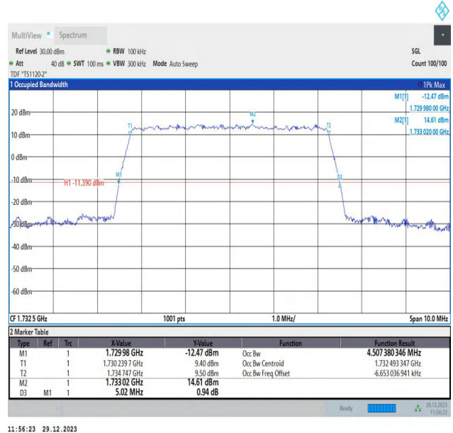
Band4-5MHz-64QAM-20175-25RB#0-PASS
