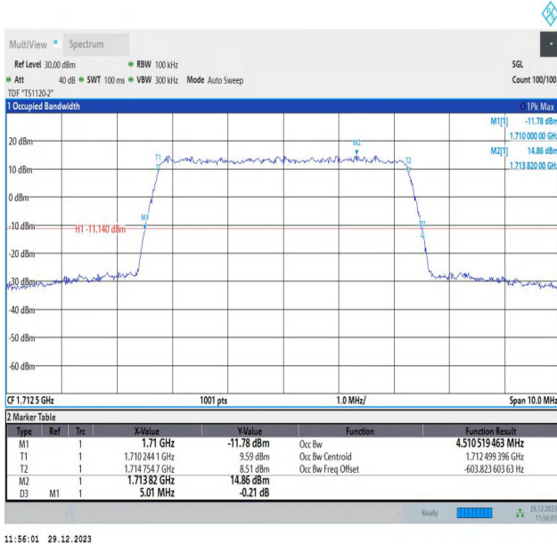
Band4-5MHz-64QAM-19975-25RB#0-PASS
