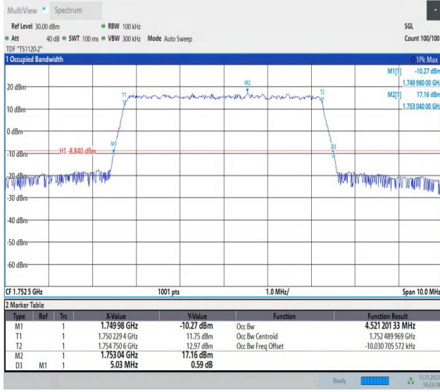
Band4-5MHz-QPSK-20375-25RB#0-PASS
