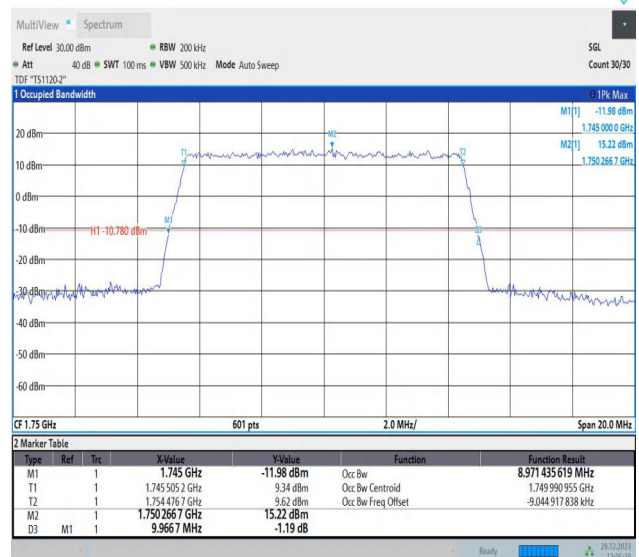
Band4-10MHz-64QAM-20350-50RB#0-PASS
