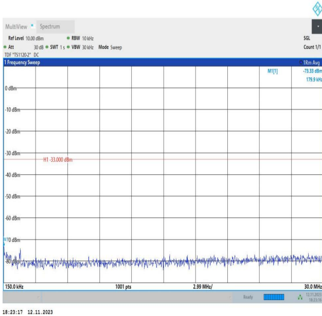
Band2_3MHz_16QAM_19185_1RB#0_0.15~30_0.15~30
