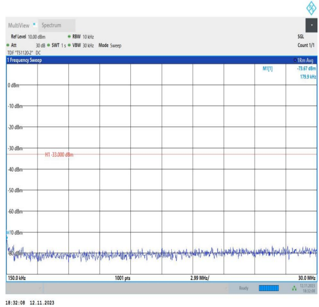
Band2_10MHz_QPSK_19150_1RB#0_0.15~30_0.15~30
