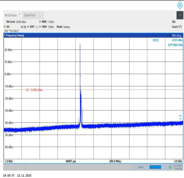
Band2_15MHz_QPSK_18675_1RB#0_1000~3000_1000~3000
