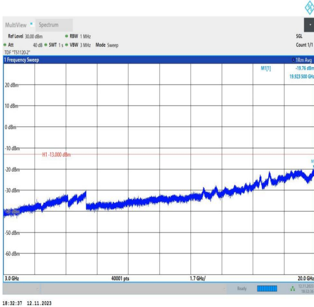
Band2_10MHz_QPSK_19150_1RB#0_3000~20000_3000~20000
