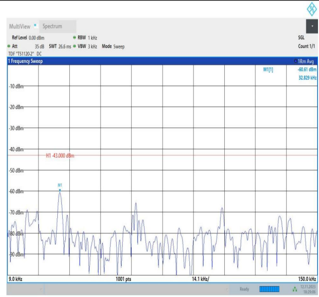
Band2_10MHz_QPSK_18650_1RB#0_0.009~0.15_0.009~0.15
