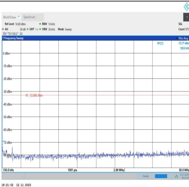
Band2_3MHz_QPSK_18900_1RB#0_0.15~30_0.15~30
