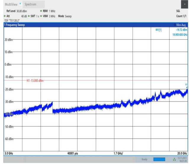
Band2_10MHz_16QAM_18900_1RB#0_3000~20000_3000~20000
