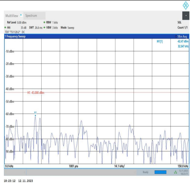
Band2_3MHz_16QAM_19185_1RB#0_0.009~0.15_0.009~0.15
