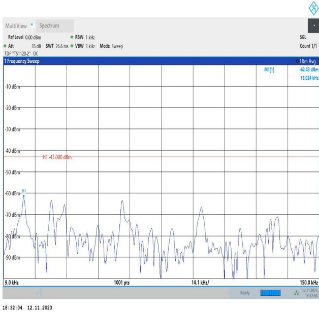
Band2_10MHz_QPSK_19150_1RB#0_0.009~0.15_0.009~0.15
