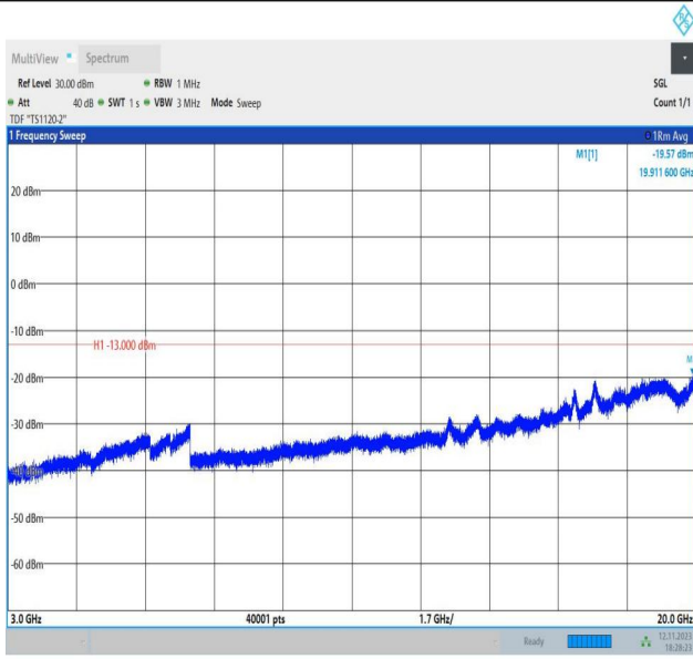
Band2_5MHz_16QAM_19175_1RB#0_3000~20000_3000~20000
