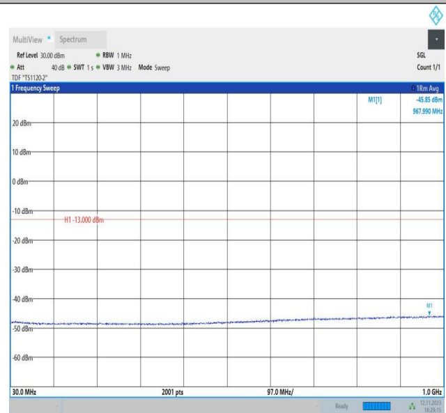
Band2_10MHz_QPSK_18650_1RB#0_30~1000_30~1000
