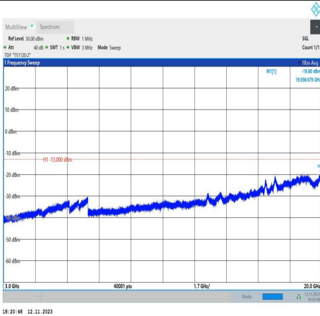
Band2_3MHz_16QAM_18615_1RB#0_3000~20000_3000~20000
