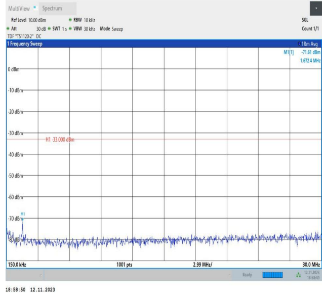
Band2_15MHz_QPSK_18675_1RB#0_0.15~30_0.15~30
