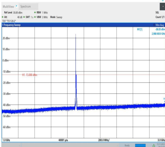
Band2_10MHz_16QAM_19150_1RB#0_1000~3000_1000~30 00
