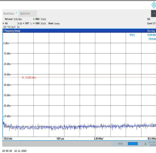
Band2_15MHz_16QAM_18675_1RB#0_0.15~30_0.15~30
