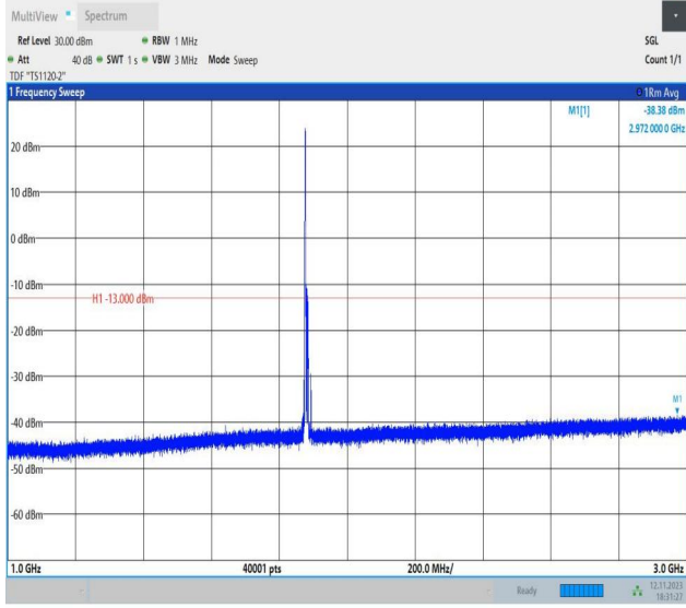
Band2_10MHz_16QAM_18900_1RB#0_1000~3000_1000~3000
