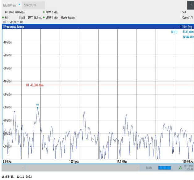
Band2_15MHz_QPSK_18675_1RB#0_0.009~0.15_0.009~0.1
