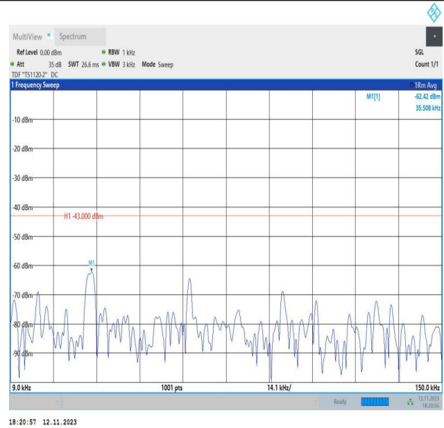
Band2_3MHz_QPSK_18900_1RB#0_0.009~0.15_0.009~0.15
