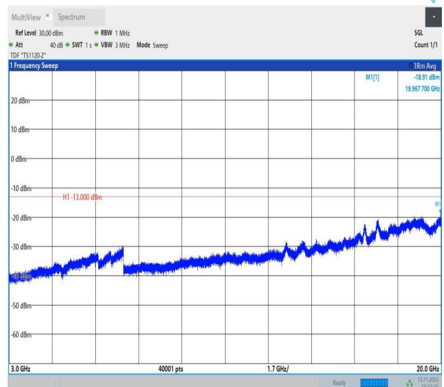
Band2_10MHz_16QAM_19150_1RB#0_3000~20000_3000~20 000
