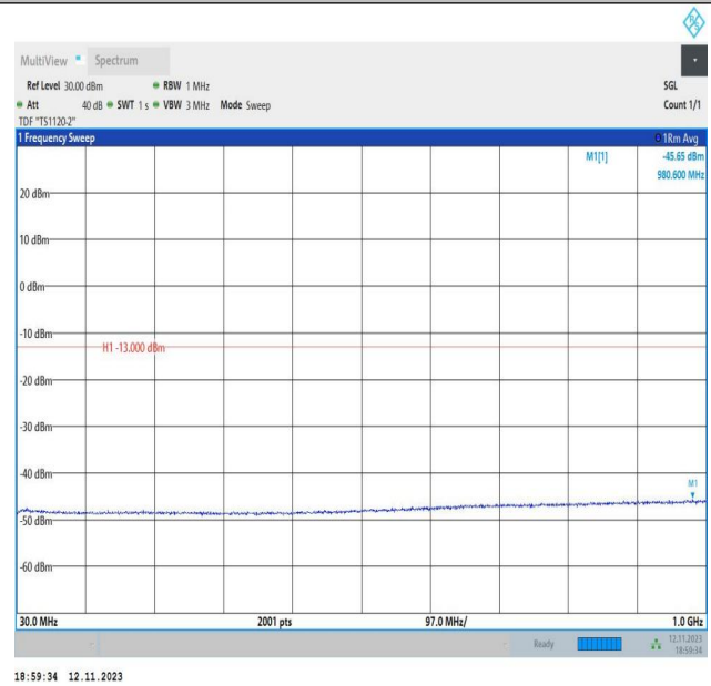
Band2_15MHz_16QAM_18675_1RB#0_30~1000_30~1000
