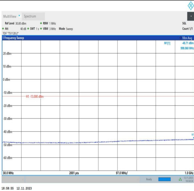
Band2_15MHz_QPSK_18675_1RB#0_30~1000_30~1000
