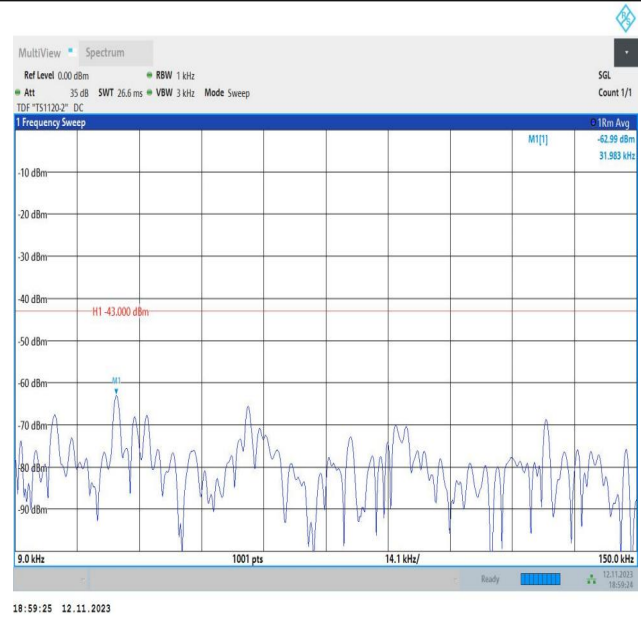
Band2_15MHz_16QAM_18675_1RB#0_0.009~0.15_0.009~0.15
