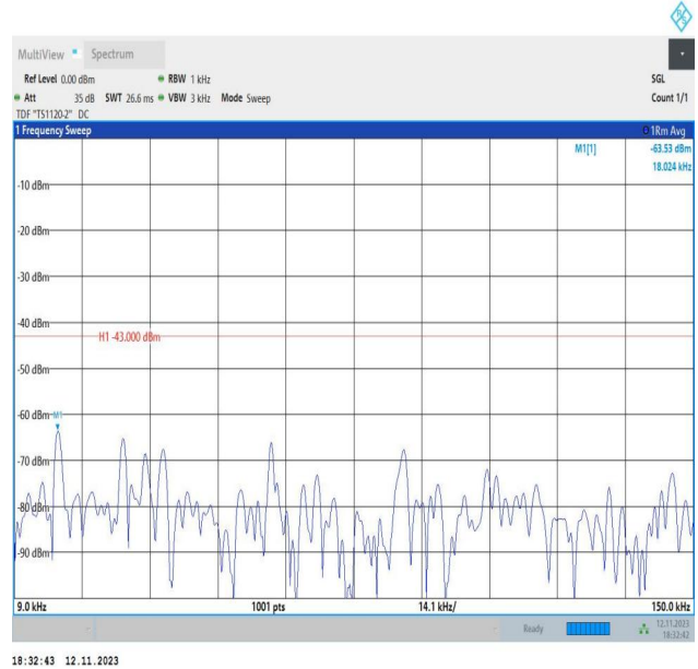
Band2_10MHz_16QAM_19150_1RB#0_0.009~0.15_0.009~0.1
