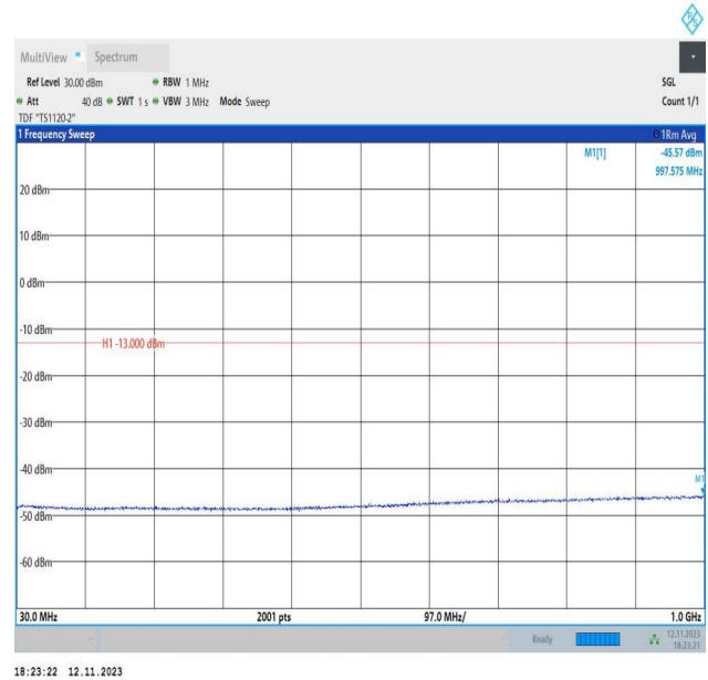
Band2_3MHz_16QAM_19185_1RB#0_30~1000_30~1000
