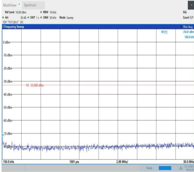
Band2_10MHz_16QAM_19150_1RB#0_0.15~30_0.15~30
