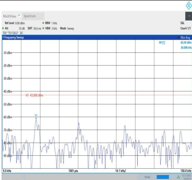
Band2_5MHz_QPSK_18625_1RB#0_0.009~0.15_0.009~0.15
