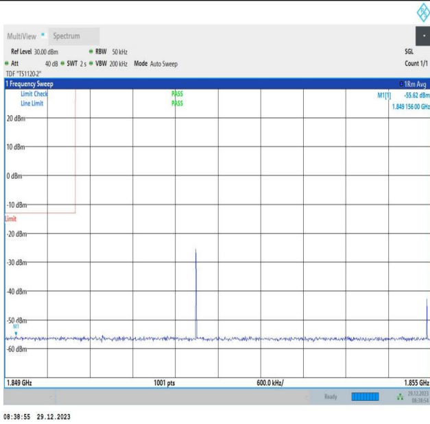
Band2_5MHz_64QAM_18625_1RB#0
