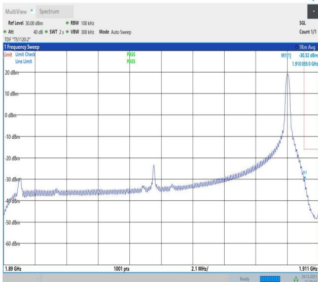
Band2_20MHz_64QAM_19100_1RB#99
