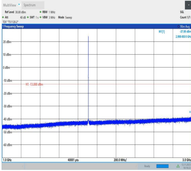
Band2_1.4MHz_16QAM_19193_1RB#0_1000~3000_1000~3000
