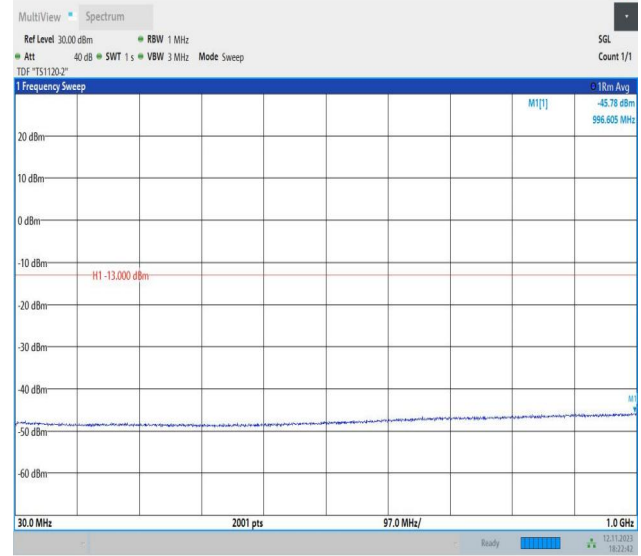
Band2_3MHz_QPSK_19185_1RB#0_30~1000_30~1000
