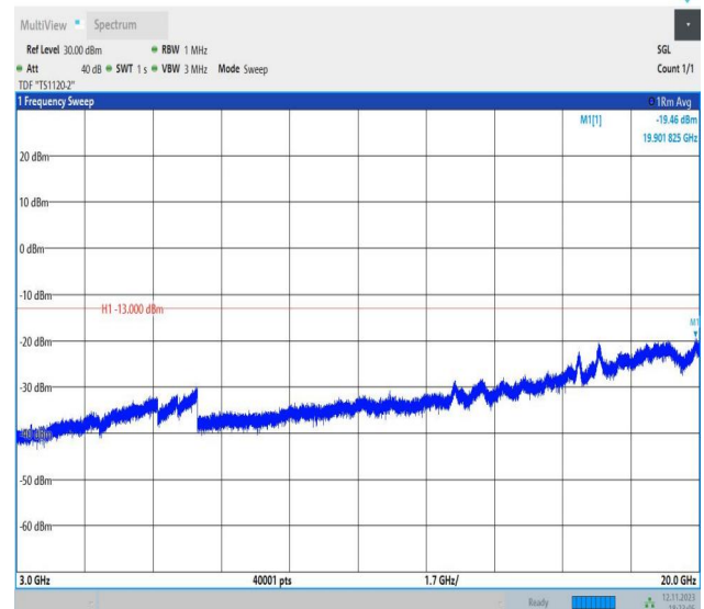
Band2_3MHz_QPSK_19185_1RB#0_3000~20000_3000~2000
