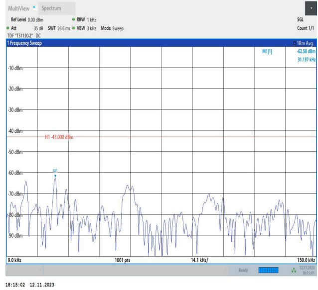
Band2_1.4MHz_16QAM_18607_1RB#0_0.009~0.15_0.009~0.15 15
