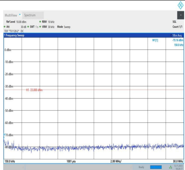
Band2_5MHz_QPSK_18625_1RB#0_0.15~30_0.15~30
