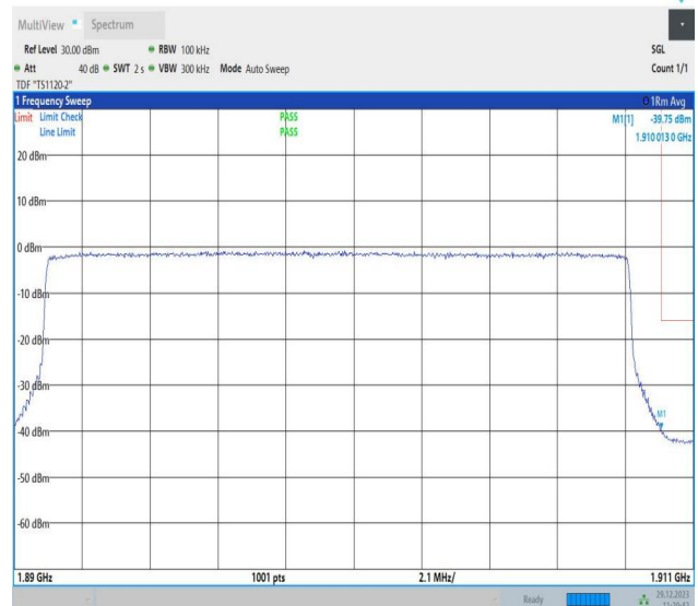
Band2_20MHz_64QAM_19100_100RB#0
