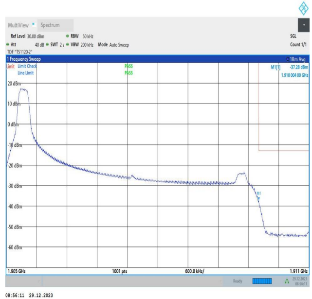
Band2_5MHz_64QAM_19175_1RB#0
