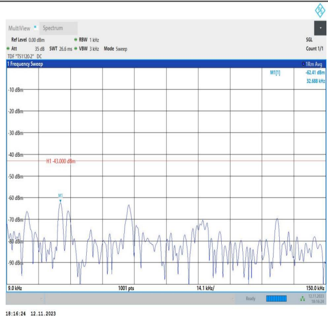
Band2_1.4MHz_16QAM_18900_1RB#0_0.009~0.15_0.009~0.15 15
