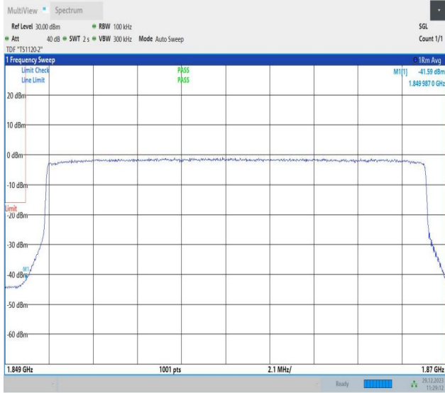
Band2_20MHz_64QAM_18700_100RB#0
