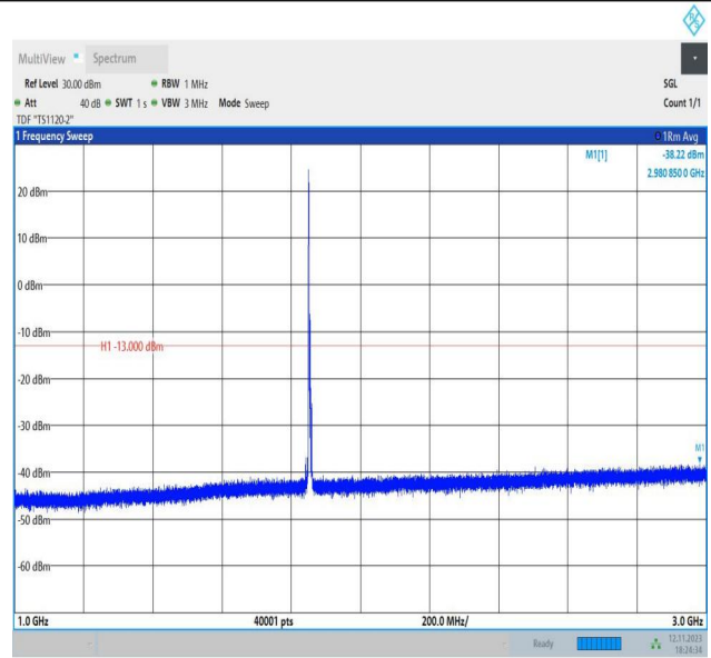
Band2_5MHz_QPSK_18625_1RB#0_1000~3000_1000~3000
