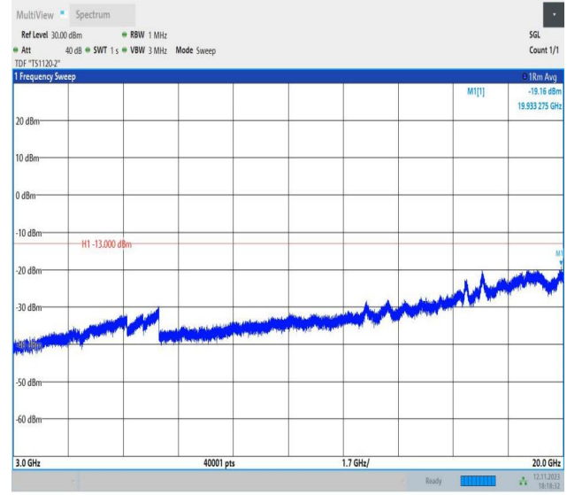
Band2_1.4MHz_16QAM_19193_1RB#0_3000~20000_3000~20000
