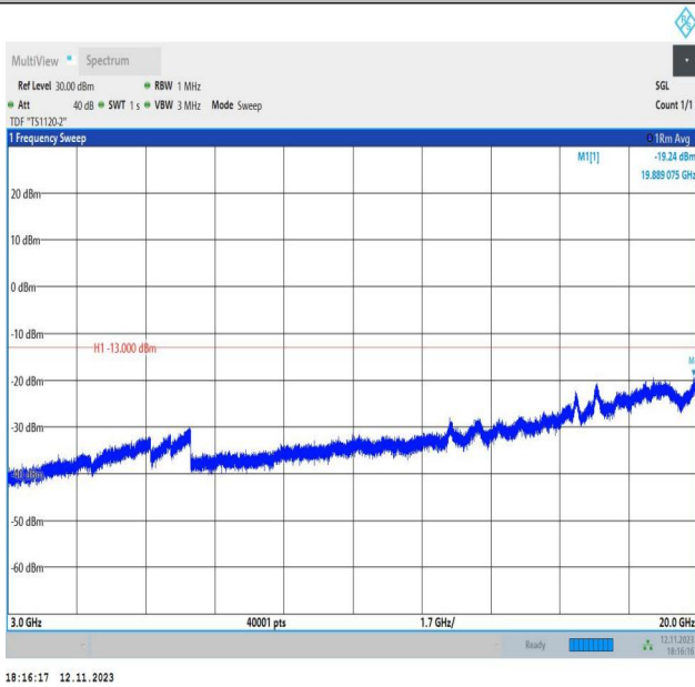
Band2_1.4MHz_QPSK_18900_1RB#0_3000~20000_3000~20000 0000
