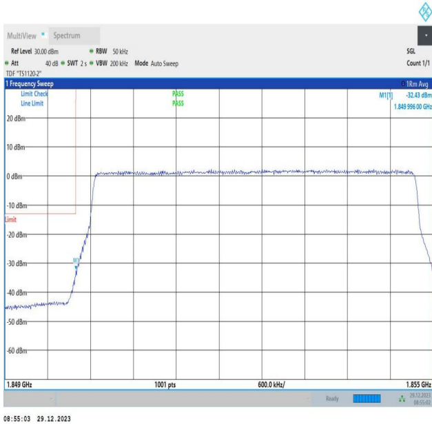
Band2_5MHz_64QAM_18625_25RB#0
