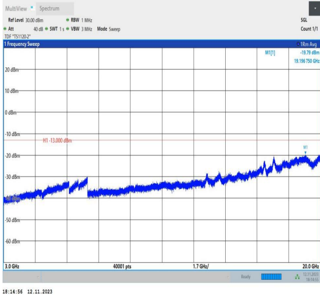
Band2_1.4MHz_QPSK_18607_1RB#0_3000~20000_3000~20000 0000
