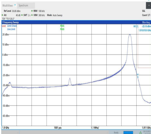
Band2_10MHz_64QAM_19150_1RB#49
