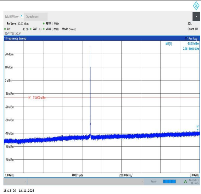
Band2_1.4MHz_QPSK_18900_1RB#0_1000~3000_1000~300 0
