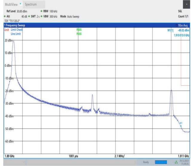
Band2_20MHz_64QAM_19100_1RB#0
