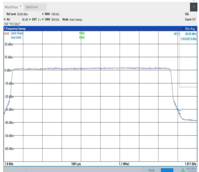
Band2_10MHz_64QAM_19150_50RB#0
