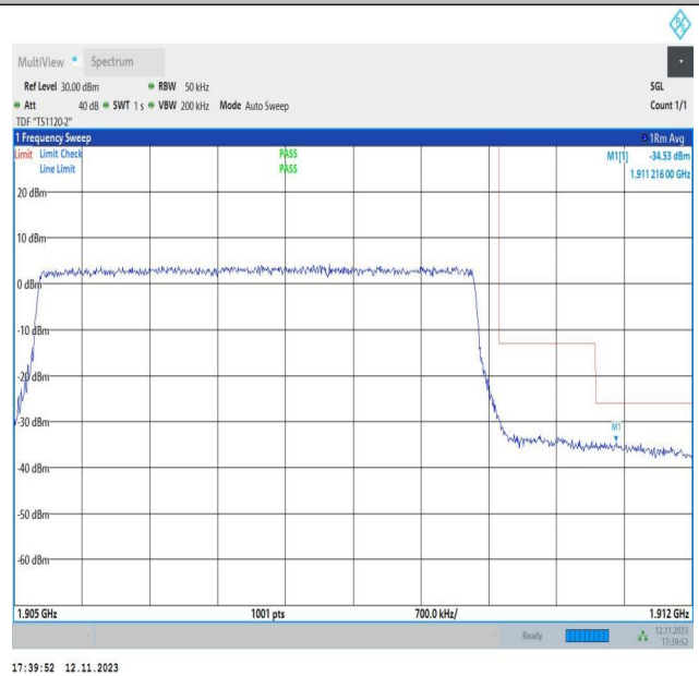
Band2_5MHz_16QAM_19175_25RB#0
