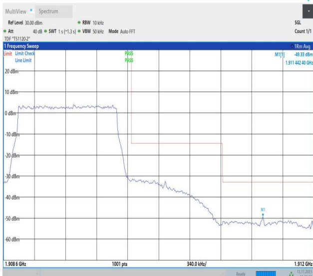
Band2_1.4MHz_QPSK_19193_6RB#0
