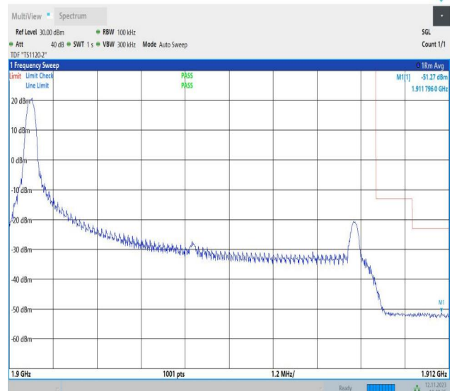
Band2_10MHz_16QAM_19150_1RB#0
