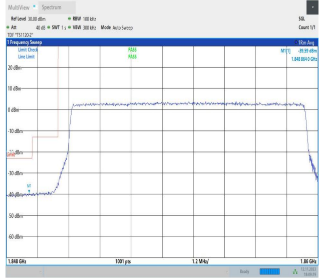
Band2_10MHz_16QAM_18650_50RB#0
