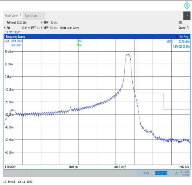
Band2_5MHz_16QAM_19175_1RB#24
