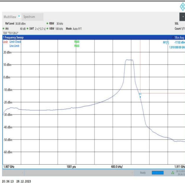
Band2_3MHz_64QAM_19185_1RB#14
