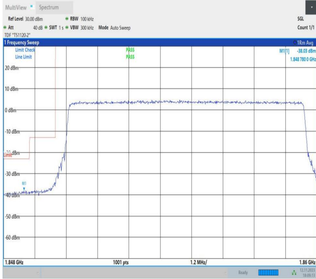
Band2_10MHz_QPSK_18650_50RB#0
