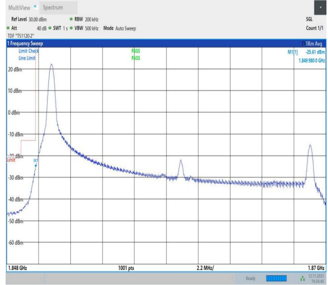
Band2_20MHz_16QAM_18700_1RB#0
