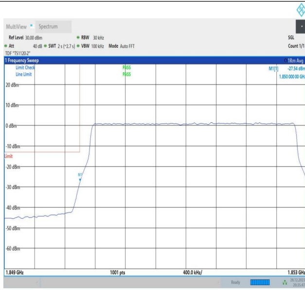
Band2_3MHz_64QAM_18615_15RB#0
