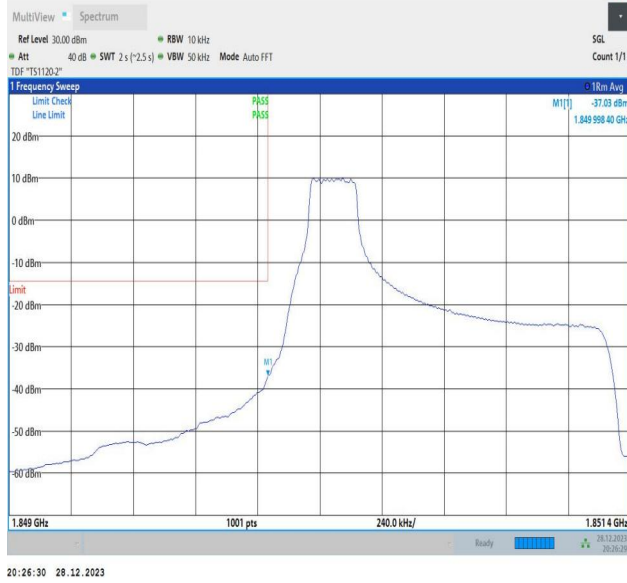
Band2_1.4MHz_64QAM_18607_1RB#0
