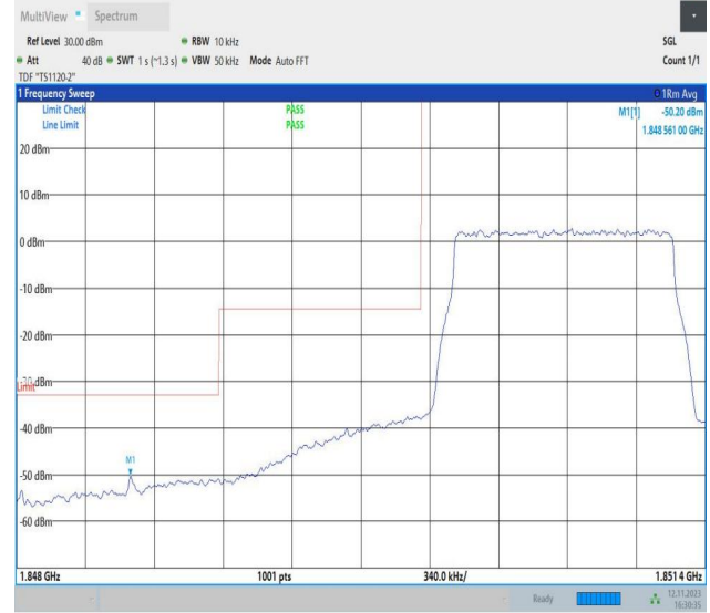
Band2_1.4MHz_16QAM_18607_6RB#0
