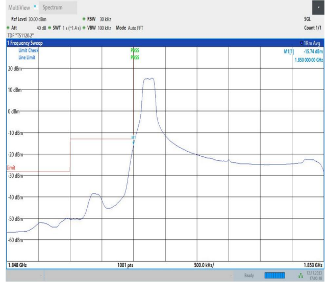
Band2_3MHz_16QAM_18615_1RB#0
