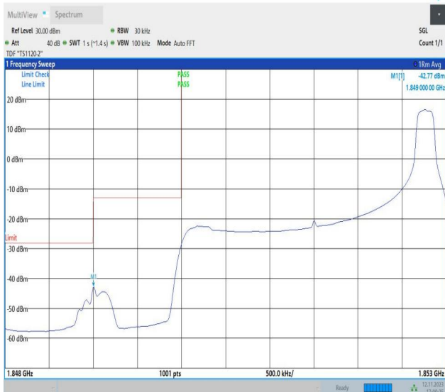
Band2_3MHz_QPSK_18615_1RB#14
