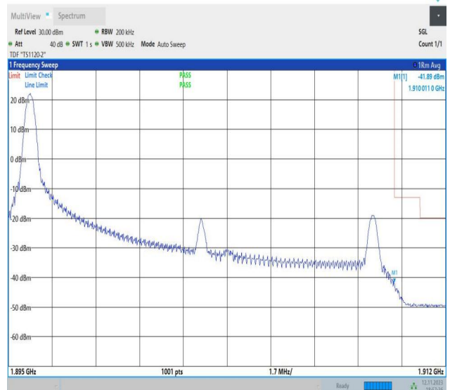
Band2_15MHz_16QAM_19125_1RB#0
