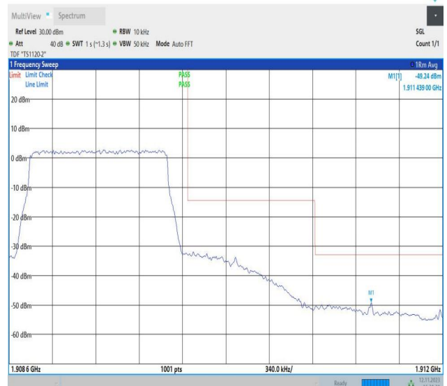
Band2_1.4MHz_16QAM_19193_6RB#0
