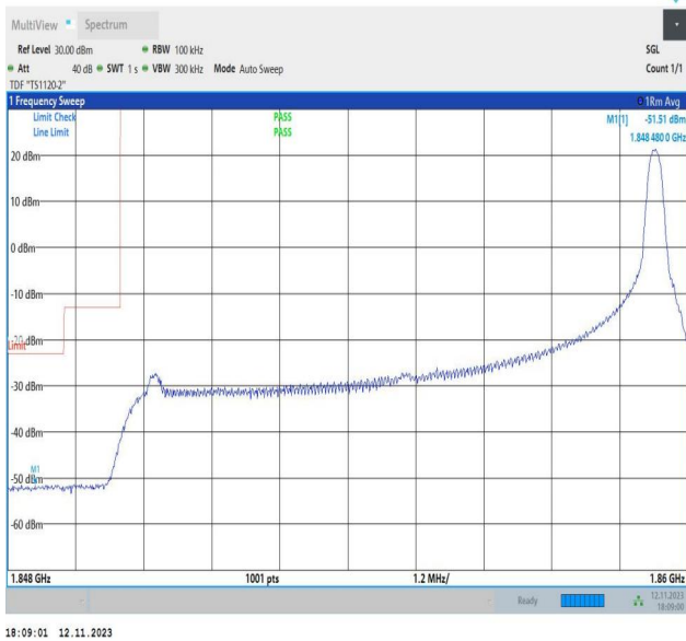
Band2_10MHz_QPSK_18650_1RB#49
