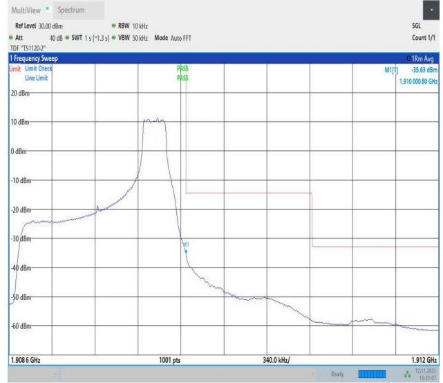
Band2_1.4MHz_16QAM_19193_1RB#5
