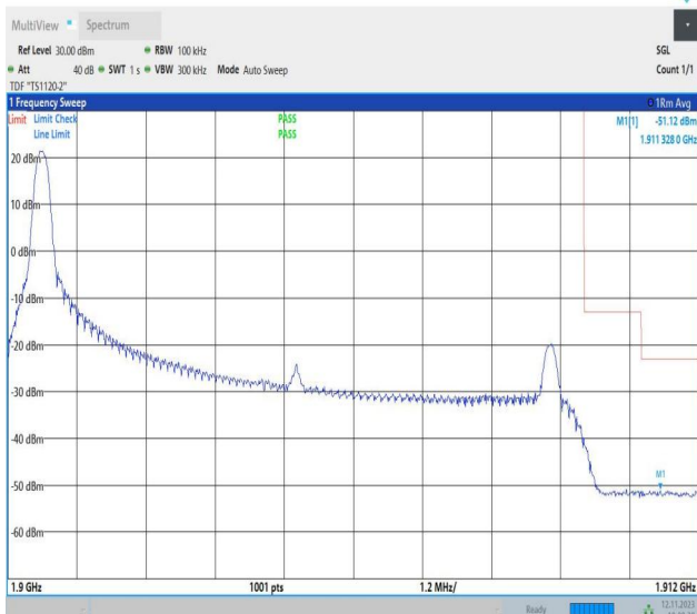
Band2_10MHz_QPSK_19150_1RB#0
