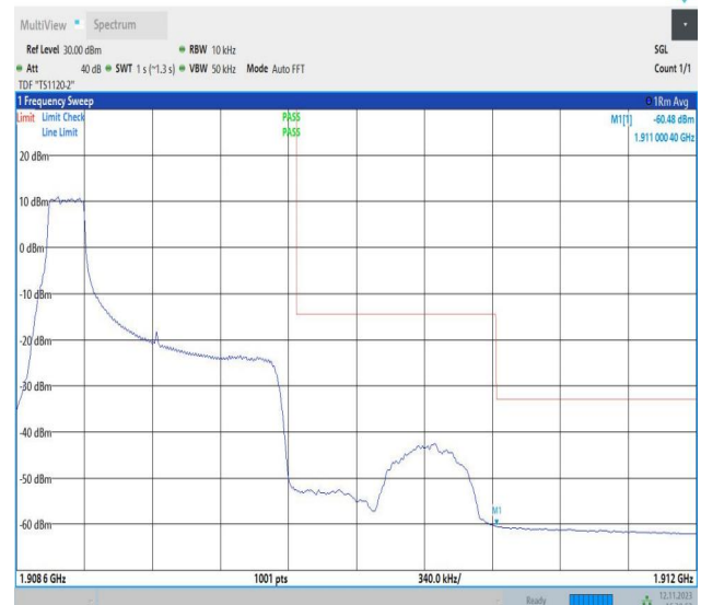
Band2_1.4MHz_16QAM_19193_1RB#0
