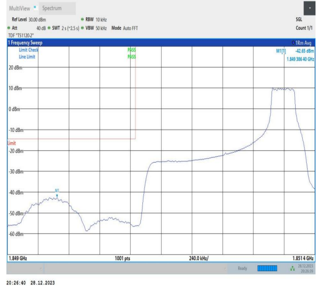
Band2_1.4MHz_64QAM_18607_1RB#5
