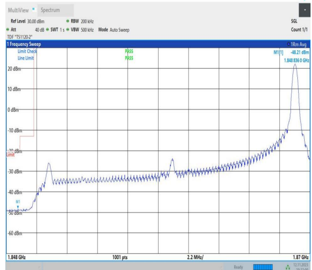
Band2_20MHz_16QAM_18700_1RB#99
