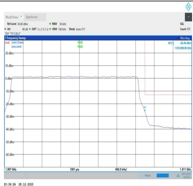
Band2_3MHz_64QAM_19185_15RB#0
