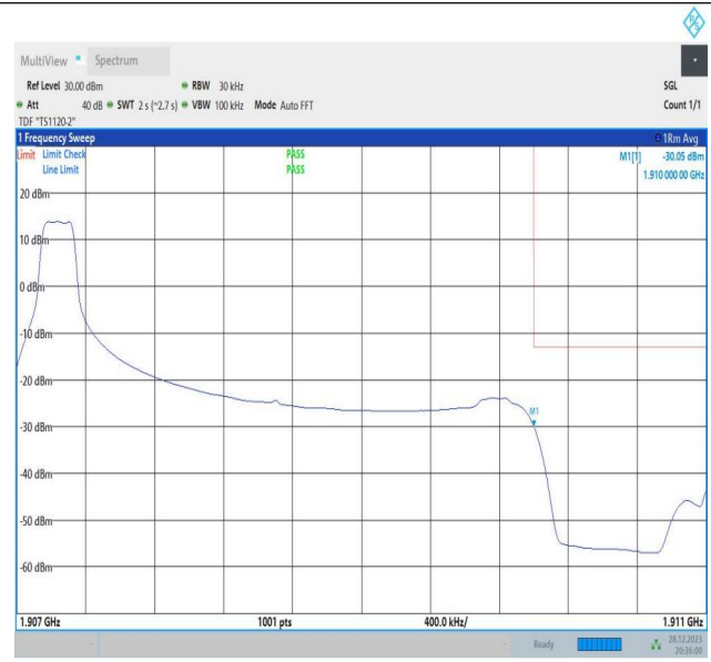
Band2_3MHz_64QAM_19185_1RB#0
