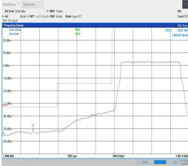
Band2_1.4MHz_QPSK_18607_6RB#0
