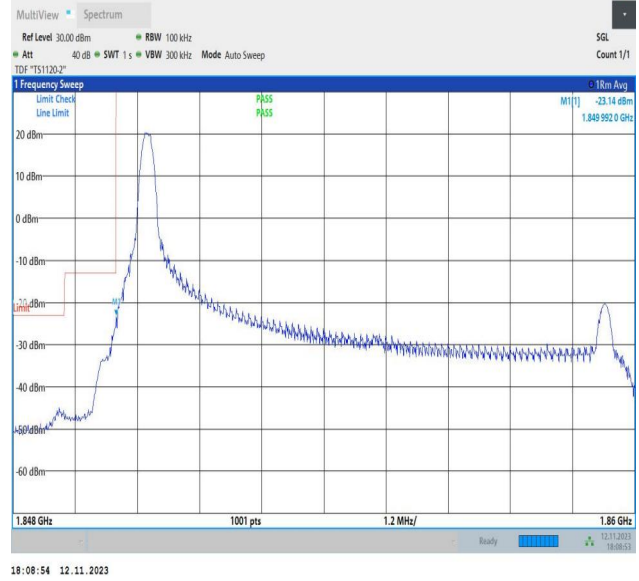
Band2_10MHz_16QAM_18650_1RB#0
