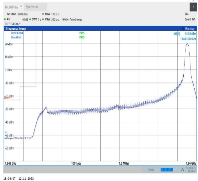
Band2_10MHz_16QAM_18650_1RB#49
