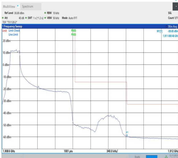
Band2_1.4MHz_QPSK_19193_1RB#0
