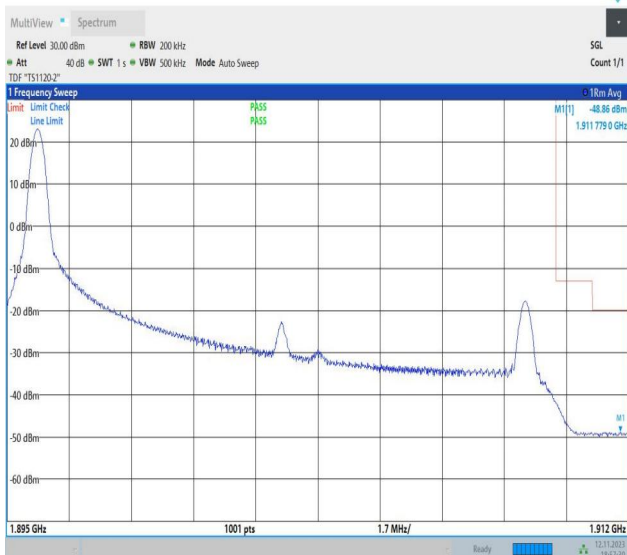
Band2_15MHz_QPSK_19125_1RB#0
