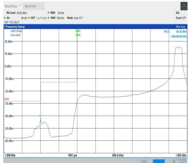
Band2_3MHz_16QAM_18615_1RB#14
