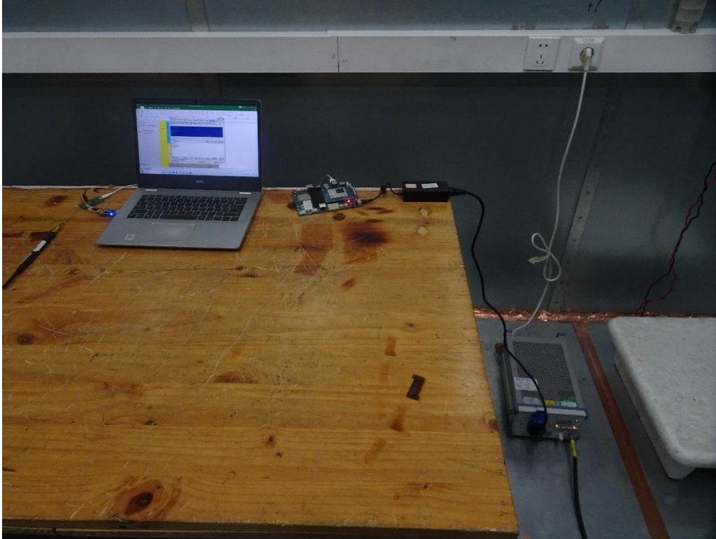
Picture 2 Conducted Emission Transmitter Unwanted Emissions Test Setup
