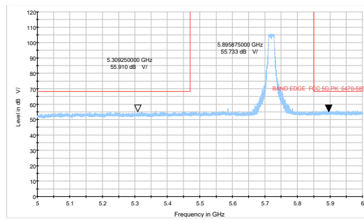
802.11ax HE20 -Channel 144: Peak + Average
