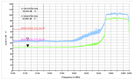
802.11ax HE20 -Channel 52: Peak + Average
