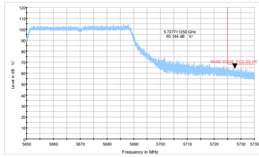
802.11ax HE40-Channel 134: Peak
