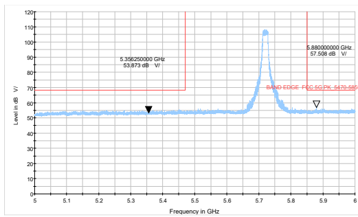
802.11n HT40-Channel 142: Peak
