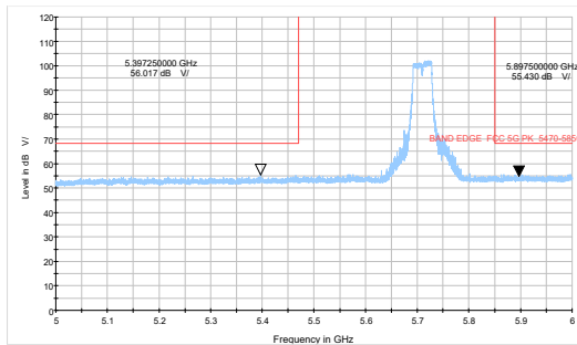
802.11ax HE40-Channel 142: Peak + Average
