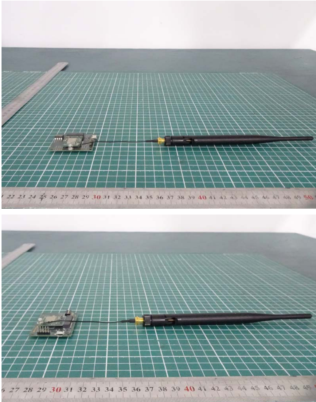
b: Auxiliary Antenna
