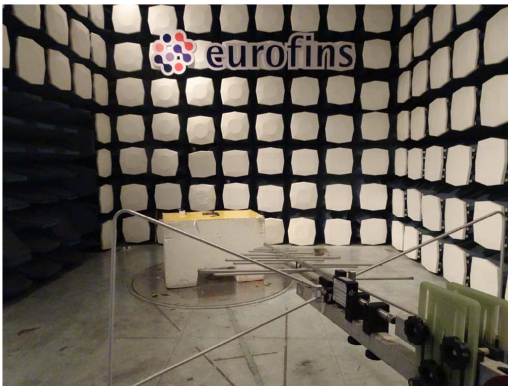
30MHz-1GHz
