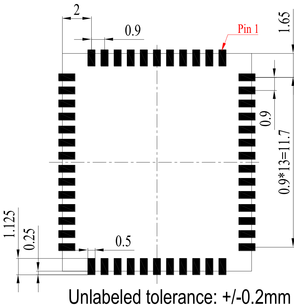
Figure 23: Recommended Footprint
