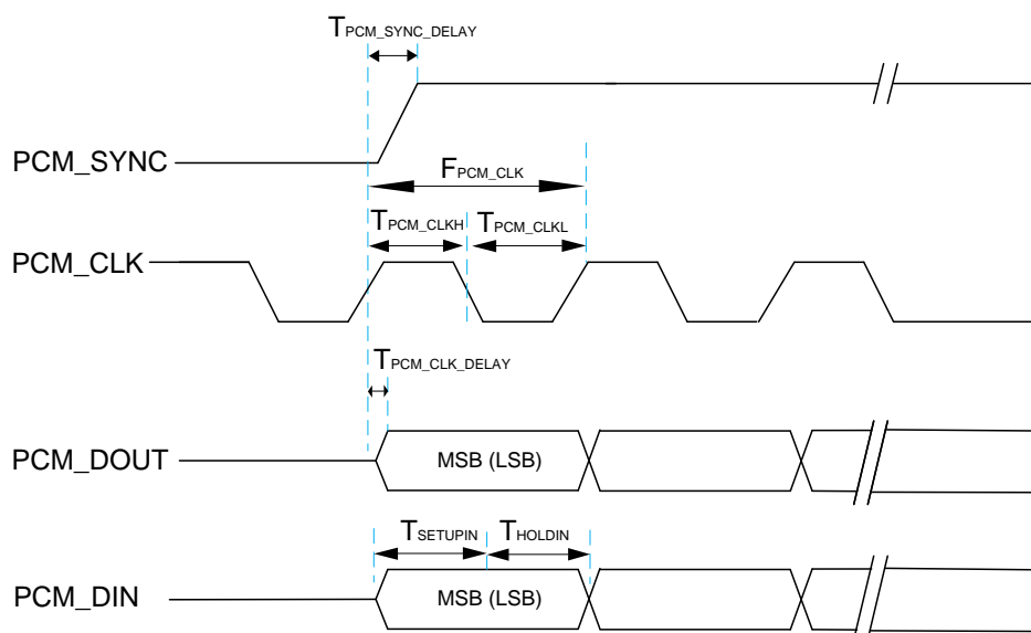
Figure 10: PCM Interface (Long Frame Sync)
