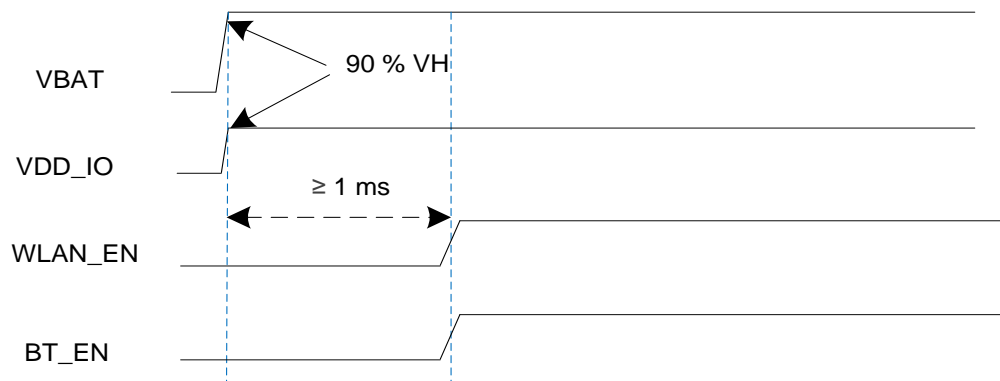
Figure 3: Power-up Timing
