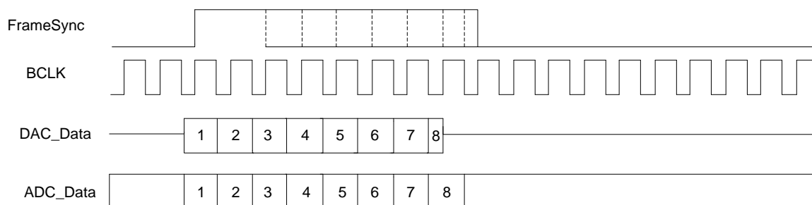
Figure 9: Short FrameSync
