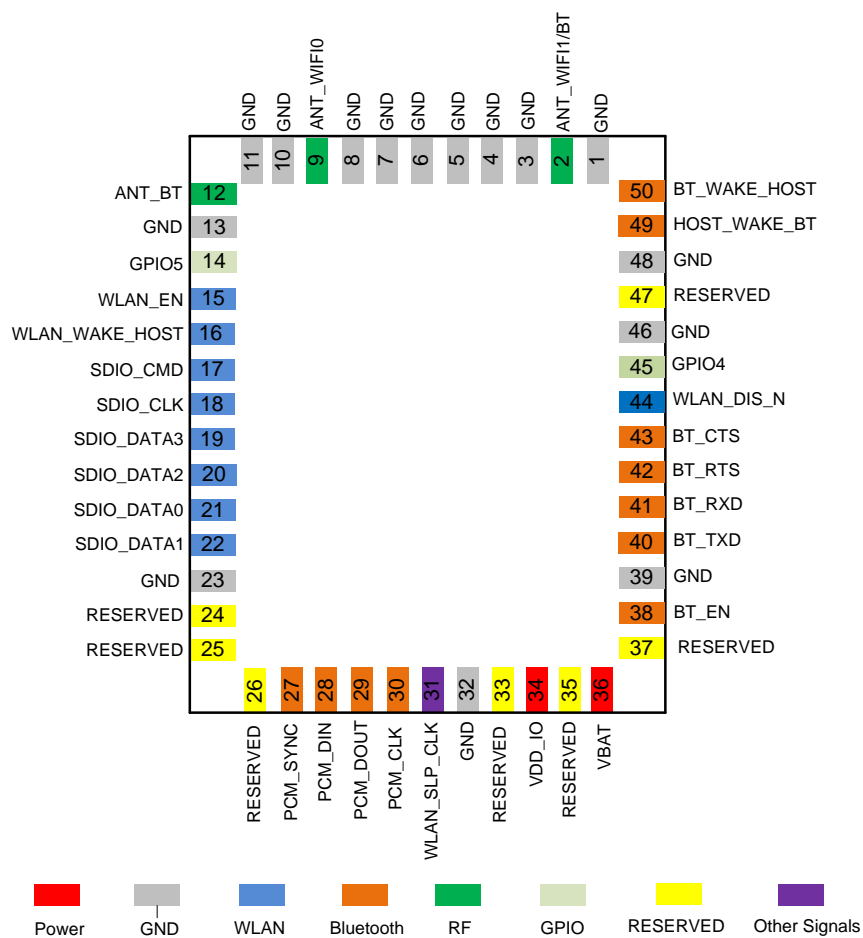
Figure 1: Pin Assignment (Top View)
