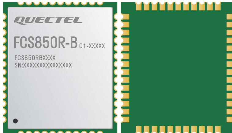
Figure 21: Top and Bottom Views (FCS850R-B)
