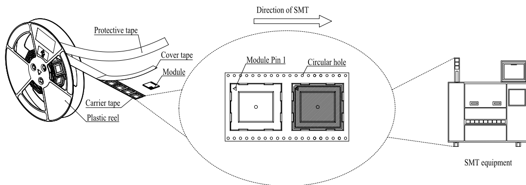
Figure 25: Mounting Direction
