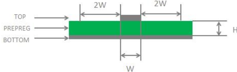
Figure 9: Microstrip Design on a 2-layer PCB
