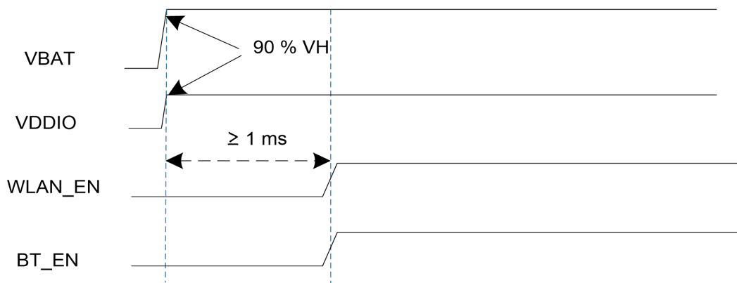
Figure 3: Power-up Timing
