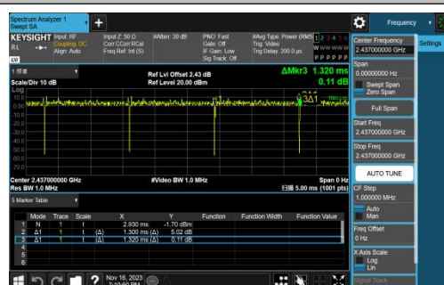
NTNV-11N20SISO-Ant1-2437
