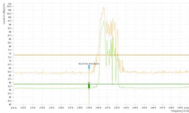
Wi-Fi 2.4_11AX20_2412_52RU_edge
