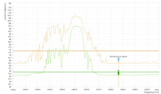
Wi-Fi 2.4_11AX20_2462_52RU_edge
