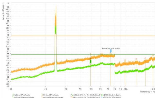
802.11b_2462_High
