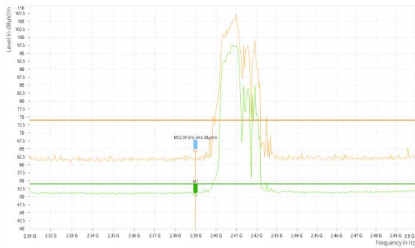
Wi-Fi 2.4_11AX20_2412_106RU_edge
