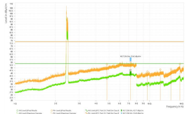
802.11g_2412_High
