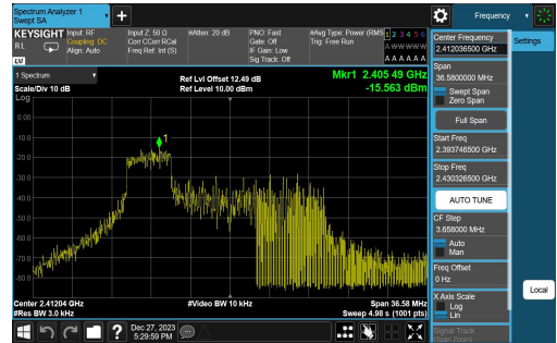
11AX20SISO-Ant1-2412-52Tone-RU40-PASS
