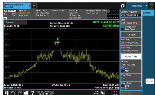
11AX20SISO-Ant1-2437-26Tone-RU4-PASS
