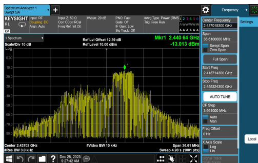
11AX20SISO-Ant1-2437-106Tone-RU53-PASS
