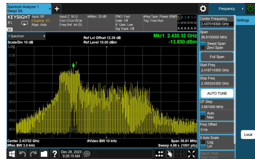
11AX20SISO-Ant1-2437-52Tone-RU40-PASS
