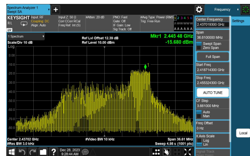
11AX20SISO-Ant1-2437-106Tone-RU54-PASS
