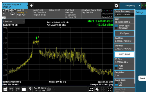
11AX20SISO-Ant1-2462-26Tone-RU0-PASS
