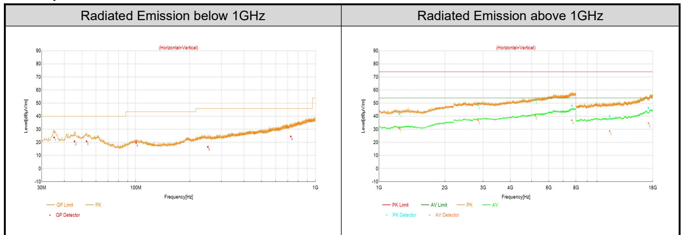
Radiated Emission Below 1GHz
