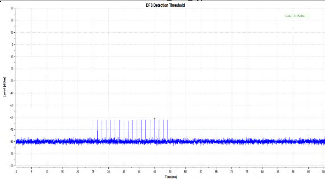
11ac160MIMO_5570_Type0
