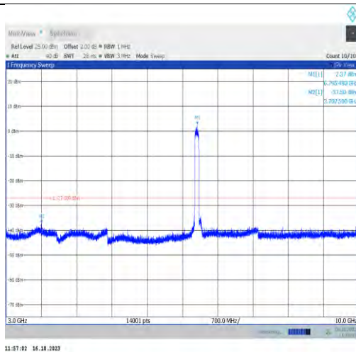
11ax80MIMO-Ant1-6785-3000~10000-PASS
