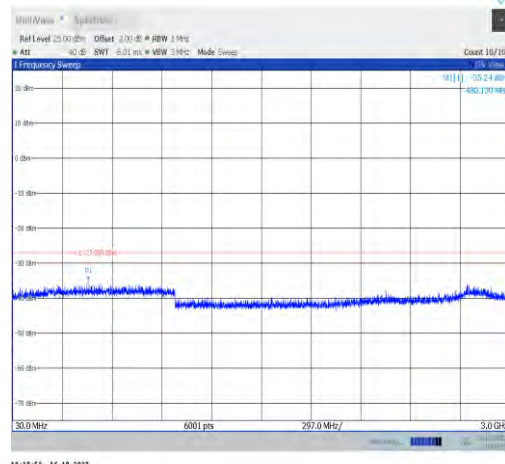
11ax80MIMO-Ant1-5985-30~3000-PASS
