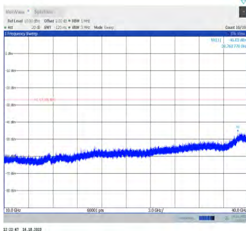
11ax80MIMO-Ant0-6865-10000~40000-PASS
