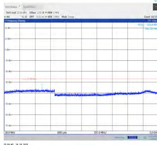
11ax80MIMO-Ant1-7025-30~3000-PASS
