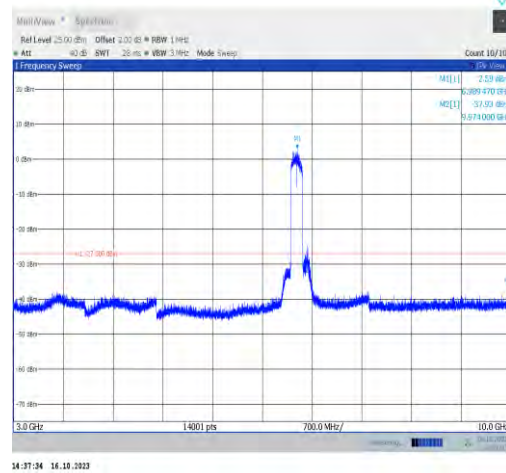
11ax160MIMO-Ant0-6985-3000~10000-PASS
