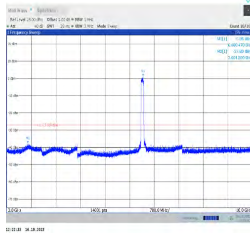
11ax80MIMO-Ant0-6865-3000~10000-PASS
