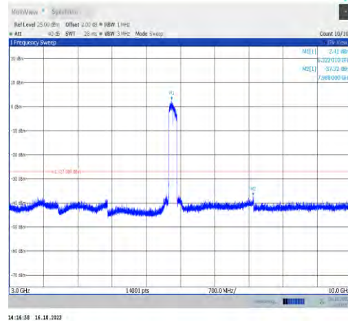
11ax160MIMO-Ant0-6345-3000~10000-PASS
