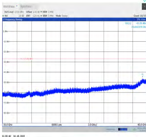
11ax80MIMO-Ant0-6785-10000~40000-PASS
