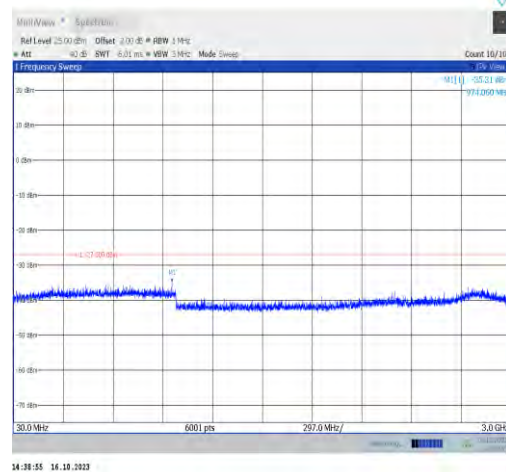
11ax160MIMO-Ant1-6985-30~3000-PASS
