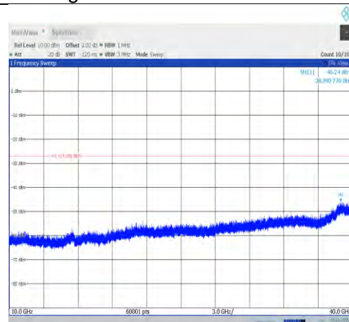
11ax80MIMO-Ant1-5985-10000~40000-PASS
