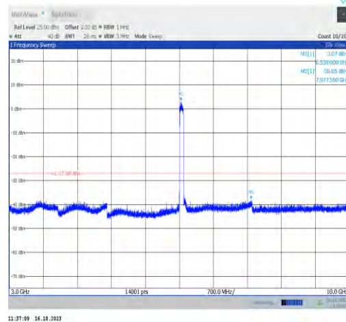
11ax80MIMO-Ant0-6545-3000~10000-PASS
