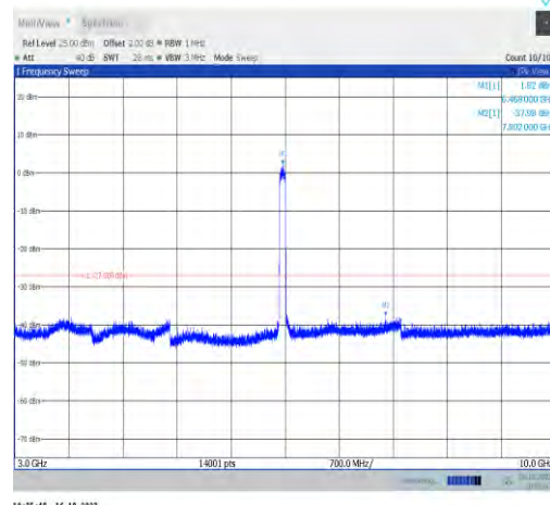
11ax80MIMO-Ant0-6465-3000~10000-PASS
