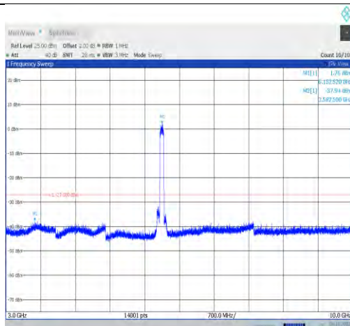
11ax80MIMO-Ant1-6145-3000~10000-PASS
