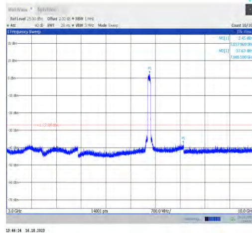
11ax80MIMO-Ant0-7025-3000~10000-PASS
