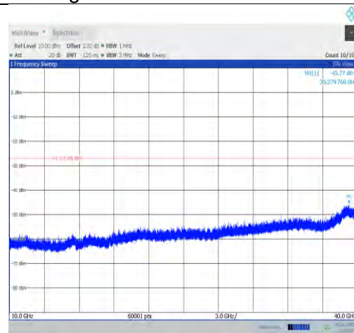
11ax160MIMO-Ant1-6345-10000~40000-PASS
