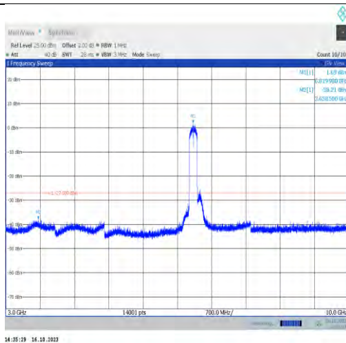
11ax160MIMO-Ant1-6825-3000~10000-PASS
