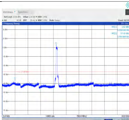
11ax80MIMO-Ant1-5985-3000~10000-PASS
