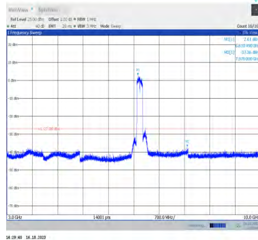
11ax160MIMO-Ant0-6665-3000~10000-PASS
