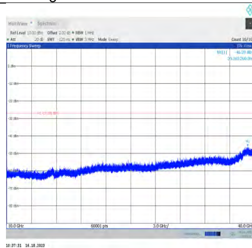
11ax80MIMO-Ant1-6465-10000~40000-PASS
