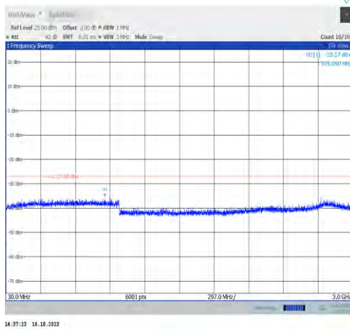
11ax160MIMO-Ant0-6985-30~3000-PASS
