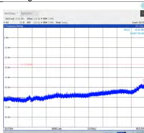
11ax40MIMO-Ant1-7085-10000~40000-PASS
