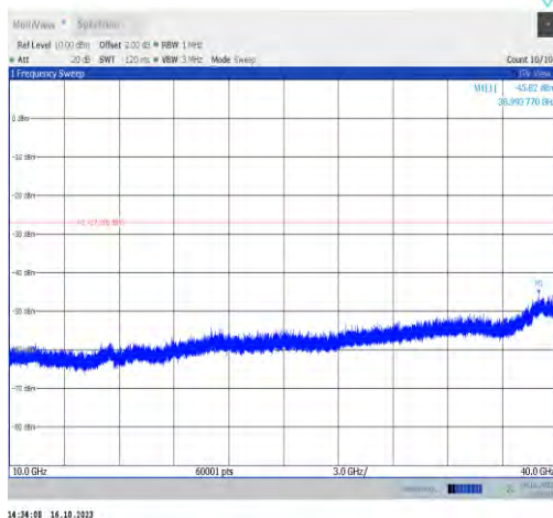
11ax160MIMO-Ant0-6825-10000~40000-PASS
