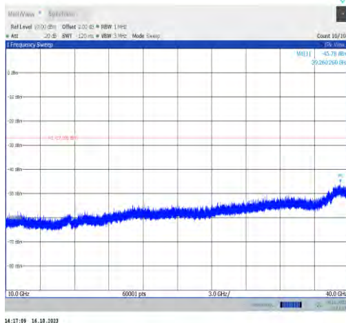
11ax160MIMO-Ant0-6345-10000~40000-PASS
