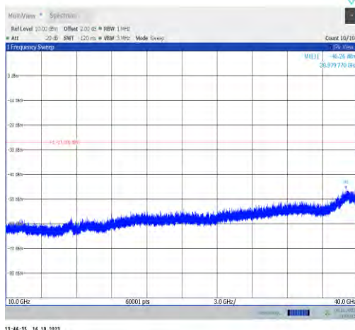
11ax80MIMO-Ant0-7025-10000~40000-PASS
