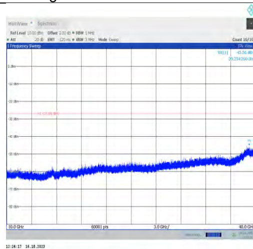
11ax80MIMO-Ant1-6865-10000~40000-PASS
