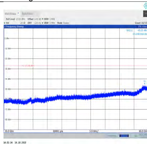
11ax160MIMO-Ant1-6665-10000~40000-PASS
