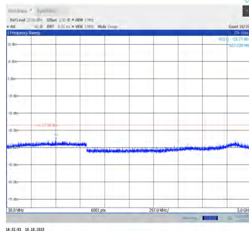
11ax160MIMO-Ant1-6665-30~3000-PASS
