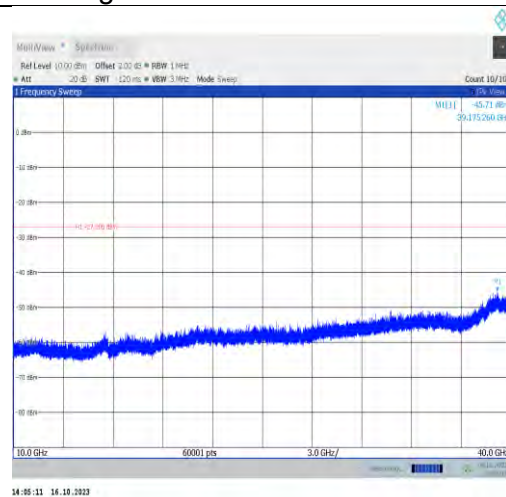
11ax160MIMO-Ant1-6025-10000~40000-PASS
