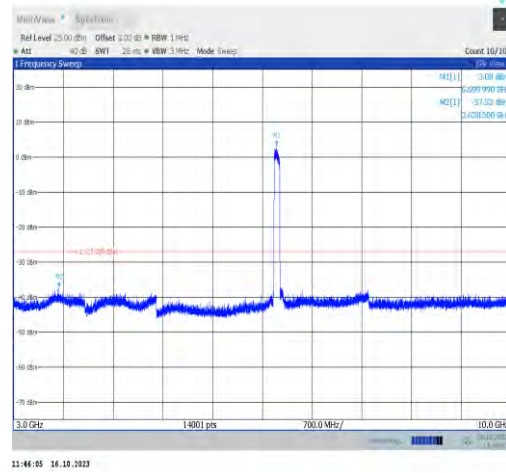
11ax80MIMO-Ant0-6705-3000~10000-PASS
