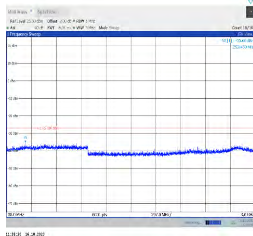
11ax80MIMO-Ant1-6545-30~3000-PASS
