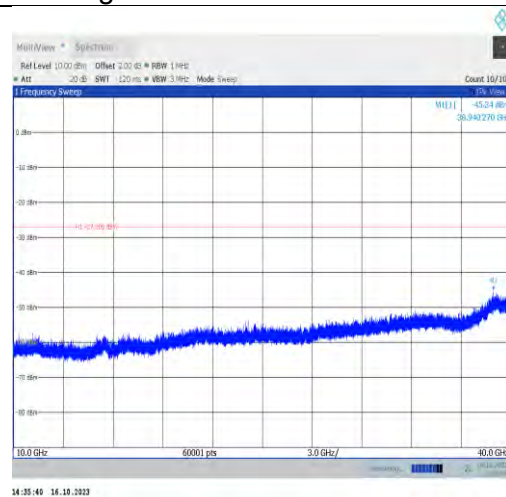
11ax160MIMO-Ant1-6825-10000~40000-PASS
