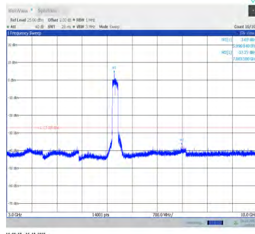
11ax160MIMO-Ant0-6025-3000~10000-PASS
