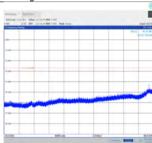
11ax80MIMO-Ant1-6625-10000~40000-PASS
