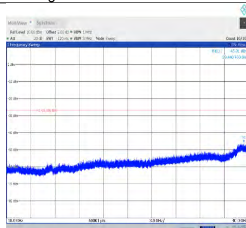
11ax80MIMO-Ant1-6385-10000~40000-PASS
