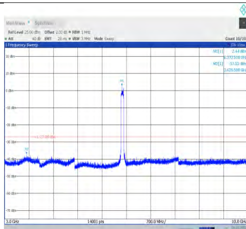
11ax80MIMO-Ant1-6385-3000~10000-PASS
