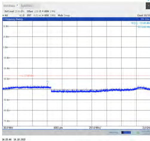
11ax160MIMO-Ant0-6825-30~3000-PASS
