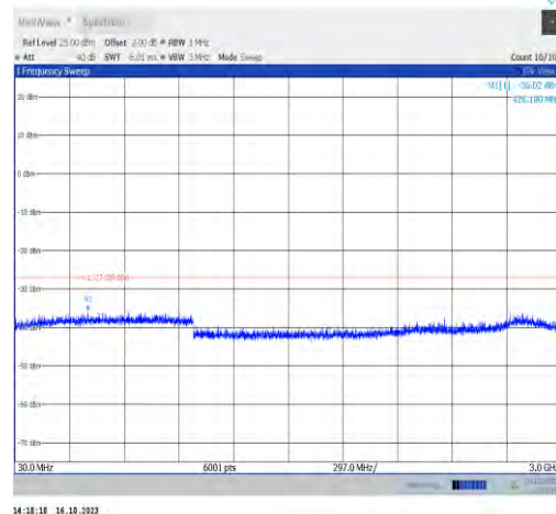
11ax160MIMO-Ant1-6345-30~3000-PASS
