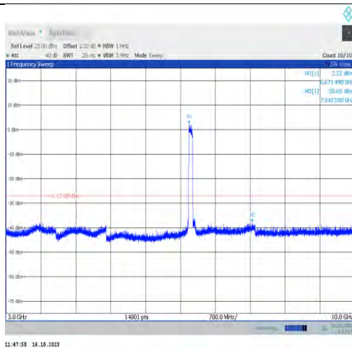
11ax80MIMO-Ant1-6705-3000~10000-PASS
