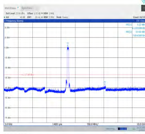
11ax80MIMO-Ant0-6145-3000~10000-PASS
