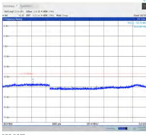
11ax160MIMO-Ant0-6025-30~3000-PASS
