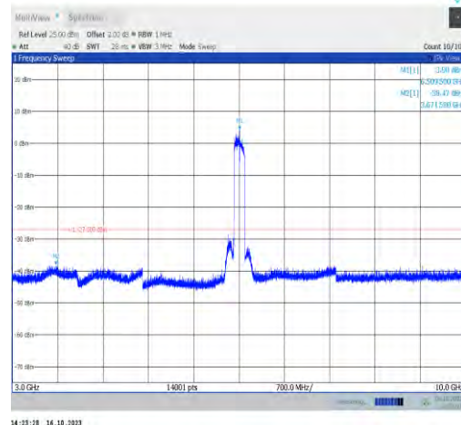
11ax160MIMO-Ant0-6505-3000~10000-PASS
