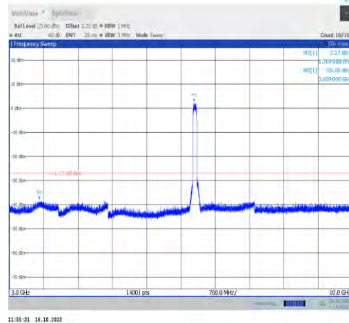
11ax80MIMO-Ant0-6785-3000~10000-PASS
