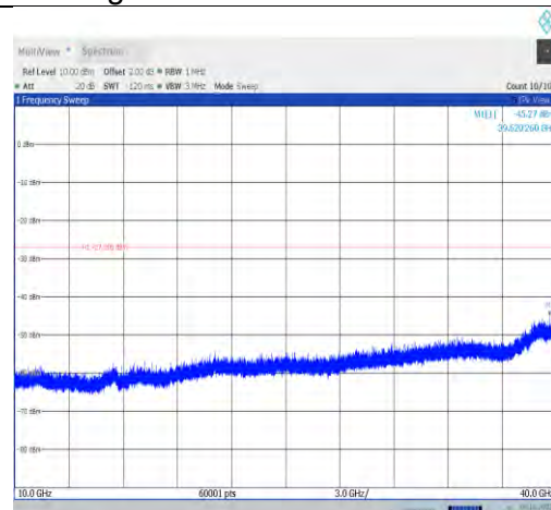
11ax80MIMO-Ant1-7025-10000~40000-PASS
