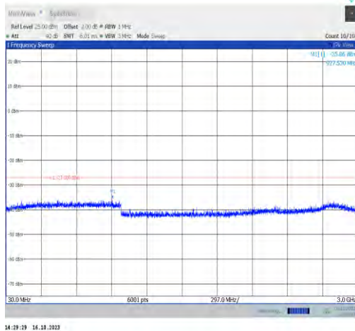
11ax160MIMO-Ant0-6665-30~3000-PASS
