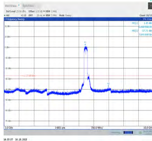
11ax160MIMO-Ant0-6825-3000~10000-PASS
