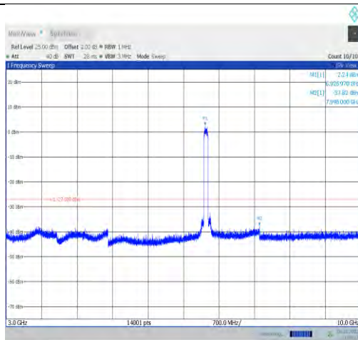
11ax80MIMO-Ant1-6945-3000~10000-PASS
