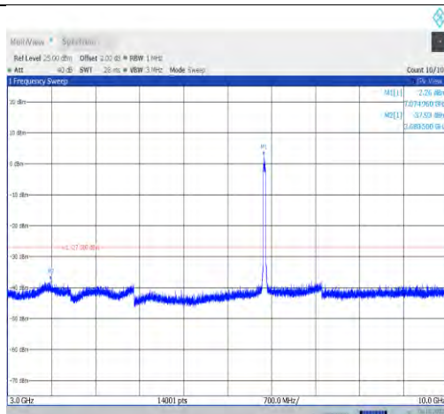
11ax40MIMO-Ant1-7085-3000~10000-PASS
