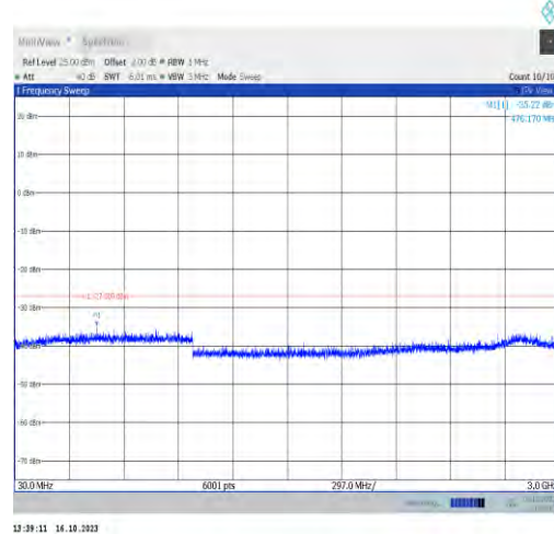
11ax80MIMO-Ant1-6945-30~3000-PASS
