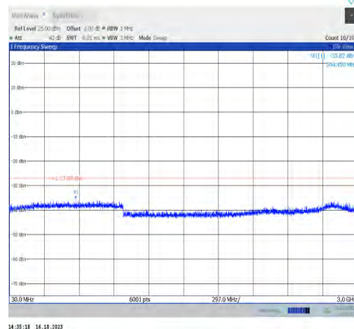
11ax160MIMO-Ant1-6825-30~3000-PASS
