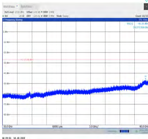
11ax160MIMO-Ant0-6665-10000~40000-PASS
