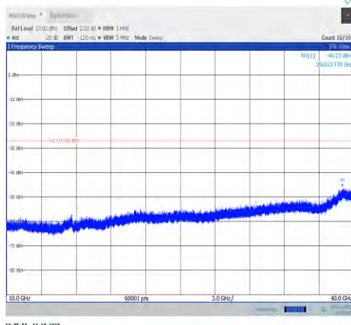
11ax80MIMO-Ant0-6465-10000~40000-PASS
