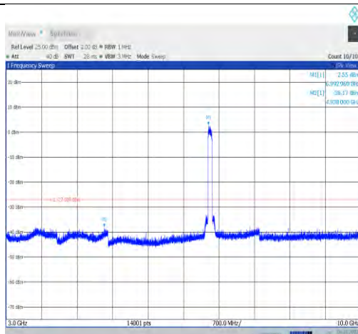
11ax80MIMO-Ant1-7025-3000~10000-PASS
