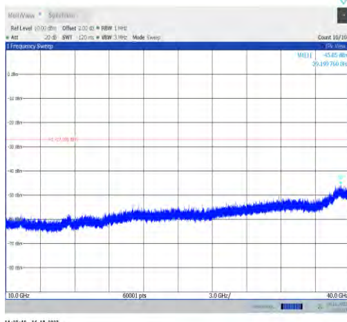
11ax160MIMO-Ant0-6505-10000~40000-PASS
