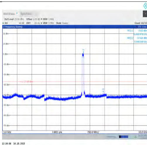
11ax80MIMO-Ant1-6865-3000~10000-PASS
