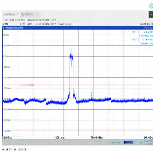
11ax160MIMO-Ant1-6185-3000~10000-PASS
