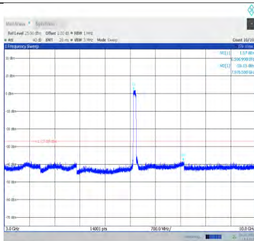
11ax80MIMO-Ant1-6625-3000~10000-PASS
