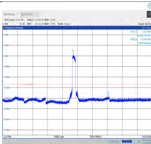
11ax160MIMO-Ant1-6345-3000~10000-PASS
