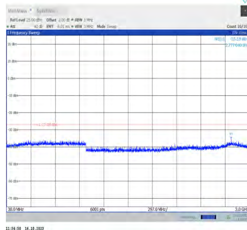
11ax80MIMO-Ant1-6785-30~3000-PASS
