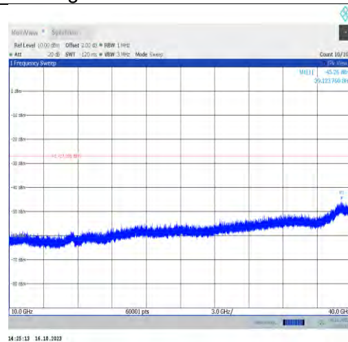
11ax160MIMO-Ant1-6505-10000~40000-PASS
