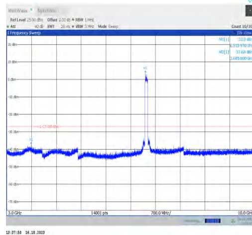
11ax80MIMO-Ant0-6945-3000~10000-PASS
