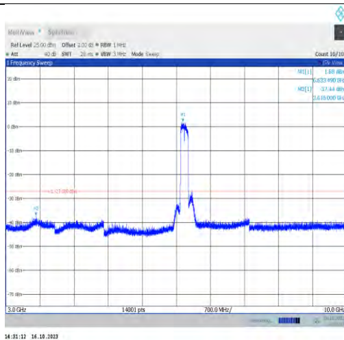
11ax160MIMO-Ant1-6665-3000~10000-PASS
