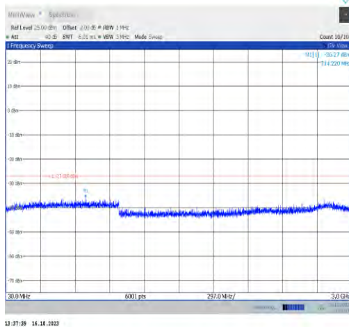
11ax80MIMO-Ant0-6945-30~3000-PASS
