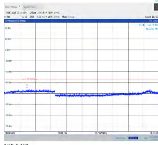
11ax160MIMO-Ant1-6505-30~3000-PASS
