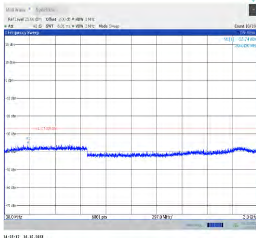
11ax160MIMO-Ant0-6505-30~3000-PASS
