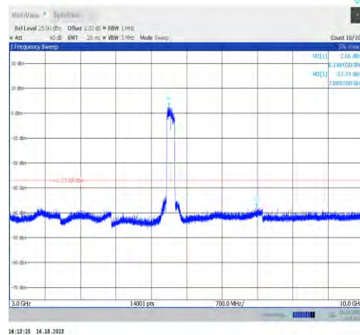
11ax160MIMO-Ant0-6185-3000~10000-PASS
