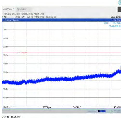
11ax80MIMO-Ant0-6945-10000~40000-PASS
