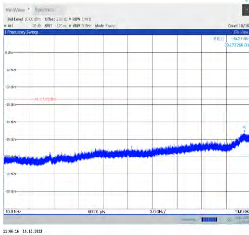
11ax80MIMO-Ant0-6705-10000~40000-PASS
