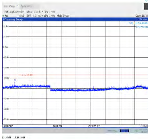
11ax80MIMO-Ant0-6545-30~3000-PASS
