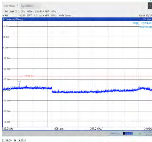
11ax80MIMO-Ant0-6785-30~3000-PASS
