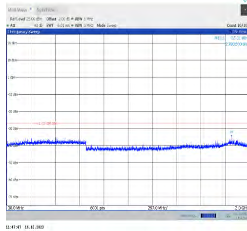
11ax80MIMO-Ant1-6705-30~3000-PASS
