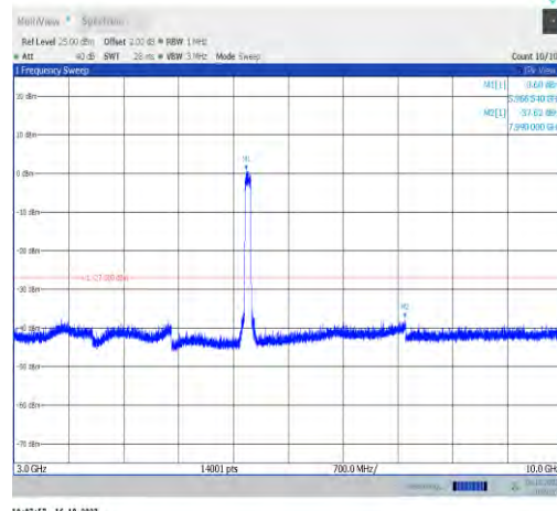
11ax80MIMO-Ant0-5985-3000~10000-PASS
