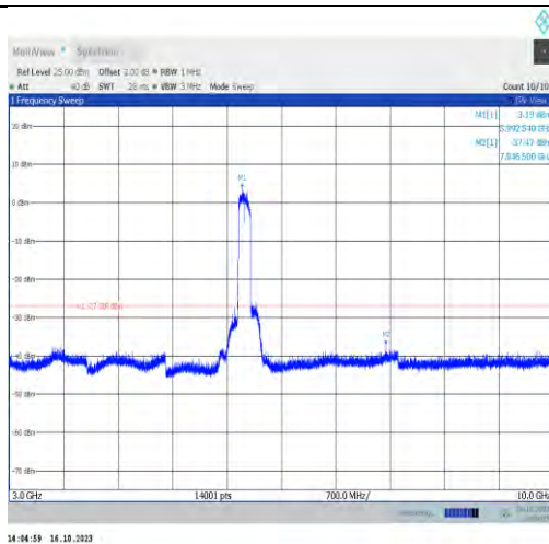
11ax160MIMO-Ant1-6025-3000~10000-PASS
