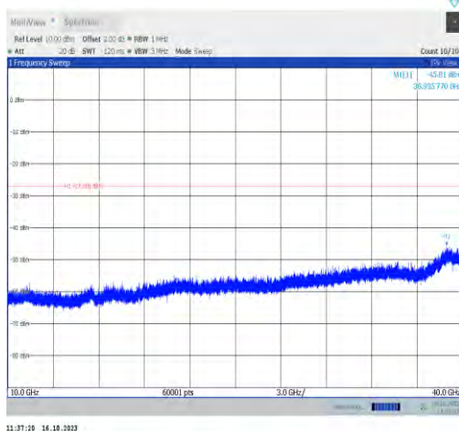
11ax80MIMO-Ant0-6545-10000~40000-PASS
