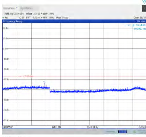
11ax80MIMO-Ant0-6145-30~3000-PASS
