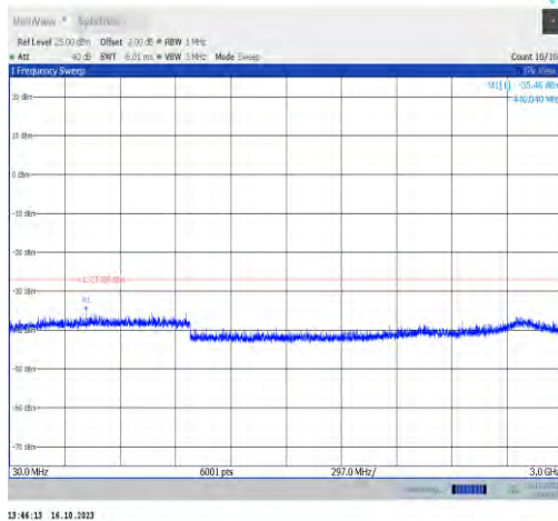
11ax80MIMO-Ant0-7025-30~3000-PASS
