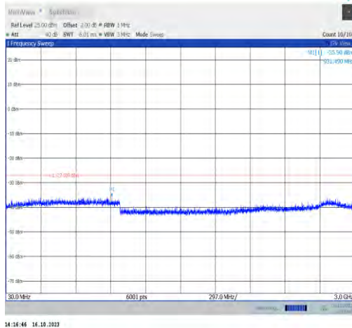
11ax160MIMO-Ant0-6345-30~3000-PASS
