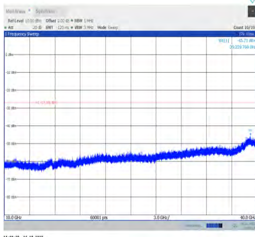
11ax160MIMO-Ant0-6025-10000~40000-PASS
