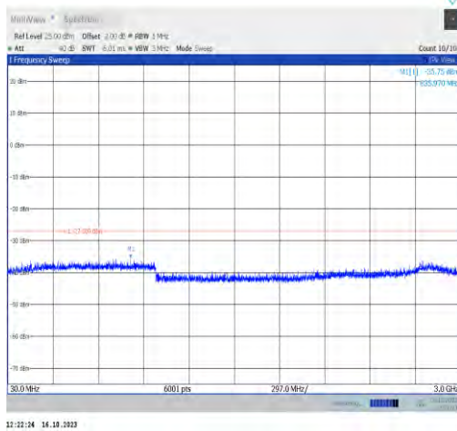
11ax80MIMO-Ant0-6865-30~3000-PASS
