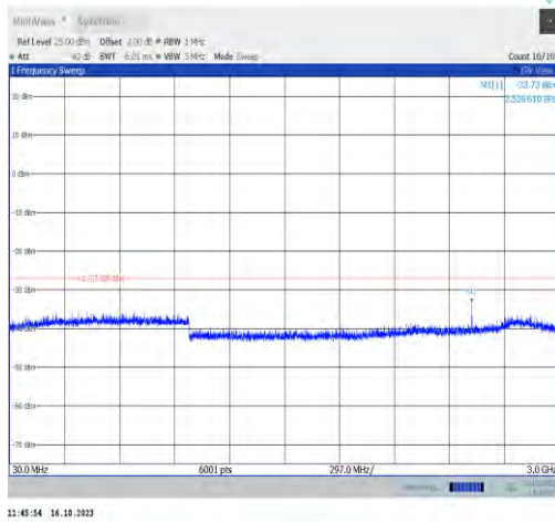
11ax80MIMO-Ant0-6705-30~3000-PASS
