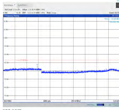
11ax80MIMO-Ant1-6465-30~3000-PASS
