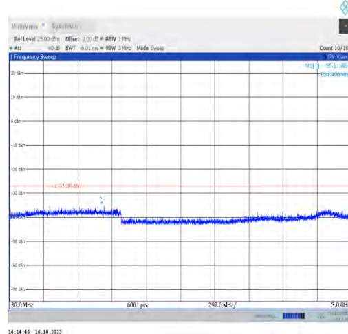
11ax160MIMO-Ant1-6185-30~3000-PASS
