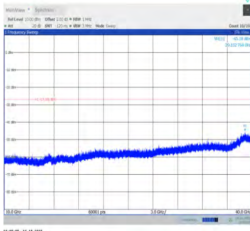
11ax80MIMO-Ant0-5985-10000~40000-PASS
