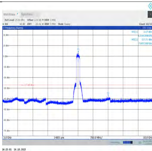
11ax160MIMO-Ant1-6505-3000~10000-PASS
