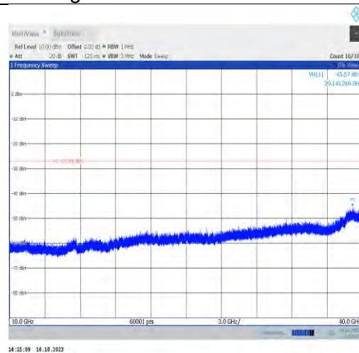
11ax160MIMO-Ant1-6185-10000~40000-PASS
