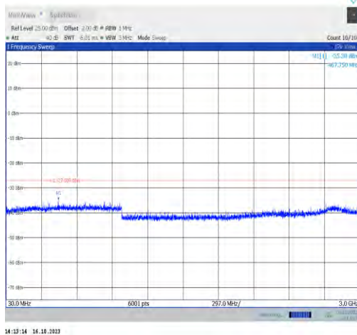
11ax160MIMO-Ant0-6185-30~3000-PASS
