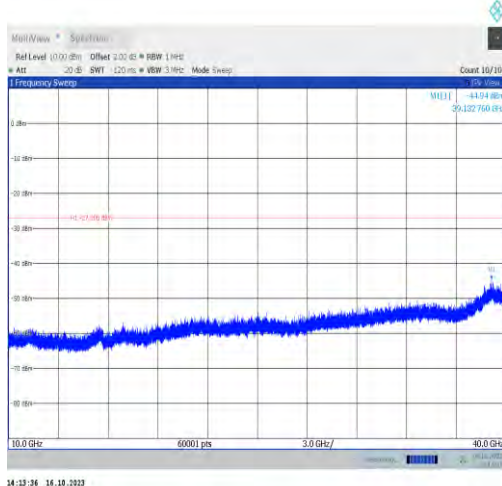
11ax160MIMO-Ant0-6185-10000~40000-PASS
