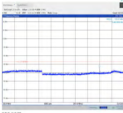
11ax80MIMO-Ant0-6465-30~3000-PASS
