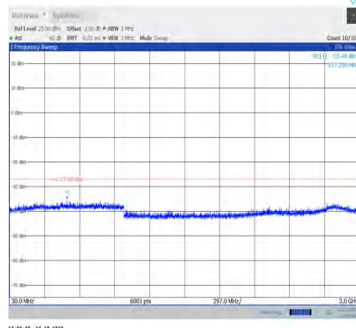
11ax160MIMO-Ant1-6025-30~3000-PASS
