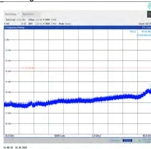
11ax80MIMO-Ant1-6705-10000~40000-PASS
