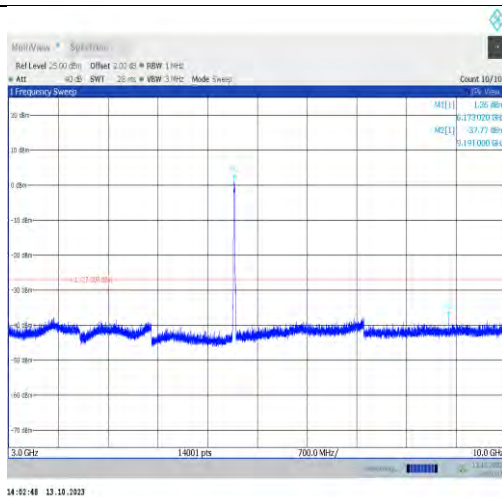
11ax20MIMO-Ant1-6175-3000~10000-PASS
