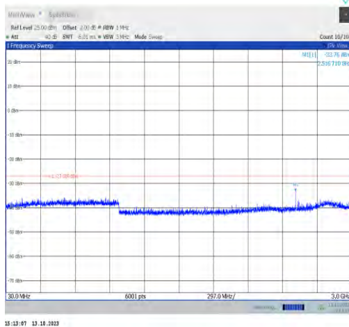
11ax20MIMO-Ant0-6515-30~3000-PASS
