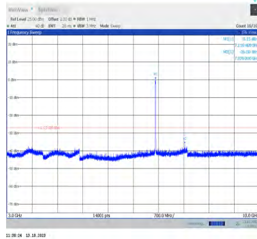
11a-CDD-Ant0-7115-3000~10000-PASS
