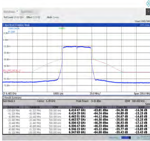
NTVN-11ax40MIMO-Ant0-6485-PASS
