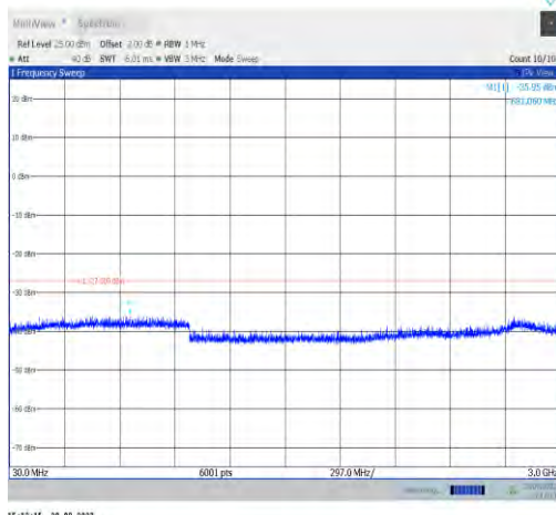
11a-CDD-Ant0-6175-30~3000-PASS
