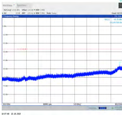
11a-CDD-Ant0-6895-10000~40000-PASS
