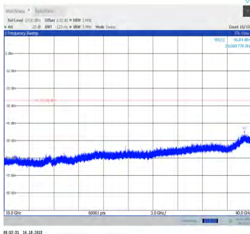
11ax40MIMO-Ant0-6445-10000~40000-PASS
