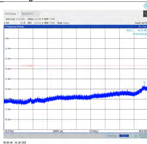
11ax40MIMO-Ant1-6445-10000~40000-PASS
