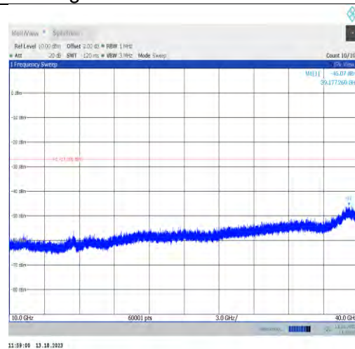
11ax20MIMO-Ant1-5955-10000~40000-PASS
