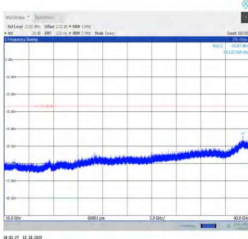
11ax20MIMO-Ant0-6175-10000~40000-PASS
