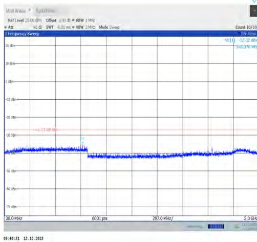
11a-CDD-Ant0-6535-30~3000-PASS
