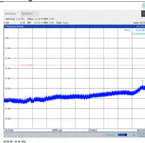
11ax20MIMO-Ant1-6415-10000~40000-PASS
