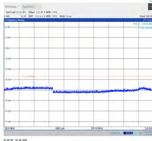
11a-CDD-Ant1-7115-30~3000-PASS
