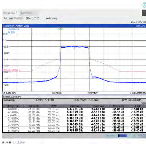
NTVN-11ax40MIMO-Ant0-6885-PASS
