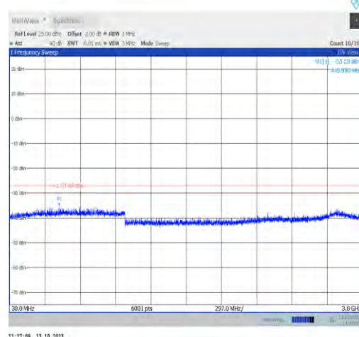
11a-CDD-Ant1-6995-30~3000-PASS
