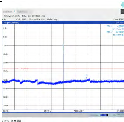
11a-CDD-Ant1-6475-3000~10000-PASS
