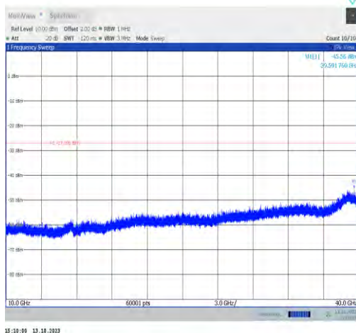
11ax20MIMO-Ant0-6475-10000~40000-PASS
