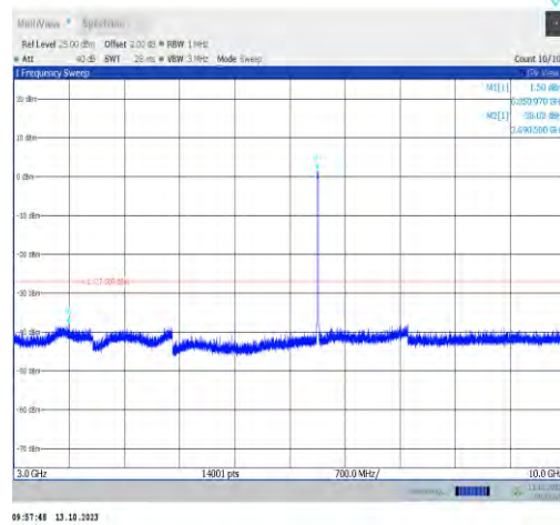
11a-CDD-Ant0-6855-3000~10000-PASS
