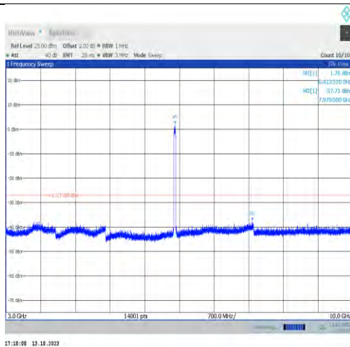
11ax40MIMO-Ant1-6405-3000~10000-PASS
