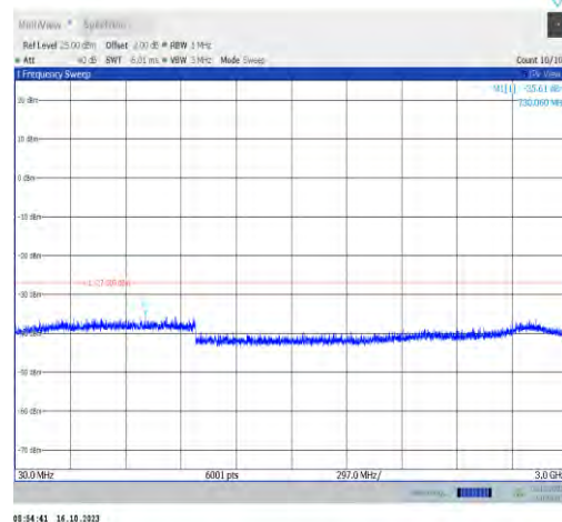
11ax40MIMO-Ant1-6445-30~3000-PASS
