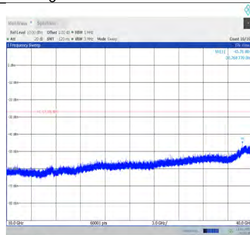
11ax20MIMO-Ant1-6995-10000~40000-PASS
