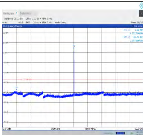
11a-CDD-Ant1-6535-3000~10000-PASS
