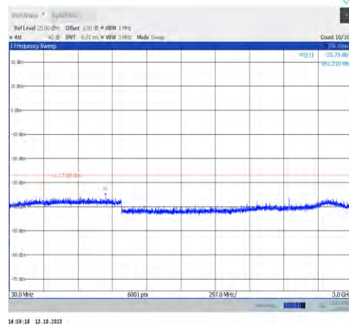
11ax20MIMO-Ant1-6415-30~3000-PASS
