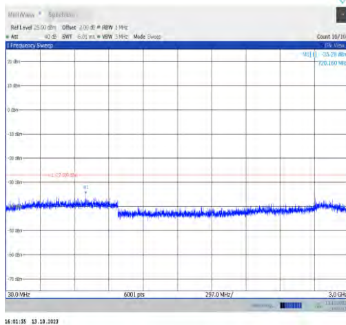
11ax20MIMO-Ant0-6995-30~3000-PASS
