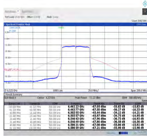
NTVN-11ax40MIMO-Ant1-6525-PASS
