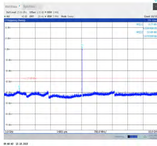
11a-CDD-Ant0-6535-3000~10000-PASS
