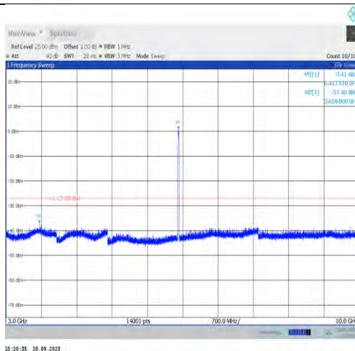
11a-CDD-Ant1-6415-3000~10000-PASS
