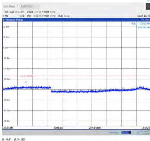
11ax20MIMO-Ant0-6855-30~3000-PASS
