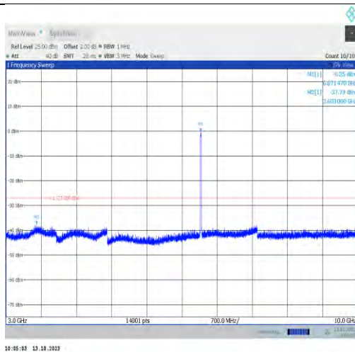
11a-CDD-Ant1-6875-3000~10000-PASS
