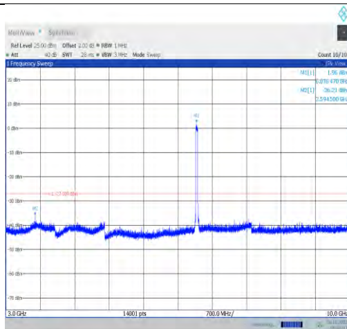
11ax40MIMO-Ant1-6885-3000~10000-PASS
