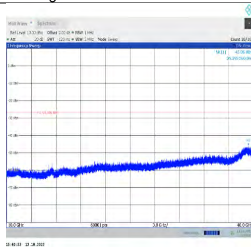
11ax20MIMO-Ant1-6855-10000~40000-PASS
