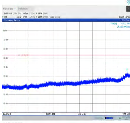
11a-CDD-Ant0-6415-10000~40000-PASS
