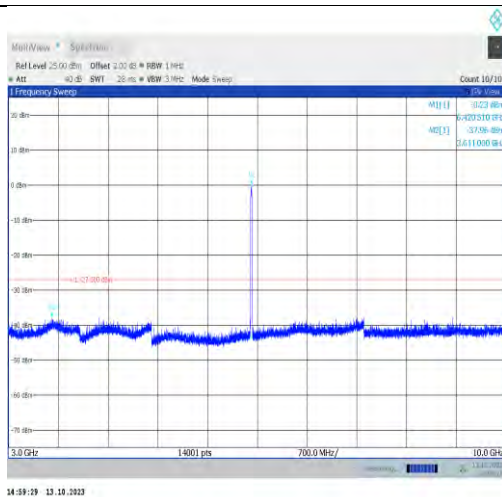
11ax20MIMO-Ant1-6415-3000~10000-PASS
