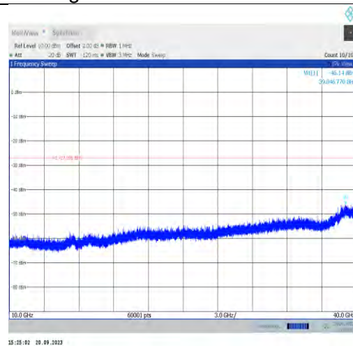
11a-CDD-Ant1-6435-10000~40000-PASS
