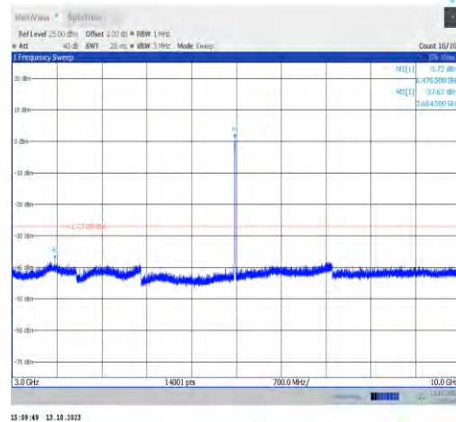
11ax20MIMO-Ant0-6475-3000~10000-PASS
