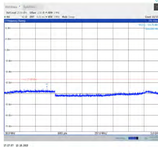
11ax40MIMO-Ant1-6405-30~3000-PASS
