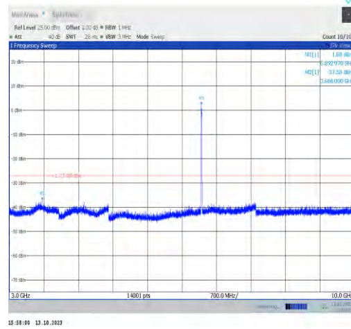
11ax20MIMO-Ant0-6895-3000~10000-PASS
