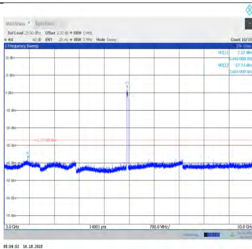
11ax40MIMO-Ant1-6445-3000~10000-PASS
