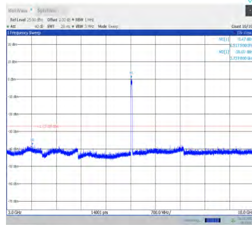
11ax40MIMO-Ant0-6525-3000~10000-PASS
