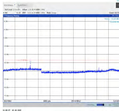
11ax20MIMO-Ant1-5955-30~3000-PASS
