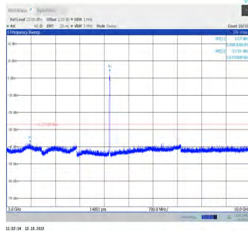
11ax20MIMO-Ant0-5955-3000~10000-PASS
