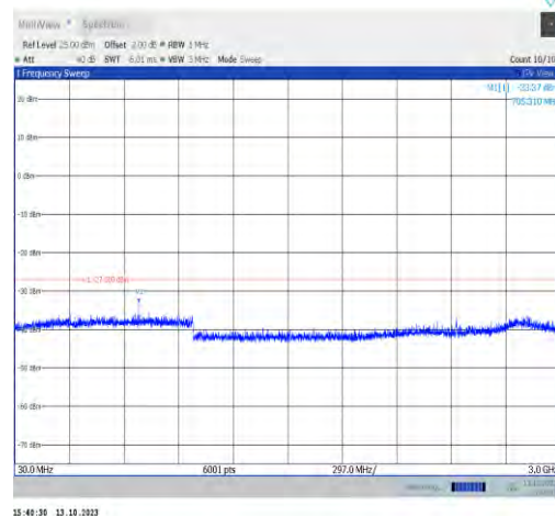
11ax20MIMO-Ant1-6855-30~3000-PASS
