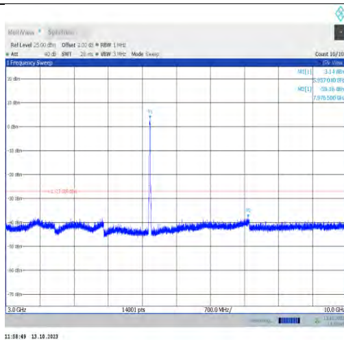
11ax20MIMO-Ant1-5955-3000~10000-PASS
