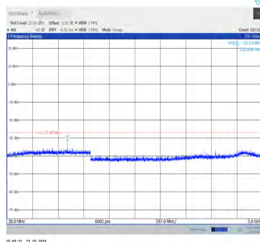
11ax20MIMO-Ant1-6435-30~3000-PASS
