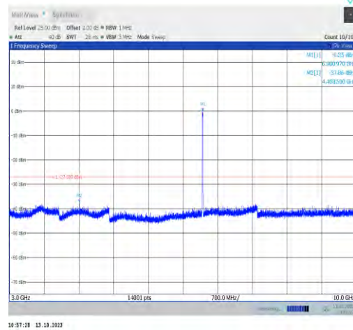
11a-CDD-Ant0-6895-3000~10000-PASS
