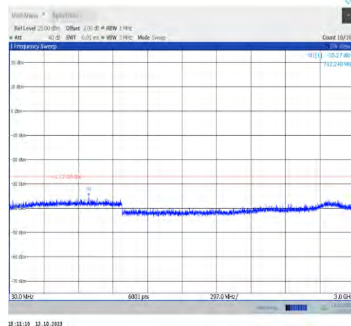
11ax20MIMO-Ant1-6475-30~3000-PASS
