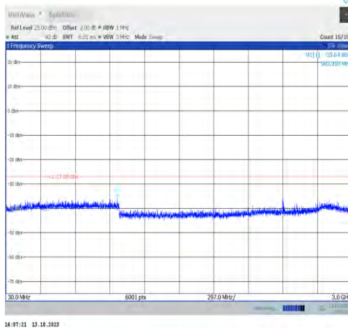
11ax20MIMO-Ant0-7115-30~3000-PASS
