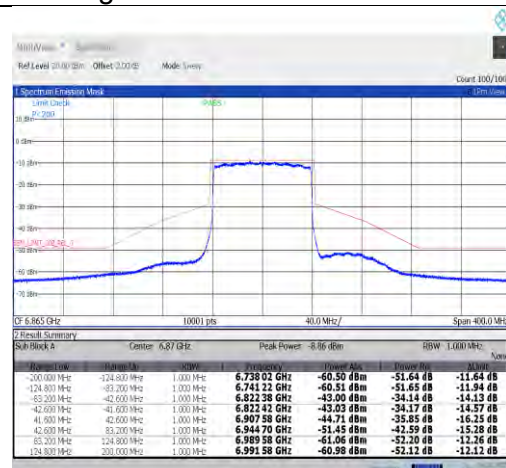
NTNV-11ax80MIMO-Ant1-6865-PASS
