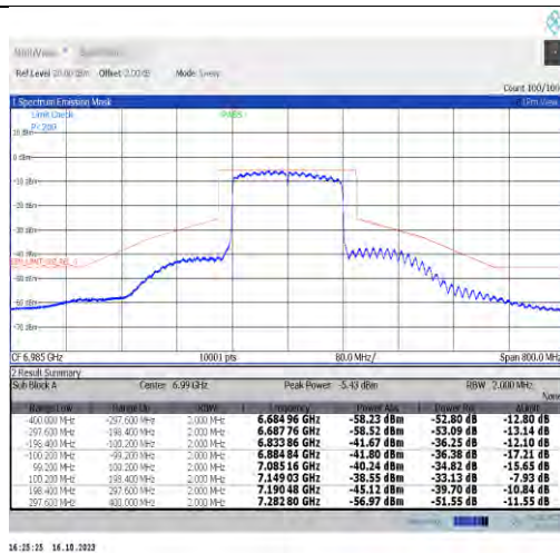
NTNV-11ax160MIMO-Ant0-6985-PASS
