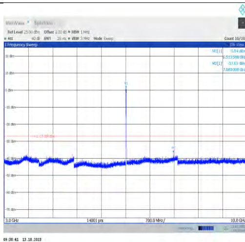
11a-CDD-Ant1-6515-3000~10000-PASS
