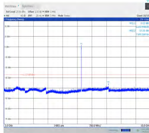
11a-CDD-Ant0-6695-3000~10000-PASS
