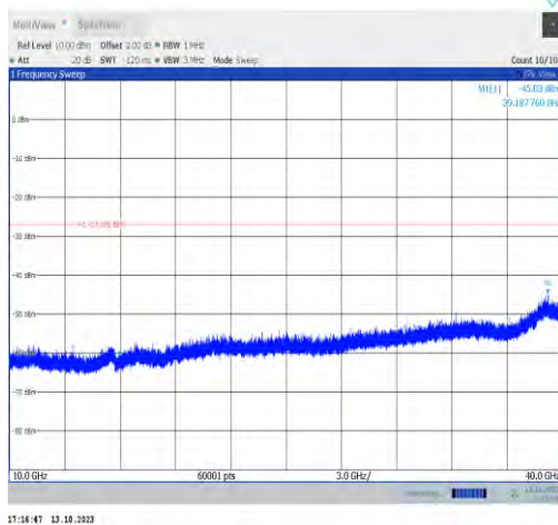
11ax40MIMO-Ant0-6405-10000~40000-PASS
