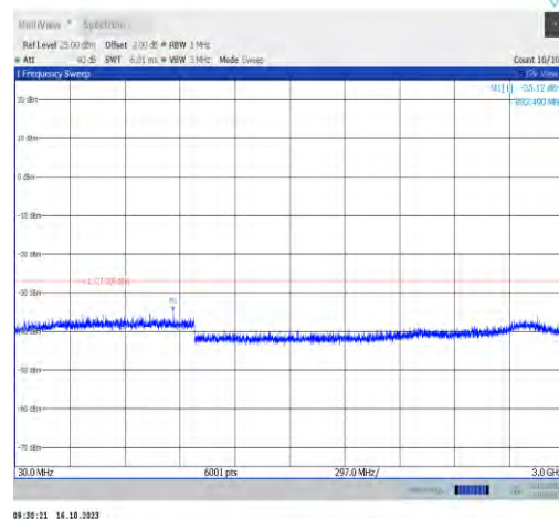
11ax40MIMO-Ant1-6565-30~3000-PASS
