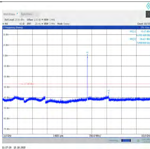
11a-CDD-Ant1-6995-3000~10000-PASS
