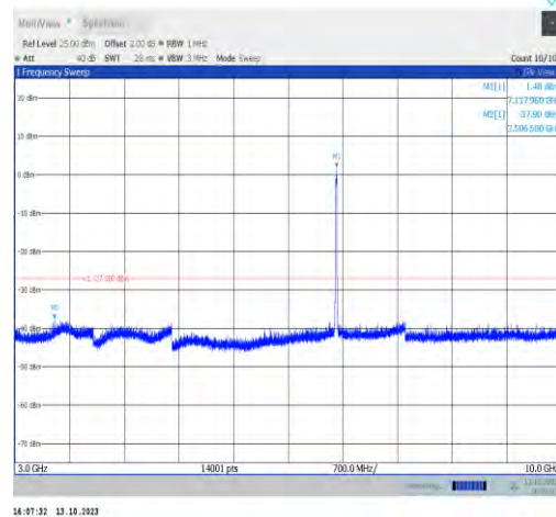
11ax20MIMO-Ant0-7115-3000~10000-PASS
