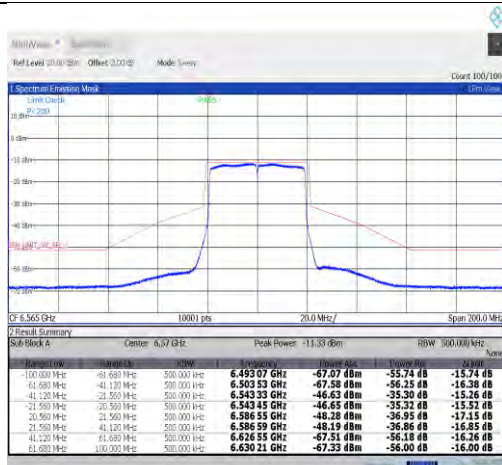
NTVN-11ax40MIMO-Ant0-6565-PASS
