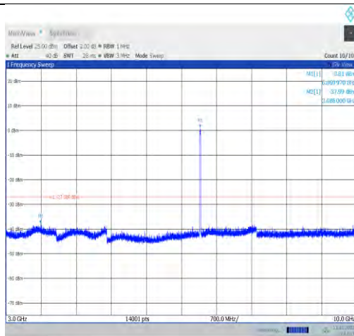
11ax20MIMO-Ant1-6875-3000~10000-PASS
