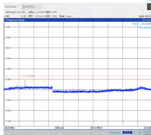
11ax40MIMO-Ant1-6845-30~3000-PASS
