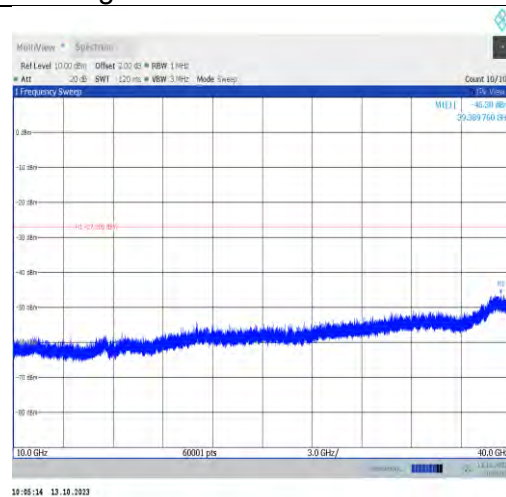
11a-CDD-Ant1-6875-10000~40000-PASS
