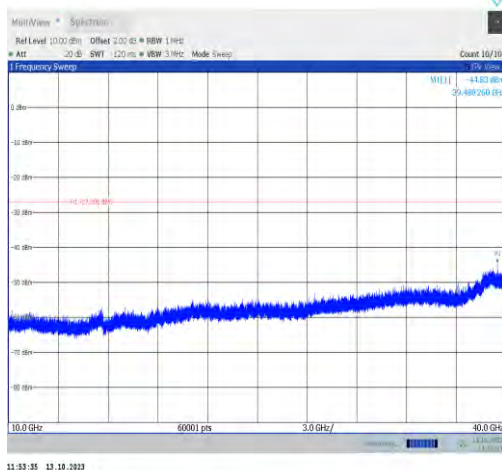
11ax20MIMO-Ant0-5955-10000~40000-PASS
