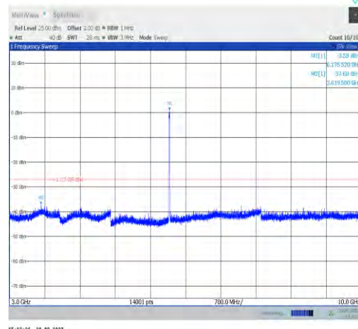
11a-CDD-Ant0-6175-3000~10000-PASS
