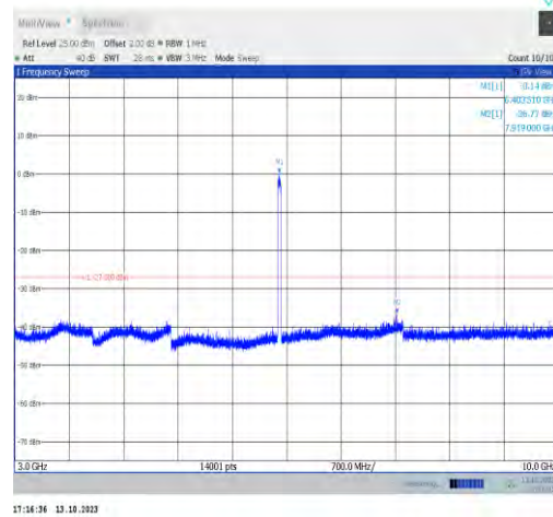
11ax40MIMO-Ant0-6405-3000~10000-PASS
