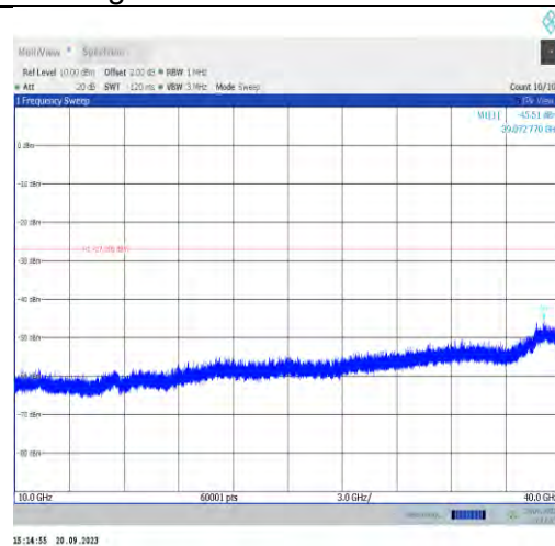
11a-CDD-Ant1-6175-10000~40000-PASS
