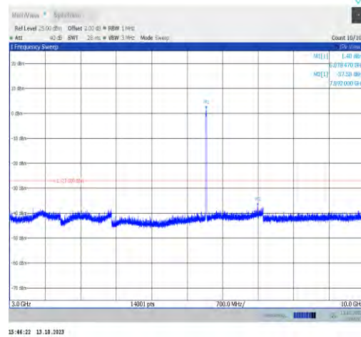
11ax20MIMO-Ant0-6875-3000~10000-PASS
