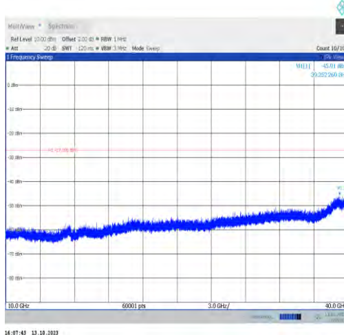
11ax20MIMO-Ant0-7115-10000~40000-PASS
