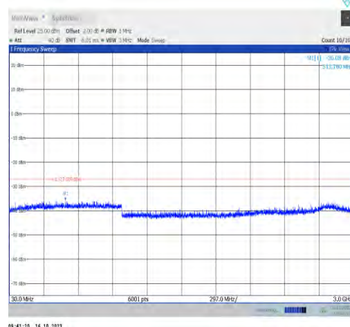
11ax40MIMO-Ant1-6885-30~3000-PASS
