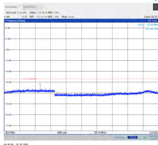
11ax40MIMO-Ant1-5965-30~3000-PASS
