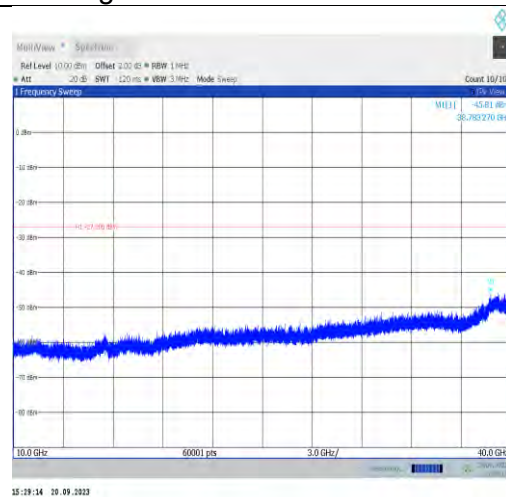
11a-CDD-Ant1-6475-10000~40000-PASS
