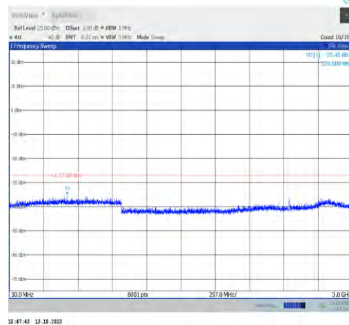
11ax20MIMO-Ant1-6875-30~3000-PASS
