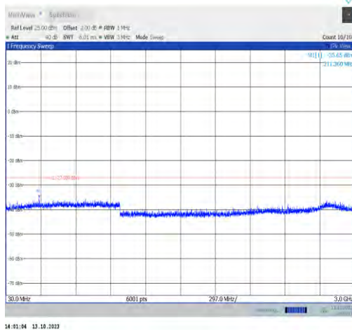
11ax20MIMO-Ant0-6175-30~3000-PASS
