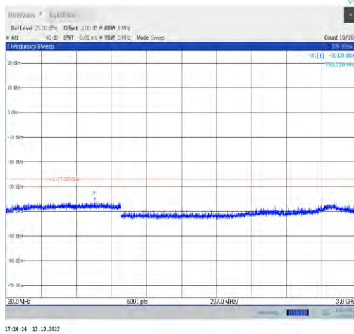
11ax40MIMO-Ant0-6405-30~3000-PASS
