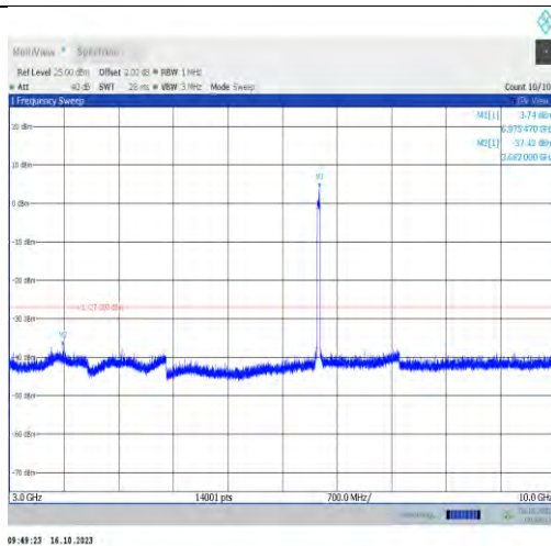
11ax40MIMO-Ant1-6965-3000~10000-PASS
