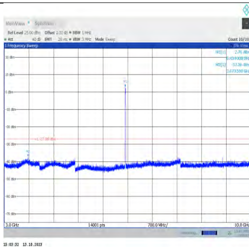
11ax20MIMO-Ant1-6435-3000~10000-PASS
