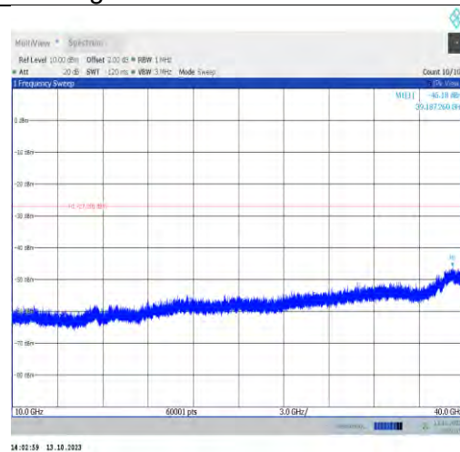
11ax20MIMO-Ant1-6175-10000~40000-PASS
