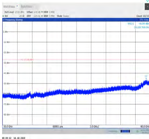
11ax40MIMO-Ant0-6565-10000~40000-PASS
