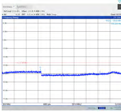
11a-CDD-Ant0-6875-30~3000-PASS
