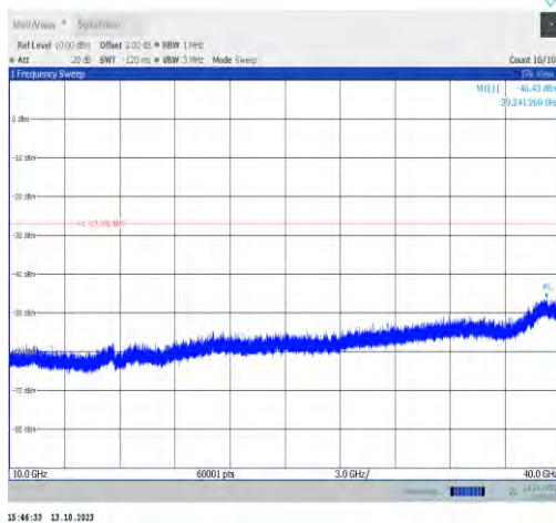
11ax20MIMO-Ant0-6875-10000~40000-PASS
