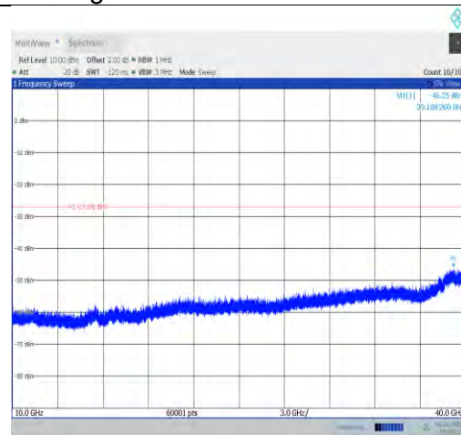
11ax40MIMO-Ant1-6485-10000~40000-PASS
