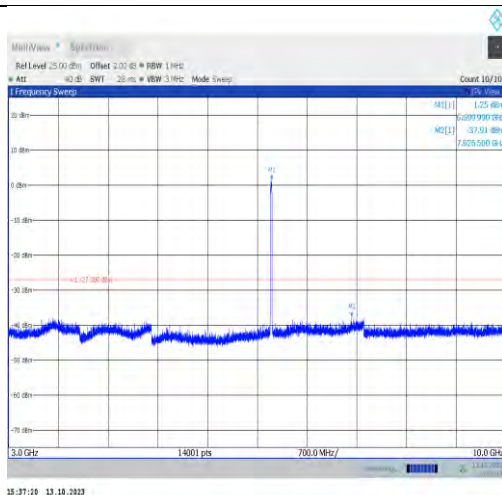
11ax20MIMO-Ant1-6695-3000~10000-PASS
