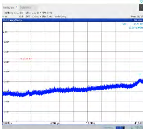
11ax40MIMO-Ant0-6525-10000~40000-PASS
