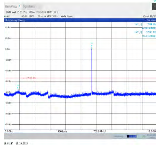
11ax20MIMO-Ant0-6995-3000~10000-PASS
