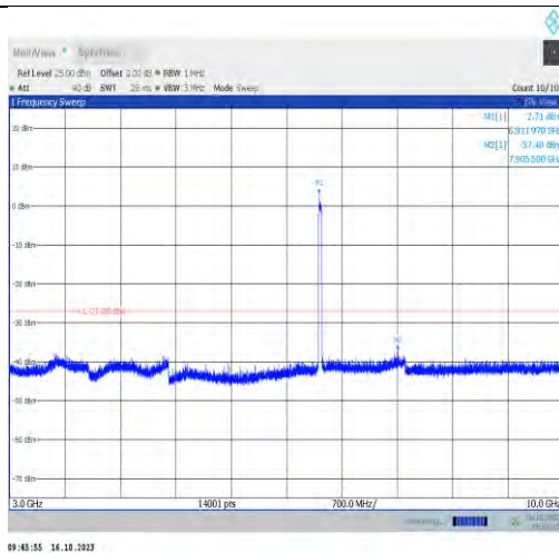
11ax40MIMO-Ant1-6925-3000~10000-PASS
