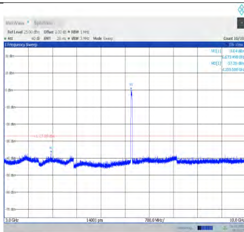
11ax40MIMO-Ant1-6685-3000~10000-PASS
