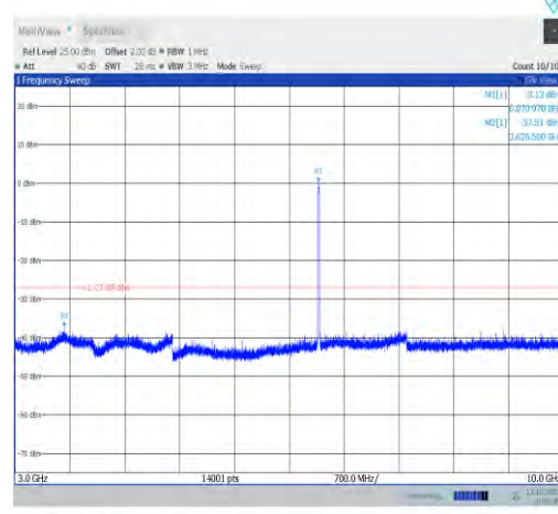
11a-CDD-Ant0-6875-3000~10000-PASS
