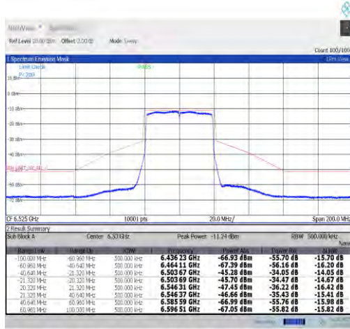
NTVN-11ax40MIMO-Ant0-6525-PASS
