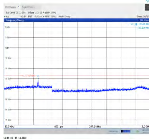
11ax20MIMO-Ant1-6995-30~3000-PASS
