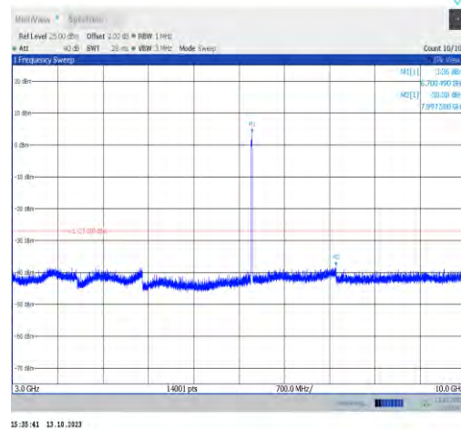
11ax20MIMO-Ant0-6695-3000~10000-PASS
