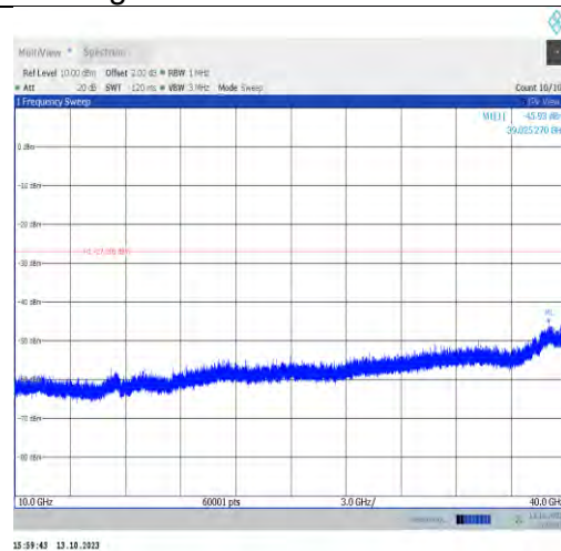
11ax20MIMO-Ant1-6895-10000~40000-PASS
