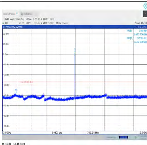
11ax20MIMO-Ant1-6475-3000~10000-PASS
