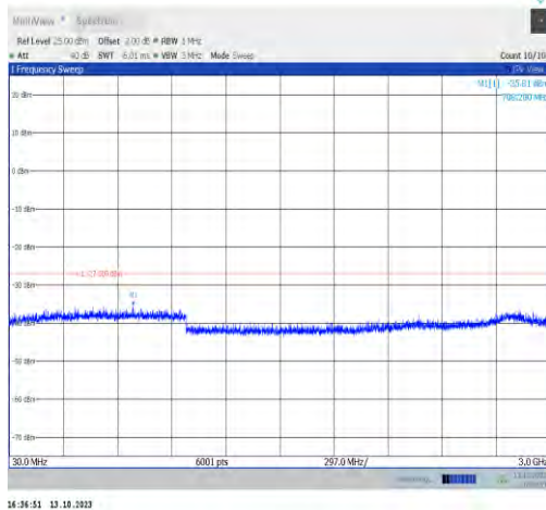
11ax40MIMO-Ant0-6165-30~3000-PASS
