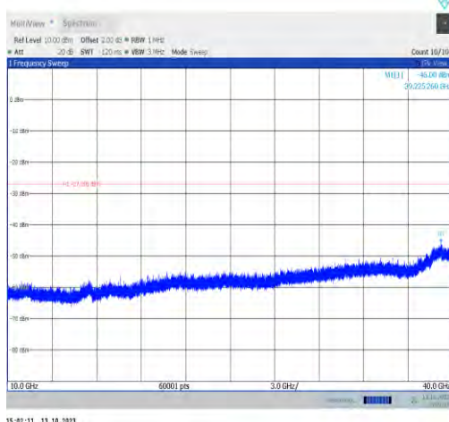
11ax20MIMO-Ant0-6435-10000~40000-PASS
