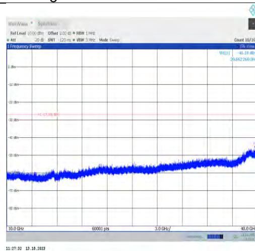
11a-CDD-Ant1-6995-10000~40000-PASS
