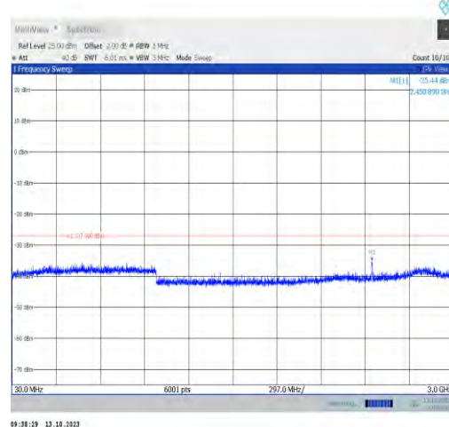
11a-CDD-Ant1-6515-30~3000-PASS
