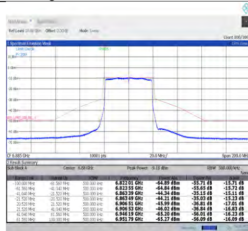
NTVN-11ax40MIMO-Ant1-6885-PASS
