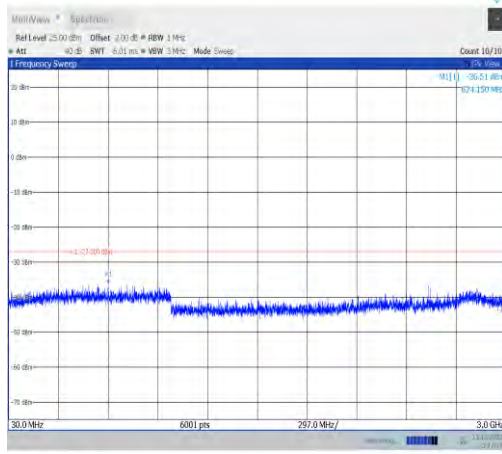
11ax20MIMO-Ant0-6535-30~3000-PASS
