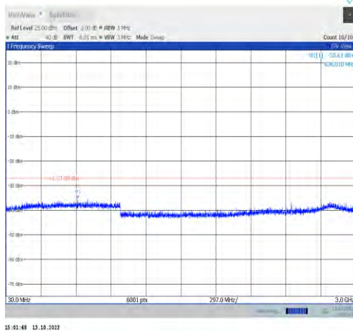
11ax20MIMO-Ant0-6435-30~3000-PASS
