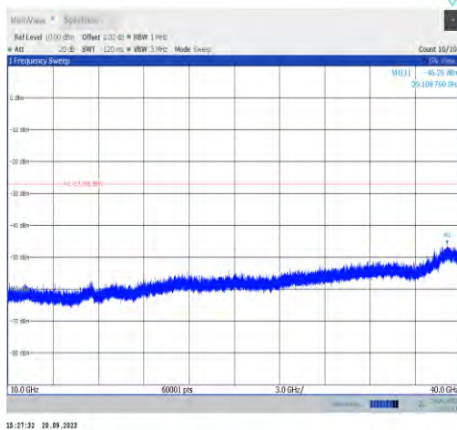
11a-CDD-Ant0-6475-10000~40000-PASS
