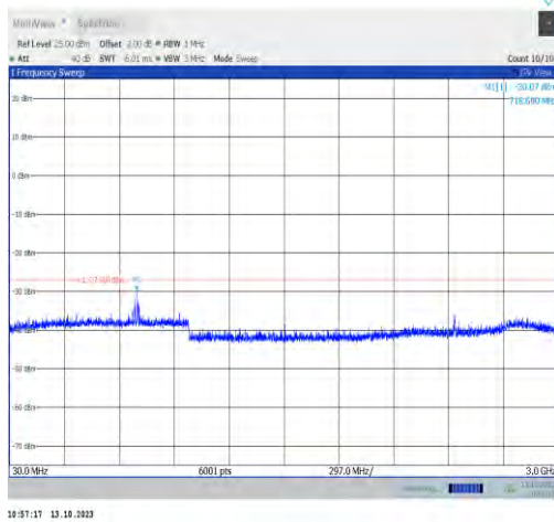
11a-CDD-Ant0-6895-30~3000-PASS
