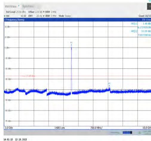
11ax20MIMO-Ant0-6175-3000~10000-PASS
