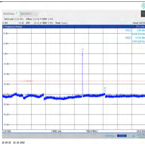
11ax20MIMO-Ant1-6895-3000~10000-PASS
