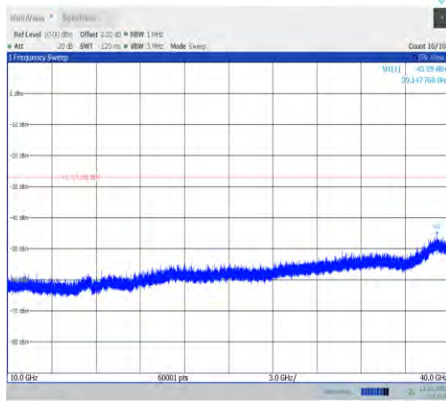
11ax20MIMO-Ant0-6535-10000~40000-PASS
