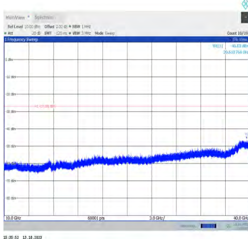
11ax20MIMO-Ant0-6695-10000~40000-PASS
