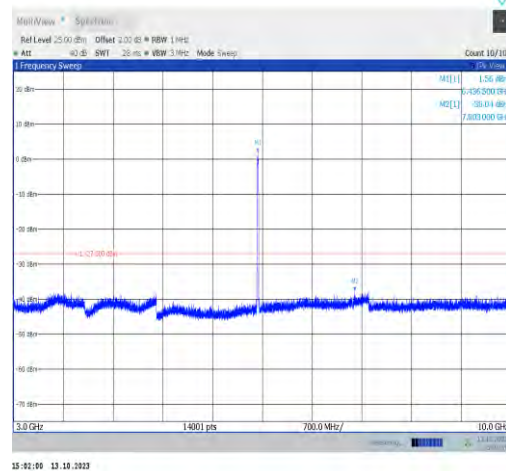
11ax20MIMO-Ant0-6435-3000~10000-PASS
