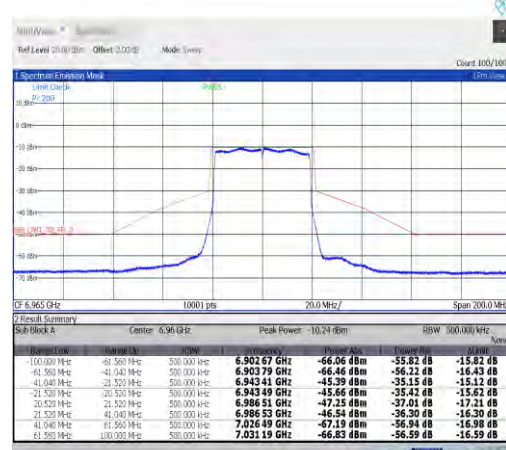
NTVN-11ax40MIMO-Ant1-6965-PASS
