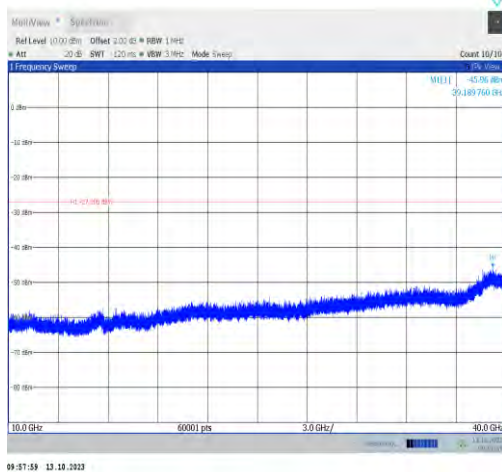
11a-CDD-Ant0-6855-10000~40000-PASS
