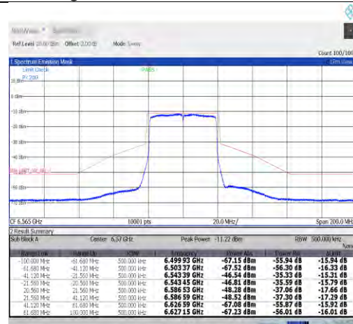
NTVN-11ax40MIMO-Ant1-6565-PASS
