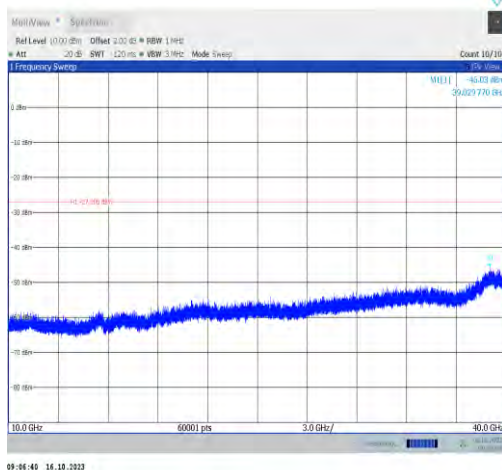
11ax40MIMO-Ant0-6485-10000~40000-PASS
