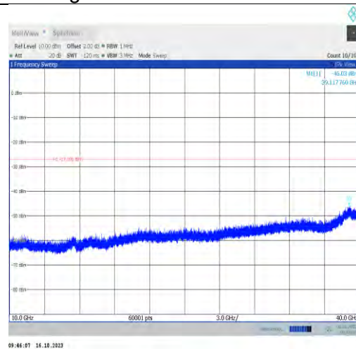
11ax40MIMO-Ant1-6925-10000~40000-PASS
