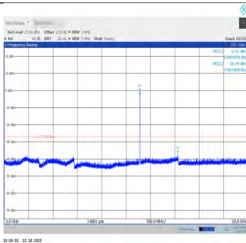
11a-CDD-Ant1-6895-3000~10000-PASS
