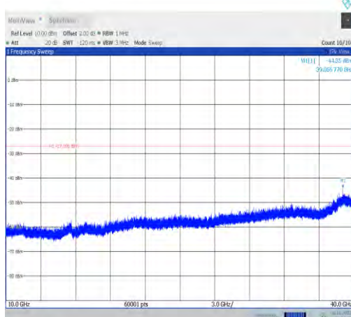
11ax40MIMO-Ant0-6925-10000~40000-PASS
