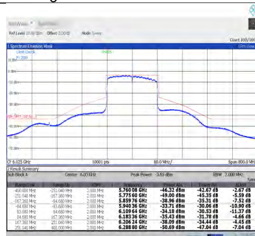
NTNV-11ax160MIMO-Ant1-6025-PASS
