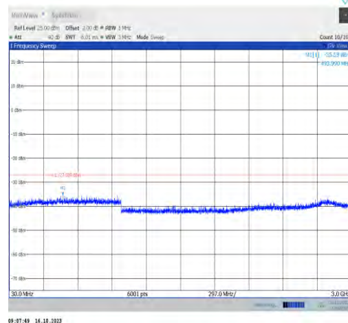
11ax40MIMO-Ant1-6485-30~3000-PASS
