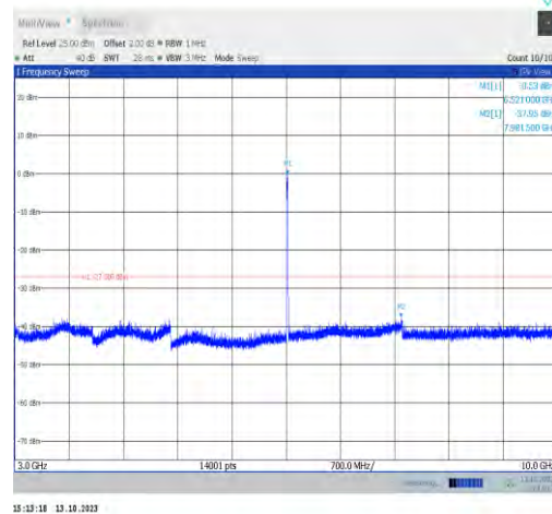
11ax20MIMO-Ant0-6515-3000~10000-PASS
