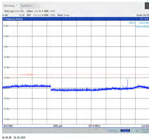
11ax20MIMO-Ant0-6475-30~3000-PASS
