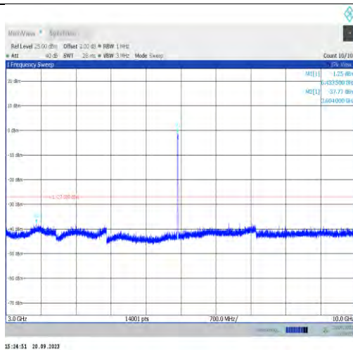
11a-CDD-Ant1-6435-3000~10000-PASS
