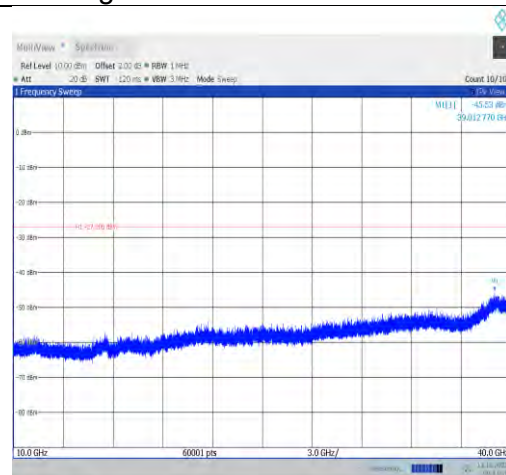
11a-CDD-Ant1-6535-10000~40000-PASS
