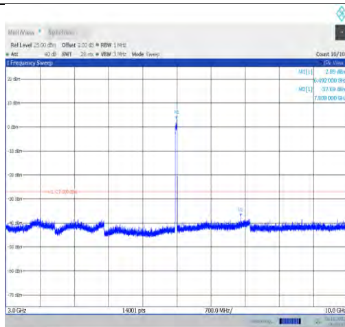
11ax40MIMO-Ant1-6485-3000~10000-PASS
