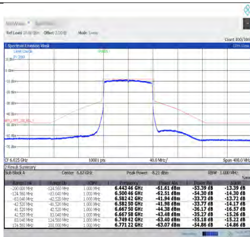
NTVN-11ax80MIMO-Ant0-6625-PASS
