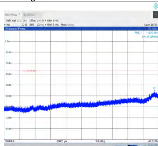
11ax20MIMO-Ant1-7115-10000~40000-PASS
