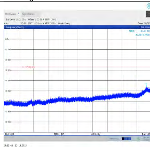
11ax20MIMO-Ant1-6435-10000~40000-PASS
