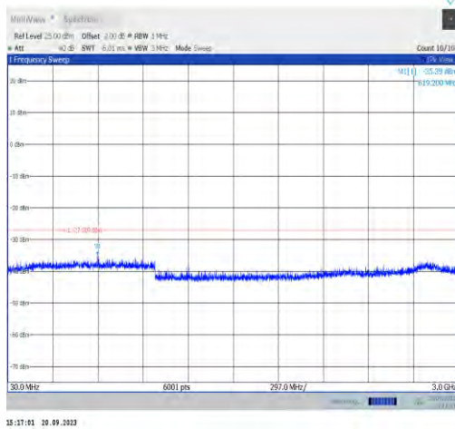
11a-CDD-Ant0-6415-30~3000-PASS
