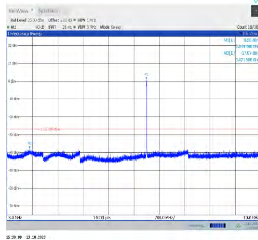
11ax20MIMO-Ant0-6855-3000~10000-PASS
