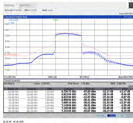
NTNV-11ax160MIMO-Ant1-6985-PASS
