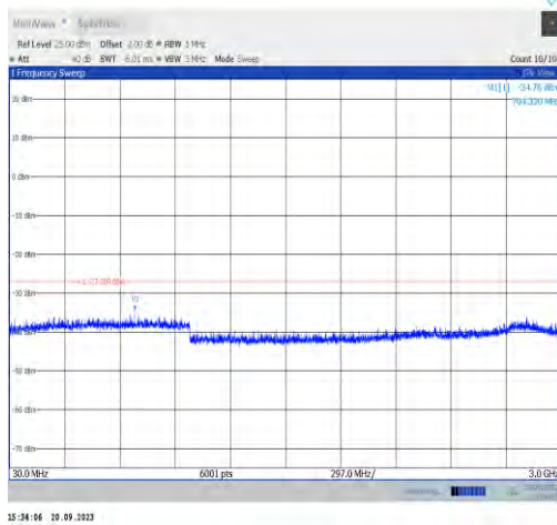
11a-CDD-Ant0-6515-30~3000-PASS
