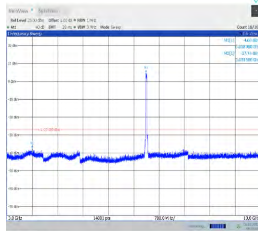
11ax40MIMO-Ant0-6845-3000~10000-PASS
