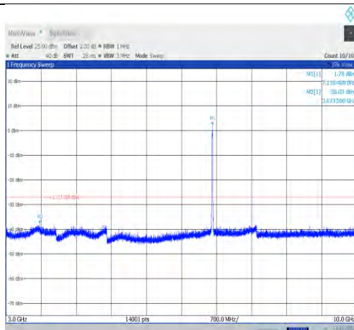
11ax20MIMO-Ant1-7115-3000~10000-PASS
