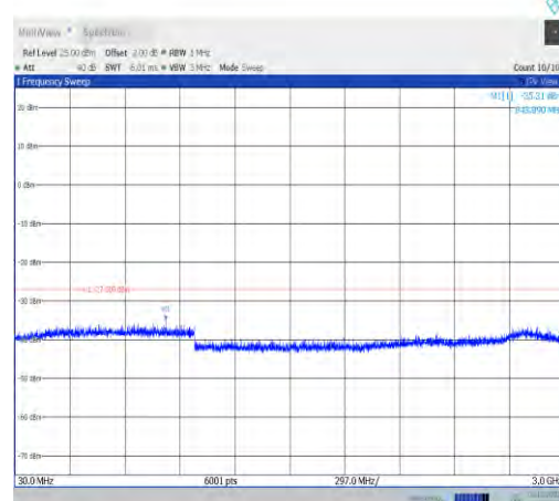
11ax40MIMO-Ant1-6925-30~3000-PASS
