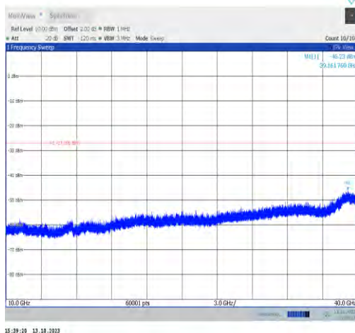
11ax20MIMO-Ant0-6855-10000~40000-PASS
