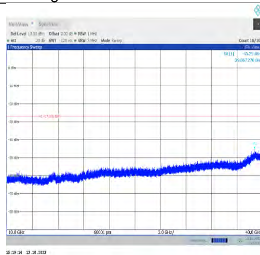
11ax20MIMO-Ant1-6535-10000~40000-PASS
