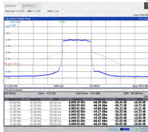
NTVN-11ax40MIMO-Ant1-6925-PASS
