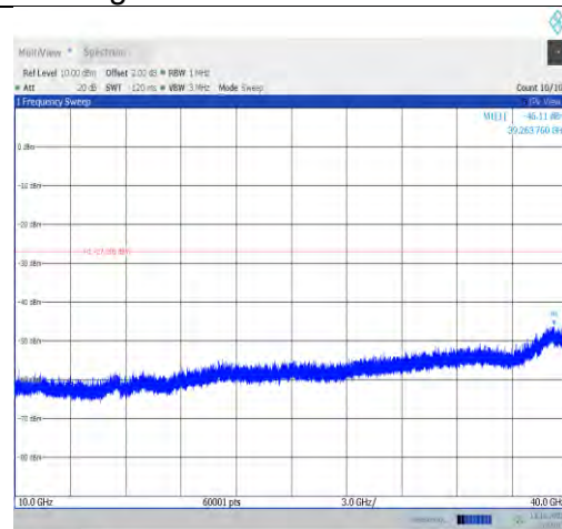
11ax20MIMO-Ant1-6515-10000~40000-PASS
