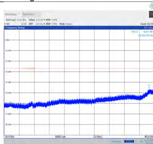
11ax40MIMO-Ant1-6685-10000~40000-PASS
