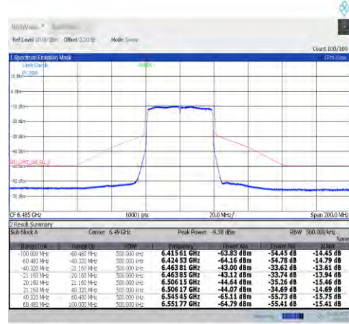
NTVN-11ax40MIMO-Ant1-6485-PASS
