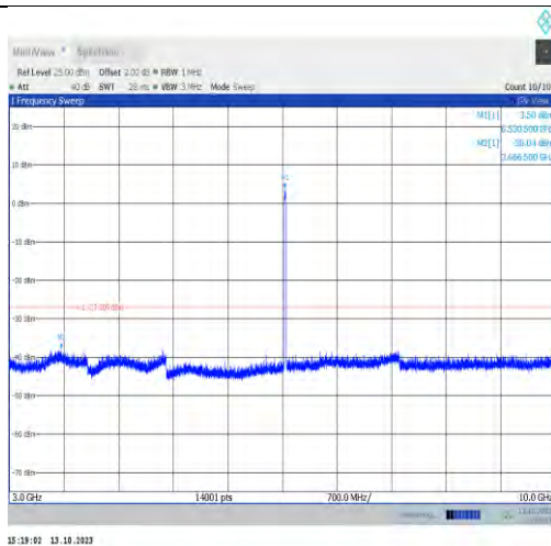
11ax20MIMO-Ant1-6535-3000~10000-PASS
