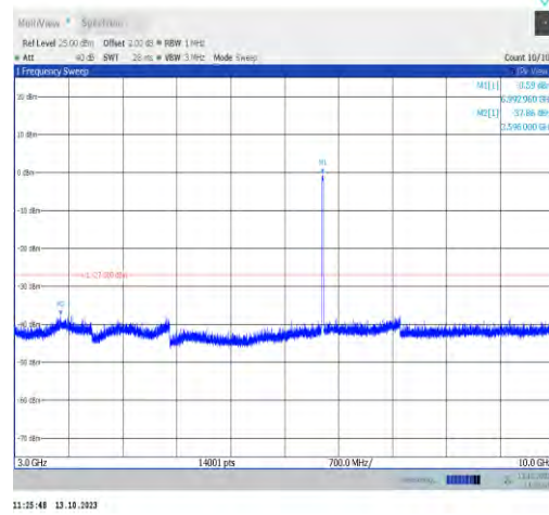
11a-CDD-Ant0-6995-3000~10000-PASS
