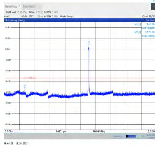
11ax40MIMO-Ant0-6885-3000~10000-PASS
