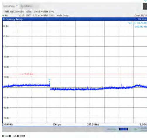
11ax20MIMO-Ant0-6875-30~3000-PASS
