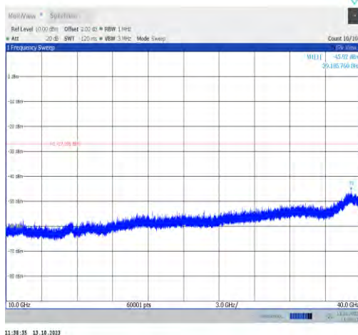
11a-CDD-Ant0-7115-10000~40000-PASS
