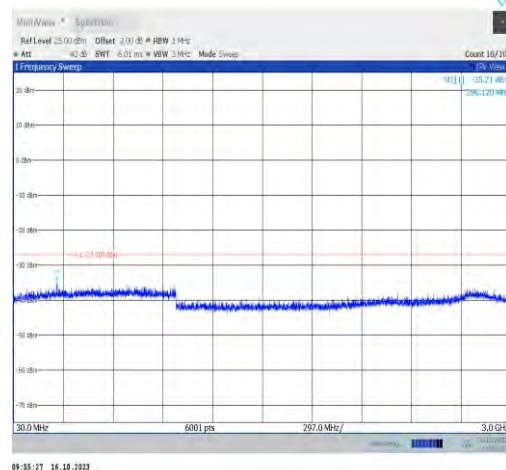
11ax40MIMO-Ant1-7085-30~3000-PASS
