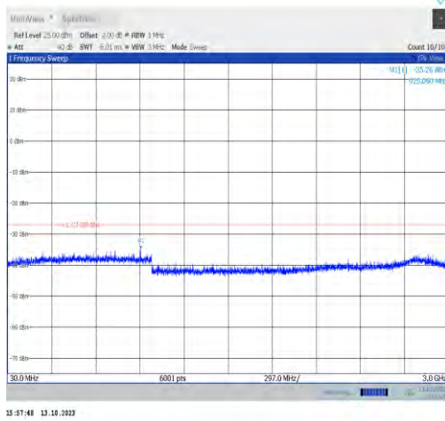
11ax20MIMO-Ant0-6895-30~3000-PASS
