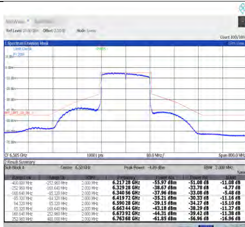
NTNV-11ax160MIMO-Ant0-6505-PASS
