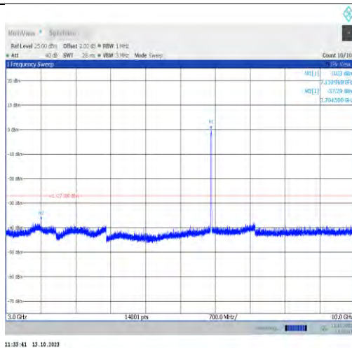
11a-CDD-Ant1-7115-3000~10000-PASS
