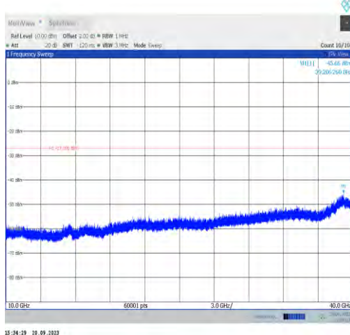
11a-CDD-Ant0-6515-10000~40000-PASS
