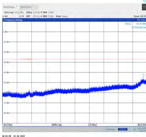
11ax20MIMO-Ant0-6995-10000~40000-PASS
