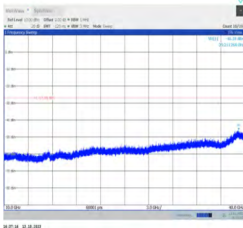
11ax40MIMO-Ant0-6165-10000~40000-PASS
