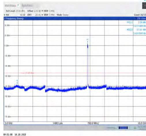
11ax40MIMO-Ant0-7085-3000~10000-PASS
