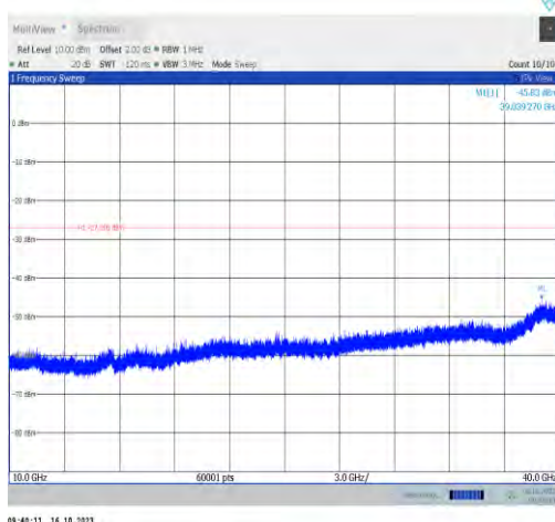
11ax40MIMO-Ant0-6885-10000~40000-PASS
