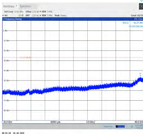
11ax40MIMO-Ant0-7085-10000~40000-PASS
