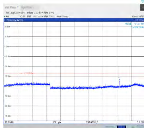
11a-CDD-Ant1-6695-30~3000-PASS
