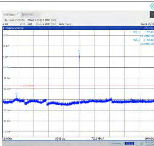
11ax20MIMO-Ant1-6515-3000~10000-PASS
