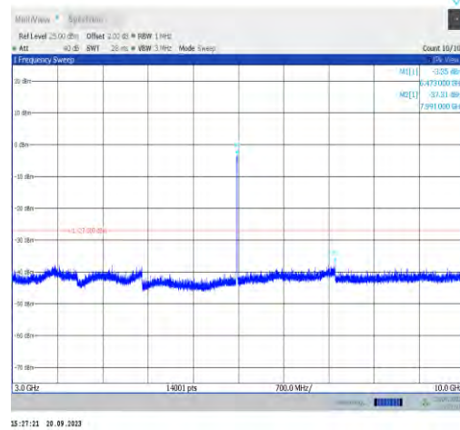
11a-CDD-Ant0-6475-3000~10000-PASS
