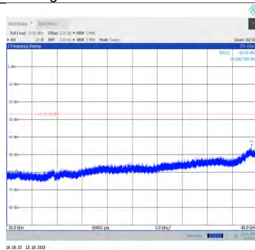
11ax40MIMO-Ant1-5965-10000~40000-PASS
