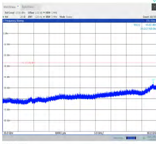
11a-CDD-Ant0-6175-10000~40000-PASS
