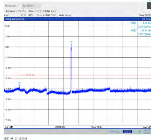
11ax40MIMO-Ant0-6165-3000~10000-PASS
