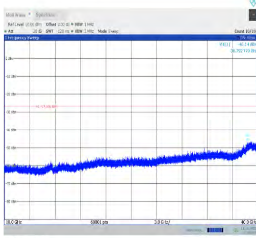
11a-CDD-Ant0-6875-10000~40000-PASS
