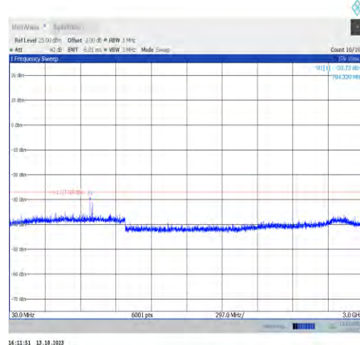
11ax20MIMO-Ant1-7115-30~3000-PASS
