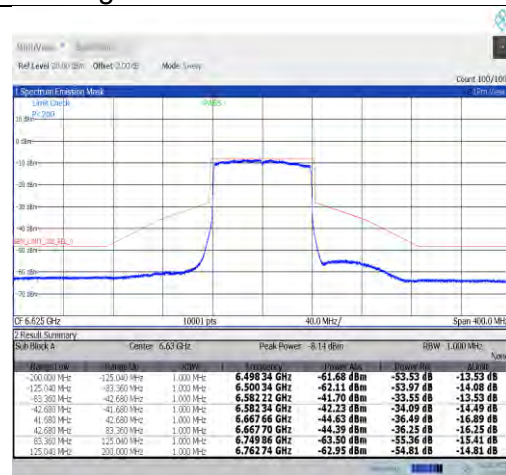
NTVN-11ax80MIMO-Ant1-6625-PASS
