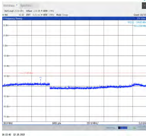
11ax40MIMO-Ant0-5965-30~3000-PASS
