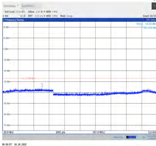
11ax40MIMO-Ant0-7085-30~3000-PASS
