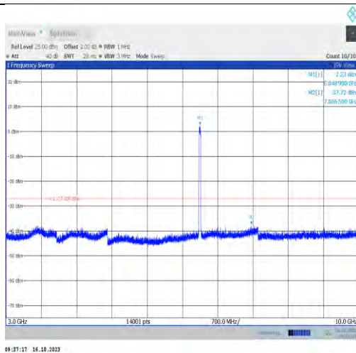
11ax40MIMO-Ant1-6845-3000~10000-PASS
