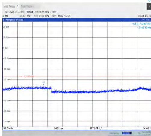
11ax40MIMO-Ant0-6525-30~3000-PASS
