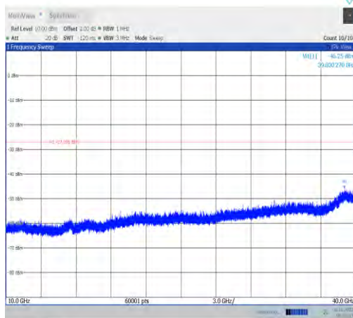
11ax40MIMO-Ant0-6845-10000~40000-PASS
