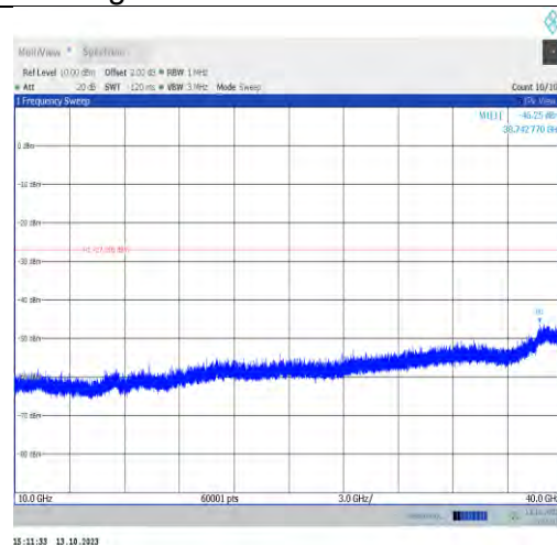
11ax20MIMO-Ant1-6475-10000~40000-PASS
