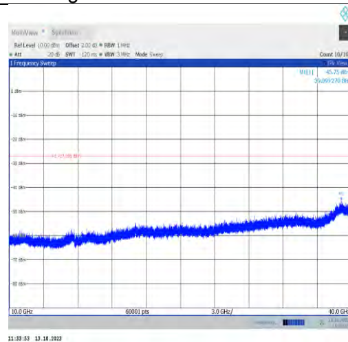
11a-CDD-Ant1-7115-10000~40000-PASS
