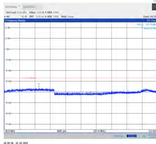
11ax40MIMO-Ant1-6165-30~3000-PASS
