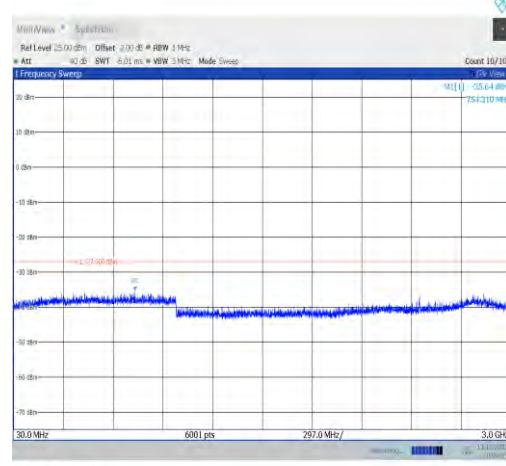
11a-CDD-Ant1-6875-30~3000-PASS
