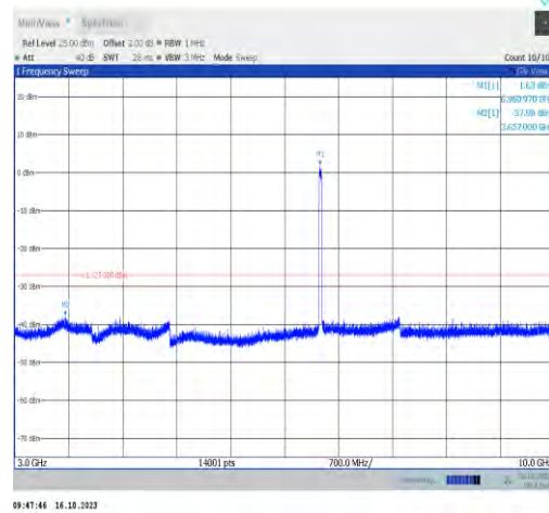
11ax40MIMO-Ant0-6965-3000~10000-PASS
