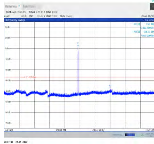
11a-CDD-Ant0-6415-3000~10000-PASS
