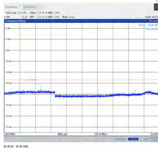
11a-CDD-Ant1-6475-30~3000-PASS
