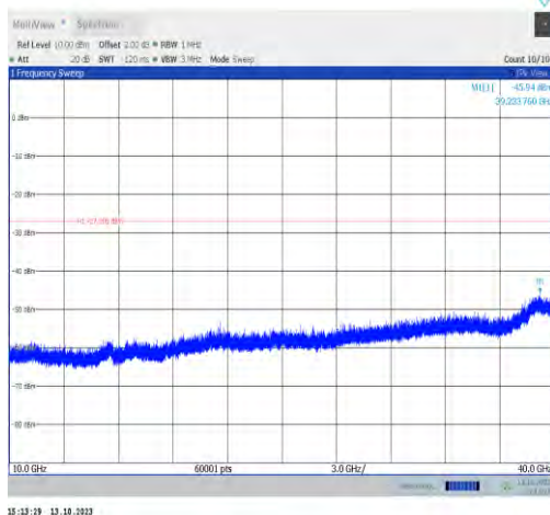
11ax20MIMO-Ant0-6515-10000~40000-PASS
