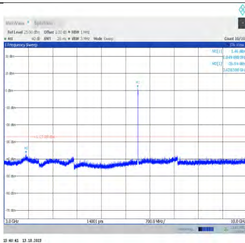
11ax20MIMO-Ant1-6855-3000~10000-PASS
