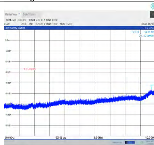
11a-CDD-Ant1-5955-10000~40000-PASS
