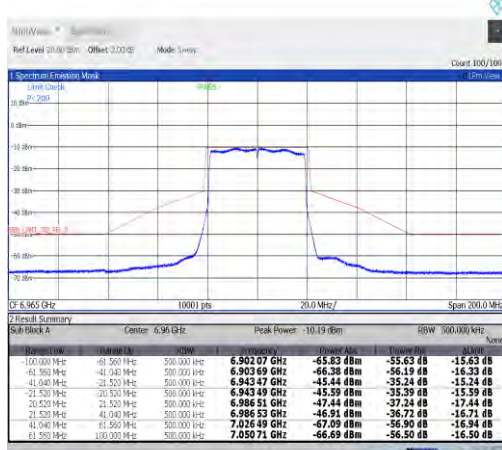
NTVN-11ax40MIMO-Ant0-6965-PASS
