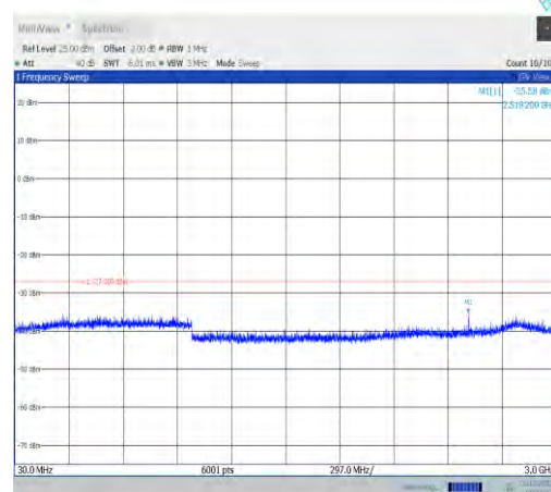
11ax40MIMO-Ant1-6525-30~3000-PASS
