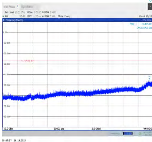
11ax40MIMO-Ant0-6965-10000~40000-PASS
