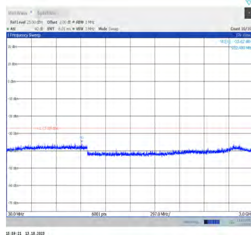
11ax20MIMO-Ant1-6895-30~3000-PASS
