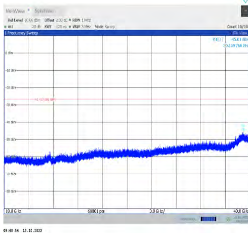
11a-CDD-Ant0-6535-10000~40000-PASS
