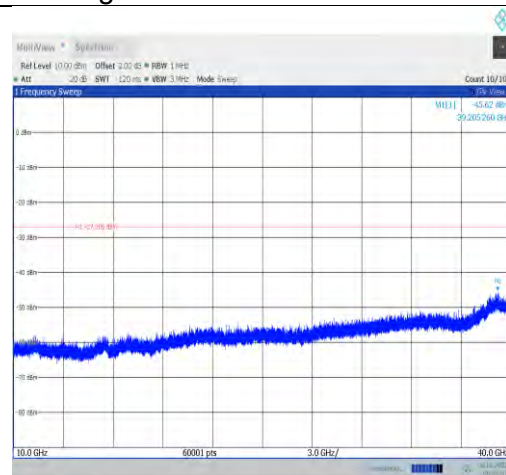
11ax40MIMO-Ant1-6885-10000~40000-PASS
