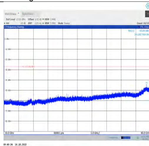
11ax40MIMO-Ant1-6965-10000~40000-PASS
