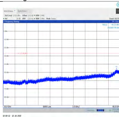
11a-CDD-Ant1-6895-10000~40000-PASS
