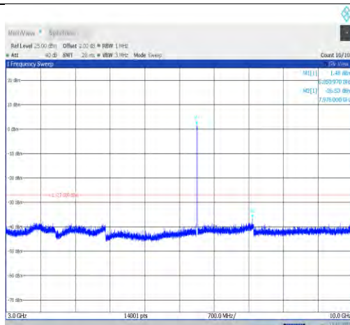
11a-CDD-Ant1-6855-3000~10000-PASS
