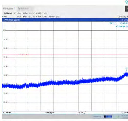
11a-CDD-Ant0-6435-10000~40000-PASS
