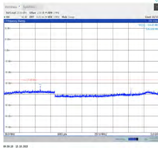
11a-CDD-Ant1-6855-30~3000-PASS
