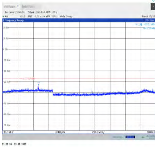
11a-CDD-Ant0-6995-30~3000-PASS
