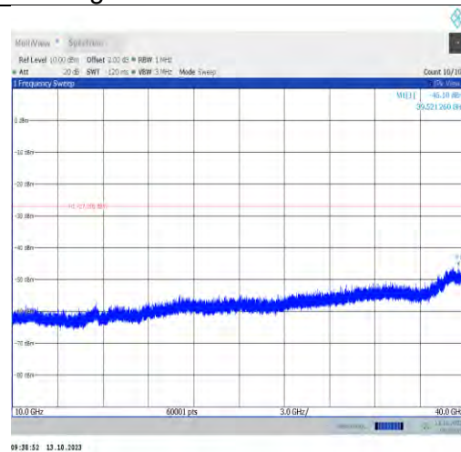
11a-CDD-Ant1-6515-10000~40000-PASS
