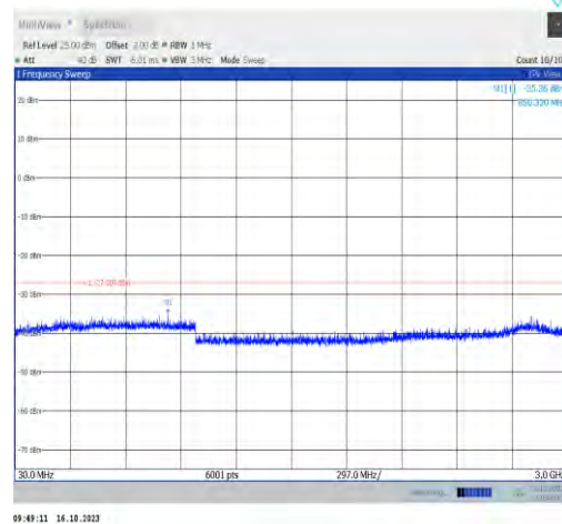
11ax40MIMO-Ant1-6965-30~3000-PASS
