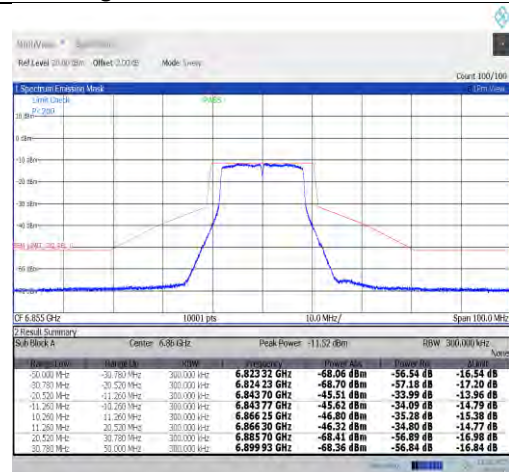
NTNV-11a-CDD-Ant1-6855-PASS
