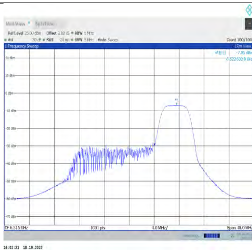
11ax20MIMO-Ant1-6515-PASS
