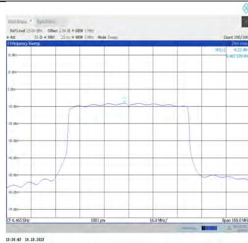
11ax80MIMO-Ant1-6465-PASS
