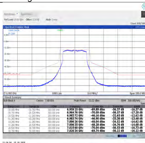
NTNV-11a-CDD-Ant1-6995-PASS
