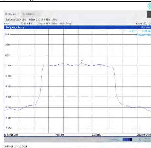
11ax40MIMO-Ant1-5965-PASS
