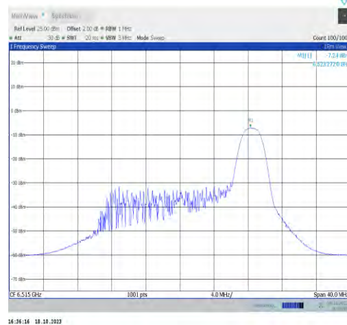
11ax20MIMO-Ant1-6515-PASS
