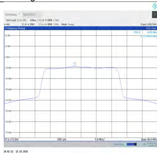
11ax20MIMO-Ant1-6175-PASS
