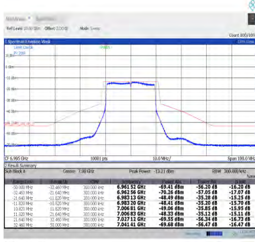
NTNV-11ax20MIMO-Ant0-6995-PASS
