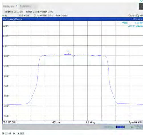
11ax40MIMO-Ant0-6525-PASS
