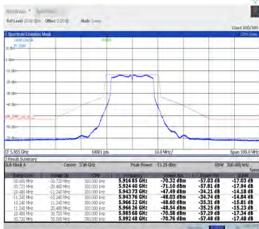
NTNV-11a-CDD-Ant0-5955-PASS
