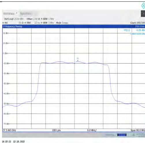
11ax40MIMO-Ant0-5965-PASS
