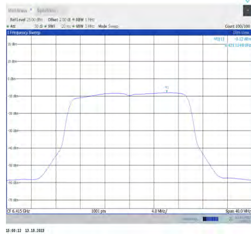
11ax20MIMO-Ant1-6415-PASS
