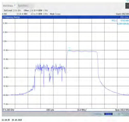
11ax80MIMO-Ant0-6385-PASS
