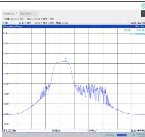
11ax20MIMO-Ant1-6175-PASS
