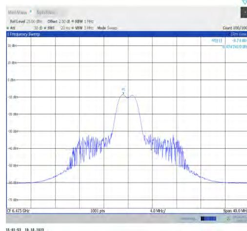
11ax20MIMO-Ant1-6475-PASS
