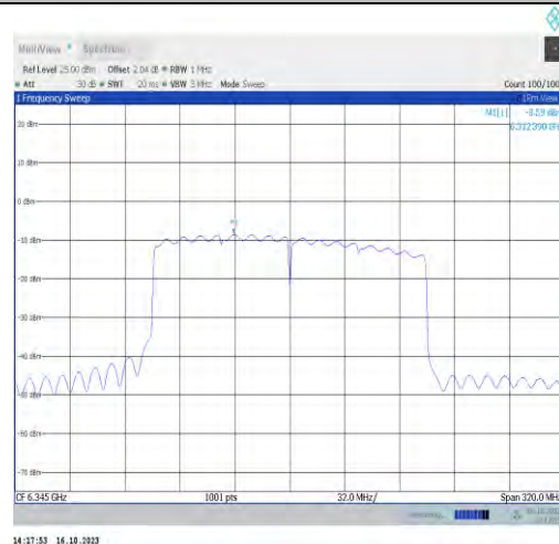
11ax160MIMO-Ant1-6345-PASS
