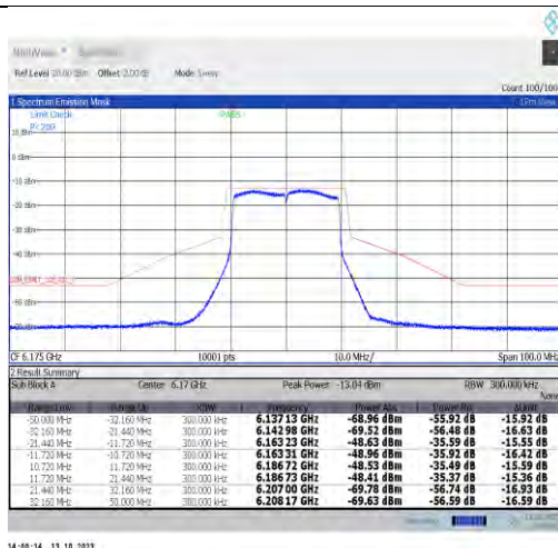
NTVN-11ax20MIMO-Ant0-6175-PASS
