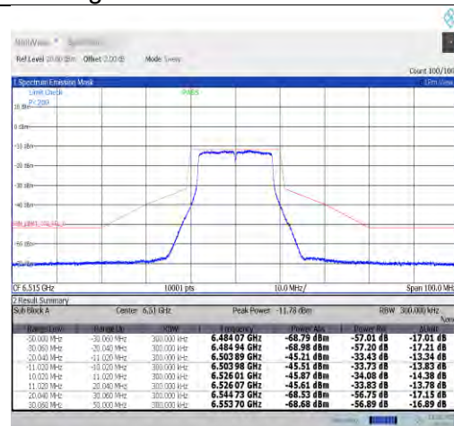
NTNV-11a-CDD-Ant1-6515-PASS
