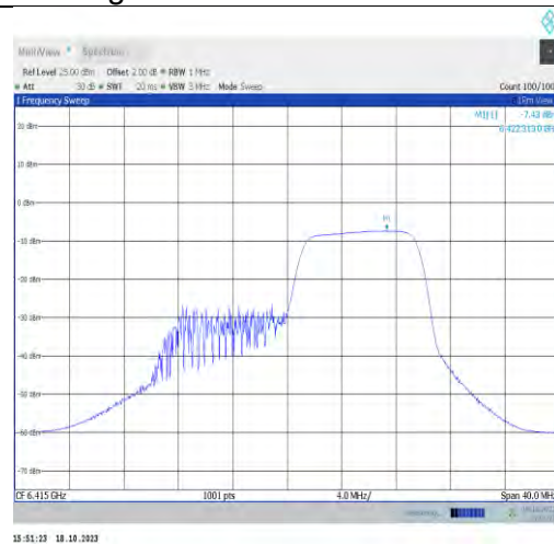
11ax20MIMO-Ant1-6415-PASS
