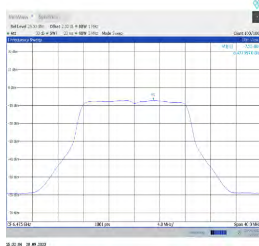
11a-CDD-Ant1-6475-PASS
