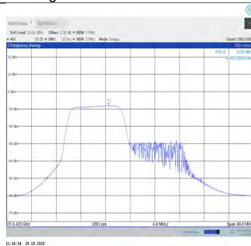
11ax20MIMO-Ant1-6435-PASS
