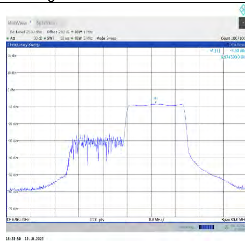
11ax40MIMO-Ant1-6965-PASS
