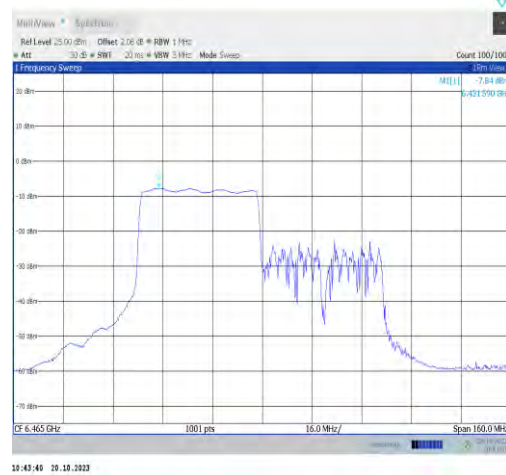
11ax80MIMO-Ant1-6465-PASS
