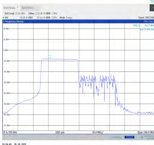
11ax80MIMO-Ant0-6705-PASS
