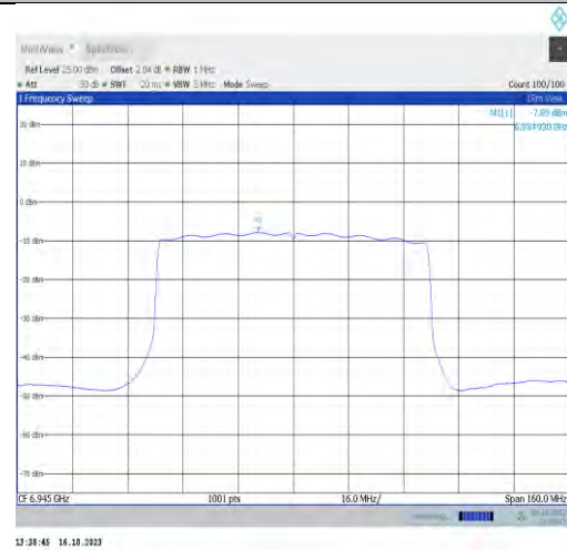
11ax80MIMO-Ant1-6945-PASS
