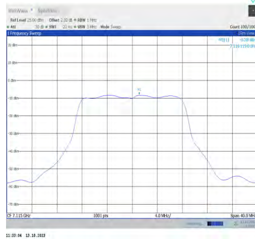
11a-CDD-Ant1-7115-PASS
