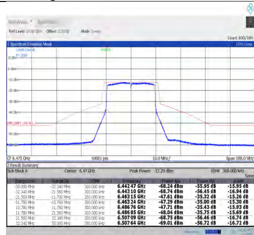
NTVN-11ax20MIMO-Ant1-6475-PASS
