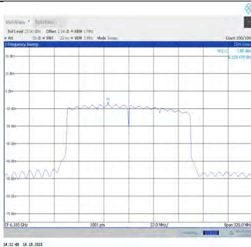
11ax160MIMO-Ant0-6185-PASS
