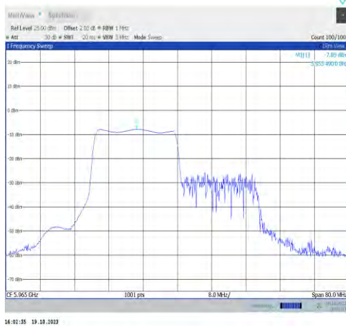
11ax40MIMO-Ant0-5965-PASS
