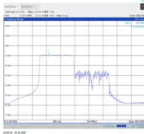
11ax80MIMO-Ant1-6945-PASS
