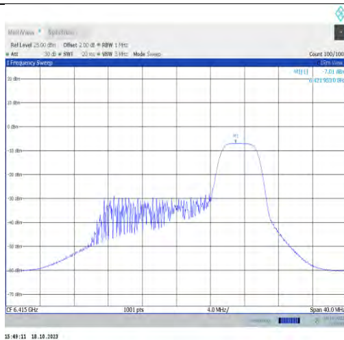
11ax20MIMO-Ant1-6415-PASS
