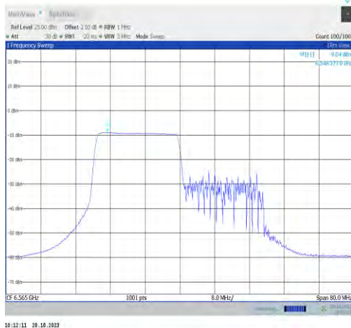
11ax40MIMO-Ant0-6565-PASS
