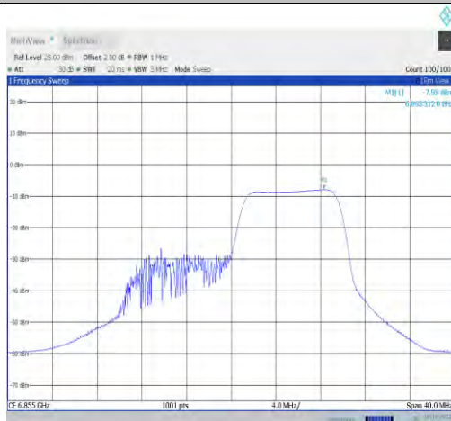
11ax20MIMO-Ant0-6855-PASS
