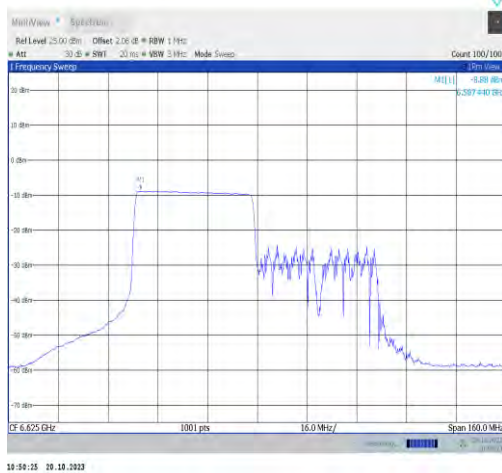
11ax80MIMO-Ant0-6625-PASS
