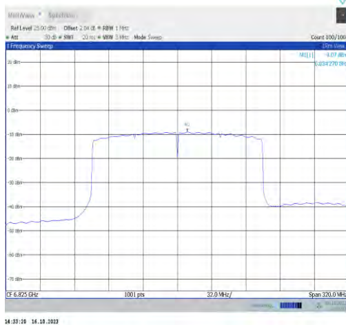
11ax160MIMO-Ant0-6825-PASS
