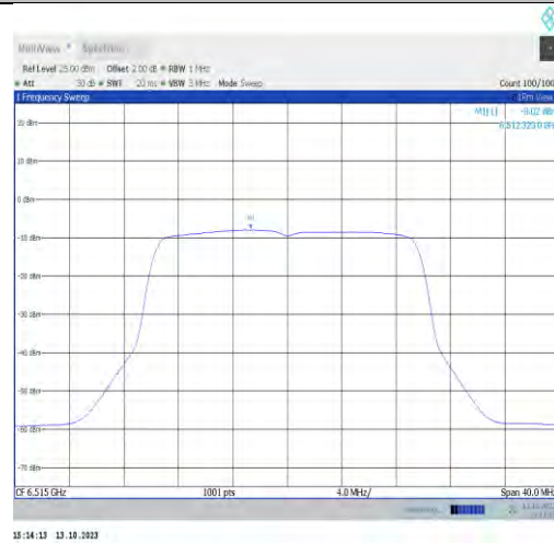
11ax20MIMO-Ant1-6515-PASS
