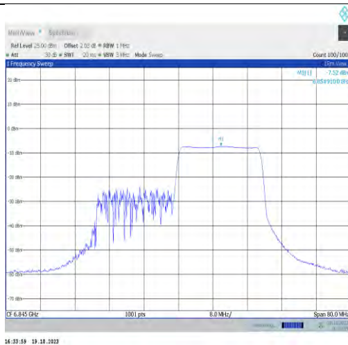
11ax40MIMO-Ant0-6845-PASS
