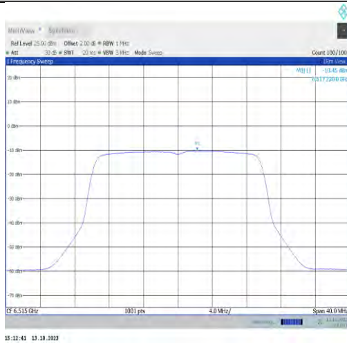
11ax20MIMO-Ant0-6515-PASS
