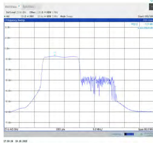
11ax40MIMO-Ant1-6445-PASS
