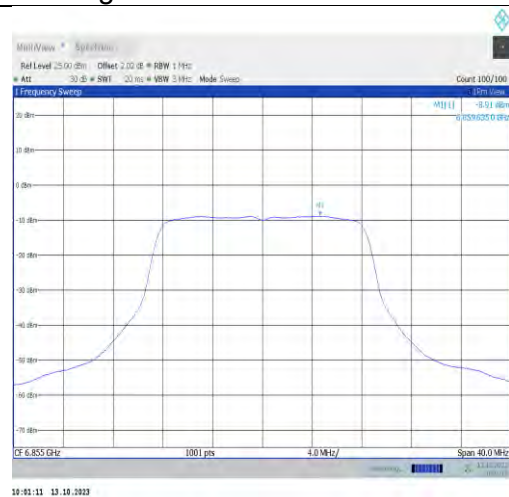
11a-CDD-Ant1-6855-PASS
