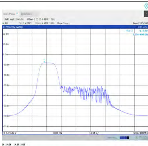
11ax20MIMO-Ant1-6895-PASS
