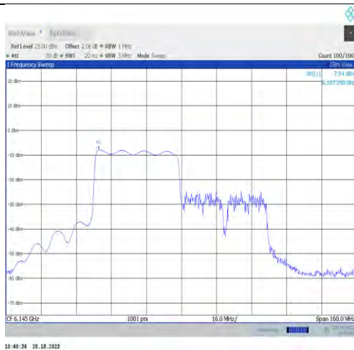
11ax80MIMO-Ant0-6145-PASS
