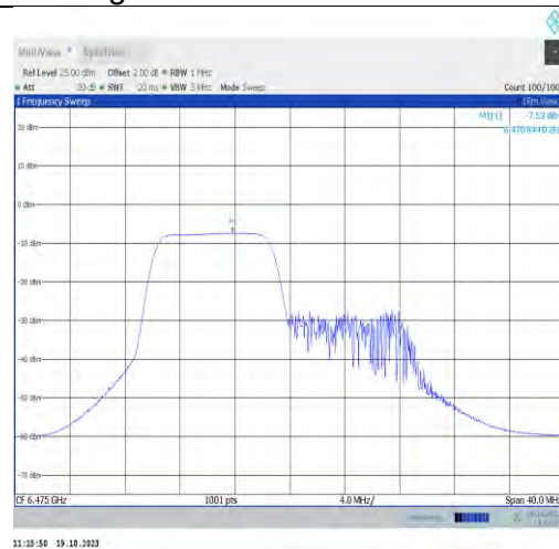
11ax20MIMO-Ant1-6475-PASS
