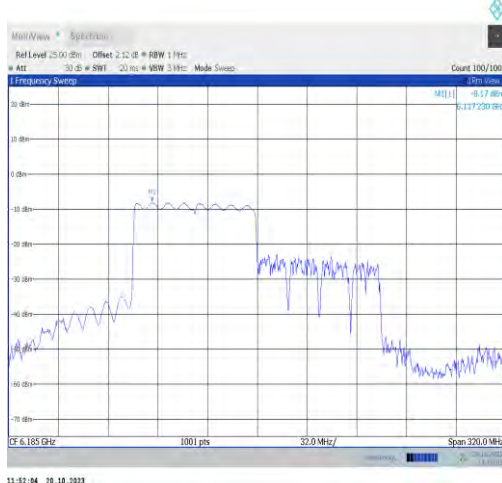
11ax160MIMO-Ant0-6185-PASS
