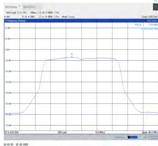
11ax20MIMO-Ant1-6435-PASS
