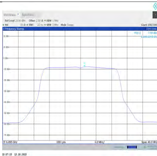
11ax20MIMO-Ant0-6895-PASS
