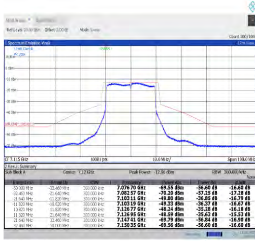
NTNV-11ax20MIMO-Ant0-7115-PASS
