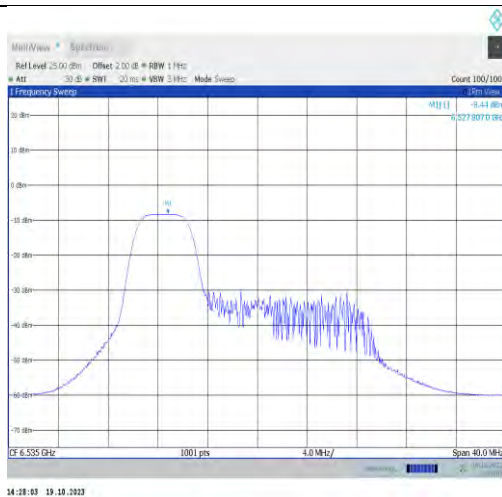
11ax20MIMO-Ant1-6535-PASS
