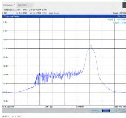
11ax20MIMO-Ant0-6515-PASS
