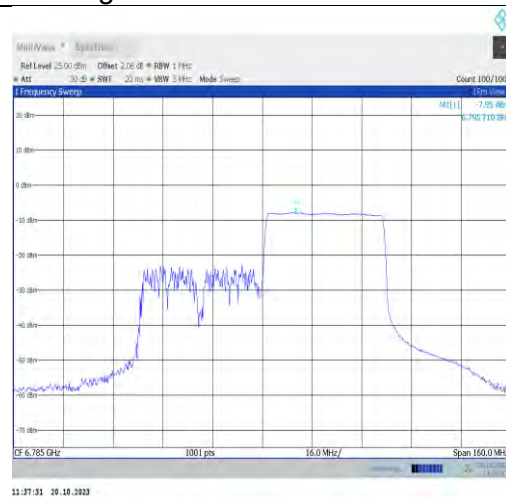
11ax80MIMO-Ant1-6785-PASS
