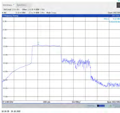
11ax80MIMO-Ant0-5985-PASS
