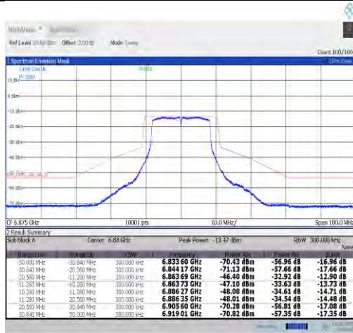
NTNV-11a-CDD-Ant0-6875-PASS
