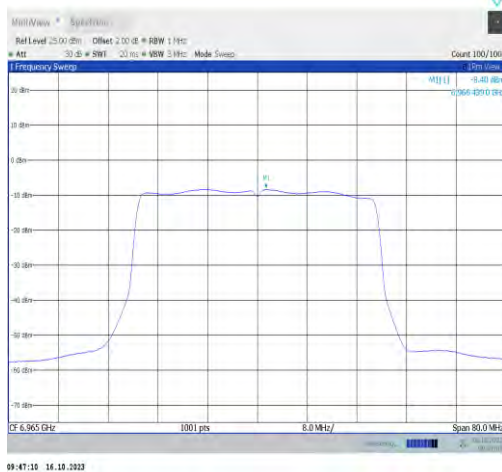
11ax40MIMO-Ant0-6965-PASS
