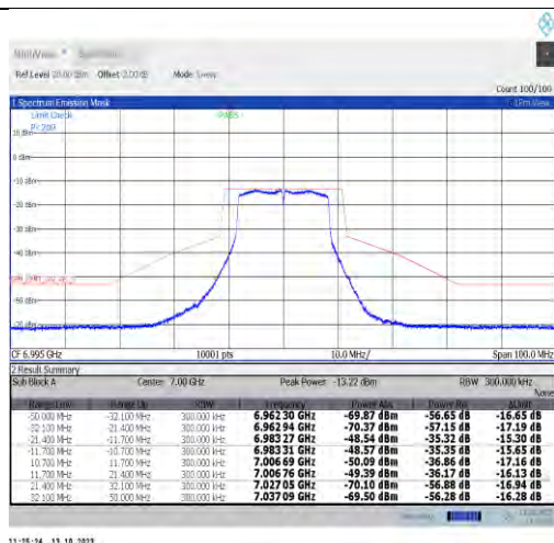
NTNV-11a-CDD-Ant0-6995-PASS
