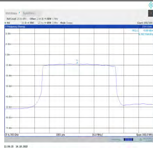
11ax80MIMO-Ant1-6785-PASS
