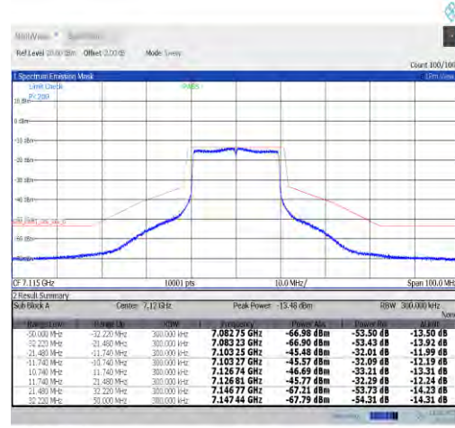
NTNV-11ax20MIMO-Ant1-7115-PASS
