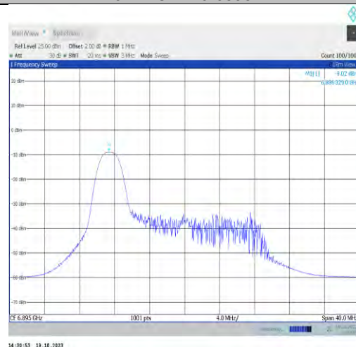
11ax20MIMO-Ant1-6895-PASS
