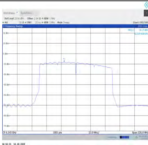
11ax160MIMO-Ant0-6345-PASS
