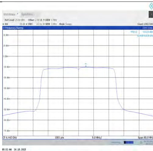
11ax40MIMO-Ant0-6445-PASS
