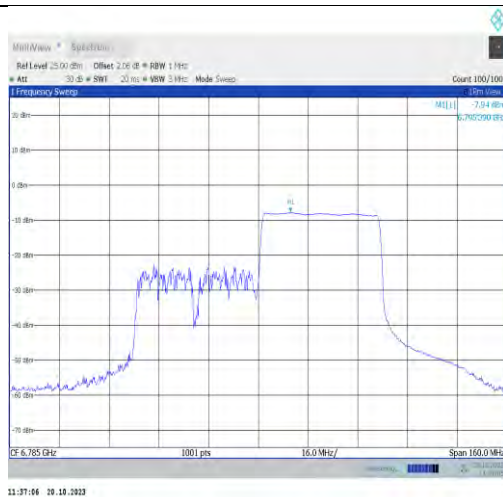
11ax80MIMO-Ant0-6785-PASS
