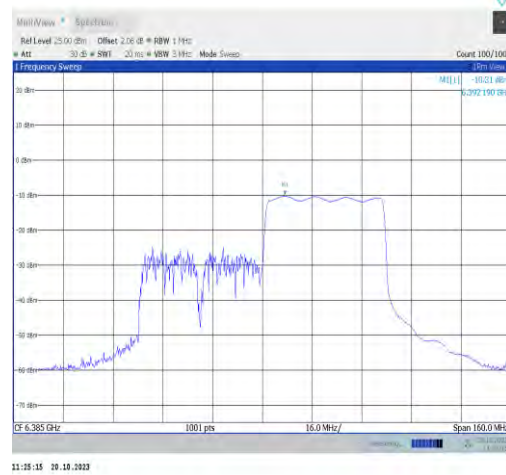
11ax80MIMO-Ant1-6385-PASS
