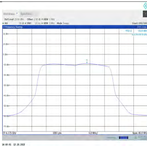
11ax20MIMO-Ant0-6175-PASS
