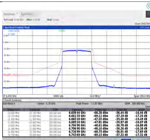
NTNV-11ax20MIMO-Ant0-6695-PASS
