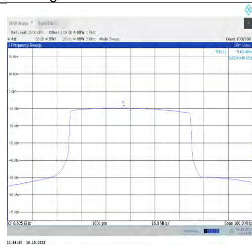
11ax80MIMO-Ant1-6625-PASS
