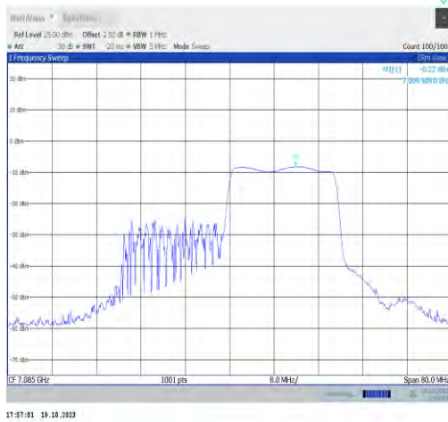
11ax40MIMO-Ant0-7085-PASS
