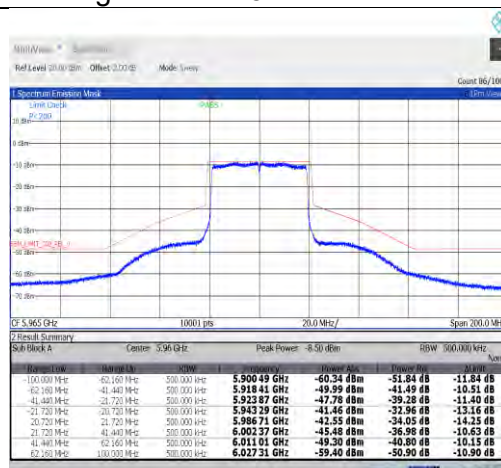
NTNV-11ax40MIMO-Ant1-5965-PASS
