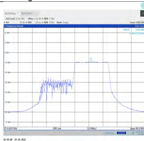
11ax40MIMO-Ant1-6845-PASS
