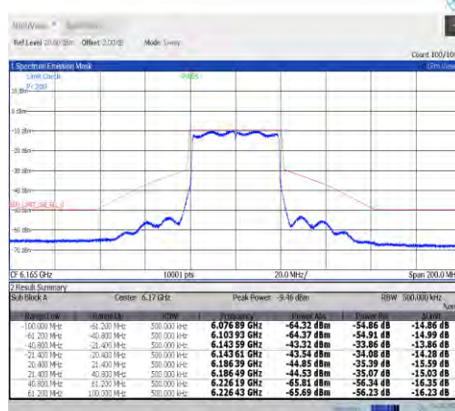
NTNV-11ax40MIMO-Ant1-6165-PASS
