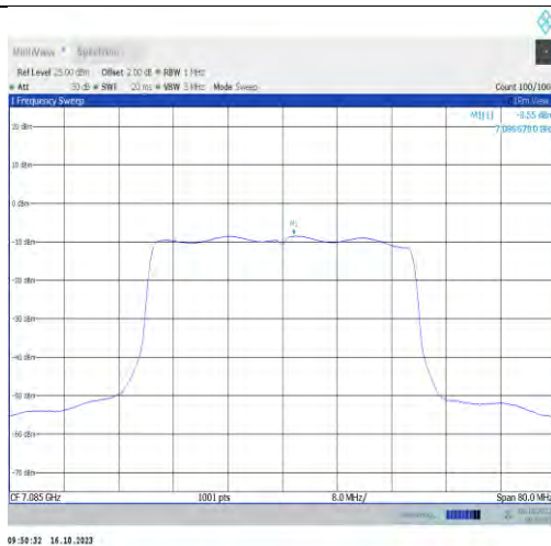
11ax40MIMO-Ant0-7085-PASS
