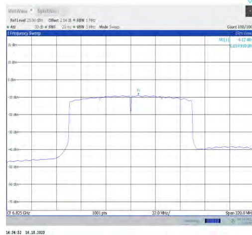
11ax160MIMO-Ant1-6825-PASS
