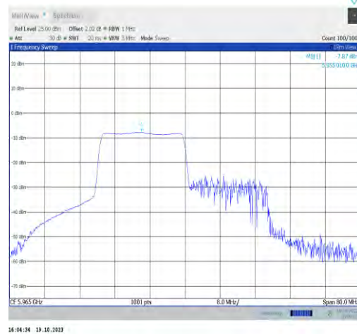
11ax40MIMO-Ant1-5965-PASS
