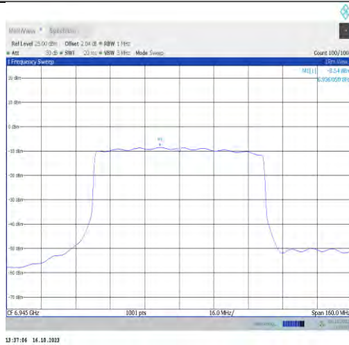
11ax80MIMO-Ant0-6945-PASS
