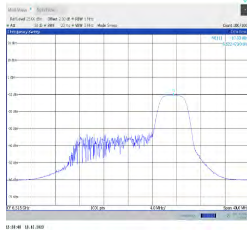
11ax20MIMO-Ant0-6515-PASS
