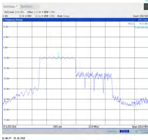
11ax160MIMO-Ant0-6025-PASS
