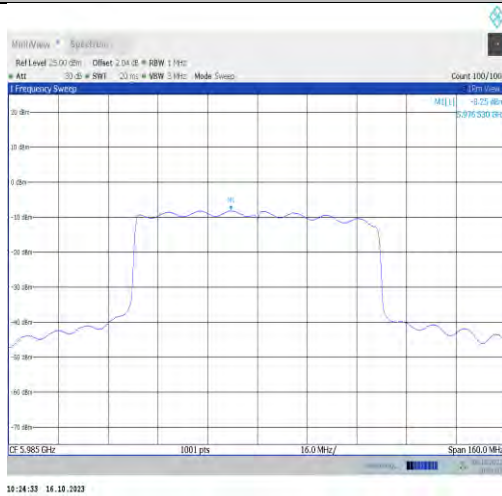
11ax80MIMO-Ant0-5985-PASS
