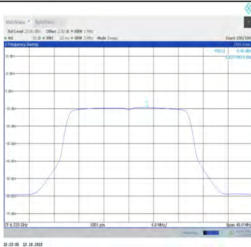
11ax20MIMO-Ant0-6535-PASS
