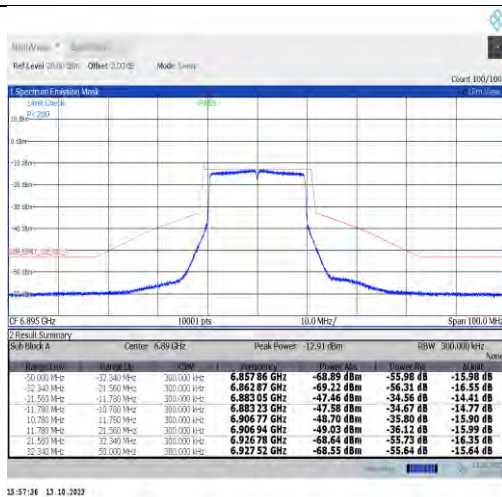
NTNV-11ax20MIMO-Ant0-6895-PASS
