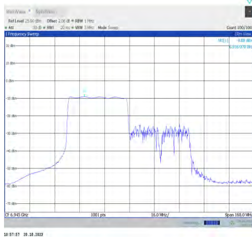
11ax80MIMO-Ant0-6945-PASS
