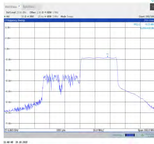
11ax80MIMO-Ant1-6865-PASS
