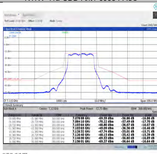
NTNV-11a-CDD-Ant1-7115-PASS
