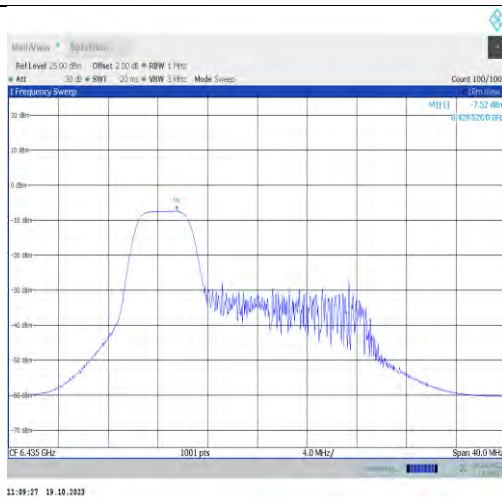
11ax20MIMO-Ant1-6435-PASS
