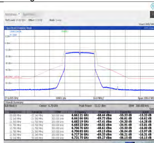
NTNV-11ax20MIMO-Ant1-6695-PASS
