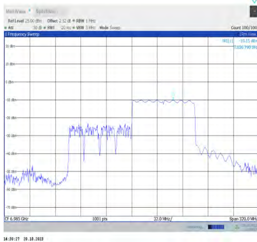
11ax160MIMO-Ant0-6985-PASS
