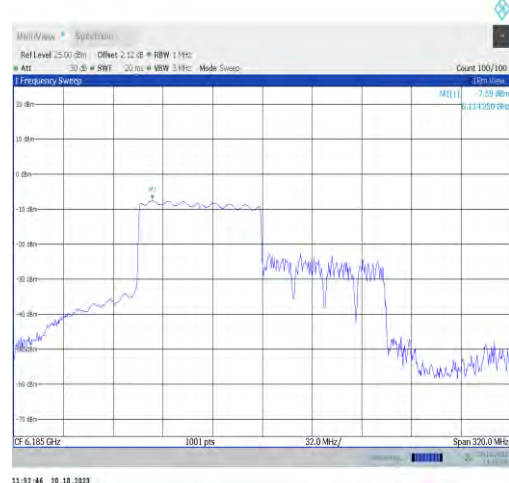
11ax160MIMO-Ant1-6185-PASS
