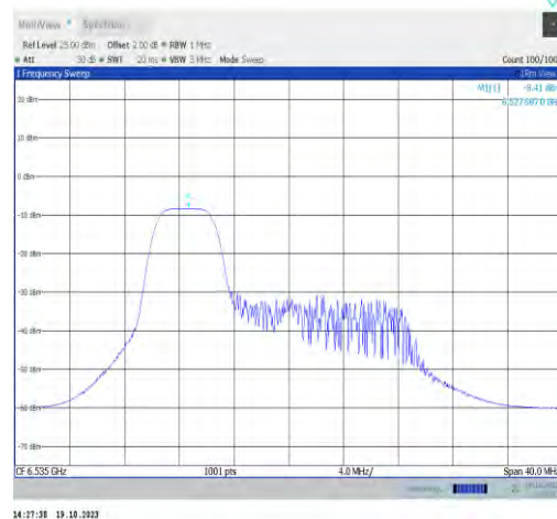
11ax20MIMO-Ant0-6535-PASS
