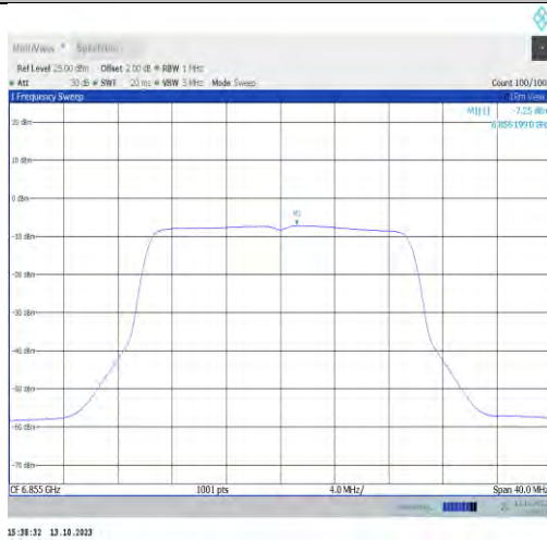
11ax20MIMO-Ant0-6855-PASS
