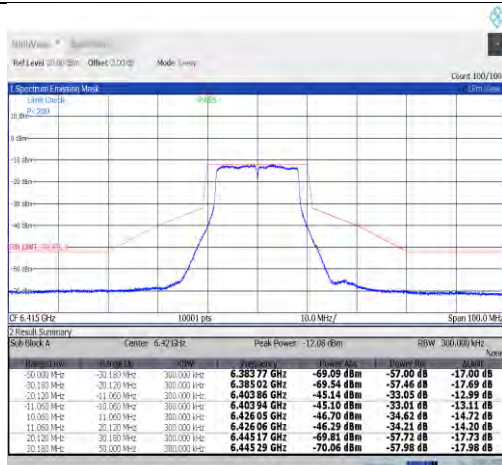
NTNV-11a-CDD-Ant0-6415-PASS
