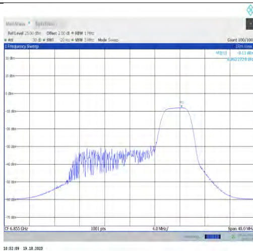
11ax20MIMO-Ant1-6855-PASS
