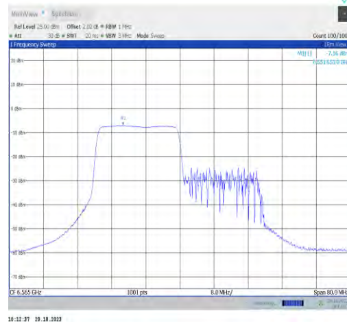
11ax40MIMO-Ant1-6565-PASS
