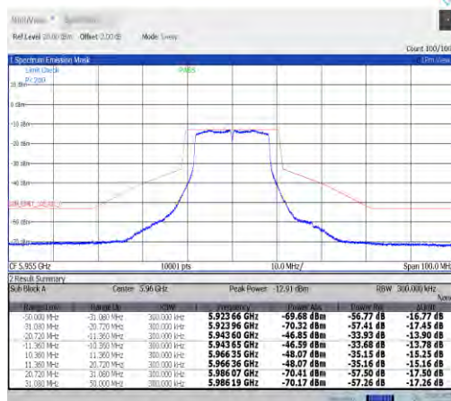
NTNV-11a-CDD-Ant1-5955-PASS
