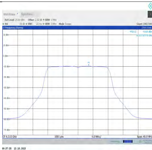
11a-CDD-Ant0-6515-PASS
