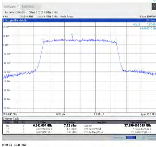
11ax40MIMO-Ant0-6845-PASS
