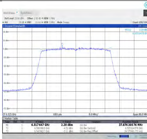
11ax40MIMO-Ant0-6525-PASS
