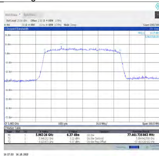
11ax80MIMO-Ant1-5985-PASS
