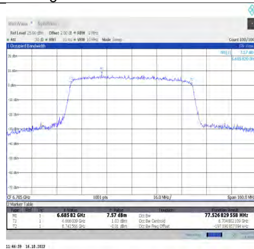
11ax80MIMO-Ant1-6705-PASS
