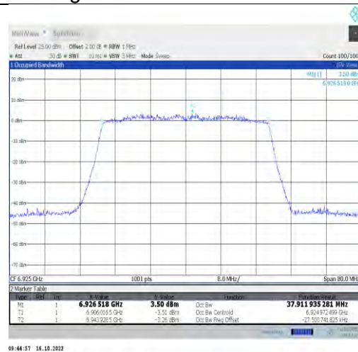
11ax40MIMO-Ant1-6925-PASS
