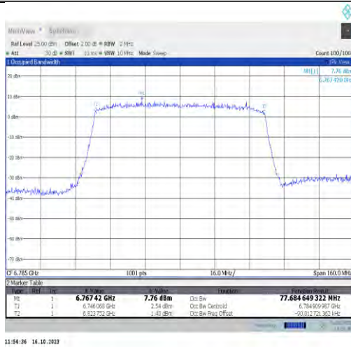
11ax80MIMO-Ant0-6785-PASS
