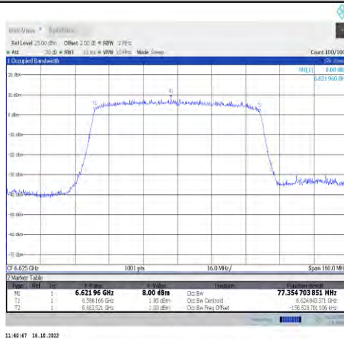
11ax80MIMO-Ant0-6625-PASS
