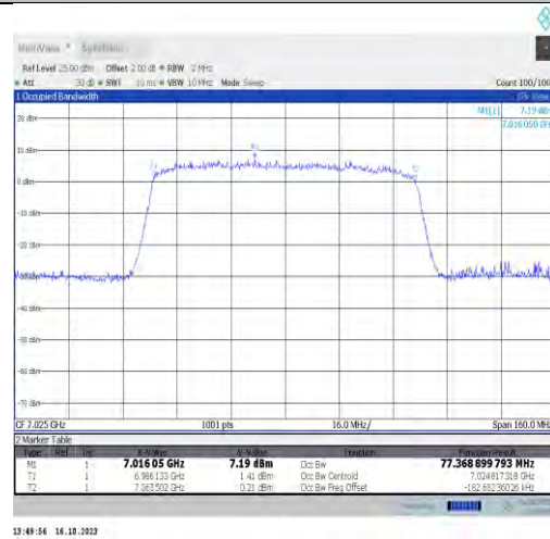
11ax80MIMO-Ant1-7025-PASS
