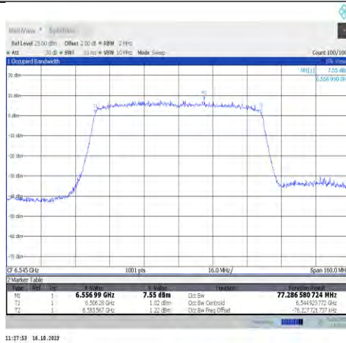
11ax80MIMO-Ant0-6545-PASS
