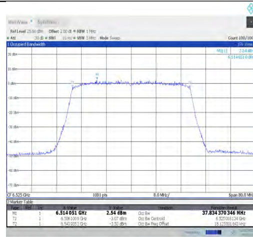
11ax40MIMO-Ant1-6525-PASS
