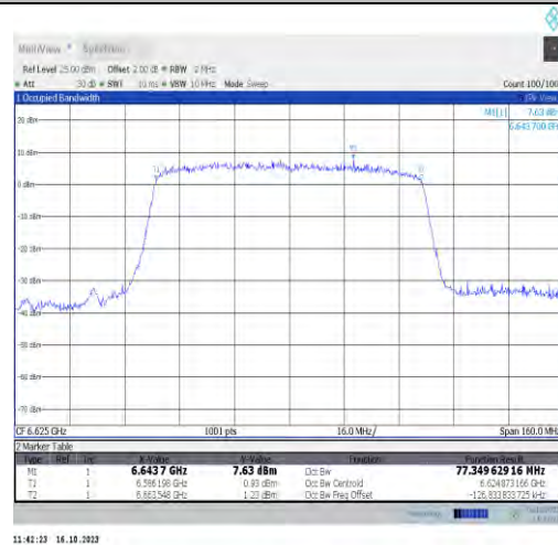
11ax80MIMO-Ant1-6625-PASS
