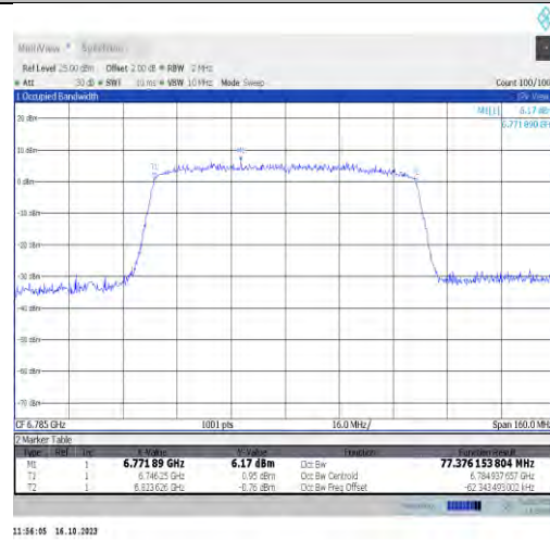
11ax80MIMO-Ant1-6785-PASS
