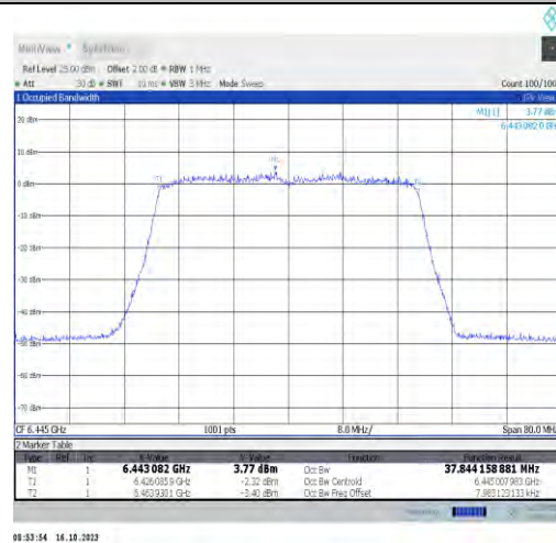
11ax40MIMO-Ant1-6445-PASS
