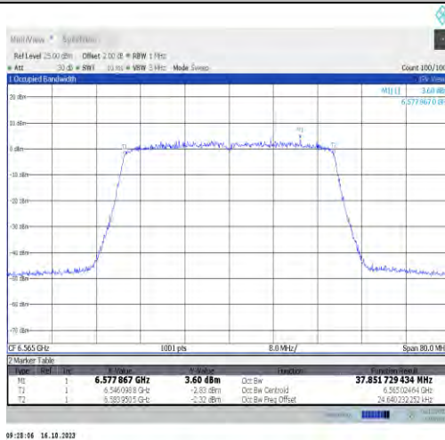
11ax40MIMO-Ant0-6565-PASS
