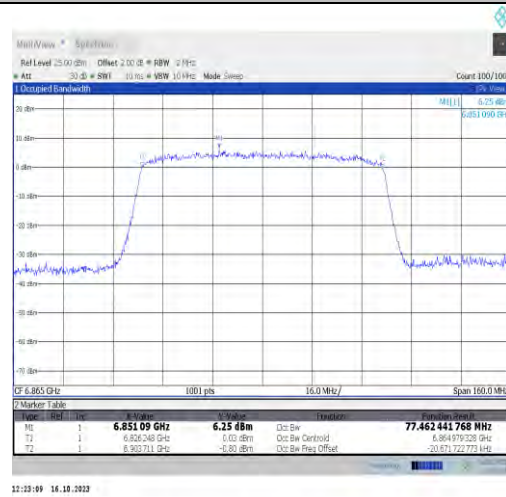
11ax80MIMO-Ant1-6865-PASS
