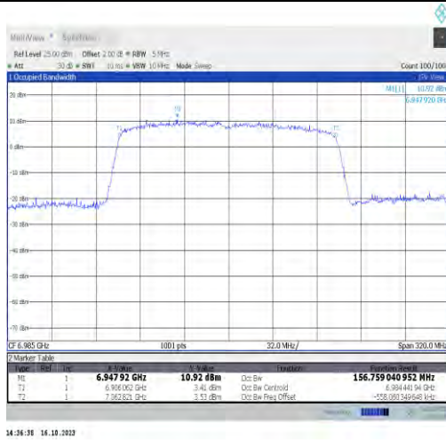
11ax160MIMO-Ant0-6985-PASS
