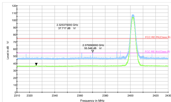
Bluetooth LE (2M) Channel 0 Peak+ Average
