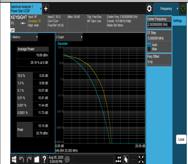
Band41-20MHz-16QAM-39725-54RB#0-PASS
