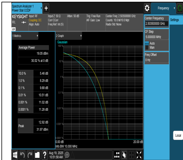
Band41-15MHz-16QAM-39725-54RB#0-PASS
