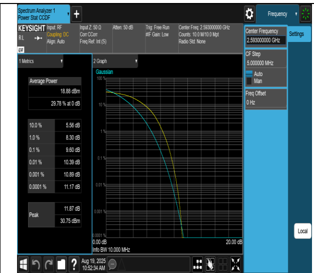
Band41-15MHz-16QAM-40620-54RB#0-PASS
