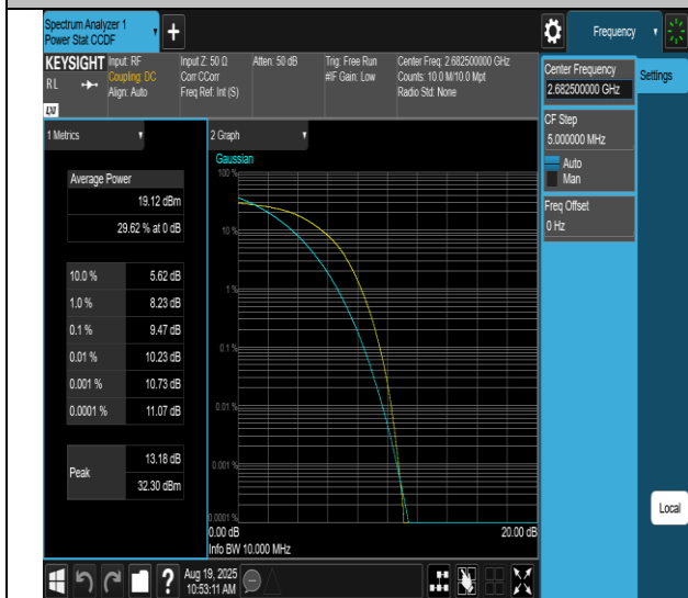
Band41-15MHz-16QAM-41515-54RB#0-PASS
