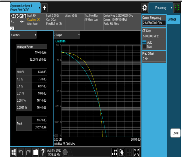
Band41-20MHz-16QAM-41515-54RB#0-PASS
