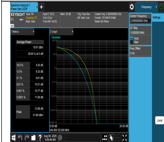
Band41-20MHz-16QAM-40620-54RB#0-PASS
