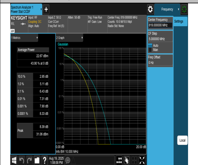
Band26(814-824)-10MHz-16QAM-26740-50RB#0-PASS
