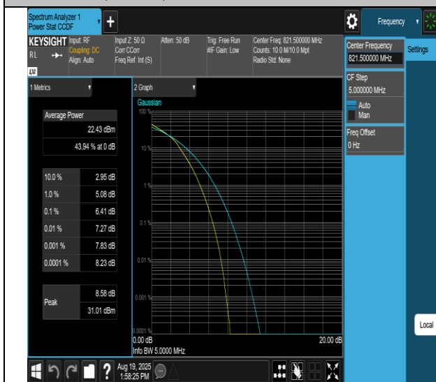
Band26(814-824)-5MHz-16QAM-26765-25RB#0-PASS
