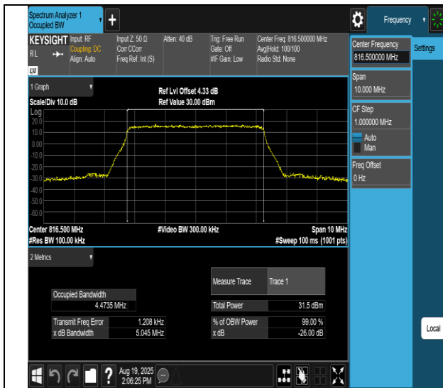
Band26(814-824)-5MHz-16QAM-26715-25RB#0-PASS
