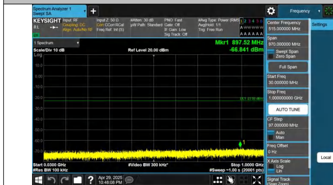
Band66-3MHz-QPSK-132322-1RB#0-30~1000-PASS
