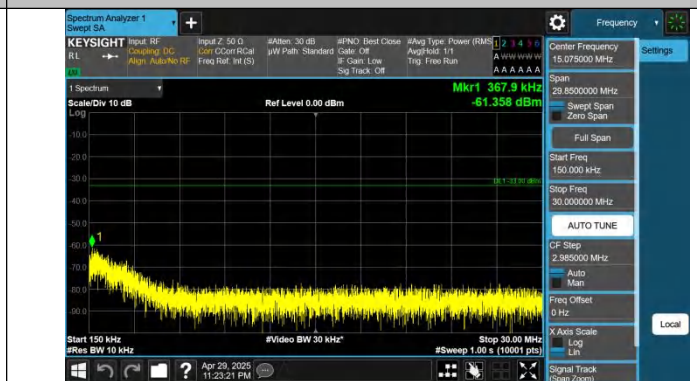
Band66-20MHz-QPSK-132572-1RB#0-0.15~30-PASS
