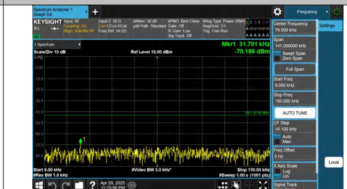
Band66-20MHz-QPSK-132572-1RB#99-0.009~0.15-PASS
