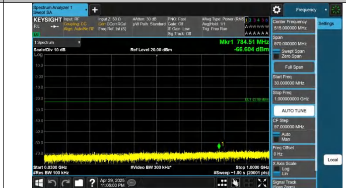
Band66-10MHz-QPSK-132322-1RB#49-30~1000-PASS
