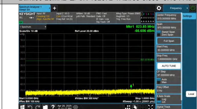
Band66-20MHz-QPSK-132072-1RB#99-30~1000-PASS
