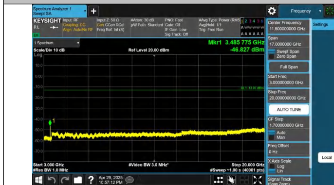
Band66-5MHz-QPSK-132322-1RB#0-3000~20000-PASS
