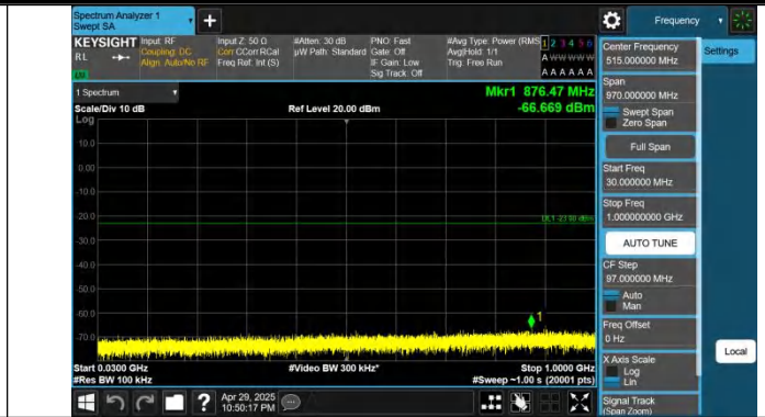
Band66-3MHz-QPSK-132657-1RB#14-30~1000-PASS
