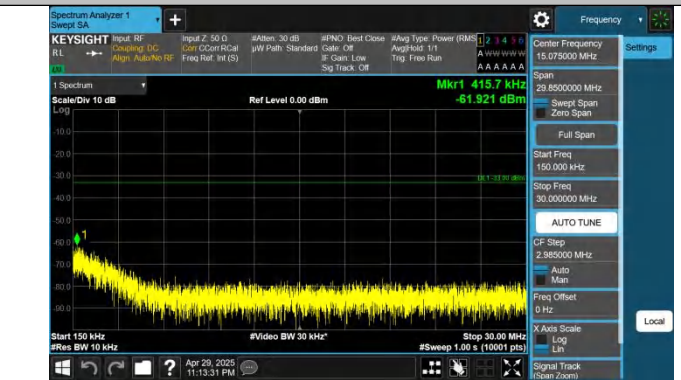
Band66-15MHz-QPSK-132322-1RB#0-0.15~30-PASS
