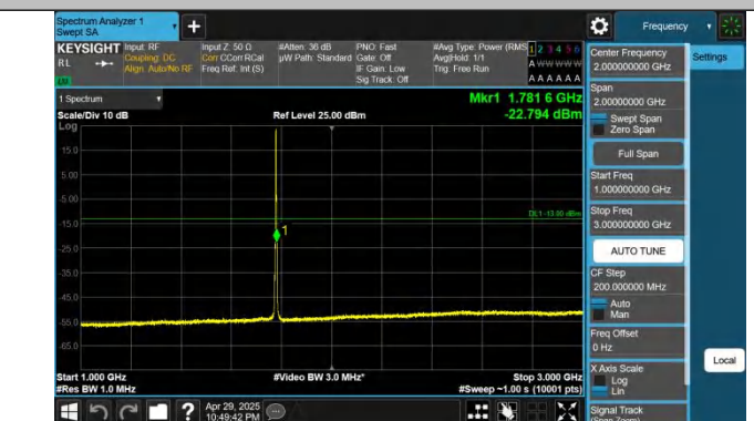
Band66-3MHz-QPSK-132657-1RB#0-1000~3000-PASS
