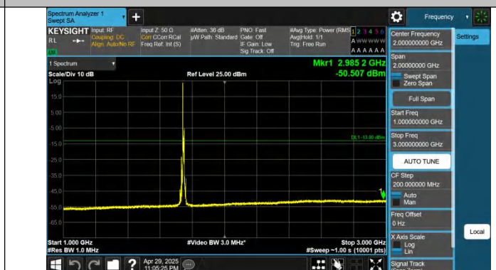
Band66-10MHz-QPSK-132322-1RB#0-1000~3000-PASS
