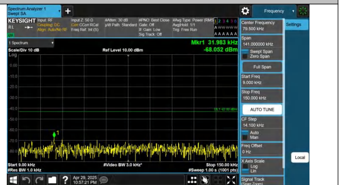
Band66-5MHz-QPSK-132322-1RB#24-0.009~0.15-PASS
