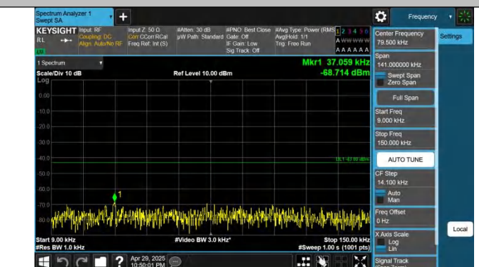
Band66-3MHz-QPSK-132657-1RB#14-0.009~0.15-PASS
