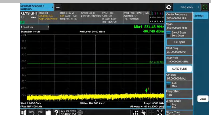
Band66-3MHz-QPSK-132322-1RB#14-30~1000-PASS
