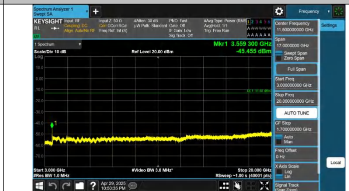
Band66-3MHz-QPSK-132657-1RB#14-3000~20000-PASS
