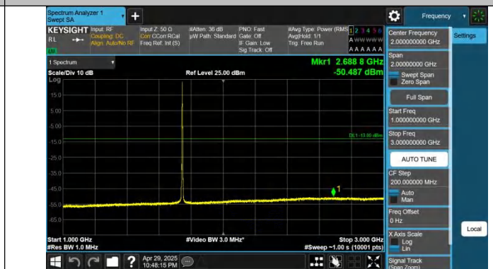
Band66-3MHz-QPSK-132322-1RB#0-1000~3000-PASS
