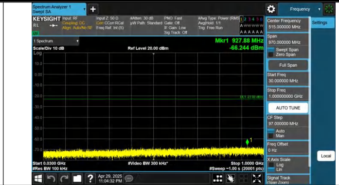
Band66-10MHz-QPSK-132022-1RB#49-30~1000-PASS
