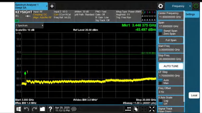
Band66-15MHz-QPSK-132047-1RB#74-3000~20000-PASS
