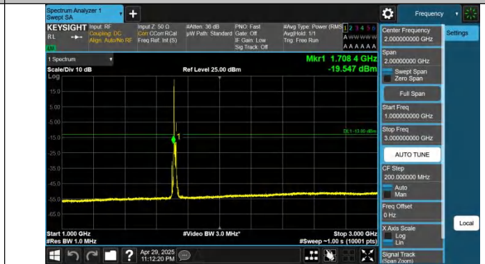
Band66-15MHz-QPSK-132047-1RB#0-1000~3000-PASS
