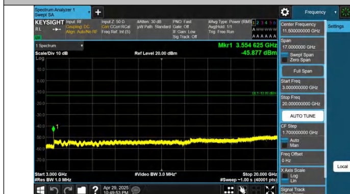
Band66-3MHz-QPSK-132657-1RB#0-3000~20000-PASS
