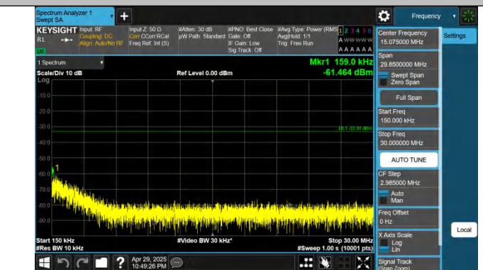
Band66-3MHz-QPSK-132657-1RB#0-0.15~30-PASS
