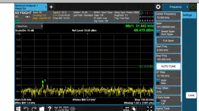
Band66-15MHz-QPSK-132322-1RB#74-0.009~0.15-PASS
