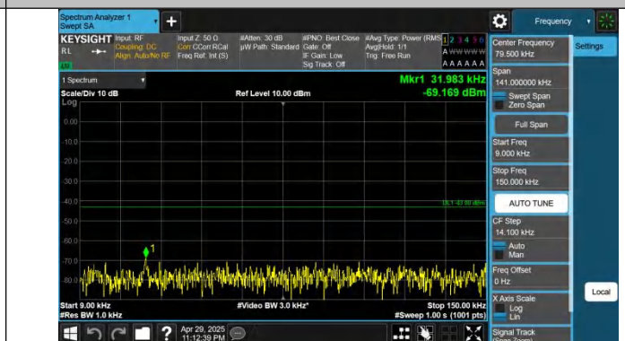
Band66-15MHz-QPSK-132047-1RB#74-0.009~0.15-PASS
