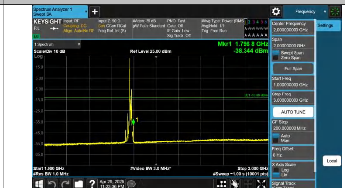
Band66-20MHz-QPSK-132572-1RB#0-1000~3000-PASS
