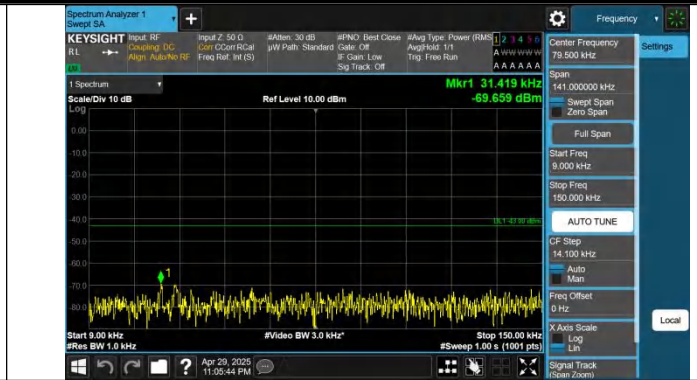
Band66-10MHz-QPSK-132322-1RB#49-0.009~0.15-PASS
