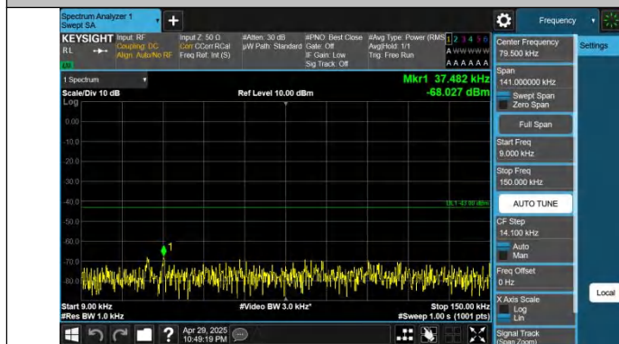
Band66-3MHz-QPSK-132657-1RB#0-0.009~0.15-PASS
