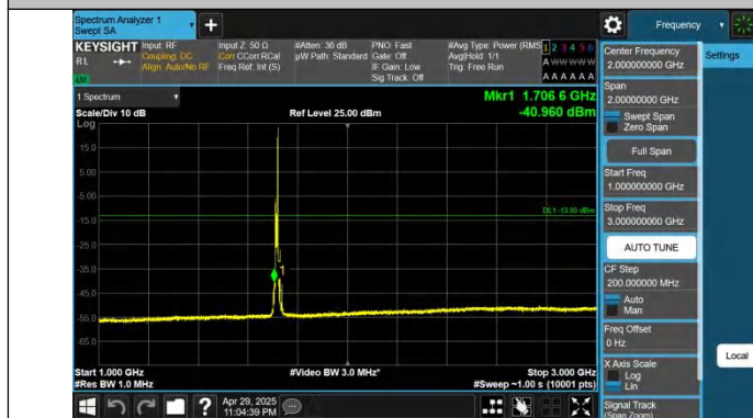
Band66-10MHz-QPSK-132022-1RB#49-1000~3000-PASS
