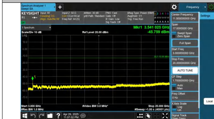
Band66-10MHz-QPSK-132622-1RB#0-3000~20000-PASS
