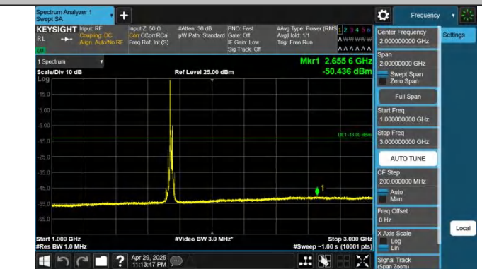
Band66-15MHz-QPSK-132322-1RB#0-1000~3000-PASS
