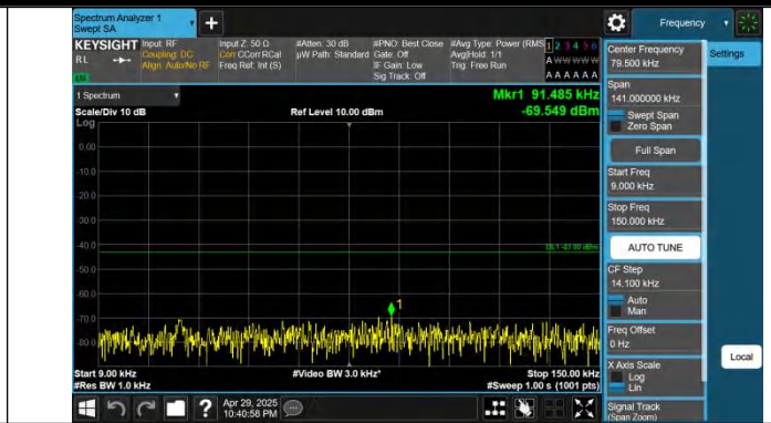
Band66-1.4MHz-QPSK-132665-1RB#5-0.009~0.15-PASS
