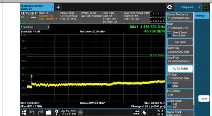
Band66-1.4MHz-QPSK-132665-1RB#5-3000~20000-PASS
