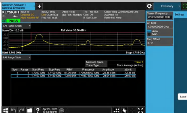
Band66-5MHz-QPSK-131997-1RB#0-PASS
