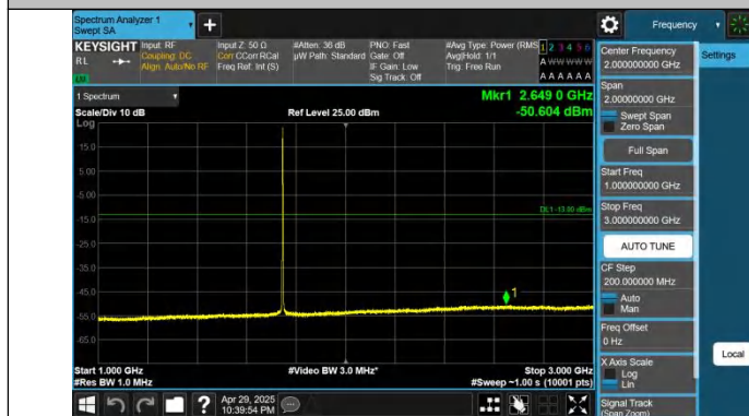
Band66-1.4MHz-QPSK-132322-1RB#5-1000~3000-PASS
