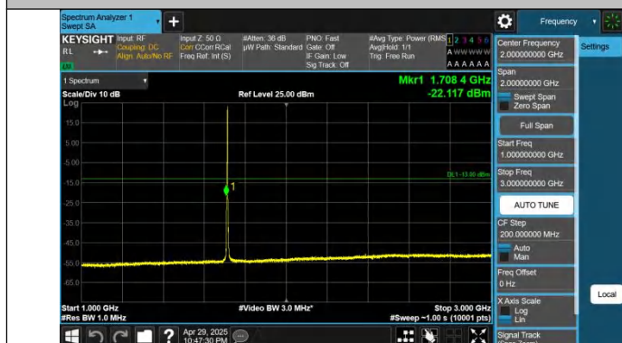
Band66-3MHz-QPSK-131987-1RB#14-1000~3000-PASS
