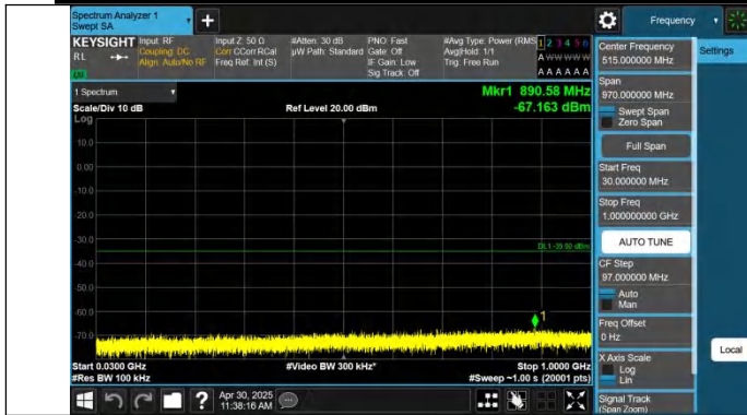
Band41-15MHz-QPSK-40620-1RB#0-30~1000-PASS
