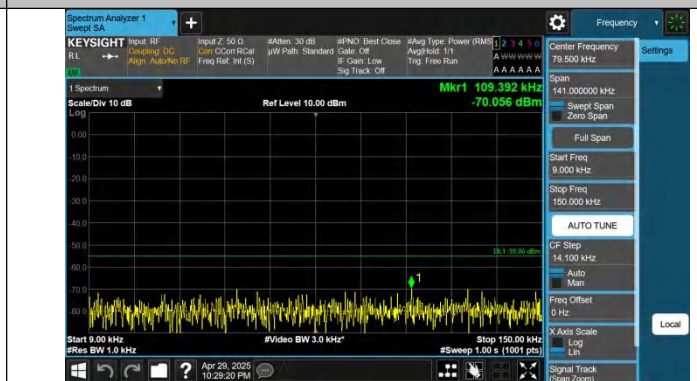
Band41-20MHz-QPSK-41490-1RB#99-0.009~0.15-PASS
