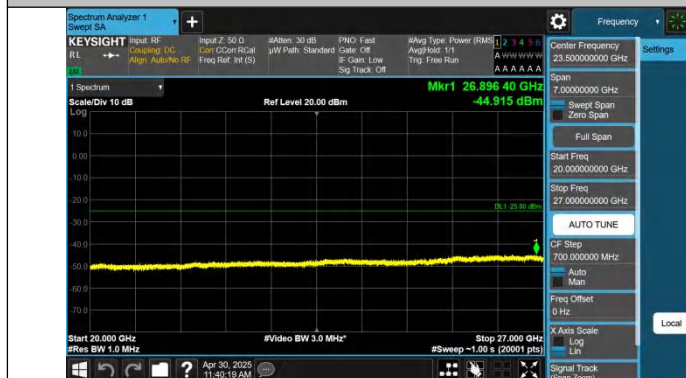
Band41-15MHz-QPSK-41515-1RB#0-20000~27000-PASS
