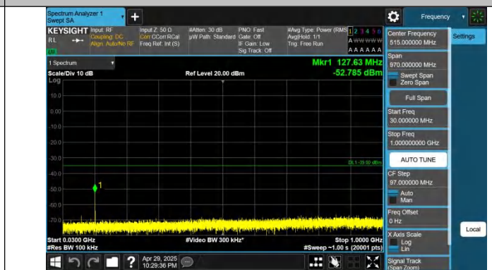
Band41-20MHz-QPSK-41490-1RB#99-30~1000-PASS
