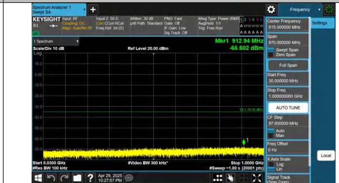
Band41-20MHz-QPSK-40620-1RB#99-30~1000-PASS
