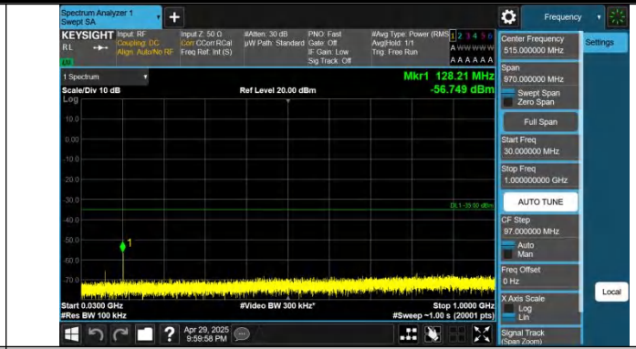
Band41-10MHz-QPSK-41540-1RB#49-30~1000-PASS
