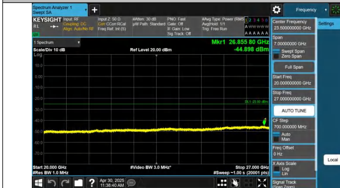
Band41-15MHz-QPSK-40620-1RB#0-20000~27000-PASS
