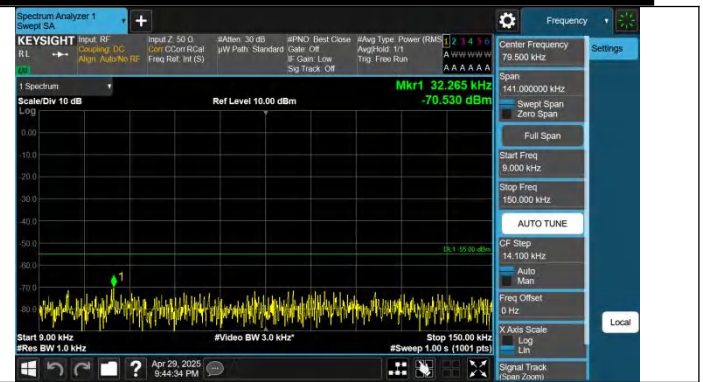
Band41-5MHz-QPSK-41565-1RB#24-0.009~0.15-PASS
