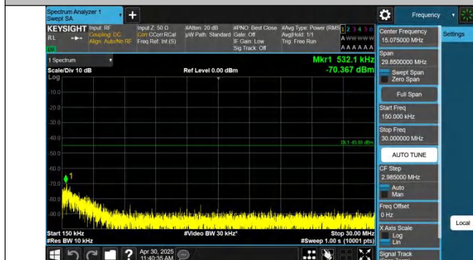
Band41-15MHz-QPSK-41515-1RB#74-0.15~30-PASS
