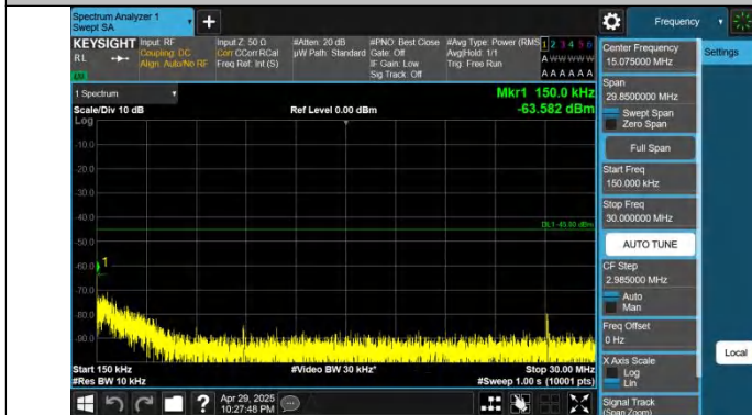
Band41-20MHz-QPSK-40620-1RB#99-0.15~30-PASS
