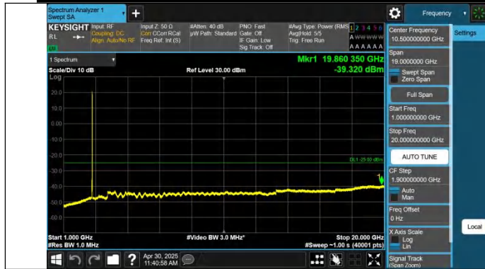
Band41-15MHz-QPSK-41515-1RB#74-1000~20000-PASS
