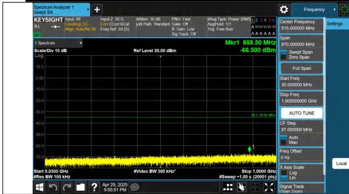
Band41-10MHz-QPSK-39700-1RB#0-30~1000-PASS
