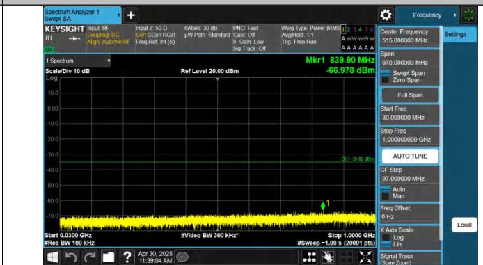
Band41-15MHz-QPSK-40620-1RB#74-30~1000-PASS
