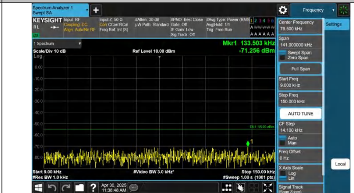
Band41-15MHz-QPSK-40620-1RB#74-0.009~0.15-PASS
