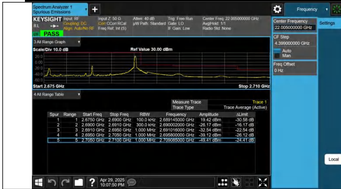
Band41-15MHz-QPSK-41515-1RB#74-PASS
