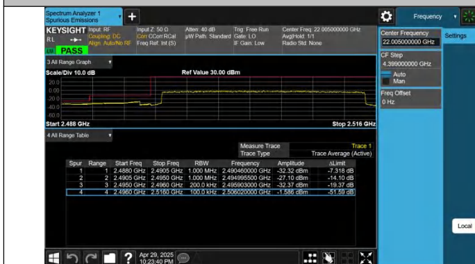
Band41-20MHz-QPSK-39750-100RB#0-PASS
