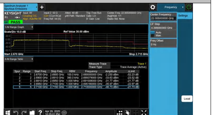
Band41-20MHz-QPSK-41490-100RB#0-PASS
