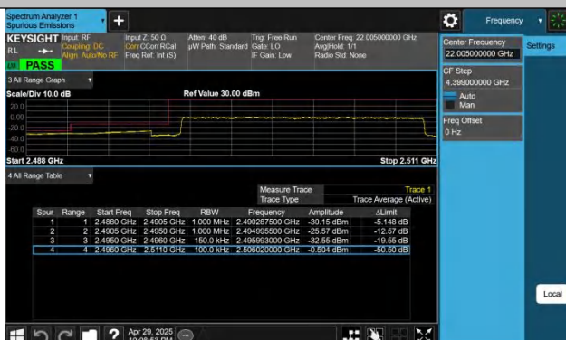
Band41-15MHz-QPSK-39725-75RB#0-PASS
