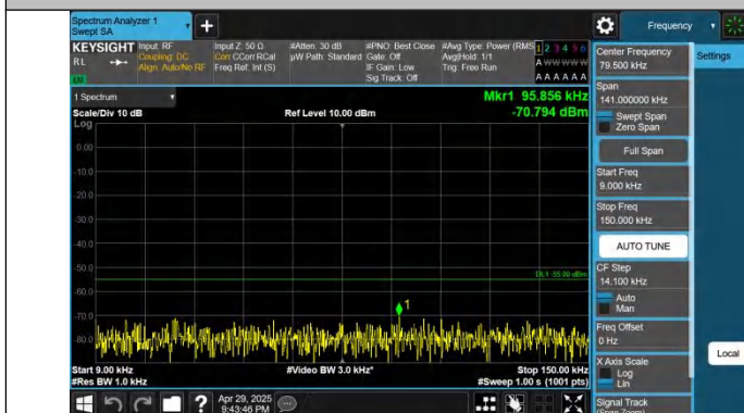
Band41-5MHz-QPSK-41565-1RB#0-0.009~0.15-PASS
