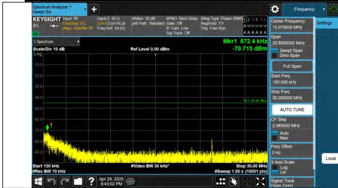
Band41-5MHz-QPSK-40620-1RB#24-0.15~30-PASS
