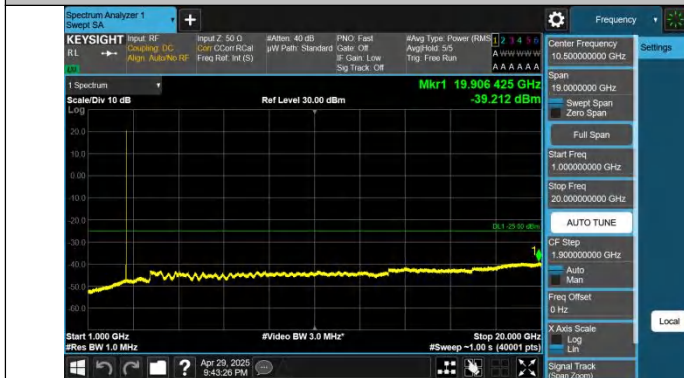
Band41-5MHz-QPSK-40620-1RB#24-1000~20000-PASS
