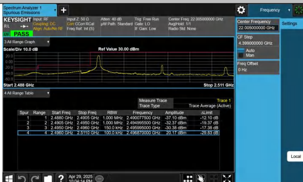
Band41-15MHz-QPSK-39725-1RB#0-PASS
