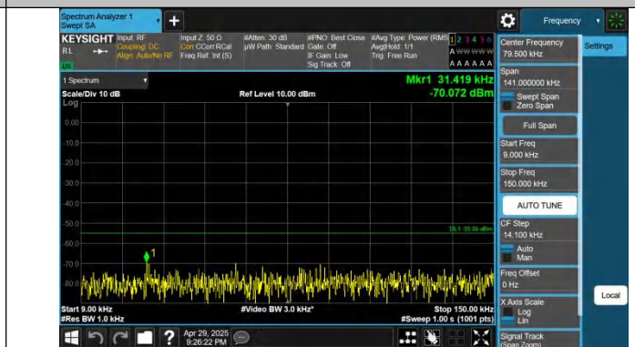
Band38-20MHz-QPSK-38150-1RB#99-0.009~0.15-PASS
