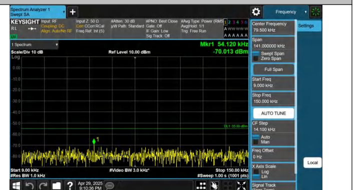
Band38-15MHz-QPSK-38175-1RB#74-0.009~0.15-PASS
