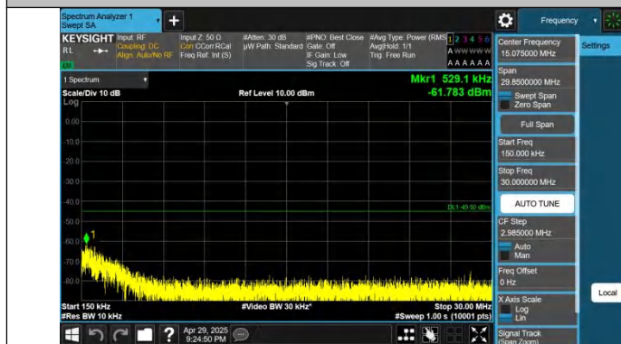
Band38-20MHz-QPSK-38000-1RB#99-0.15~30-PASS
