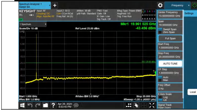
Band38-10MHz-QPSK-38000-1RB#49-1000~20000-PASS
