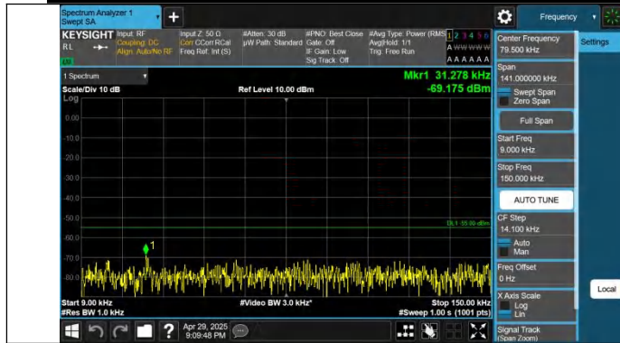
Band38-15MHz-QPSK-38175-1RB#0-0.009~0.15-PASS
