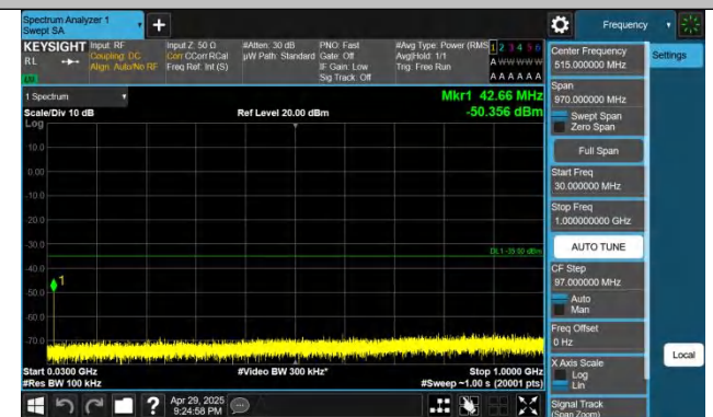
Band38-20MHz-QPSK-38000-1RB#99-30~1000-PASS
