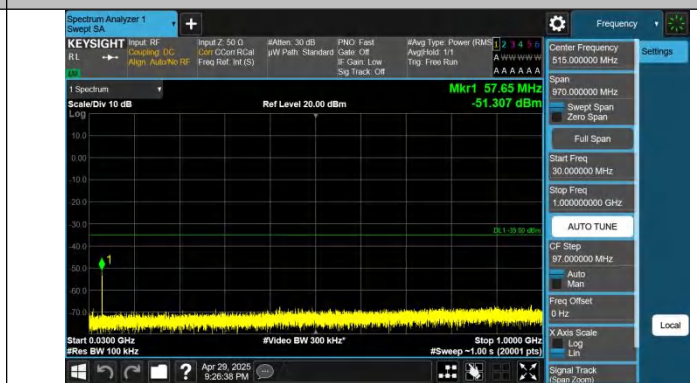
Band38-20MHz-QPSK-38150-1RB#99-30~1000-PASS
