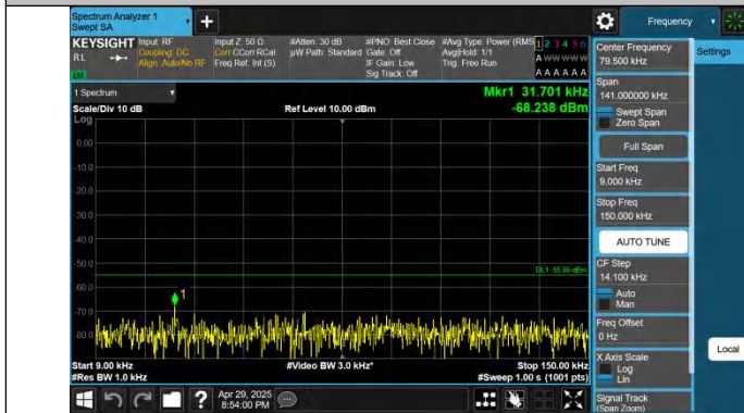
Band38-10MHz-QPSK-38200-1RB#0-0.009~0.15-PASS
