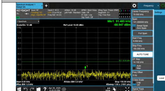
Band38-20MHz-QPSK-38150-1RB#0-0.009~0.15-PASS
