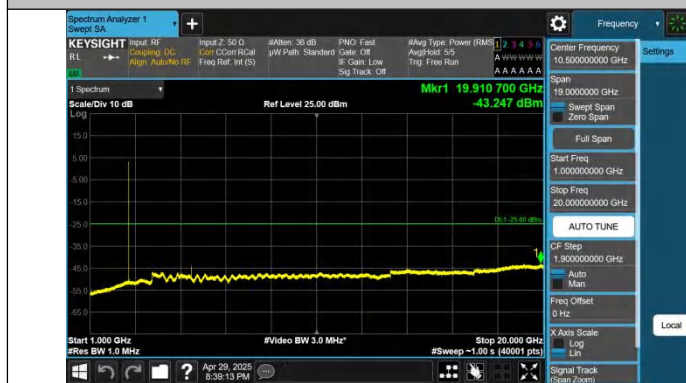
Band38-5MHz-QPSK-38225-1RB#24-1000~20000-PASS
