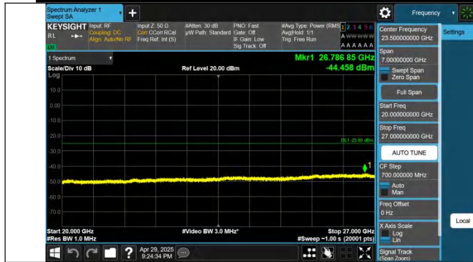
Band38-20MHz-QPSK-38000-1RB#0-20000~27000-PASS
