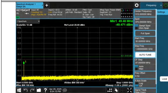
Band38-10MHz-QPSK-38200-1RB#0-30~1000-PASS
