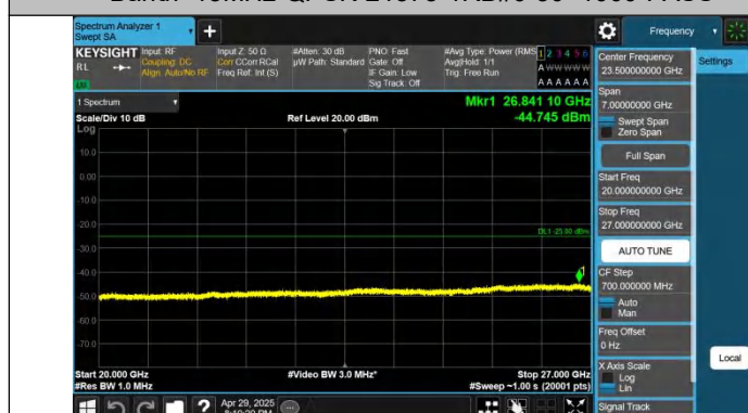
Band7-15MHz-QPSK-21375-1RB#0-20000~27000-PASS
