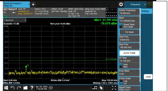
Band7-5MHz-QPSK-21425-1RB#24-0.009~0.15-PASS
