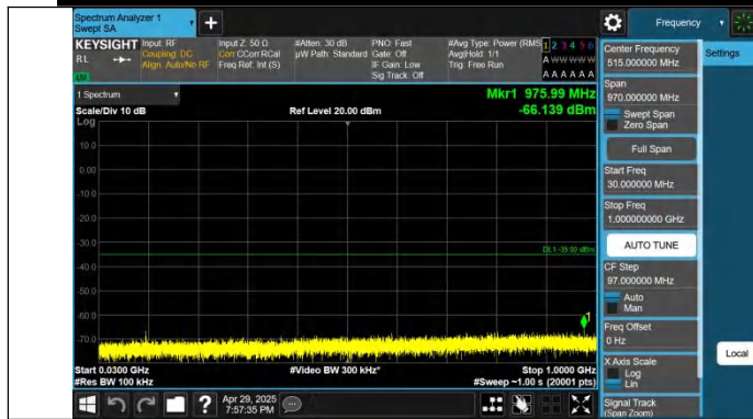
Band7-10MHz-QPSK-20800-1RB#0-30~1000-PASS
