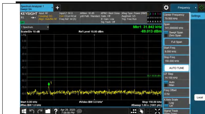
Band7-10MHz-QPSK-21100-1RB#0-0.009~0.15-PASS
