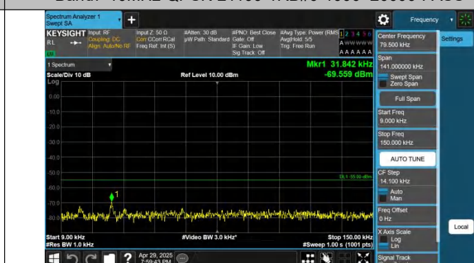
Band7-10MHz-QPSK-21100-1RB#49-0.009~0.15-PASS
