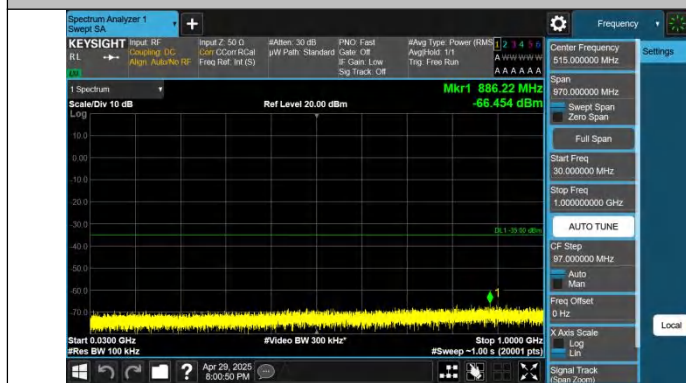
Band7-10MHz-QPSK-21400-1RB#0-30~1000-PASS
