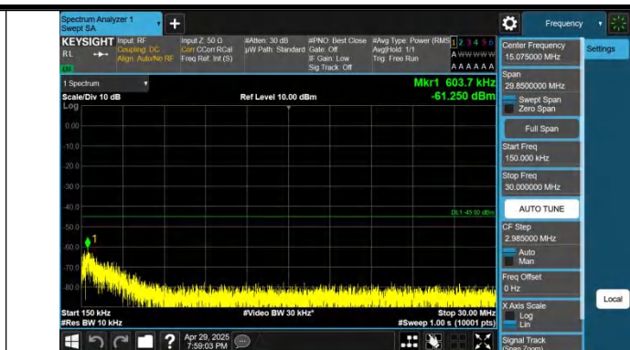
Band7-10MHz-QPSK-21100-1RB#0-0.15~30-PASS
