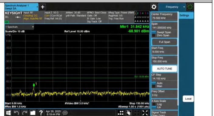
Band7-20MHz-QPSK-21350-1RB#99-0.009~0.15-PASS
