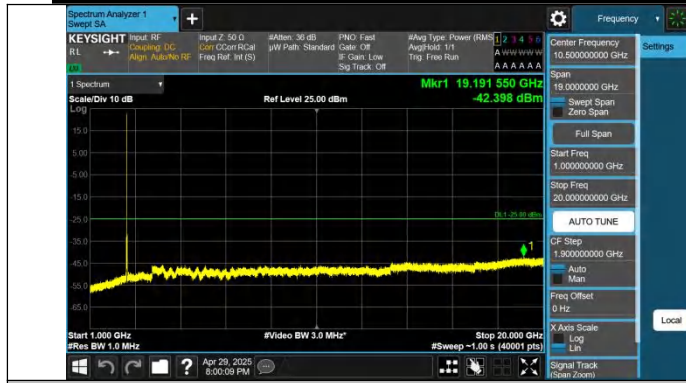
Band7-10MHz-QPSK-21100-1RB#49-1000~20000-PASS
