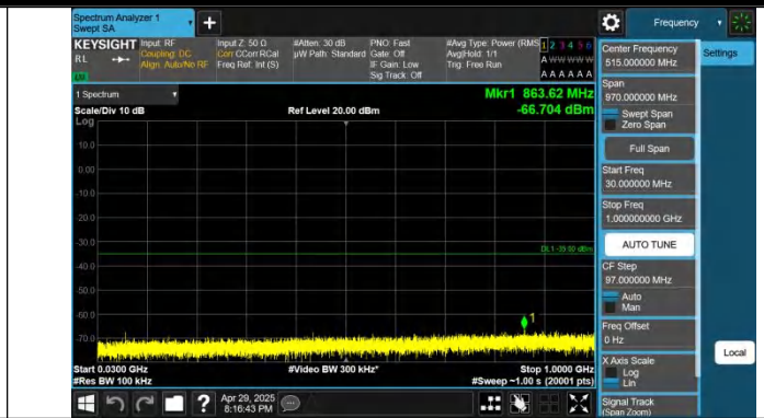
Band7-20MHz-QPSK-20850-1RB#99-30~1000-PASS
