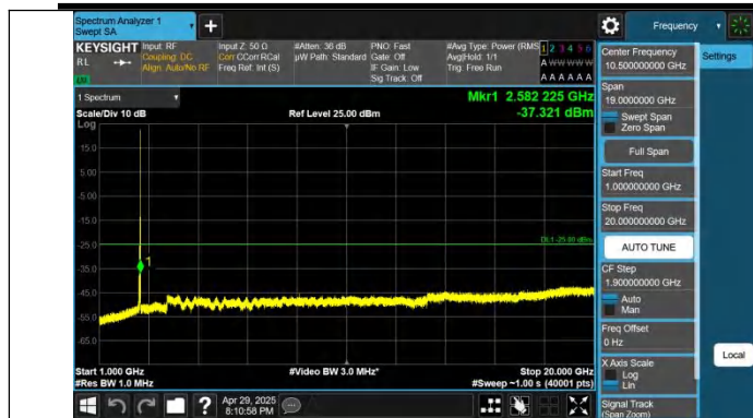
Band7-15MHz-QPSK-21375-1RB#74-1000~20000-PASS
