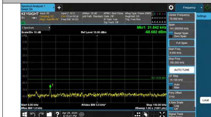
Band7-20MHz-QPSK-20850-1RB#0-0.009~0.15-PASS
