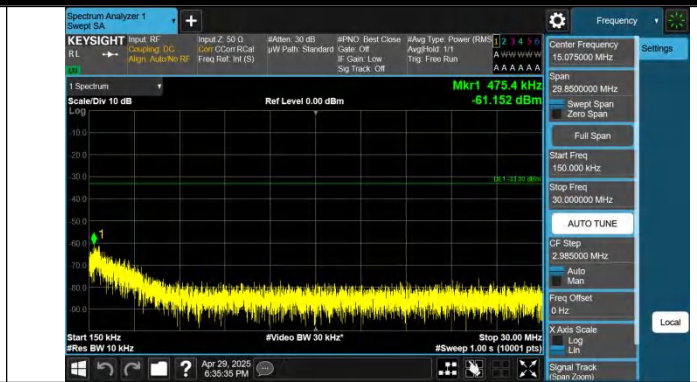
Band4-5MHz-QPSK-20375-1RB#0-0.15~30-PASS
