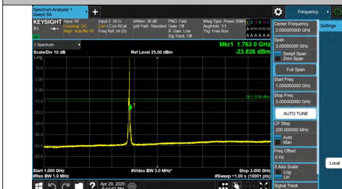
Band4-10MHz-QPSK-20350-1RB#49-1000~3000-PASS
