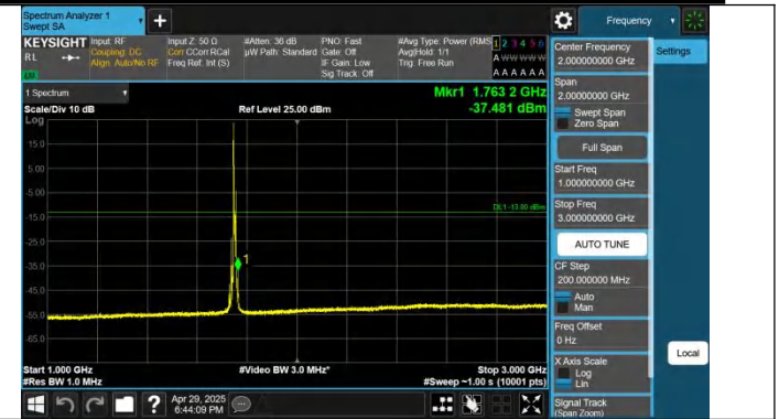
Band4-10MHz-QPSK-20350-1RB#0-1000~3000-PASS
