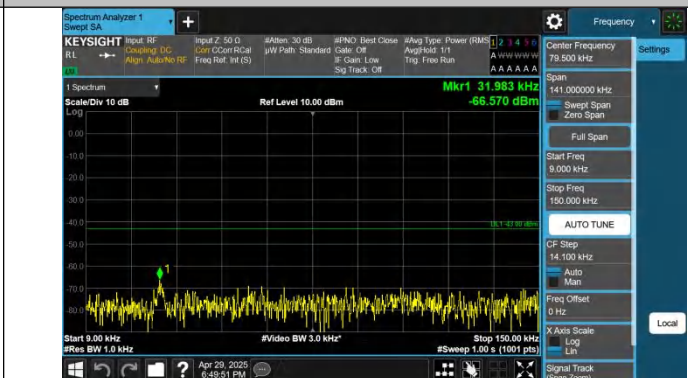
Band4-15MHz-QPSK-20025-1RB#74-0.009~0.15-PASS
