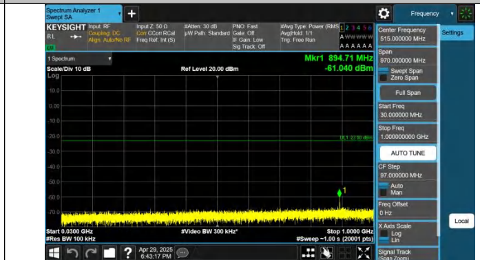
Band4-10MHz-QPSK-20175-1RB#49-30~1000-PASS
