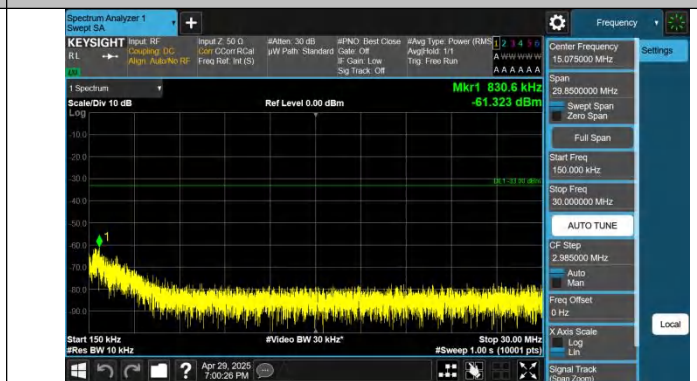
Band4-20MHz-QPSK-20300-1RB#0-0.15~30-PASS
