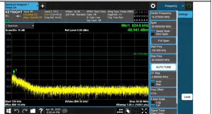
Band4-15MHz-QPSK-20175-1RB#0-0.15~30-PASS
