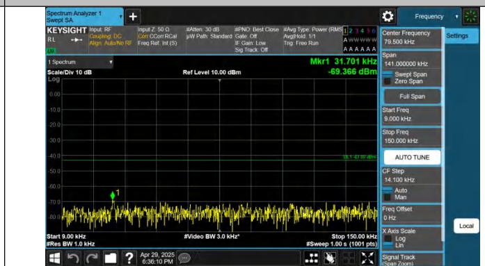
Band4-5MHz-QPSK-20375-1RB#24-0.009~0.15-PASS
