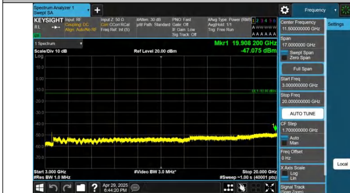
Band4-10MHz-QPSK-20350-1RB#0-3000~20000-PASS
