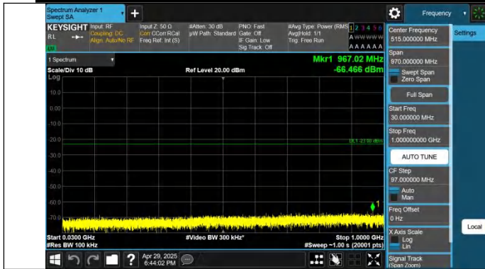
Band4-10MHz-QPSK-20350-1RB#0-30~1000-PASS
