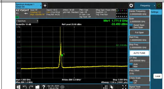
Band4-20MHz-QPSK-20300-1RB#0-1000~3000-PASS
