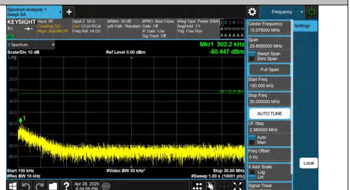
Band4-5MHz-QPSK-20175-1RB#0-0.15~30-PASS
