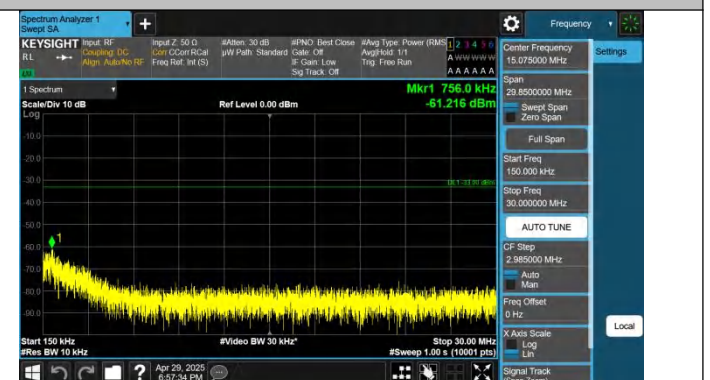
Band4-20MHz-QPSK-20050-1RB#0-0.15~30-PASS
