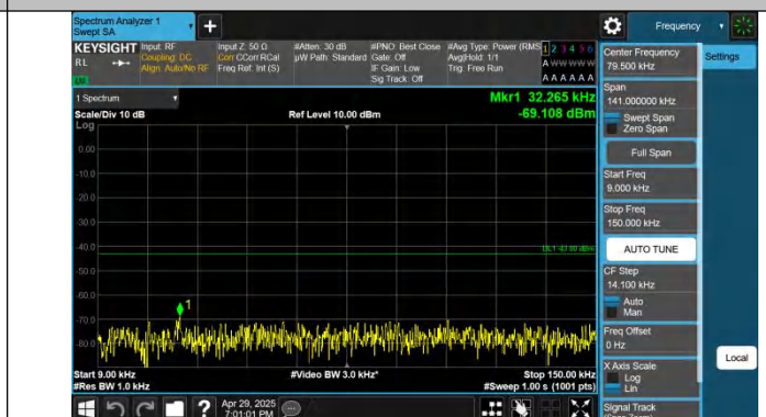
Band4-20MHz-QPSK-20300-1RB#99-0.009~0.15-PASS
