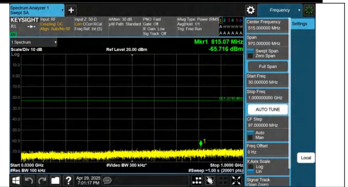
Band4-20MHz-QPSK-20300-1RB#99-30~1000-PASS
