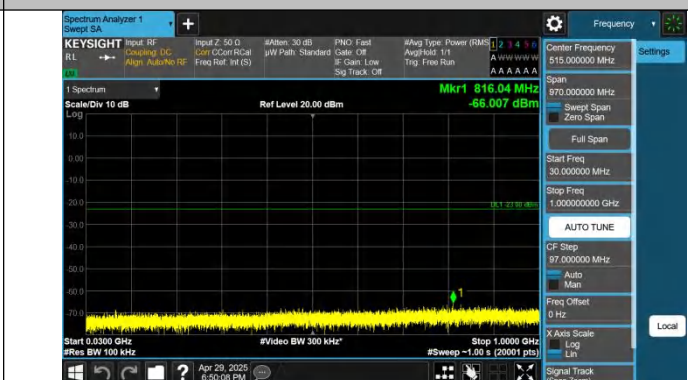
Band4-15MHz-QPSK-20025-1RB#74-30~1000-PASS
