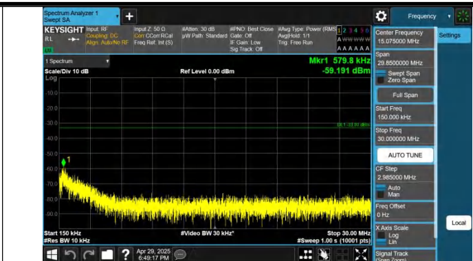
Band4-15MHz-QPSK-20025-1RB#0-0.15~30-PASS
