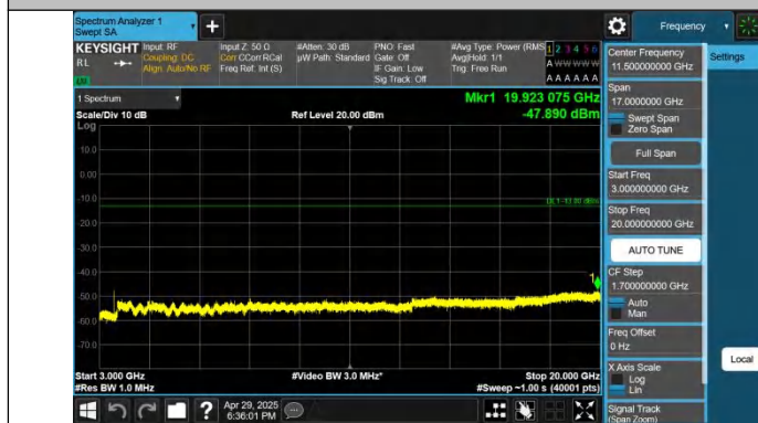
Band4-5MHz-QPSK-20375-1RB#0-3000~20000-PASS
