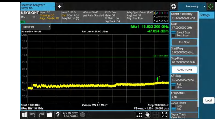
Band4-20MHz-QPSK-20175-1RB#99-3000~20000-PASS
