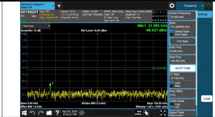
Band4-10MHz-QPSK-20175-1RB#49-0.009~0.15-PASS
