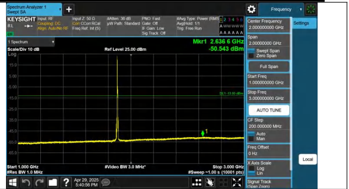
Band2-5MHz-QPSK-18900-1RB#0-1000~3000-PASS
