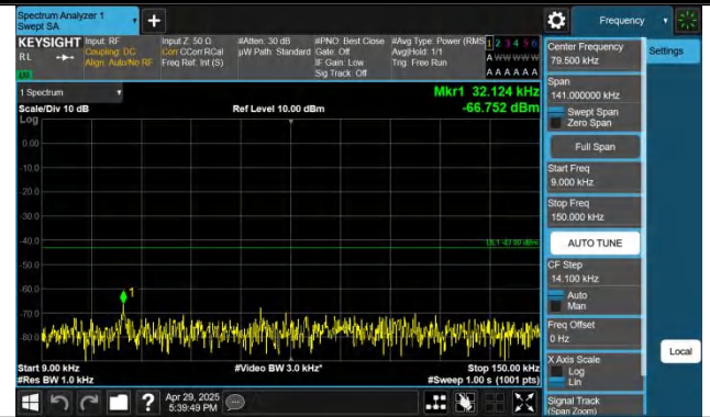
Band2-5MHz-QPSK-18625-1RB#24-0.009~0.15-PASS
