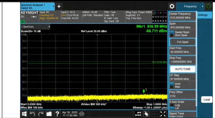
Band2-3MHz-QPSK-19185-1RB#14-30~1000-PASS
