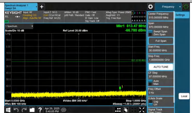
Band2-5MHz-QPSK-18625-1RB#24-30~1000-PASS
