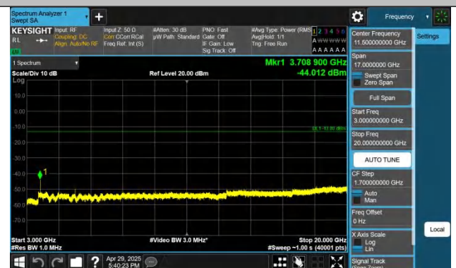
Band2-5MHz-QPSK-18625-1RB#24-3000~20000-PASS
