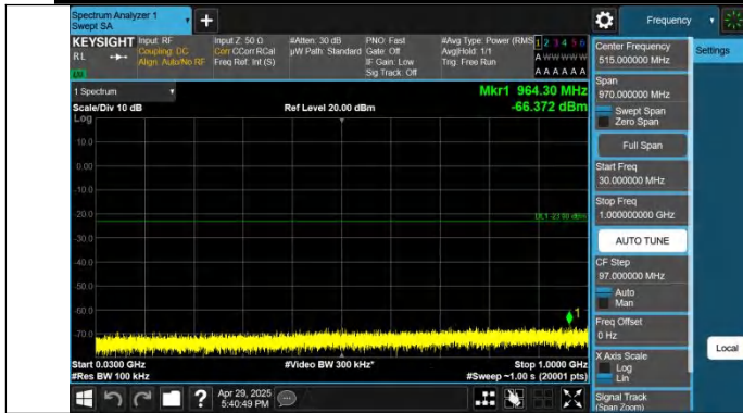
Band2-5MHz-QPSK-18900-1RB#0-30~1000-PASS
