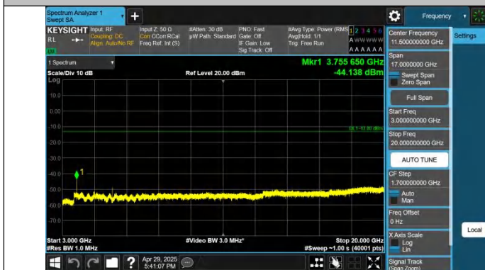
Band2-5MHz-QPSK-18900-1RB#0-3000~20000-PASS
