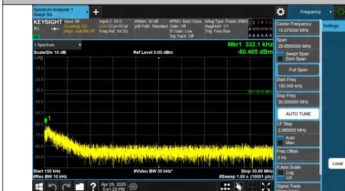
Band2-5MHz-QPSK-18900-1RB#24-0.15~30-PASS
