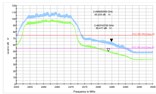
802.11n HT20-Channel 11 Peak+ Average
