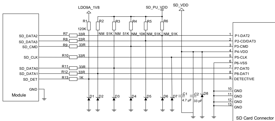
Figure 23: Reference Design of SD Card Interface
