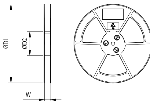
Figure 46: Plastic Reel Dimension Drawing
