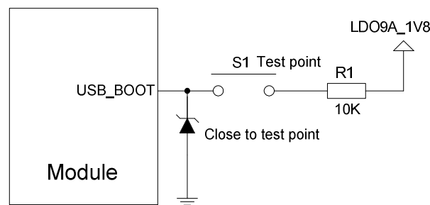
Figure 13: Reference Design of USB_BOOT
