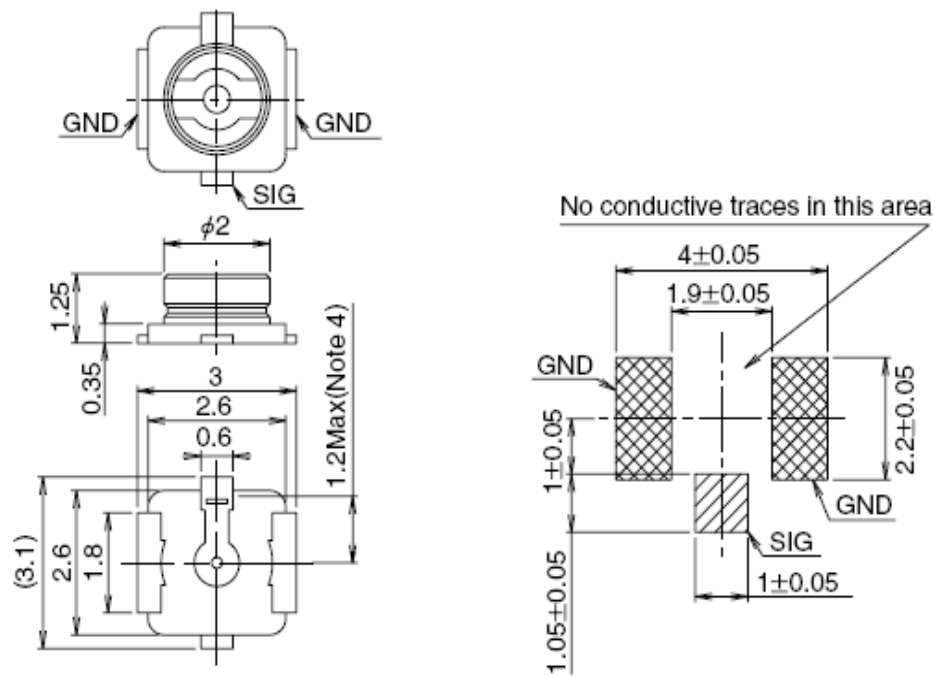
Figure 36: Dimensions of the Receptacle (Unit: mm)
