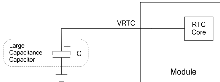
Figure 10: RTC Powered by Large Capacitance Capacitor
