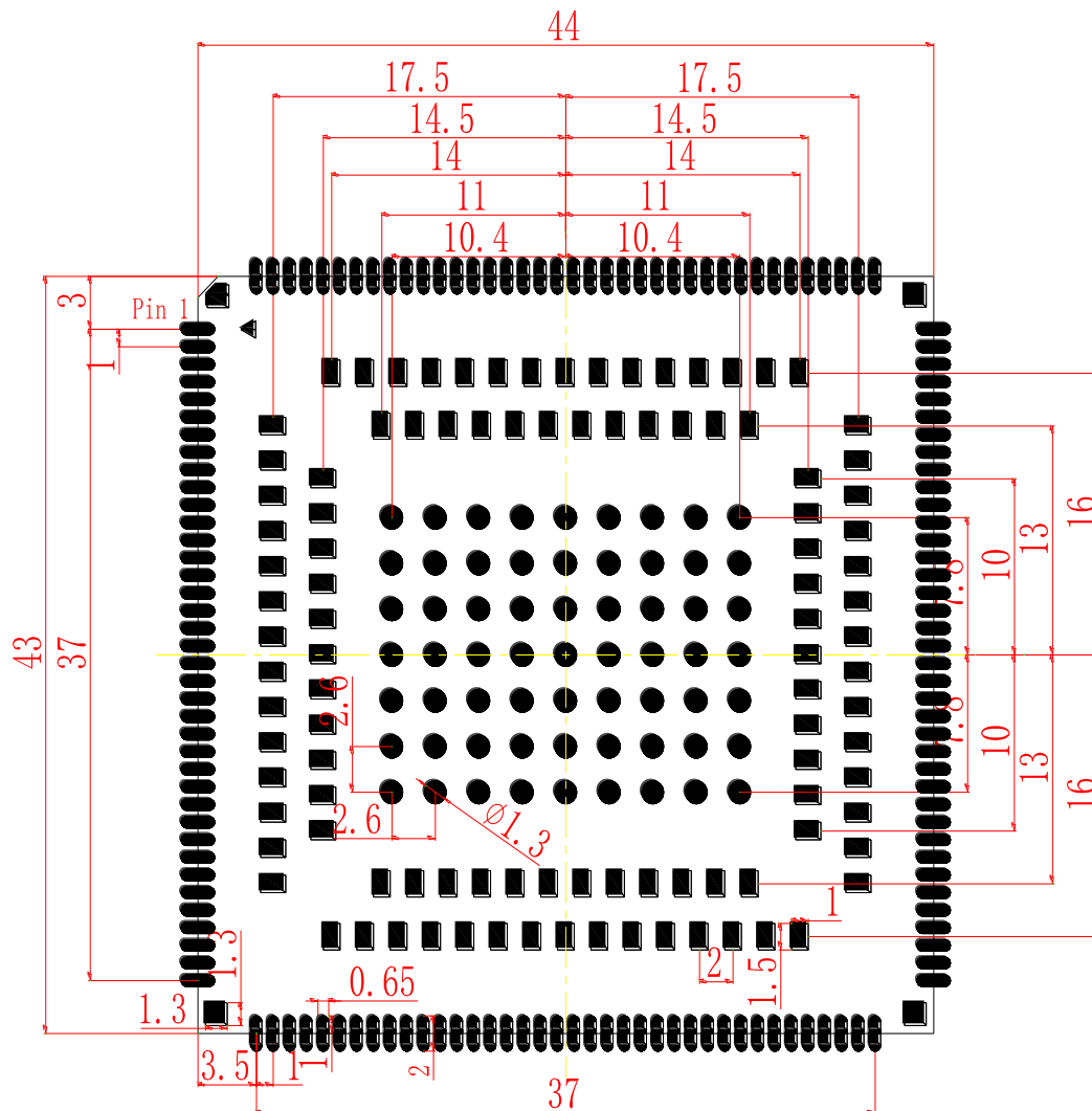
Figure 42: Recommended Footprint (Top View)
