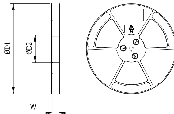
Figure 46: Plastic Reel Dimension Drawing
