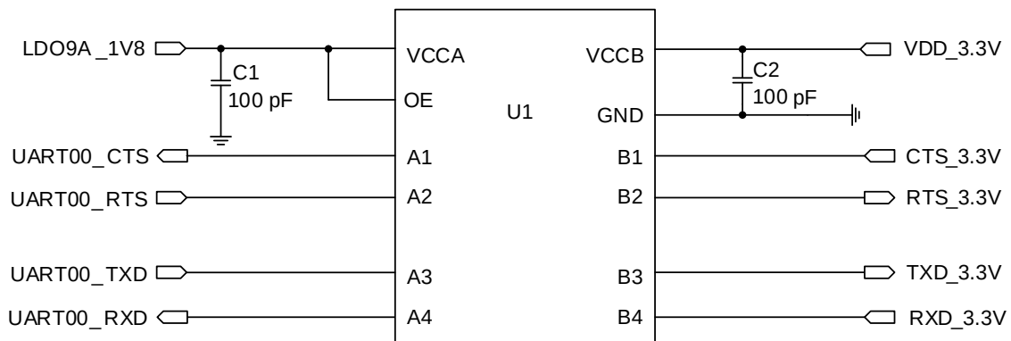
Figure 17: Reference Design with Level Translator Chip (for UART00)
