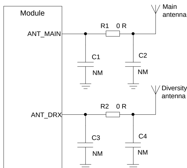
Figure 29: Reference Design for RF Antenna Interfaces
