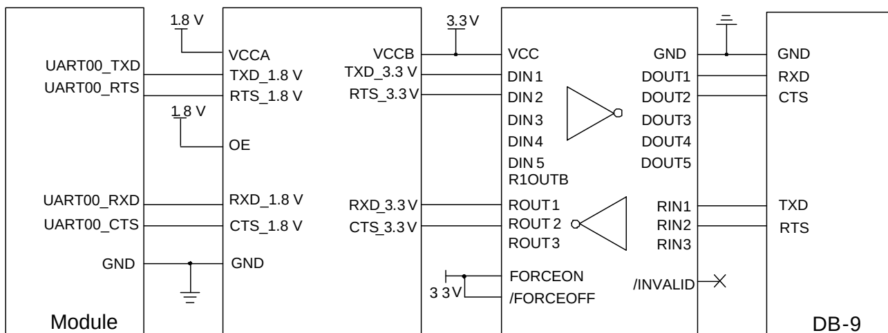
Figure 18: RS-232 Level Match Circuit (for UART00)
