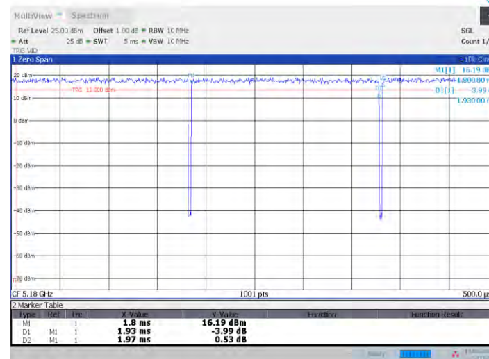
11n20SISO_Ant0_5180
