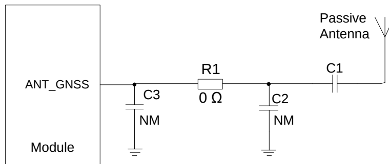
Figure 31: Reference Circuit Design for Passive GNSS Antenna
