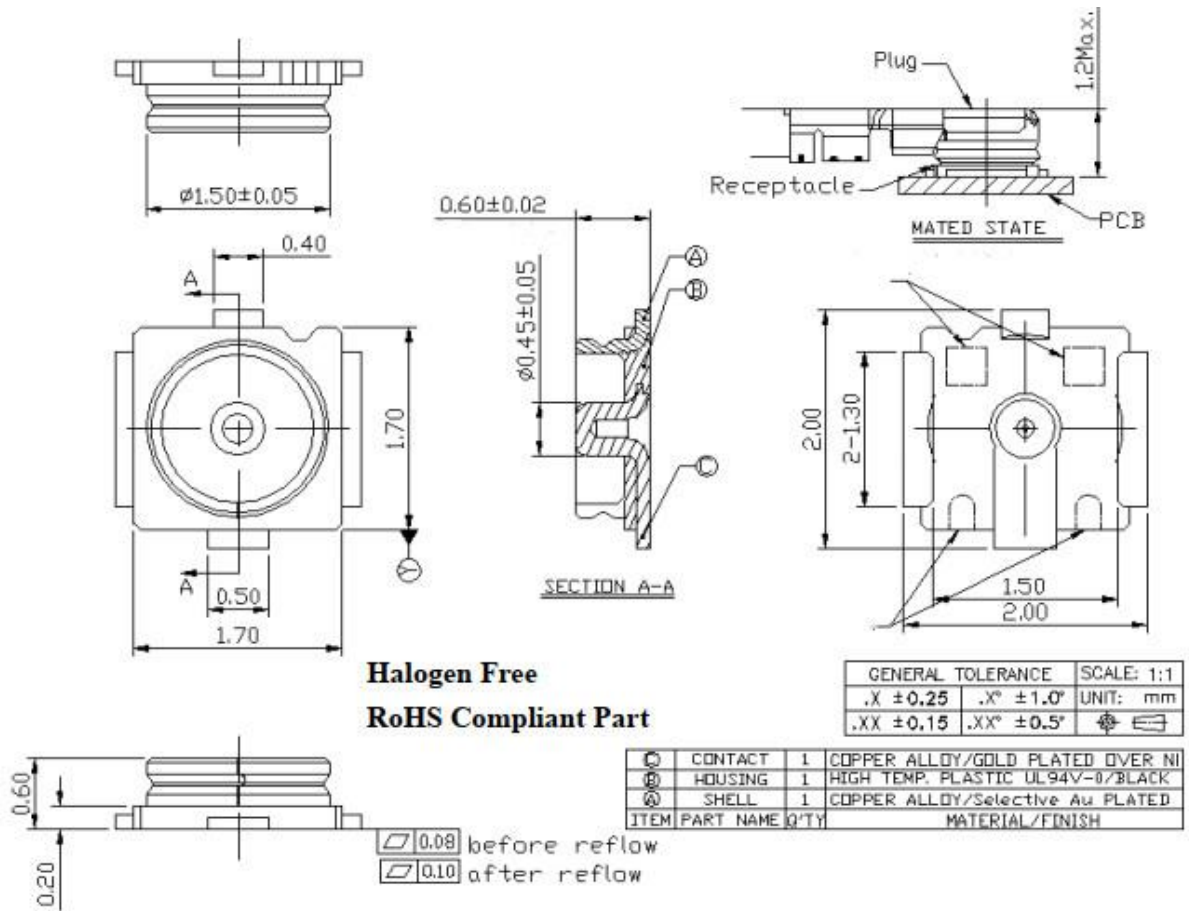
Figure 31: Dimensions of the ECT 818000500 Connector (Unit: mm)
