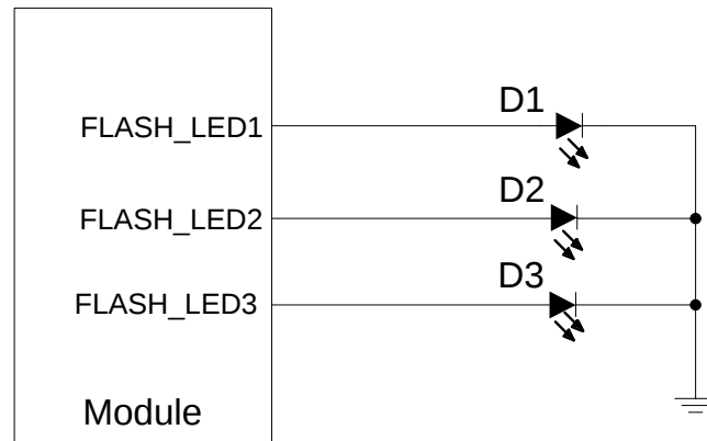
Figure 28: Reference Circuit Design for Flashlight Interfaces
