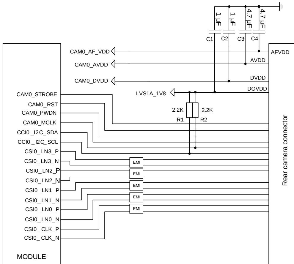
Figure 26: Reference Circuit Design for CSIO
