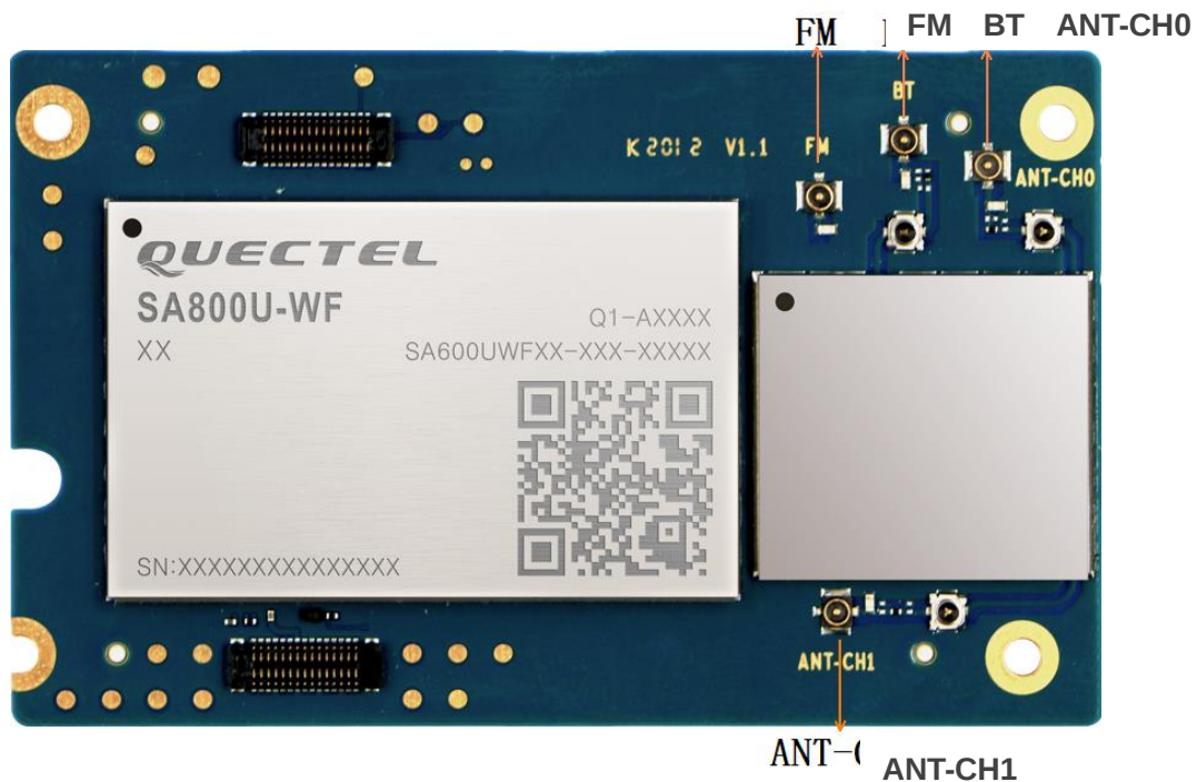
Figure 30: Antenna Connectors
