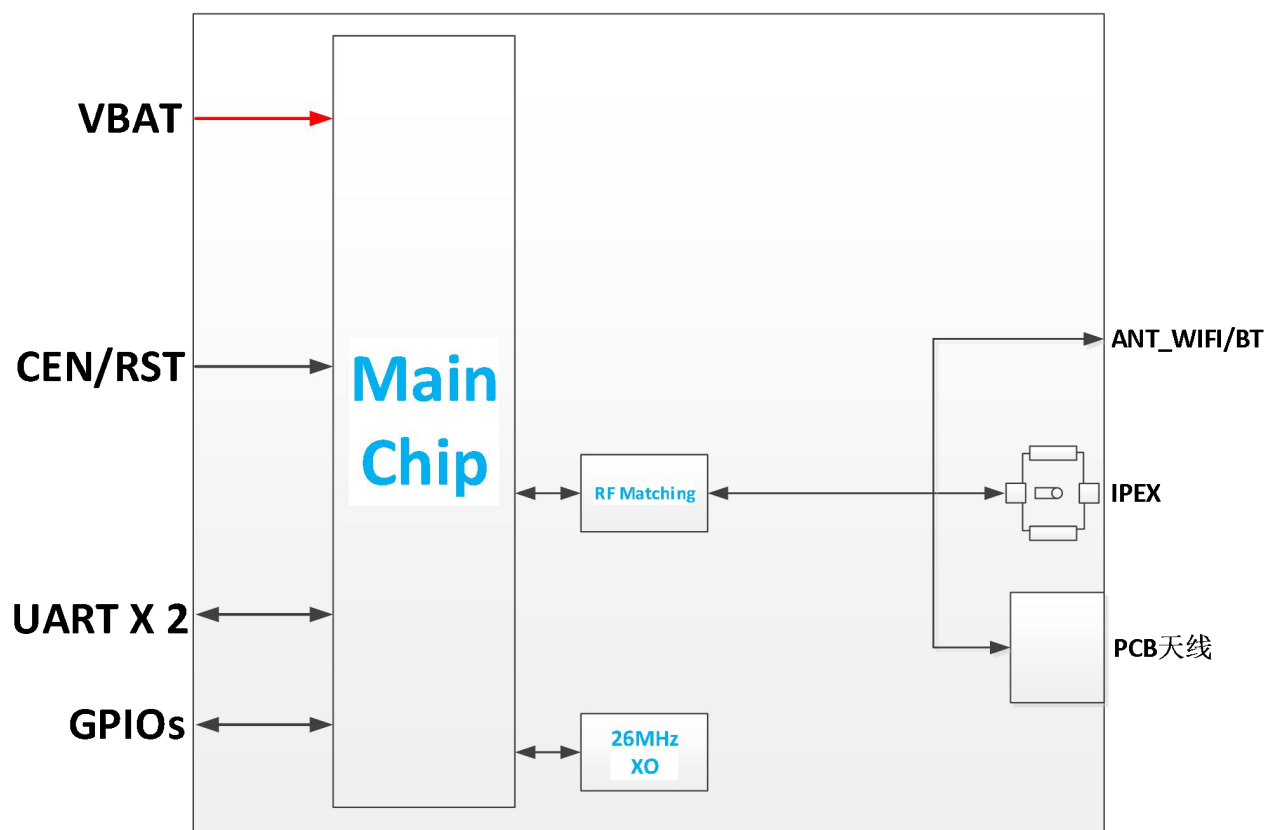
Figure 1: Functional Diagram
