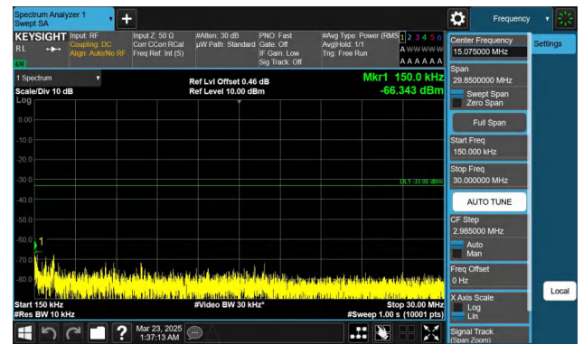
Band66-10MHz-QPSK-132622-1RB#0-0.15~30-PASS
