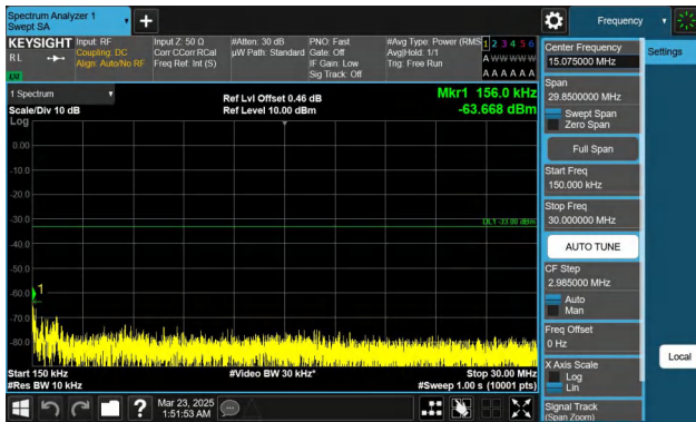
Band66-20MHz-QPSK-132322-1RB#99-0.15~30-PASS
