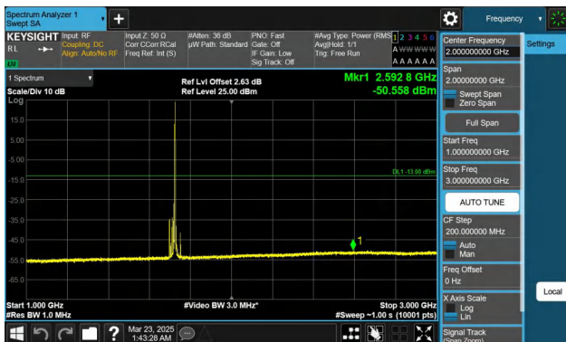
Band66-15MHz-QPSK-132047-1RB#74-1000~3000-PASS
