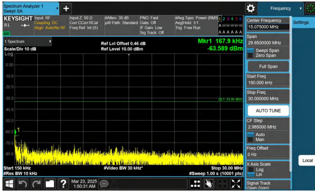
Band66-20MHz-QPSK-132072-1RB#99-0.15~30-PASS
