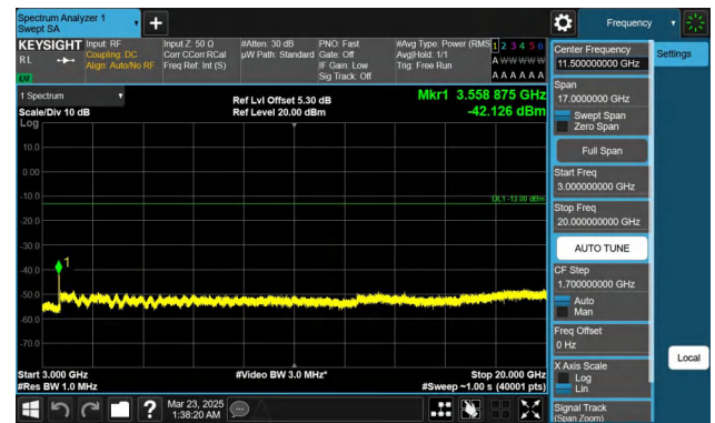
Band66-10MHz-QPSK-132622-1RB#49-3000~20000-PASS
