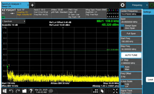
Band66-15MHz-QPSK-132322-1RB#74-0.15~30-PASS
