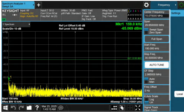
Band66-15MHz-QPSK-132047-1RB#74-0.15~30-PASS
