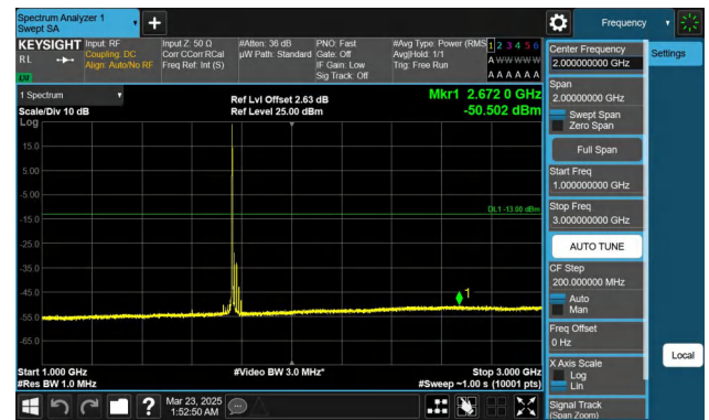
Band66-20MHz-QPSK-132572-1RB#0-1000~3000-PASS
