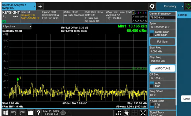
Band66-15MHz-QPSK-132322-1RB#0-0.009~0.15-PASS
