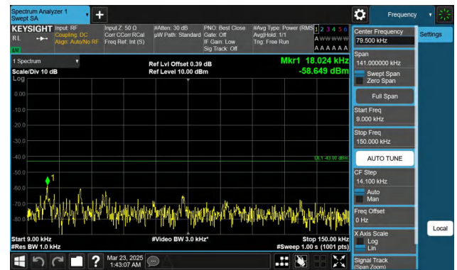
Band66-15MHz-QPSK-132047-1RB#74-0.009~0.15-PASS
