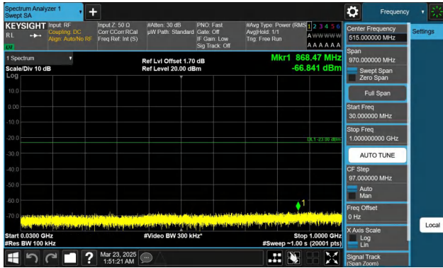
Band66-20MHz-QPSK-132322-1RB#0-30~1000-PASS
