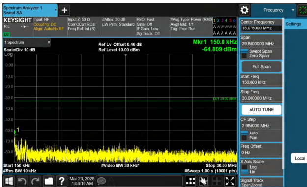
Band66-20MHz-QPSK-132572-1RB#99-0.15~30-PASS
