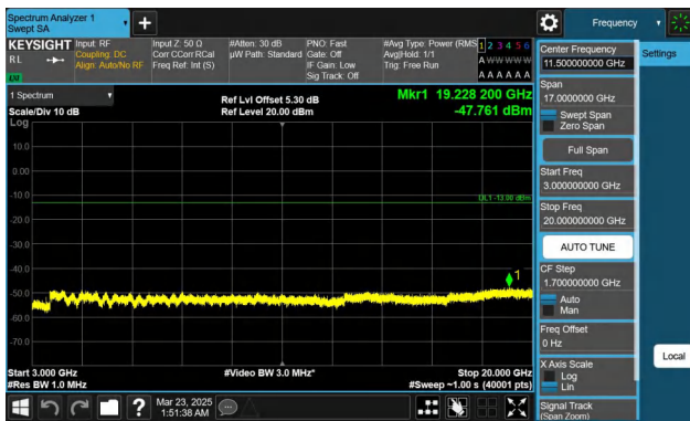
Band66-20MHz-QPSK-132322-1RB#0-3000~20000-PASS
