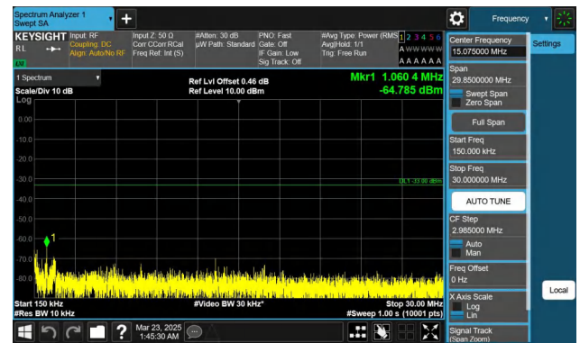
Band66-15MHz-QPSK-132597-1RB#0-0.15~30-PASS
