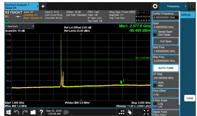
Band66-20MHz-QPSK-132072-1RB#0-1000~3000-PASS
