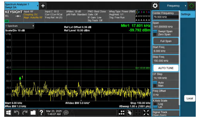
Band66-15MHz-QPSK-132597-1RB#74-0.009~0.15-PASS
