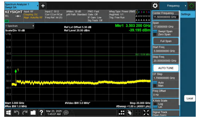
Band66-15MHz-QPSK-132322-1RB#74-3000~20000-PASS
