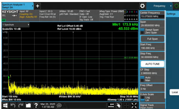
Band66-10MHz-QPSK-132622-1RB#49-0.15~30-PASS
