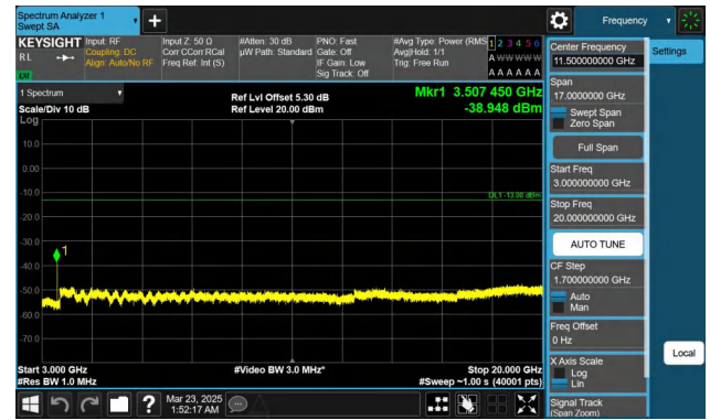
Band66-20MHz-QPSK-132322-1RB#99-3000~20000-PASS
