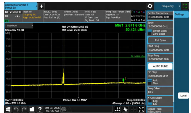
Band66-10MHz-QPSK-132622-1RB#0-1000~3000-PASS
