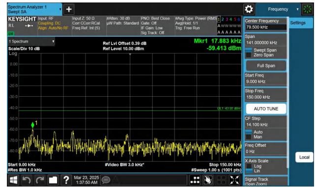
Band66-10MHz-QPSK-132622-1RB#49-0.009~0.15-PASS
