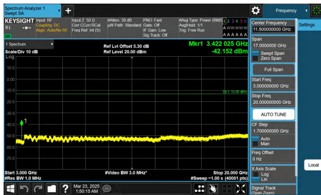
Band66-20MHz-QPSK-132072-1RB#0-3000~20000-PASS
