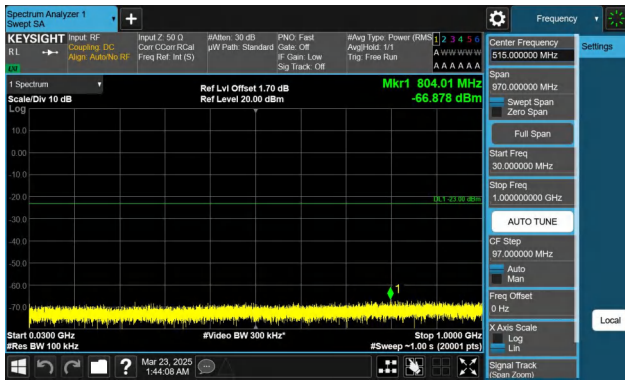
Band66-15MHz-QPSK-132322-1RB#0-30~1000-PASS
