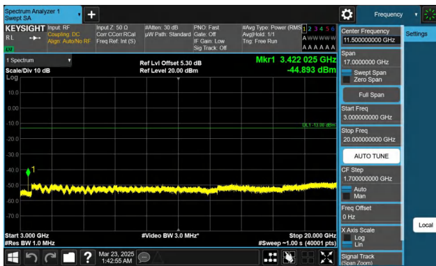
Band66-15MHz-QPSK-132047-1RB#0-3000~20000-PASS
