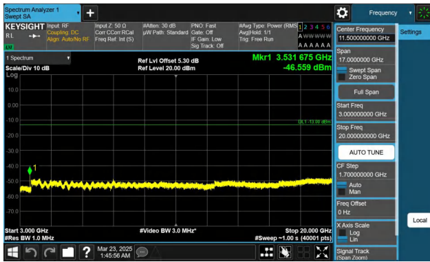
Band66-15MHz-QPSK-132597-1RB#0-3000~20000-PASS
