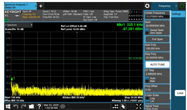
Band66-20MHz-QPSK-132572-1RB#0-0.15~30-PASS
