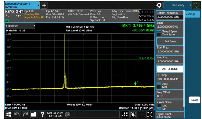
Band66-20MHz-QPSK-132322-1RB#0-1000~3000-PASS
