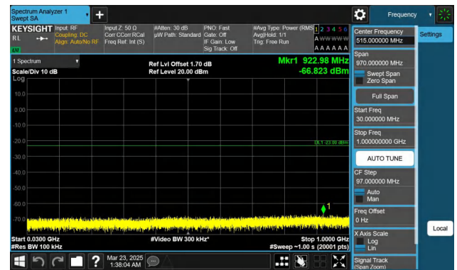
Band66-10MHz-QPSK-132622-1RB#49-30~1000-PASS
