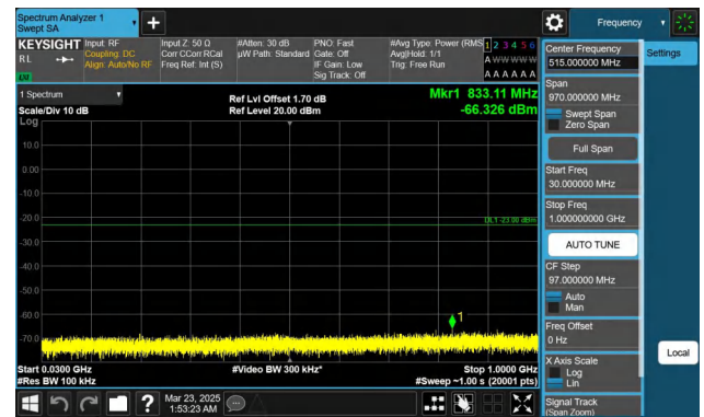
Band66-20MHz-QPSK-132572-1RB#99-30~1000-PASS
