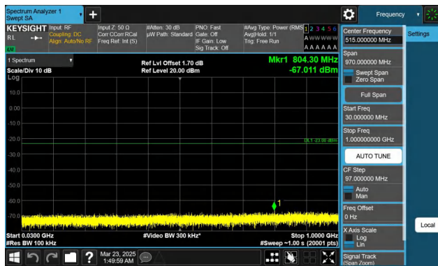
Band66-20MHz-QPSK-132072-1RB#0-30~1000-PASS
