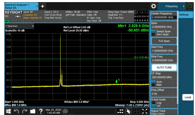
Band66-15MHz-QPSK-132047-1RB#0-1000~3000-PASS
