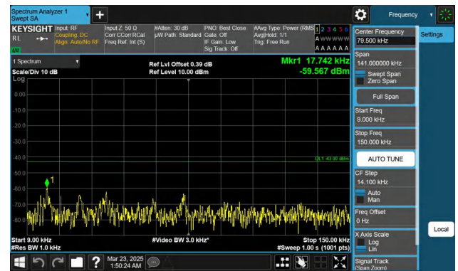
Band66-20MHz-QPSK-132072-1RB#99-0.009~0.15-PASS
