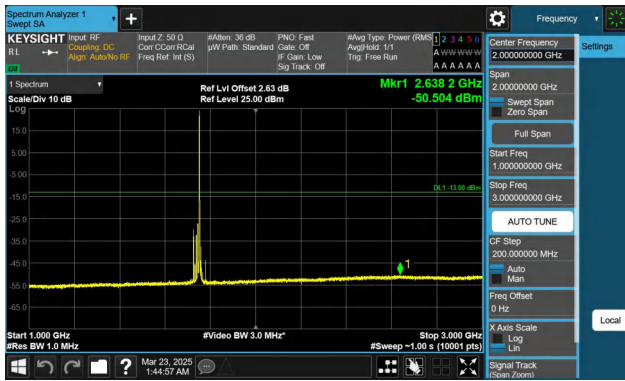
Band66-15MHz-QPSK-132322-1RB#74-1000~3000-PASS
