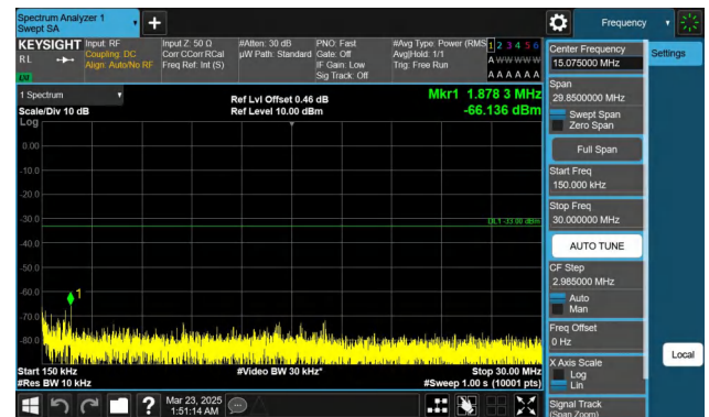
Band66-20MHz-QPSK-132322-1RB#0-0.15~30-PASS
