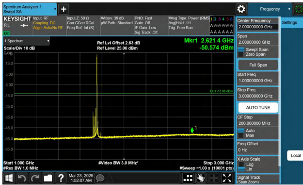
Band66-20MHz-QPSK-132322-1RB#99-1000~3000-PASS
