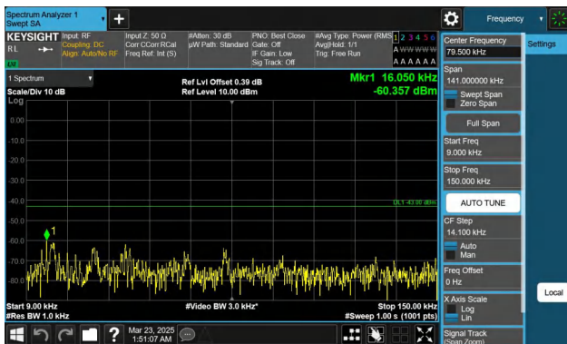
Band66-20MHz-QPSK-132322-1RB#0-0.009~0.15-PASS
