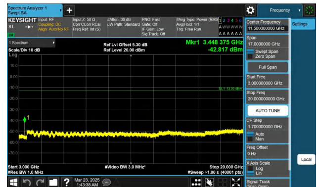
Band66-15MHz-QPSK-132047-1RB#74-3000~20000-PASS
