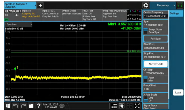
Band66-20MHz-QPSK-132572-1RB#99-3000~20000-PASS
