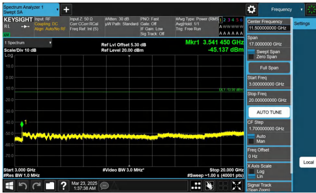
Band66-10MHz-QPSK-132622-1RB#0-3000~20000-PASS
