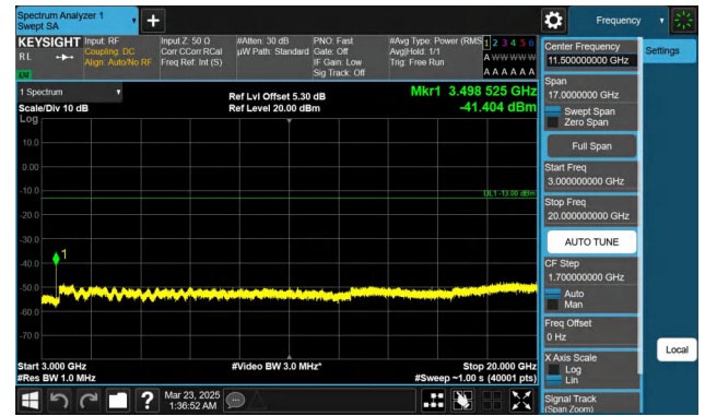
Band66-10MHz-QPSK-132322-1RB#49-3000~20000-PASS
