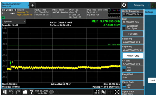
Band66-15MHz-QPSK-132322-1RB#0-3000~20000-PASS
