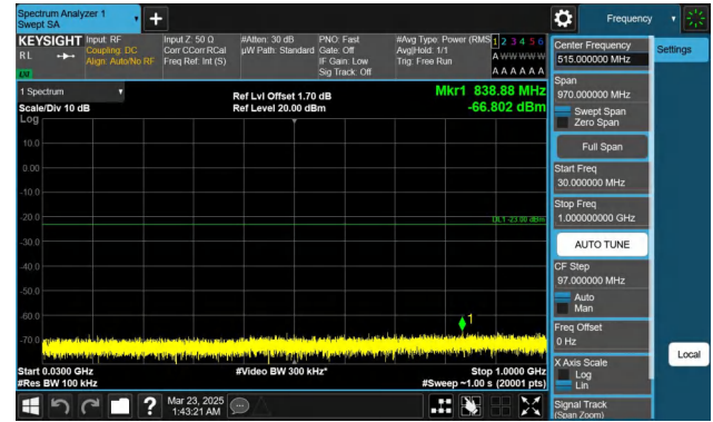
Band66-15MHz-QPSK-132047-1RB#74-30~1000-PASS
