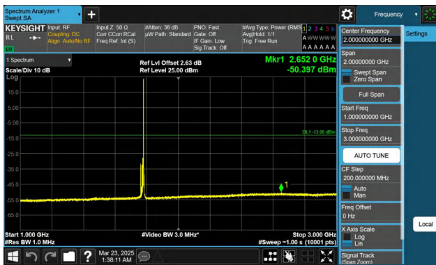
Band66-10MHz-QPSK-132622-1RB#49-1000~3000-PASS
