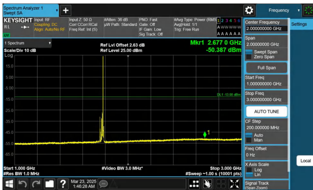
Band66-15MHz-QPSK-132597-1RB#74-1000~3000-PASS
