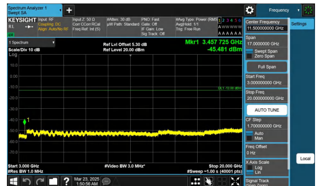
Band66-20MHz-QPSK-132072-1RB#99-3000~20000-PASS
