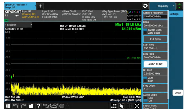
Band66-15MHz-QPSK-132322-1RB#0-0.15~30-PASS
