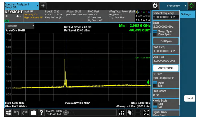
Band66-15MHz-QPSK-132597-1RB#0-1000~3000-PASS
