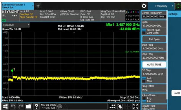
Band66-3MHz-QPSK-132322-1RB#0-3000~20000-PASS
