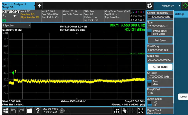
Band66-5MHz-QPSK-132647-1RB#0-3000~20000-PASS
