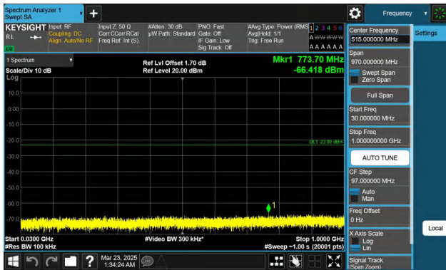
Band66-10MHz-QPSK-132022-1RB#0-30~1000-PASS
