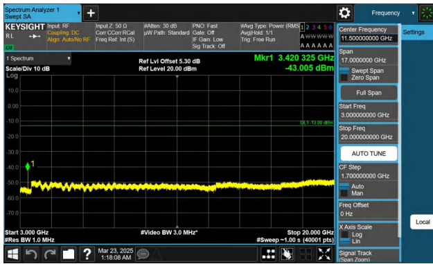
Band66-3MHz-QPSK-131987-1RB#0-3000~20000-PASS
