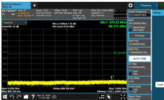
Band66-3MHz-QPSK-131987-1RB#0-30~1000-PASS
