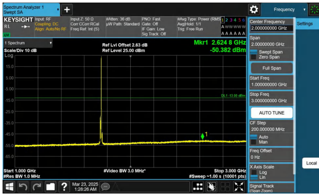
Band66-5MHz-QPSK-132322-1RB#24-1000~3000-PASS
