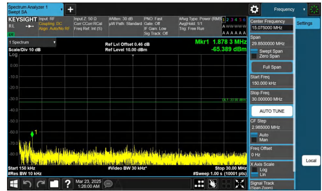
Band66-5MHz-QPSK-131997-1RB#0-0.15~30-PASS
