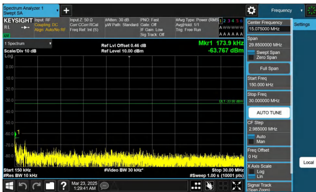
Band66-5MHz-QPSK-132647-1RB#24-0.15~30-PASS
