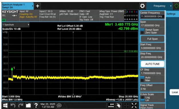
Band66-5MHz-QPSK-132322-1RB#0-3000~20000-PASS
