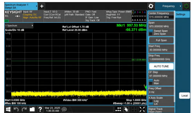
Band66-10MHz-QPSK-132322-1RB#49-30~1000-PASS
