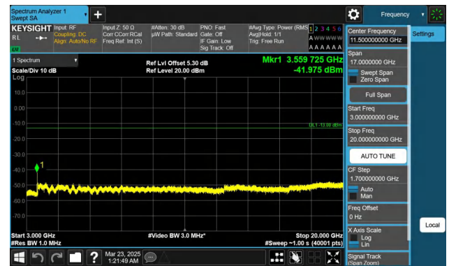
Band66-3MHz-QPSK-132657-1RB#14-3000~20000-PASS
