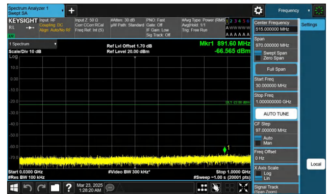
Band66-5MHz-QPSK-132322-1RB#24-30~1000-PASS
