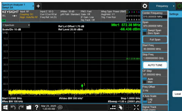
Band66-3MHz-QPSK-132657-1RB#0-30~1000-PASS
