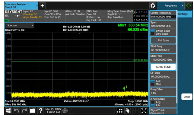
Band66-5MHz-QPSK-131997-1RB#24-30~1000-PASS
