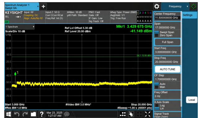
Band66-5MHz-QPSK-131997-1RB#24-3000~20000-PASS
