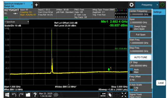
Band66-10MHz-QPSK-132022-1RB#0-1000~3000-PASS
