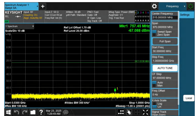
Band66-5MHz-QPSK-132647-1RB#24-30~1000-PASS
