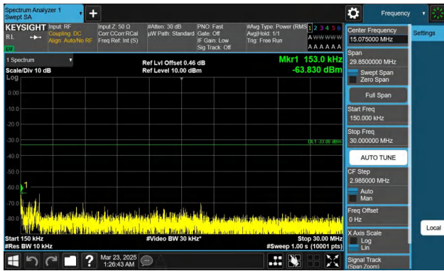
Band66-5MHz-QPSK-131997-1RB#24-0.15~30-PASS
