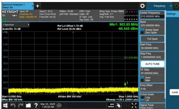
Band66-5MHz-QPSK-131997-1RB#0-30~1000-PASS
