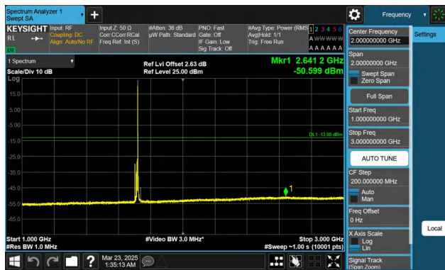
Band66-10MHz-QPSK-132022-1RB#49-1000~3000-PASS
