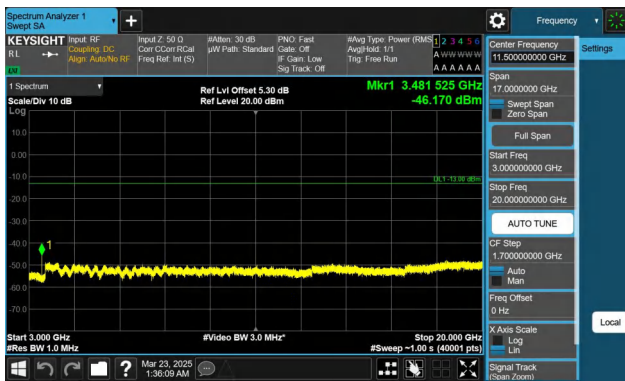
Band66-10MHz-QPSK-132322-1RB#0-3000~20000-PASS
