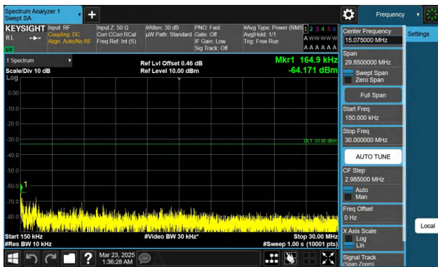
Band66-10MHz-QPSK-132322-1RB#49-0.15~30-PASS
