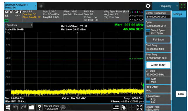
Band66-3MHz-QPSK-132322-1RB#14-30~1000-PASS
