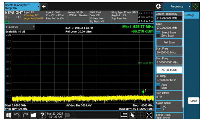
Band66-3MHz-QPSK-132657-1RB#14-30~1000-PASS
