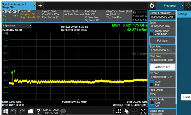
Band66-10MHz-QPSK-132022-1RB#0-3000~20000-PASS
