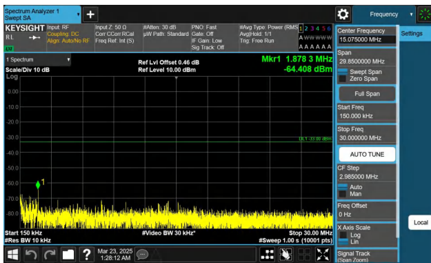
Band66-5MHz-QPSK-132322-1RB#24-0.15~30-PASS
