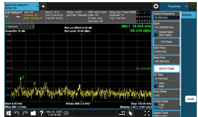
Band66-3MHz-QPSK-132322-1RB#14-0.009~0.15-PASS
