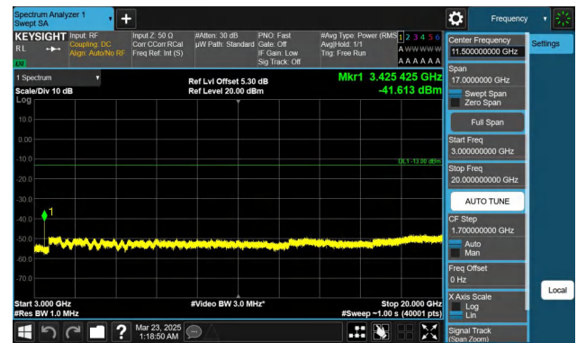
Band66-3MHz-QPSK-131987-1RB#14-3000~20000-PASS
