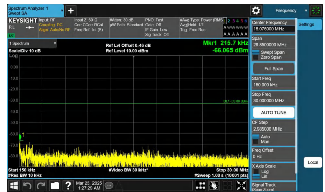
Band66-5MHz-QPSK-132322-1RB#0-0.15~30-PASS
