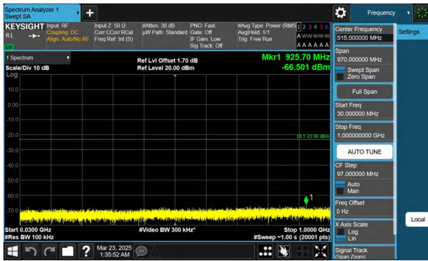
Band66-10MHz-QPSK-132322-1RB#0-30~1000-PASS
