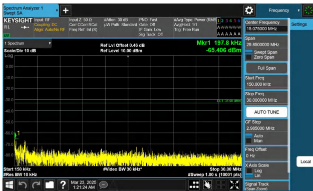
Band66-3MHz-QPSK-132657-1RB#14-0.15~30-PASS
