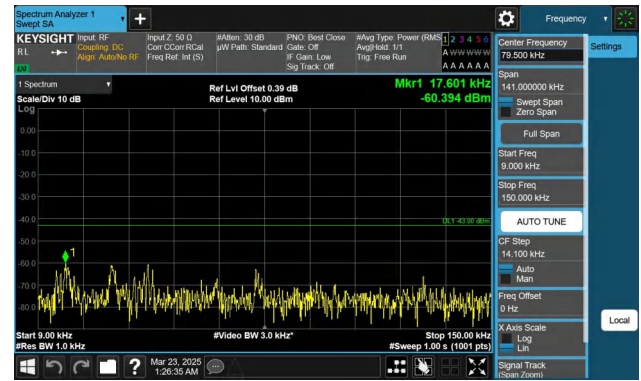
Band66-5MHz-QPSK-131997-1RB#24-0.009~0.15-PASS
