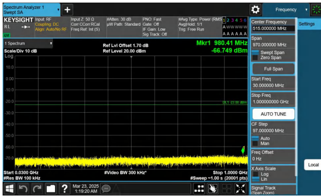
Band66-3MHz-QPSK-132322-1RB#0-30~1000-PASS
