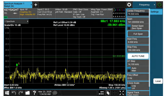
Band66-10MHz-QPSK-132022-1RB#49-0.009~0.15-PASS
