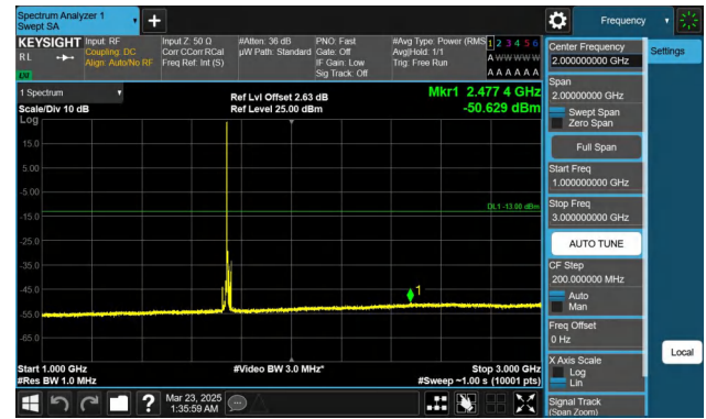
Band66-10MHz-QPSK-132322-1RB#0-1000~3000-PASS
