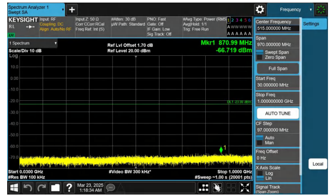
Band66-3MHz-QPSK-131987-1RB#14-30~1000-PASS
