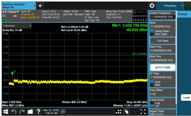
Band66-5MHz-QPSK-131997-1RB#0-3000~20000-PASS
