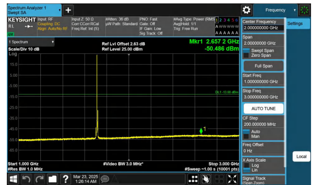
Band66-5MHz-QPSK-131997-1RB#0-1000~3000-PASS
