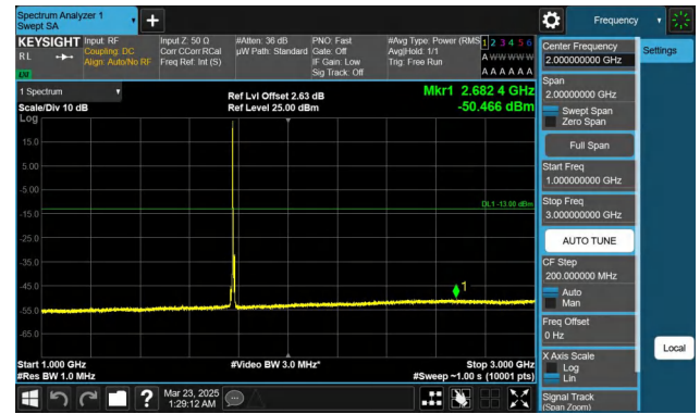
Band66-5MHz-QPSK-132647-1RB#0-1000~3000-PASS
