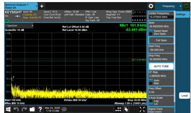
Band66-3MHz-QPSK-132322-1RB#0-0.15~30-PASS
