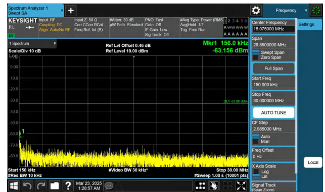
Band66-5MHz-QPSK-132647-1RB#0-0.15~30-PASS
