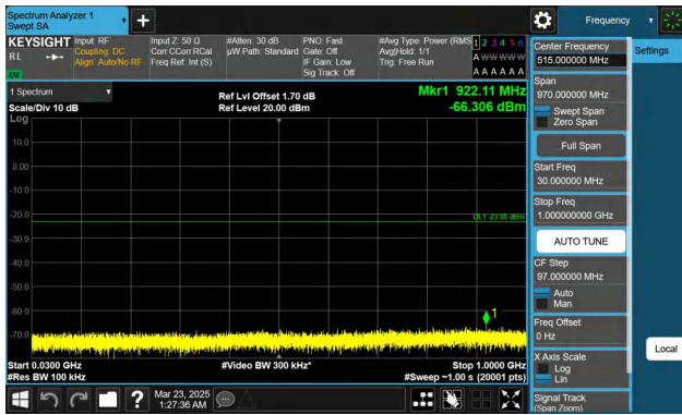
Band66-5MHz-QPSK-132322-1RB#0-30~1000-PASS
