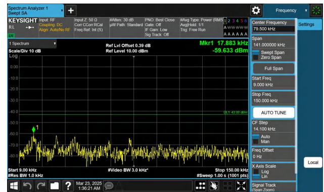
Band66-10MHz-QPSK-132322-1RB#49-0.009~0.15-PASS
