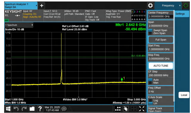
Band66-5MHz-QPSK-132322-1RB#0-1000~3000-PASS
