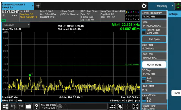
Band66-5MHz-QPSK-132322-1RB#0-0.009~0.15-PASS
