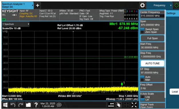
Band66-5MHz-QPSK-132647-1RB#0-30~1000-PASS
