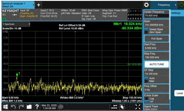
Band66-10MHz-QPSK-132022-1RB#0-0.009~0.15-PASS
