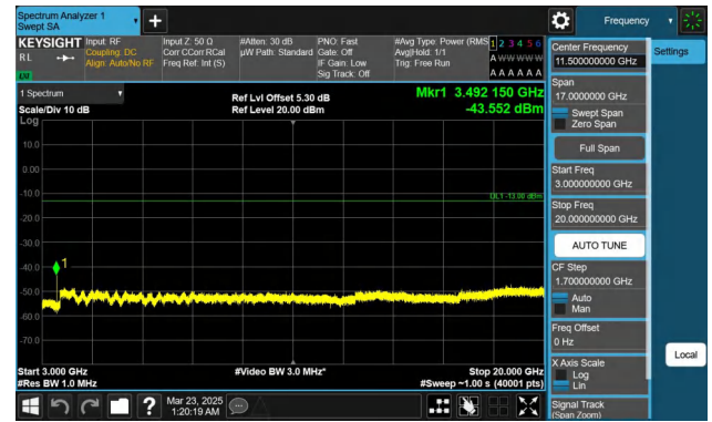
Band66-3MHz-QPSK-132322-1RB#14-3000~20000-PASS
