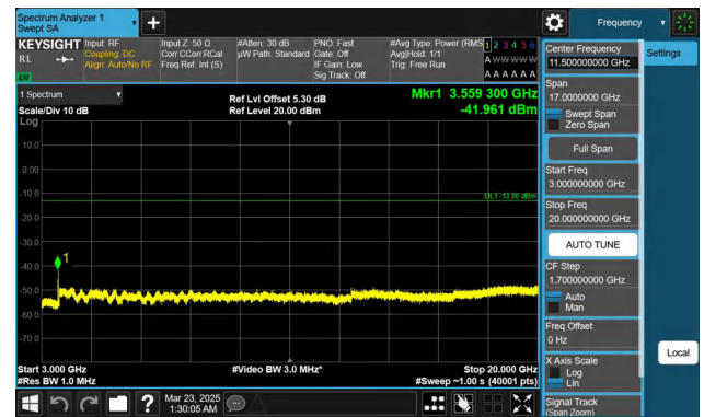
Band66-5MHz-QPSK-132647-1RB#24-3000~20000-PASS
