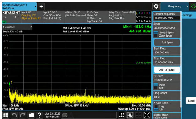
Band66-3MHz-QPSK-132322-1RB#14-0.15~30-PASS
