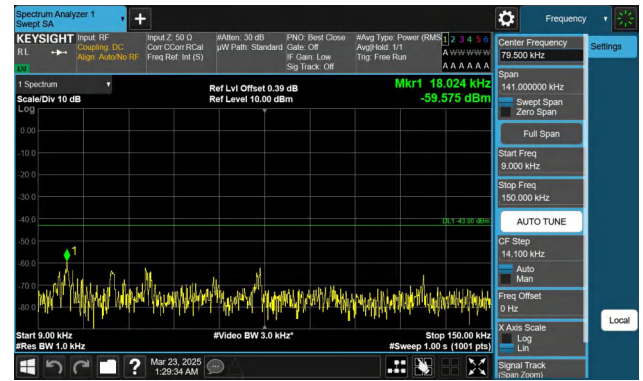
Band66-5MHz-QPSK-132647-1RB#24-0.009~0.15-PASS
