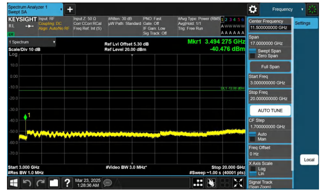
Band66-5MHz-QPSK-132322-1RB#24-3000~20000-PASS
