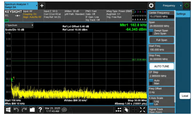
Band66-3MHz-QPSK-131987-1RB#0-0.15~30-PASS
