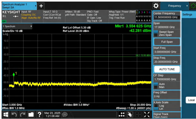
Band66-3MHz-QPSK-132657-1RB#0-3000~20000-PASS
