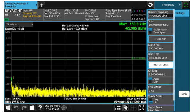
Band66-10MHz-QPSK-132022-1RB#0-0.15~30-PASS
