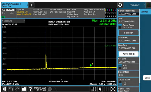
Band66-5MHz-QPSK-131997-1RB#24-1000~3000-PASS
