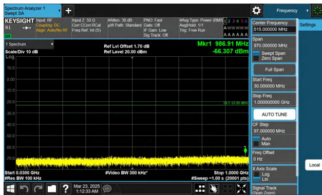
Band66-1.4MHz-QPSK-132665-1RB#0-30~1000-PASS
