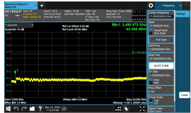
Band66-1.4MHz-QPSK-132322-1RB#5-3000~20000-PASS
