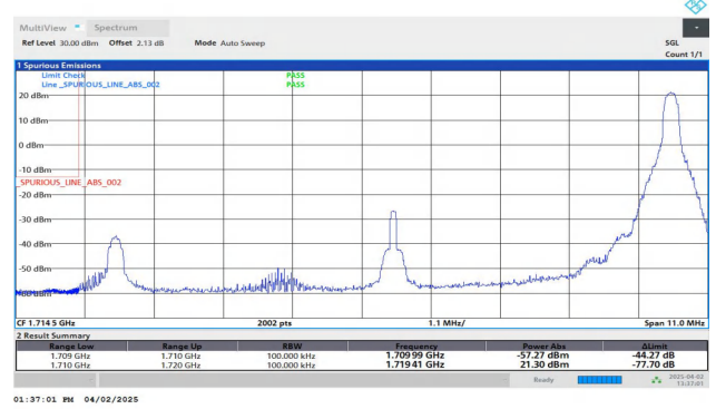
Band66-10MHz-QPSK-132022-1RB#49-PASS
