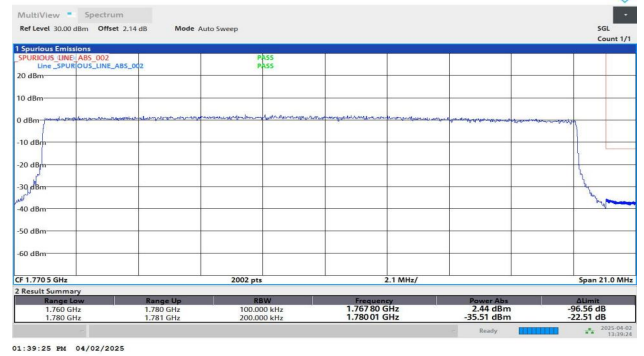
Band66-20MHz-QPSK-132572-100RB#0-PASS
