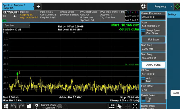
Band66-1.4MHz-QPSK-132665-1RB#0-0.009~0.15-PASS
