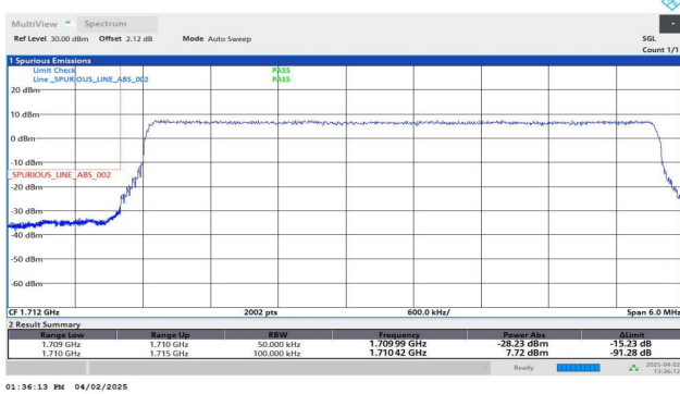
Band66-5MHz-QPSK-131997-25RB#0-PASS
