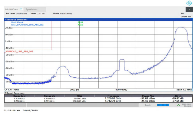
Band66-3MHz-QPSK-131987-1RB#14-PASS
