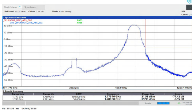
Band66-3MHz-QPSK-132657-1RB#14-PASS
