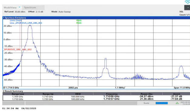
Band66-10MHz-QPSK-132022-1RB#0-PASS
