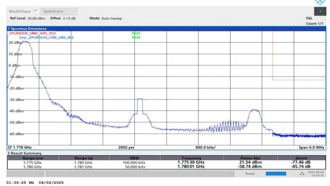
Band66-5MHz-QPSK-132647-1RB#0-PASS
