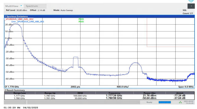
Band66-3MHz-QPSK-132657-1RB#0-PASS
