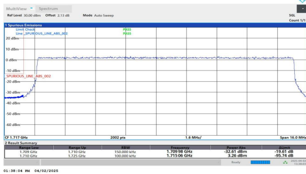
Band66-15MHz-QPSK-132047-75RB#0-PASS
