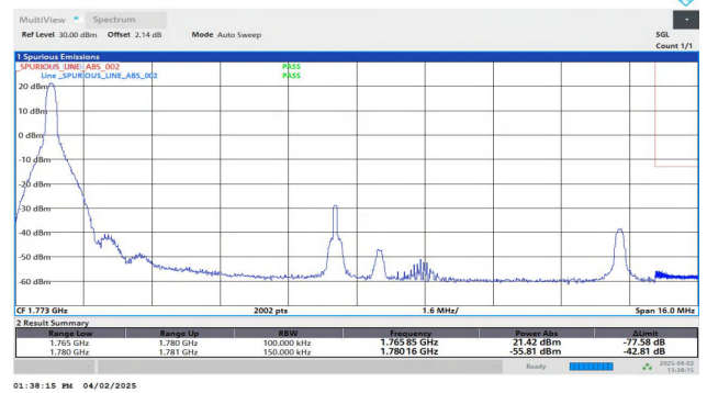
Band66-15MHz-QPSK-132597-1RB#0-PASS
