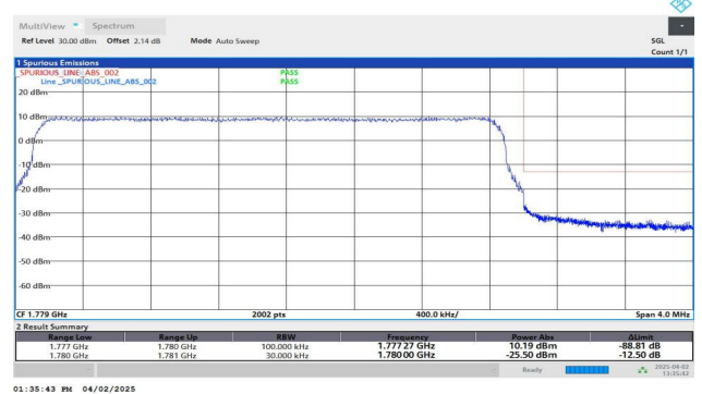
Band66-3MHz-QPSK-132657-15RB#0-PASS
