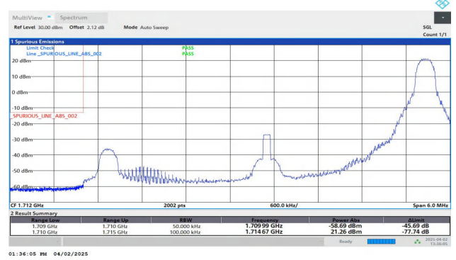
Band66-5MHz-QPSK-131997-1RB#24-PASS
