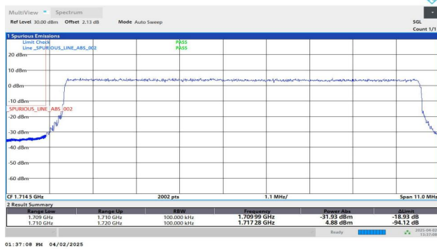
Band66-10MHz-QPSK-132022-50RB#0-PASS
