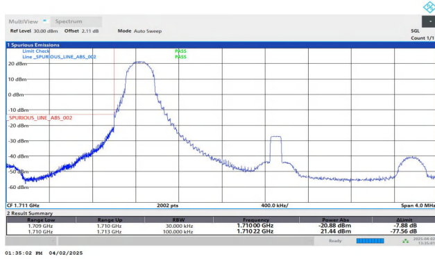
Band66-3MHz-QPSK-131987-1RB#0-PASS
