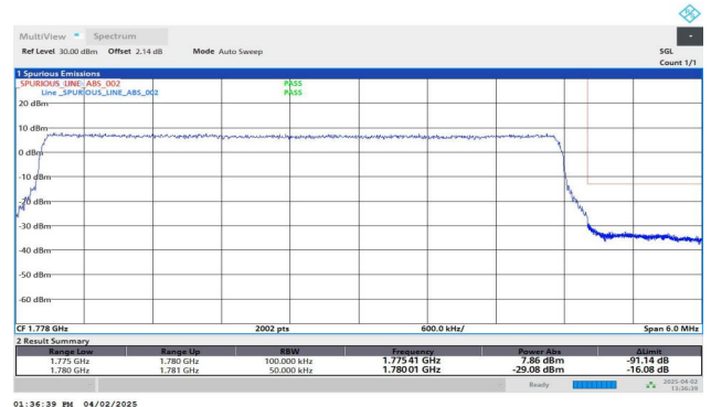
Band66-5MHz-QPSK-132647-25RB#0-PASS
