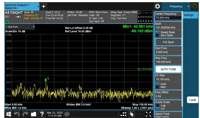
Band66-1.4MHz-QPSK-132322-1RB#5-0.009~0.15-PASS
