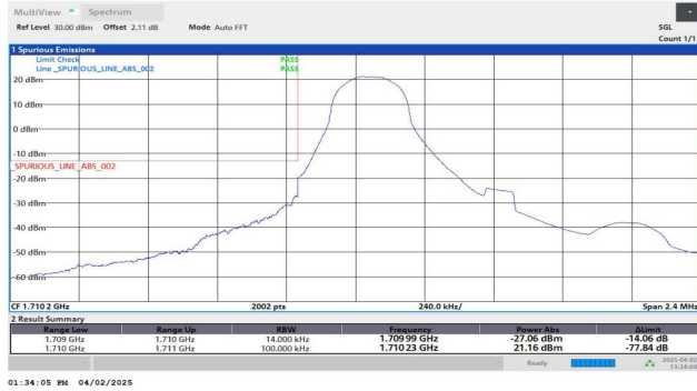
Band66-1.4MHz-QPSK-131979-1RB#0-PASS
