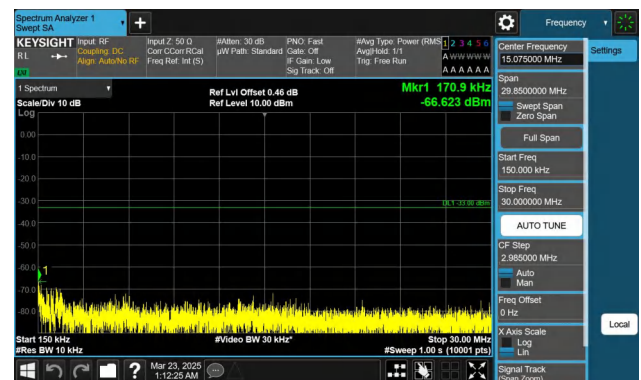
Band66-1.4MHz-QPSK-132665-1RB#0-0.15~30-PASS
