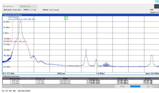
Band66-15MHz-QPSK-132047-1RB#0-PASS
