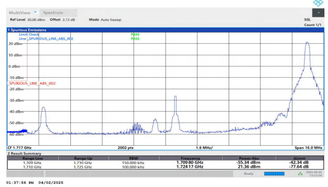
Band66-15MHz-QPSK-132047-1RB#74-PASS
