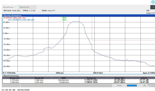
Band66-1.4MHz-QPSK-132665-1RB#5-PASS
