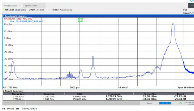
Band66-15MHz-QPSK-132597-1RB#74-PASS
