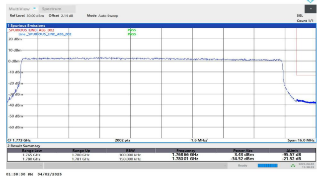
Band66-15MHz-QPSK-132597-75RB#0-PASS
