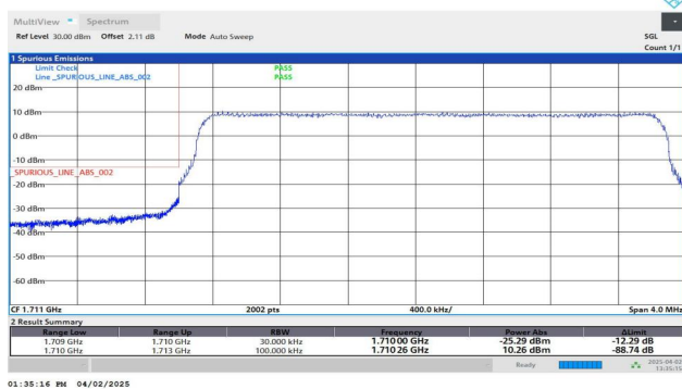
Band66-3MHz-QPSK-131987-15RB#0-PASS
