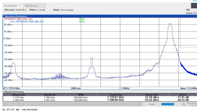
Band66-10MHz-QPSK-132622-1RB#49-PASS
