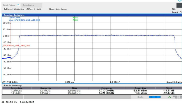
Band66-20MHz-QPSK-132072-100RB#0-PASS
