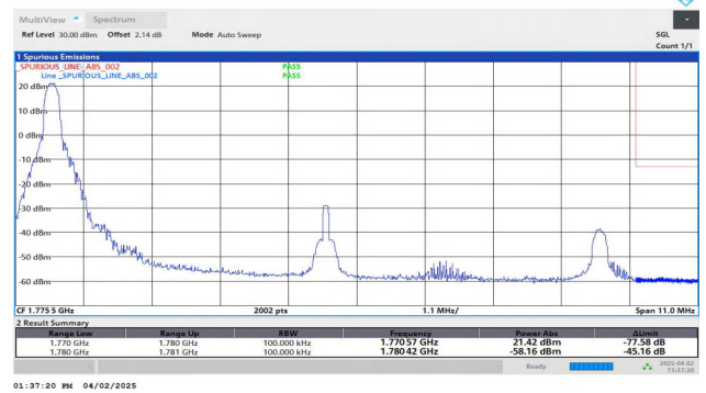
Band66-10MHz-QPSK-132622-1RB#0-PASS
