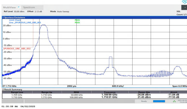
Band66-5MHz-QPSK-131997-1RB#0-PASS
