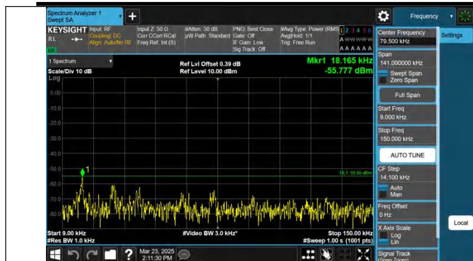
Band41-15MHz-QPSK-40620-1RB#0-0.009~0.15-PASS
