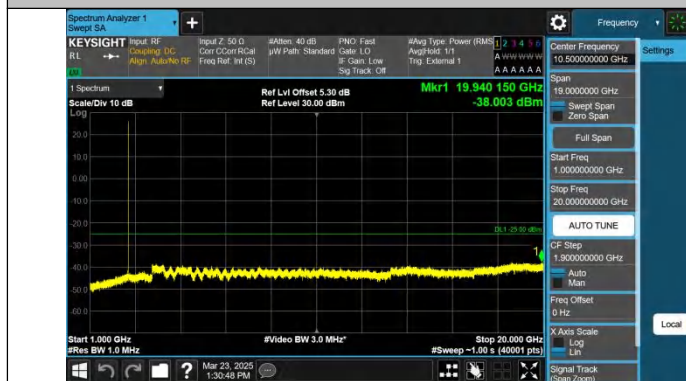
Band41-10MHz-QPSK-40620-1RB#49-1000~20000-PASS
