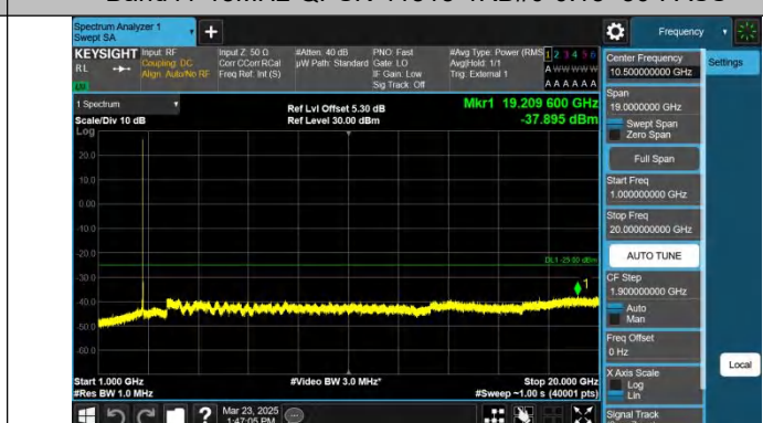
Band41-15MHz-QPSK-41515-1RB#0-1000~20000-PASS
