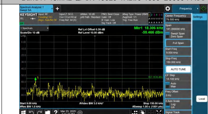
Band41-15MHz-QPSK-40620-1RB#74-0.009~0.15-PASS
