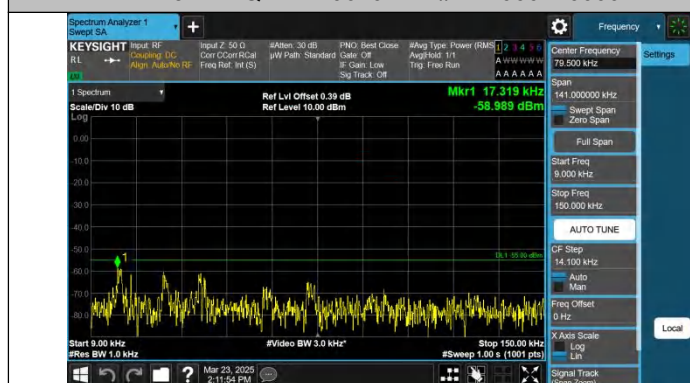
Band41-15MHz-QPSK-41515-1RB#0-0.009~0.15-PASS
