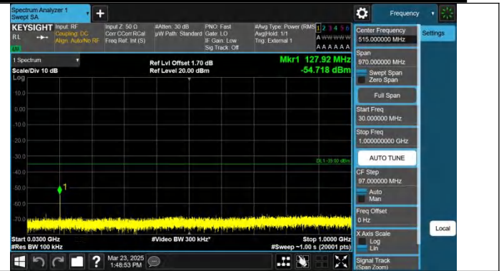
Band41-15MHz-QPSK-41515-1RB#74-30~1000-PASS
