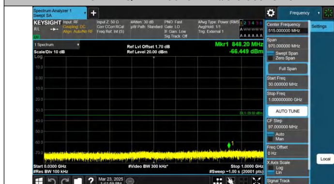
Band41-15MHz-QPSK-40620-1RB#0-30~1000-PASS
