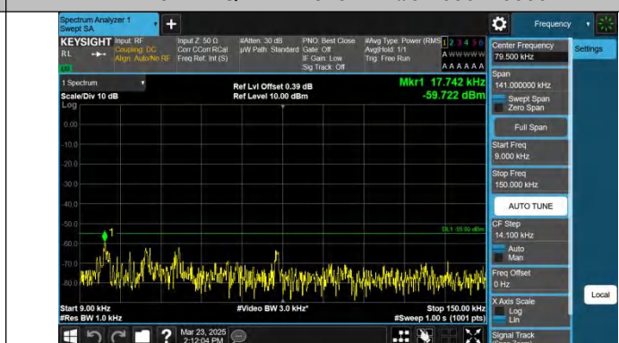
Band41-15MHz-QPSK-41515-1RB#74-0.009~0.15-PASS
