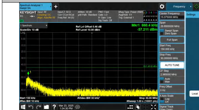
Band41-10MHz-QPSK-41540-1RB#49-0.15~30-PASS
