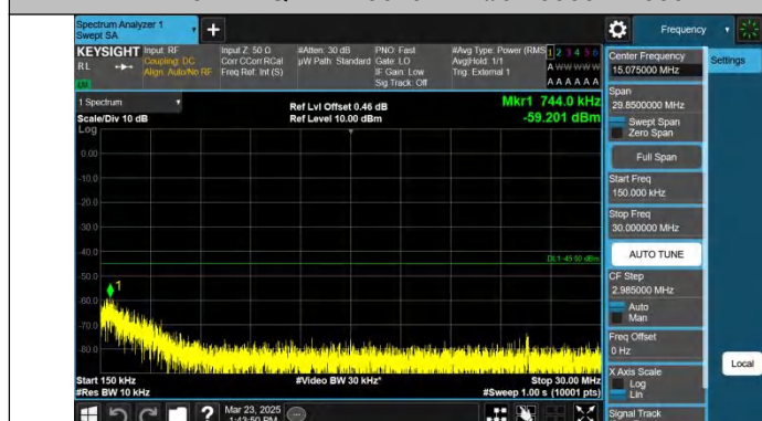
Band41-15MHz-QPSK-40620-1RB#74-0.15~30-PASS
