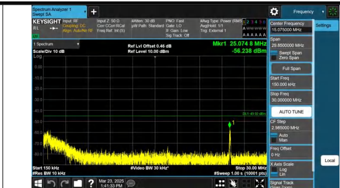
Band41-15MHz-QPSK-40620-1RB#0-0.15~30-PASS
