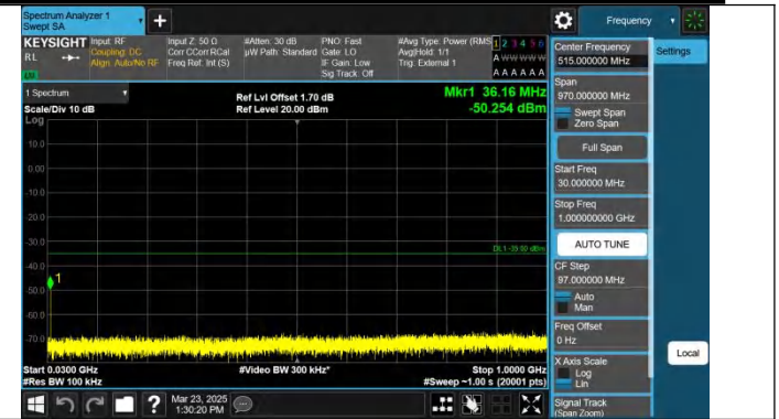
Band41-10MHz-QPSK-40620-1RB#49-30~1000-PASS
