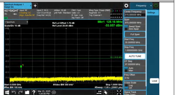
Band41-10MHz-QPSK-41540-1RB#49-30~1000-PASS
