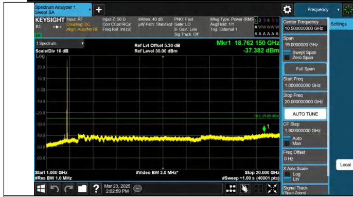
Band41-20MHz-QPSK-41490-1RB#99-1000~20000-PASS
