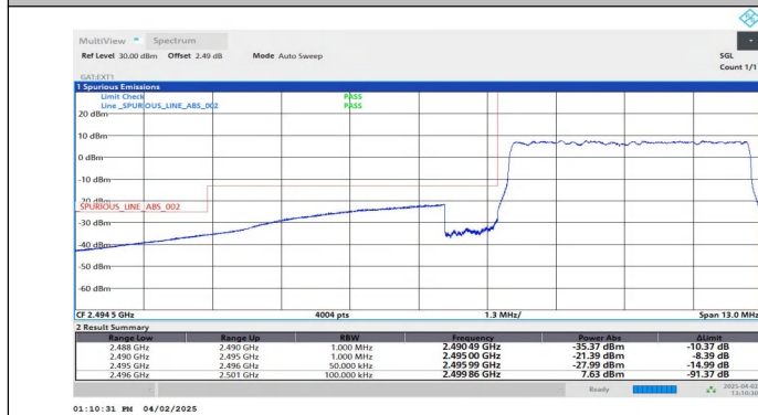
Band41-5MHz-QPSK-39675-25RB#0-PASS
