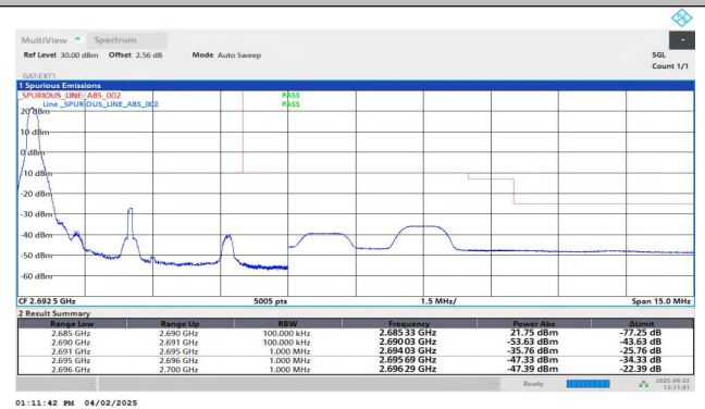
Band41-5MHz-QPSK-41565-1RB#0-PASS
