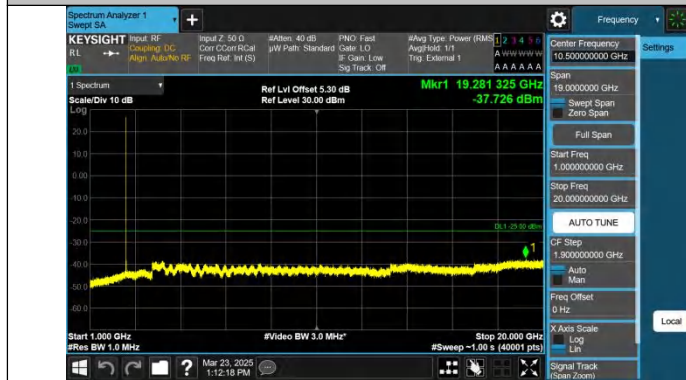
Band41-5MHz-QPSK-39675-1RB#24-1000~20000-PASS
