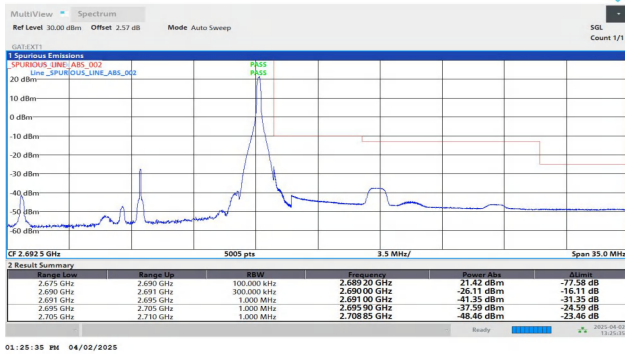
Band41-15MHz-QPSK-41515-1RB#74-PASS
