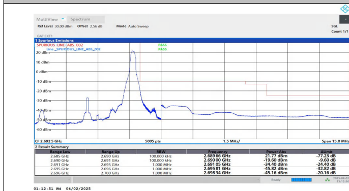
Band41-5MHz-QPSK-41565-1RB#24-PASS
