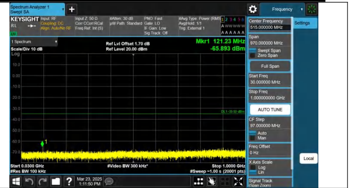
Band41-5MHz-QPSK-39675-1RB#24-30~1000-PASS
