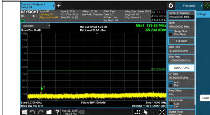
Band41-5MHz-QPSK-39675-1RB#0-30~1000-PASS
