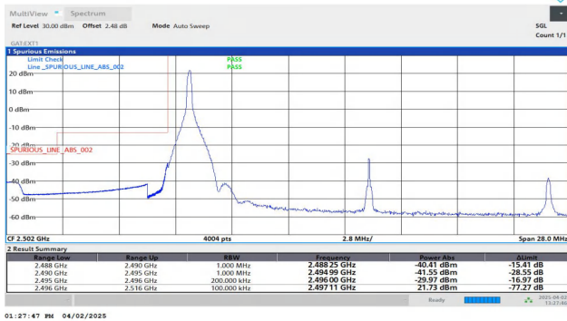
Band41-20MHz-QPSK-39750-1RB#0-PASS
