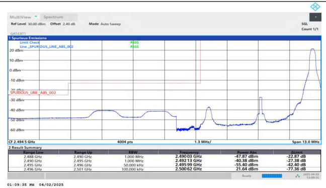
Band41-5MHz-QPSK-39675-1RB#24-PASS
