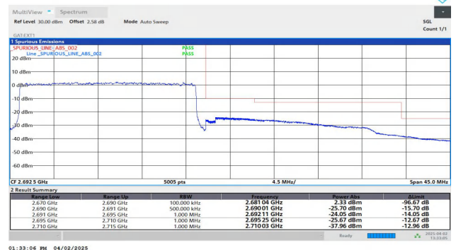
Band41-20MHz-QPSK-41490-100RB#0-PASS
