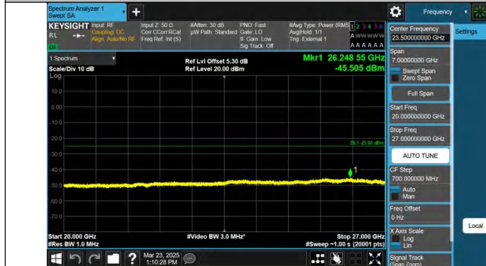
Band41-5MHz-QPSK-39675-1RB#0-20000~27000-PASS
