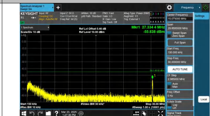
Band41-10MHz-QPSK-40620-1RB#0-0.15~30-PASS
