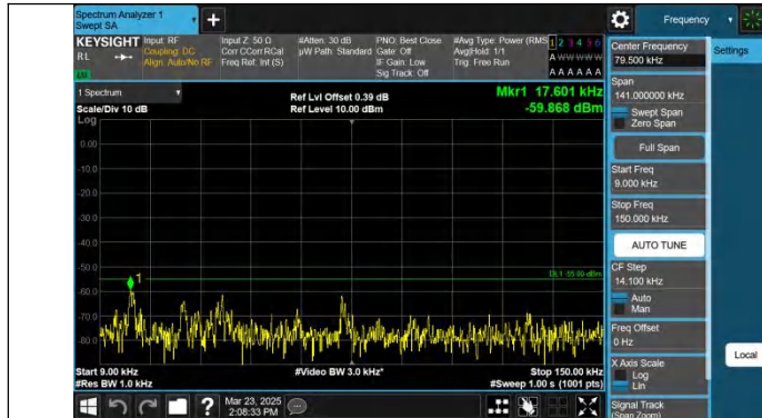
Band41-5MHz-QPSK-39675-1RB#0-0.009~0.15-PASS
