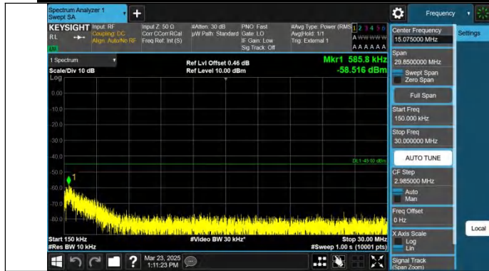
Band41-5MHz-QPSK-39675-1RB#24-0.15~30-PASS
