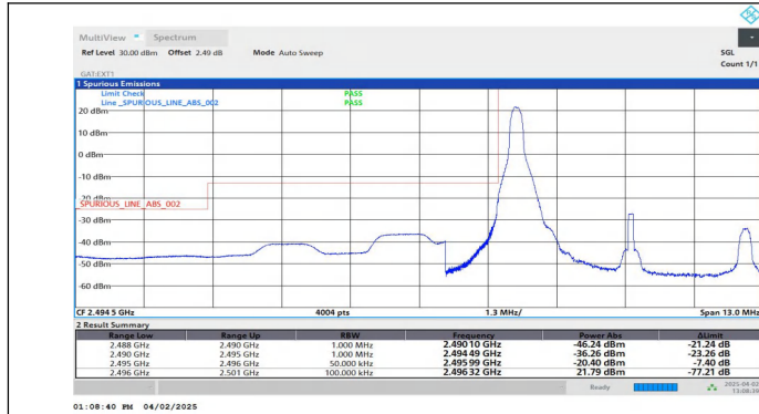
Band41-5MHz-QPSK-39675-1RB#0-PASS
