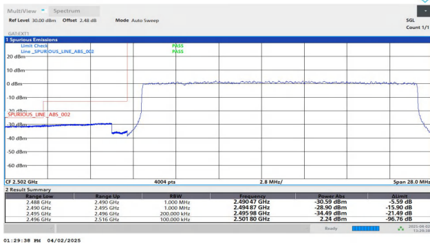
Band41-20MHz-QPSK-39750-100RB#0-PASS
