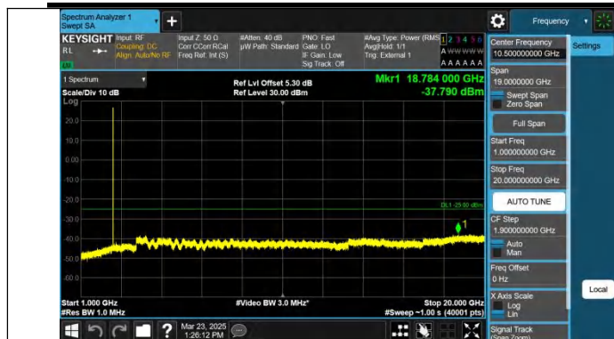
Band41-10MHz-QPSK-39700-1RB#49-1000~20000-PASS
