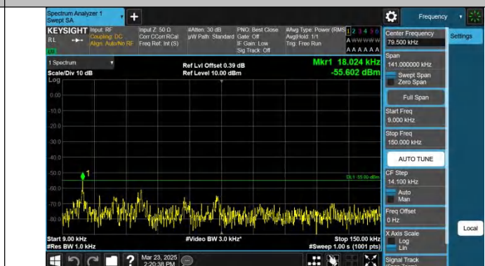
Band41-10MHz-QPSK-40620-1RB#49-0.009~0.15-PASS
