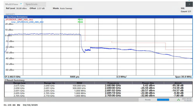
Band41-15MHz-QPSK-41515-75RB#0-PASS
