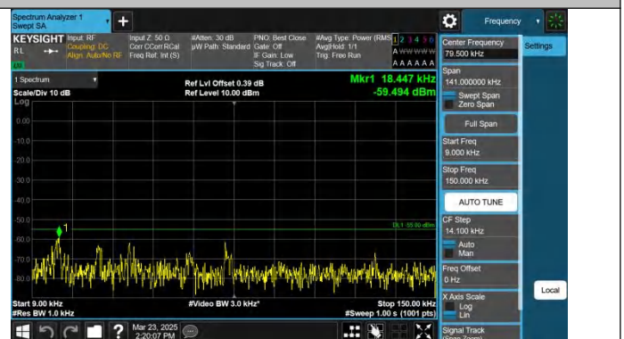
Band41-10MHz-QPSK-39700-1RB#49-0.009~0.15-PASS
