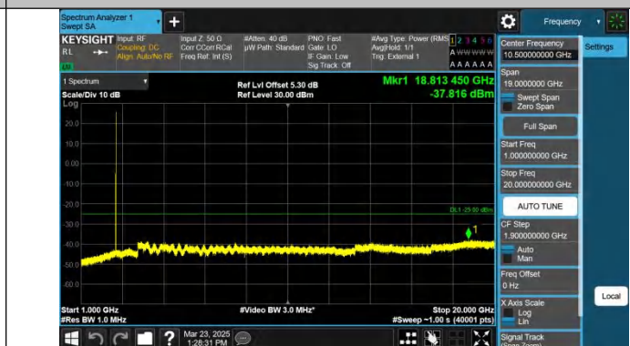
Band41-10MHz-QPSK-40620-1RB#0-1000~20000-PASS
