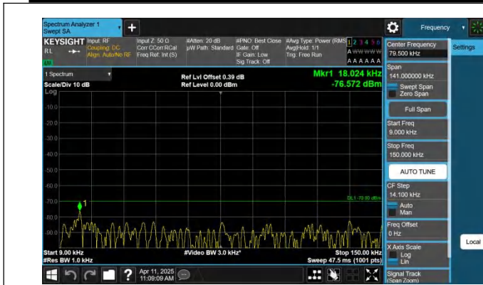
Band30-10MHz-QPSK-27710-1RB#0-0.009~0.15-PASS
