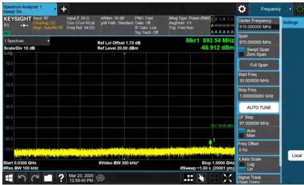
Band30-5MHz-QPSK-27710-1RB#0-30~1000-PASS
