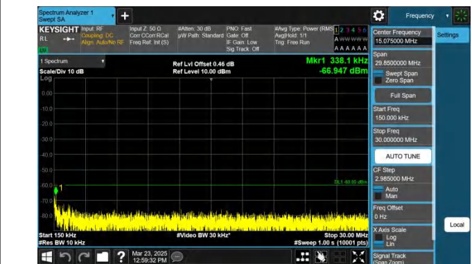
Band30-5MHz-QPSK-27710-1RB#0-0.15~30-PASS
