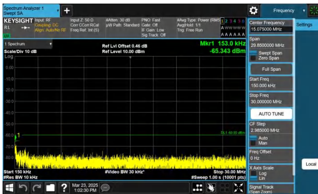
Band30-5MHz-QPSK-27735-1RB#24-0.15~30-PASS
