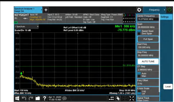
Band30-10MHz-QPSK-27710-1RB#0-0.15~30-PASS
