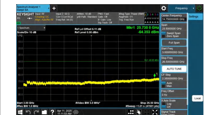
Band30-5MHz-QPSK-27685-1RB#24-3000~26500-PASS
