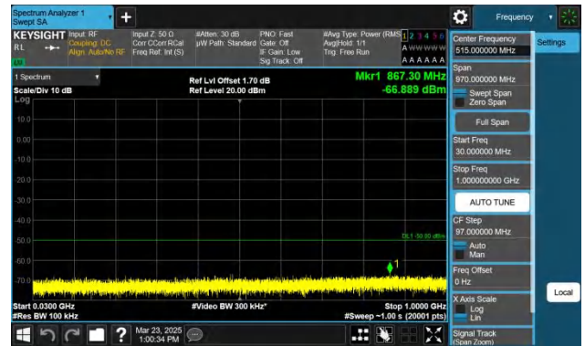
Band30-5MHz-QPSK-27710-1RB#24-30~1000-PASS
