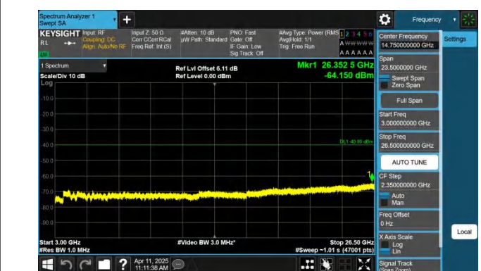
Band30-10MHz-QPSK-27710-1RB#49-3000~26500-PASS
