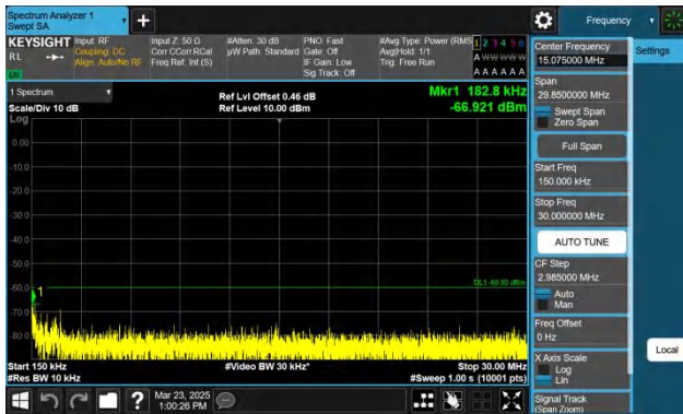
Band30-5MHz-QPSK-27710-1RB#24-0.15~30-PASS
