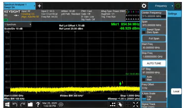
Band30-5MHz-QPSK-27735-1RB#24-30~1000-PASS
