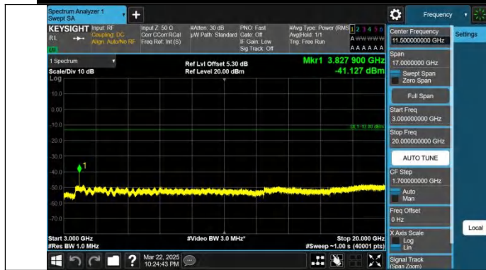
Band25-1.4MHz-QPSK-26683-1RB#0-3000~20000-PASS
