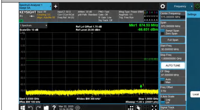
Band25-1.4MHz-QPSK-26683-1RB#0-30~1000-PASS
