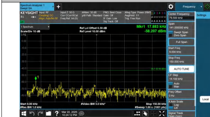
Band25-1.4MHz-QPSK-26683-1RB#0-0.009~0.15-PASS
