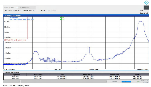
Band25-5MHz-QPSK-26065-1RB#24-PASS
