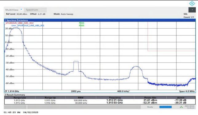
Band25-3MHz-QPSK-26675-1RB#0-PASS
