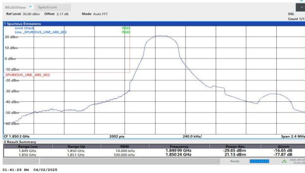
Band25-1.4MHz-QPSK-26047-1RB#0-PASS
