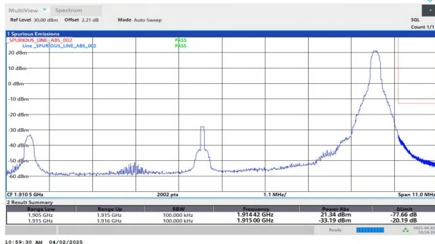
Band25-10MHz-QPSK-26640-1RB#49-PASS
