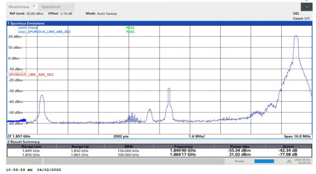
Band25-15MHz-QPSK-26115-1RB#74-PASS
