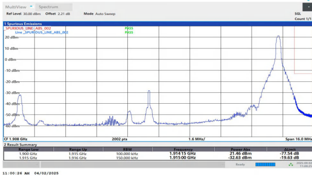
Band25-15MHz-QPSK-26615-1RB#74-PASS
