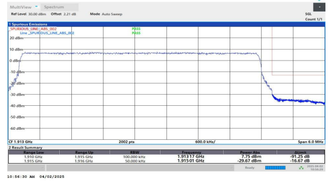
Band25-5MHz-QPSK-26665-25RB#0-PASS
