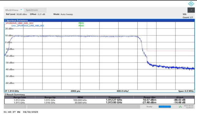
Band25-3MHz-QPSK-26675-15RB#0-PASS
