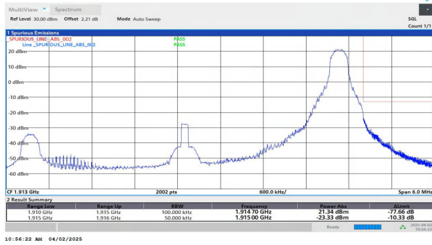
Band25-5MHz-QPSK-26665-1RB#24-PASS
