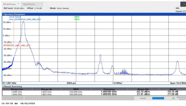
Band25-15MHz-QPSK-26115-1RB#0-PASS
