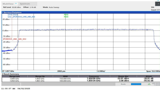
Band25-15MHz-QPSK-26115-75RB#0-PASS
