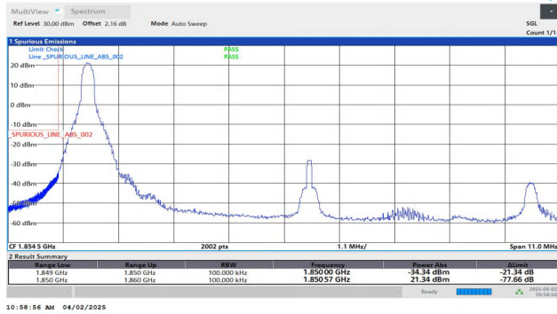
Band25-10MHz-QPSK-26090-1RB#0-PASS
