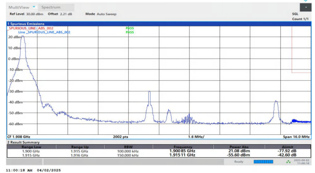
Band25-15MHz-QPSK-26615-1RB#0-PASS
