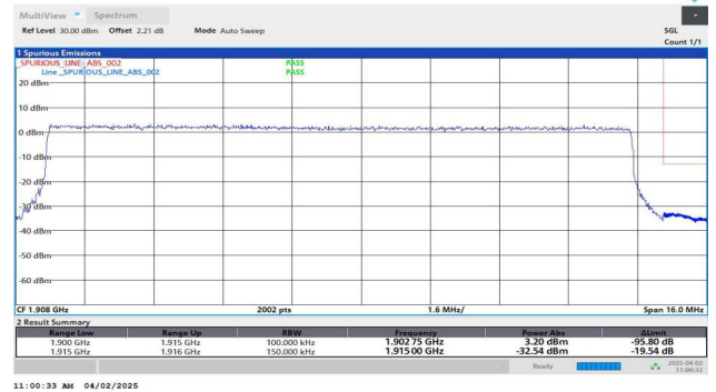
Band25-15MHz-QPSK-26615-75RB#0-PASS
