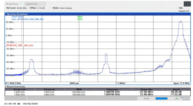
Band25-10MHz-QPSK-26090-1RB#49-PASS
