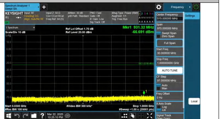
Band25-1.4MHz-QPSK-26683-1RB#5-30~1000-PASS
