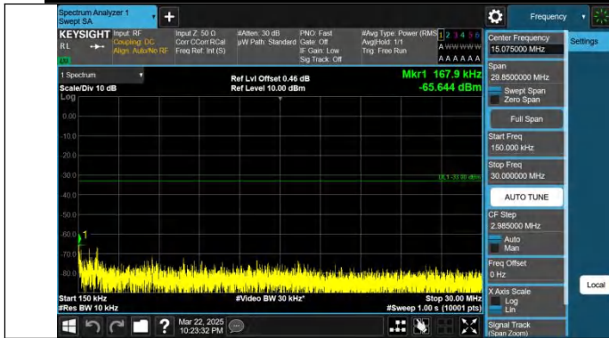
Band25-1.4MHz-QPSK-26365-1RB#5-0.15~30-PASS
