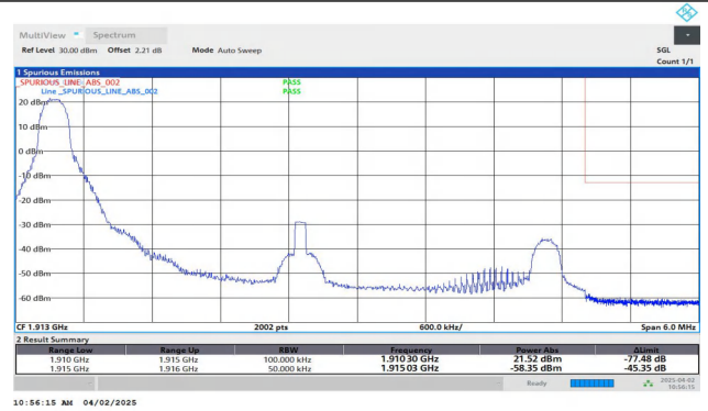
Band25-5MHz-QPSK-26665-1RB#0-PASS
