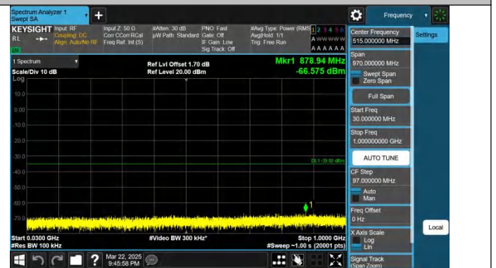
Band7-20MHz-QPSK-21350-1RB#99-30~1000-PASS
