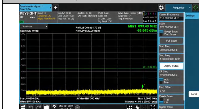
Band7-15MHz-QPSK-21375-1RB#0-30~1000-PASS
