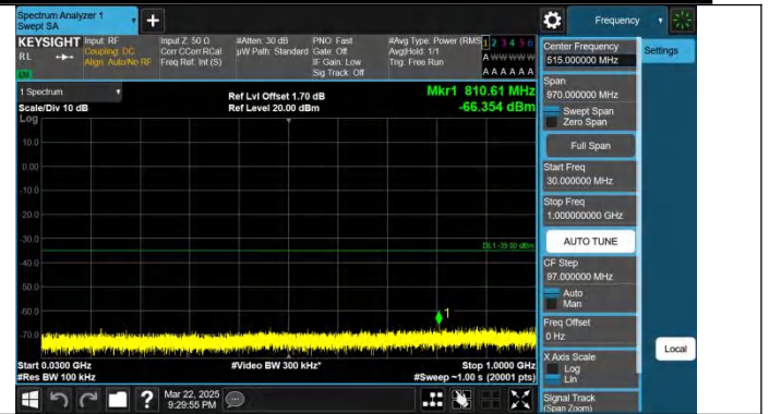
Band7-10MHz-QPSK-21400-1RB#49-30~1000-PASS
