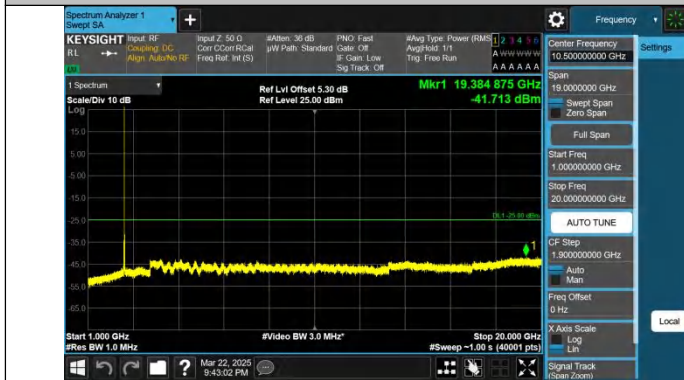
Band7-20MHz-QPSK-20850-1RB#99-1000~20000-PASS
