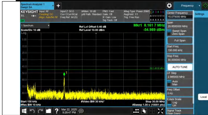
Band7-10MHz-QPSK-21400-1RB#49-0.15~30-PASS
