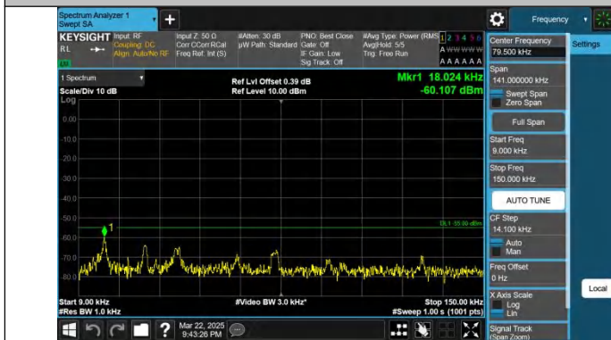
Band7-20MHz-QPSK-21100-1RB#0-0.009~0.15-PASS
