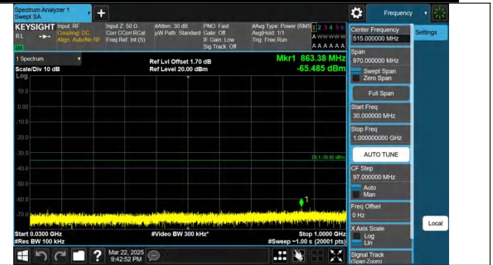
Band7-20MHz-QPSK-20850-1RB#99-30~1000-PASS
