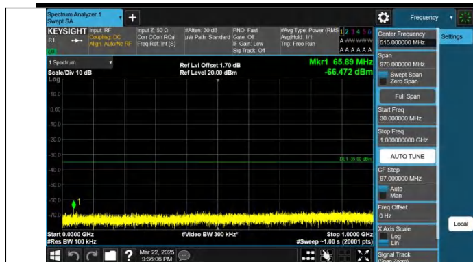
Band7-15MHz-QPSK-21100-1RB#0-30~1000-PASS
