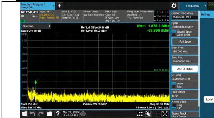
Band7-20MHz-QPSK-20850-1RB#99-0.15~30-PASS
