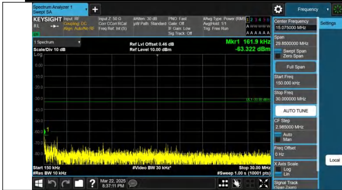
Band4-10MHz-QPSK-20000-1RB#49-0.15~30-PASS
