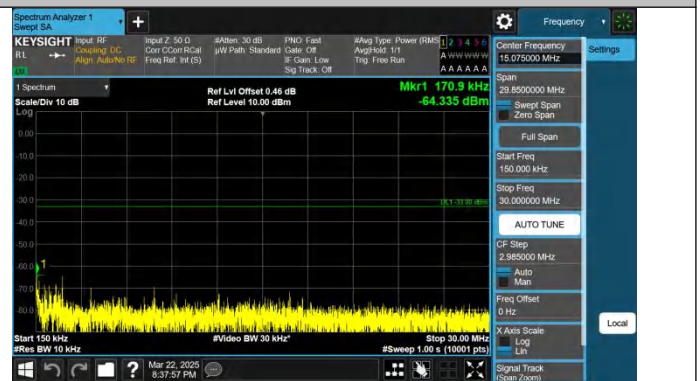
Band4-10MHz-QPSK-20175-1RB#0-0.15~30-PASS
