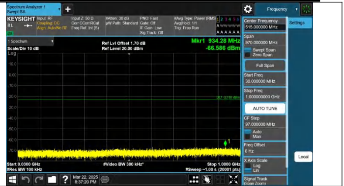
Band4-10MHz-QPSK-20000-1RB#49-30~1000-PASS
