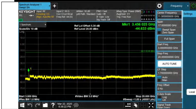
Band4-10MHz-QPSK-20175-1RB#0-3000~20000-PASS
