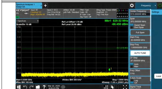
Band4-20MHz-QPSK-20300-1RB#0-30~1000-PASS
