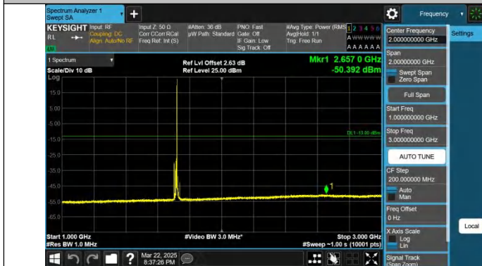
Band4-10MHz-QPSK-20000-1RB#49-1000~3000-PASS
