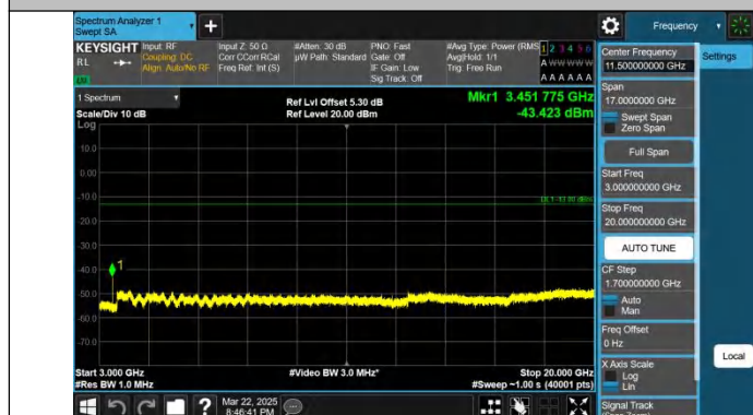
Band4-15MHz-QPSK-20175-1RB#0-3000~20000-PASS
