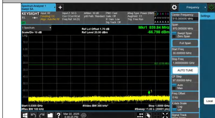
Band4-15MHz-QPSK-20175-1RB#0-30~1000-PASS
