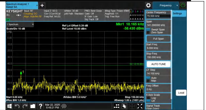
Band4-15MHz-QPSK-20325-1RB#74.0.009~0.15-PASS
