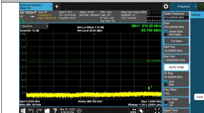
Band4-10MHz-QPSK-20175-1RB#0-30~1000-PASS
