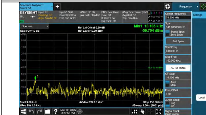
Band4-10MHz-QPSK-20175-1RB#0-0.009~0.15-PASS
