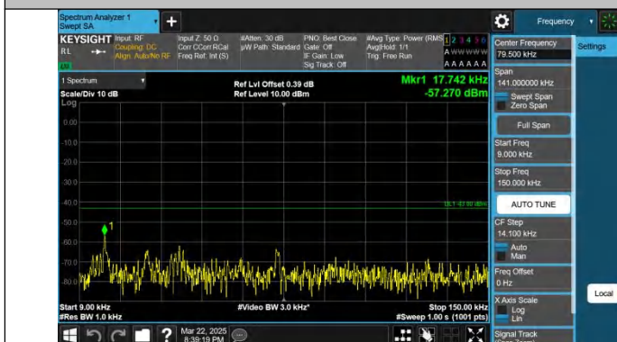
Band4-10MHz-QPSK-20350-1RB#0-0.009~0.15-PASS
