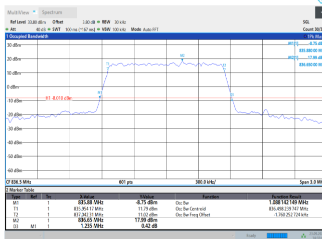
Band26-1.4MHz-QPSK-26915-6RB#0
